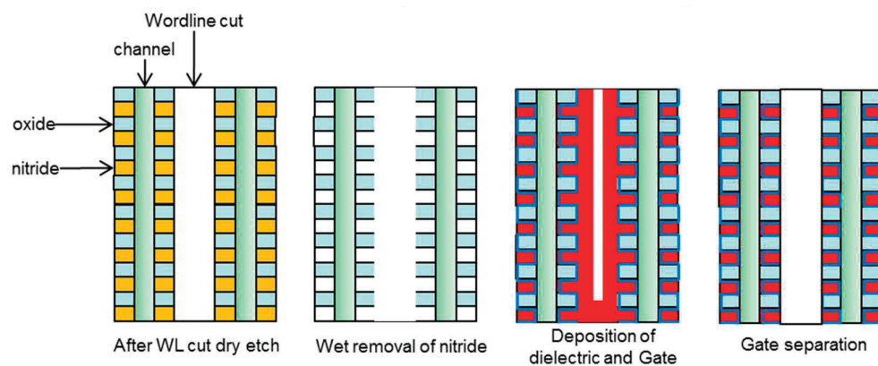
Figure 8. TCAT/V-NAND process.
