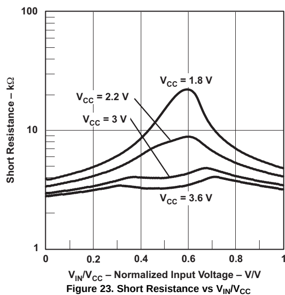
Figure 23. Short Resistance vs V_{IN}/V_{CC}
