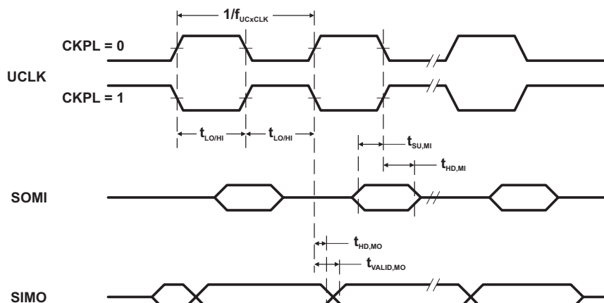
Figure 16. SPI Master Mode, CKPH = 0
