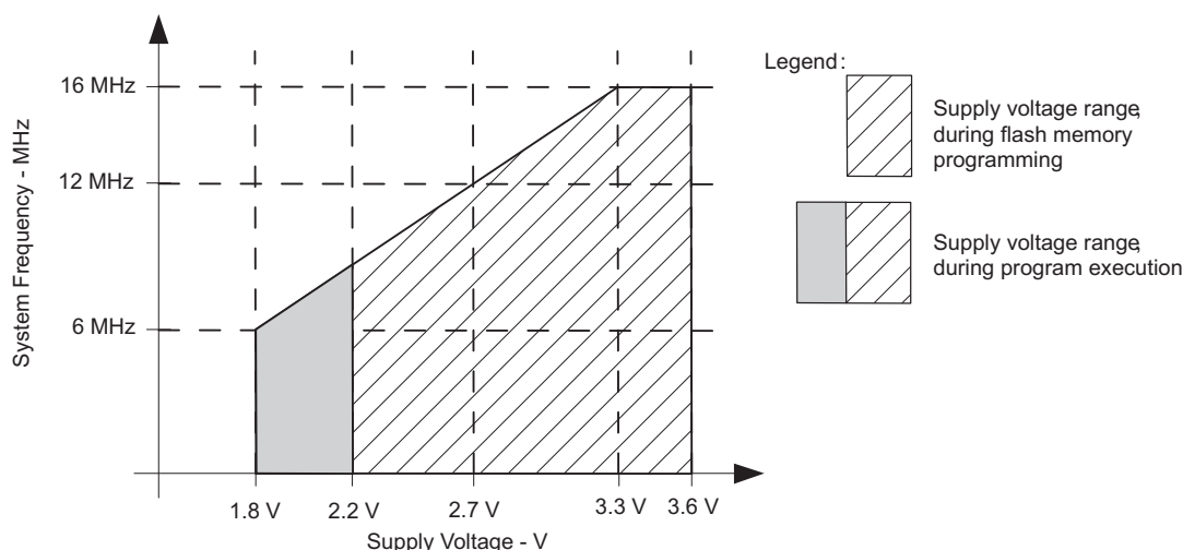
Figure 1. Safe Operating Area
