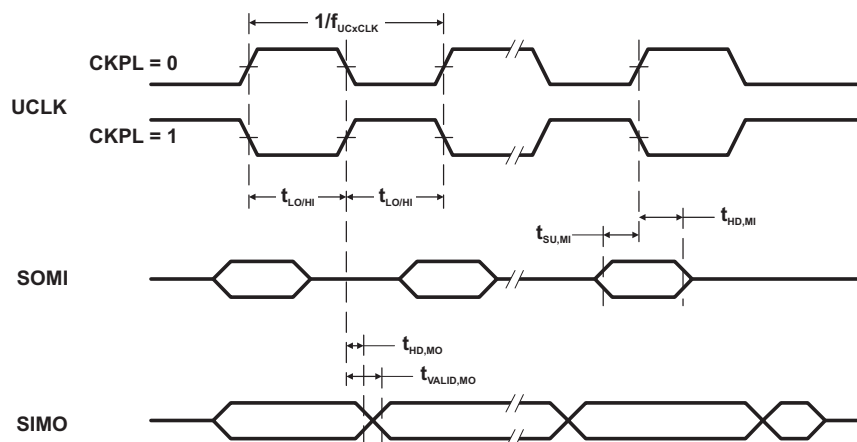
Figure 17. SPI Master Mode, CKPH = 1
