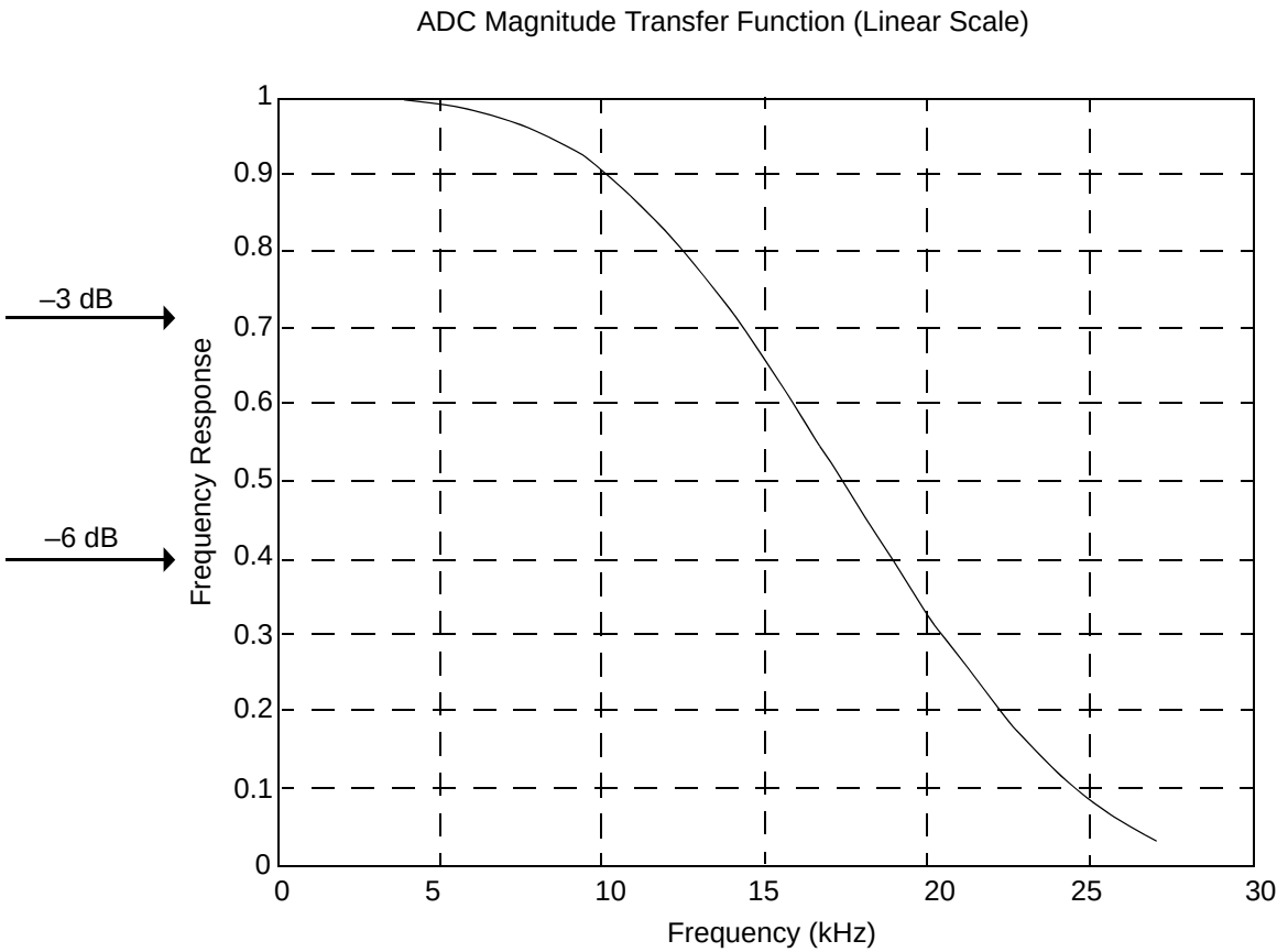
Figure 49. Analog-to-Digital Converter Frequency Response
