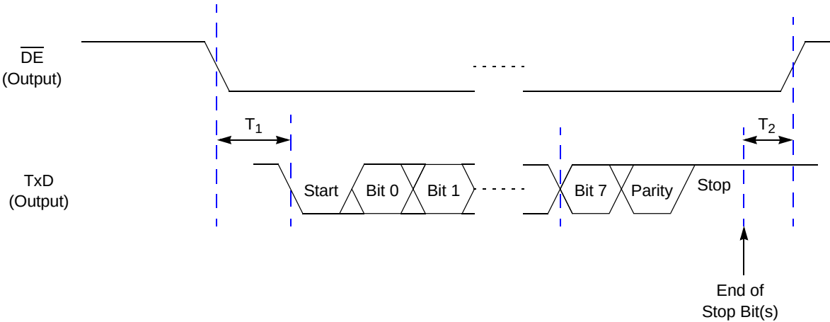
Figure 57. UART Timing without \overline{\text{CTS}}
