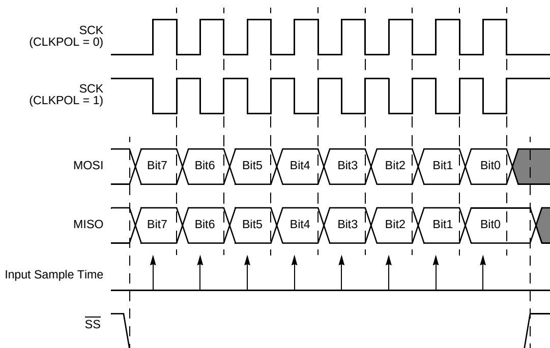
Figure 25. SPI Timing When PHASE is 0
