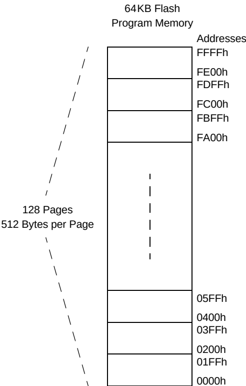
Figure 35. Flash Memory Arrangement
