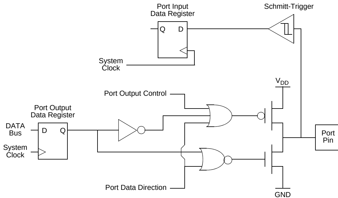
Figure 10. GPIO Port Pin Block Diagram
