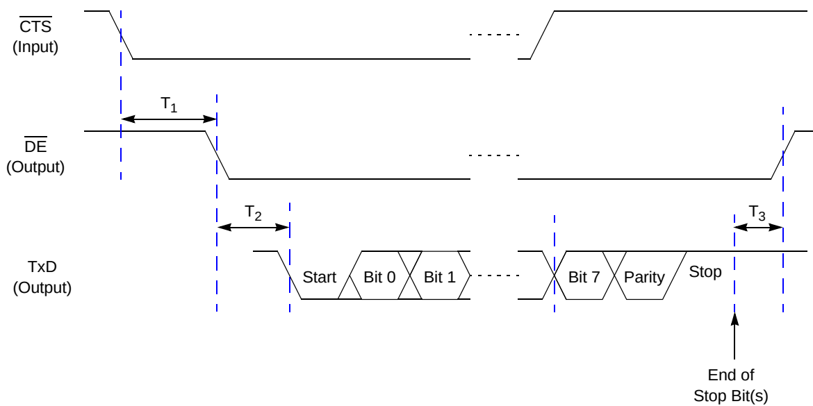
Figure 56. UART Timing with \overline{\text{CTS}}
