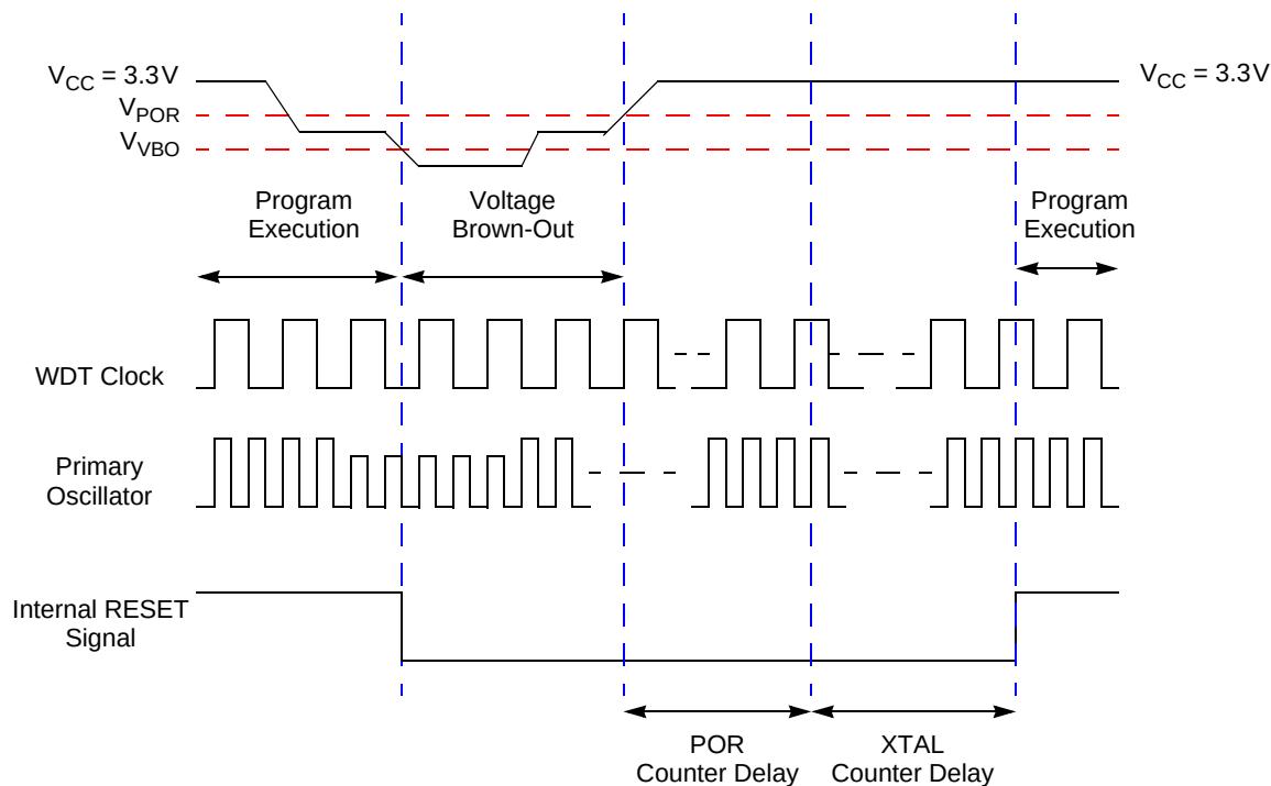
Figure 9. Voltage Brown-Out Reset Operation
