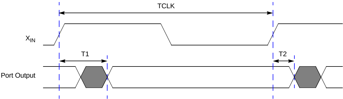
Figure 51. GPIO Port Output Timing
