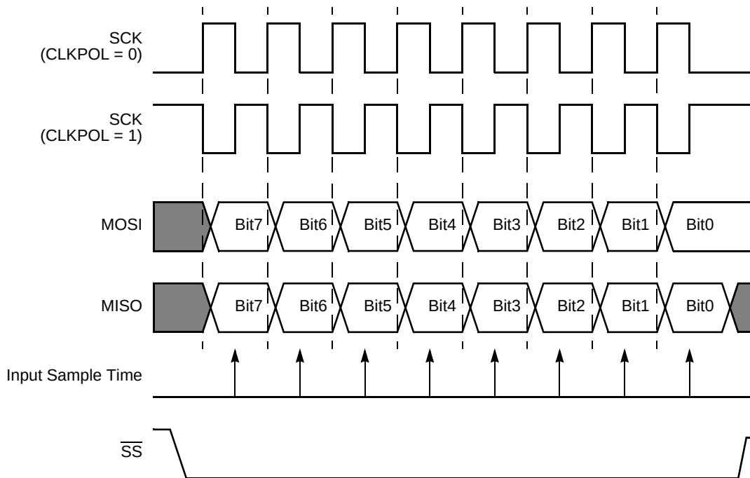
Figure 26. SPI Timing When PHASE is 1
