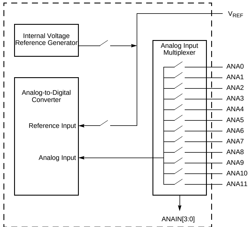
Figure 34. Analog-to-Digital Converter Block Diagram
