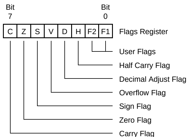
Figure 58. Flags Register
