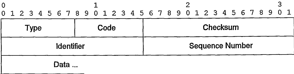
ICMP Packet - Echo or Echo Reply Message
