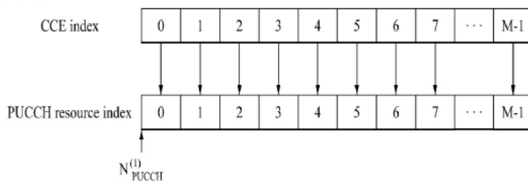
(a) M CCEs to M PUCCH resources mapping
