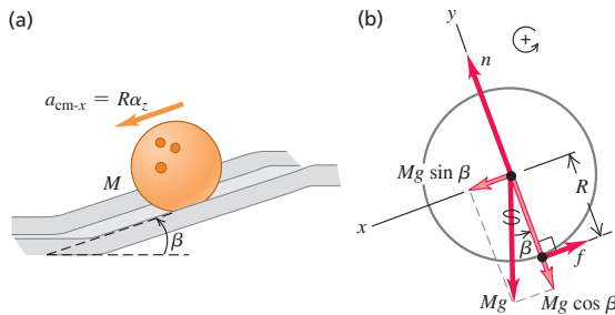
Figure 10.19 A bowling ball rolling down a ramp.
