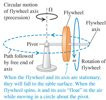
Figure 10.32 A gyroscope supported at one end. The horizontal circular motion of the flywheel and axis is called precession. The angular speed of precession is \Omega .
