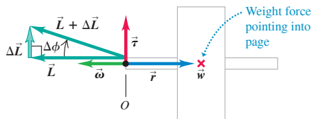
(b) Vector diagram
