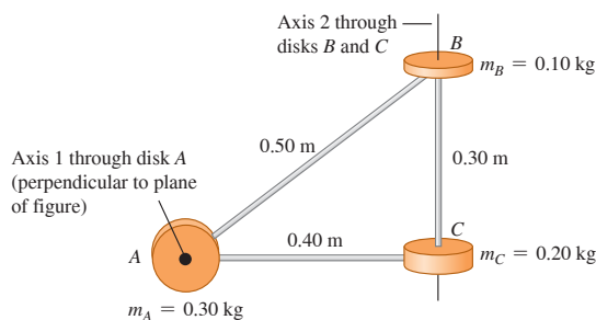
Figure 9.15 An oddly shaped machine part.
