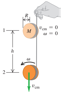
Figure 10.15 Calculating the speed of a primitive yo-yo.
