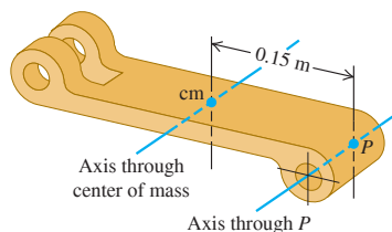
Figure 9.21 Calculating I_{cm} from a measurement of I_P .
