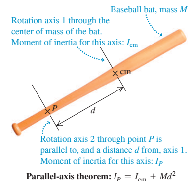
Figure 9.19 The parallel-axis theorem.
