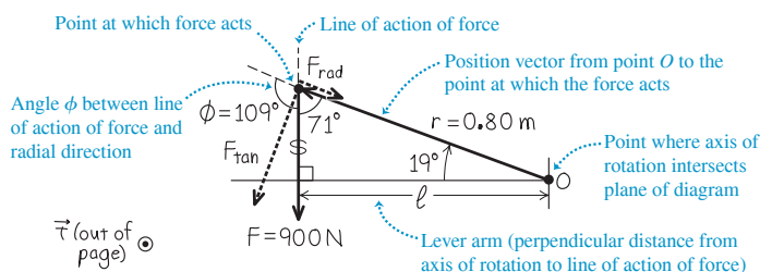
(b) Free-body diagram
