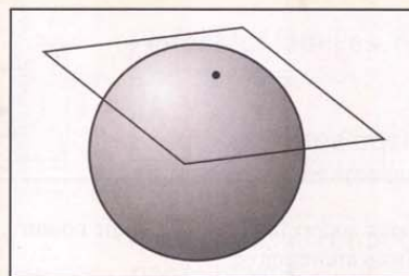
Tangent plane to a sphere
