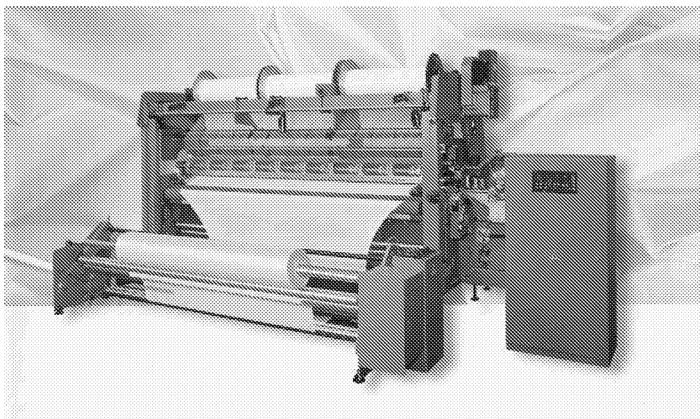
Fig. 23.2 Tricot machine HKS 2-3 [Karl Mayer].
