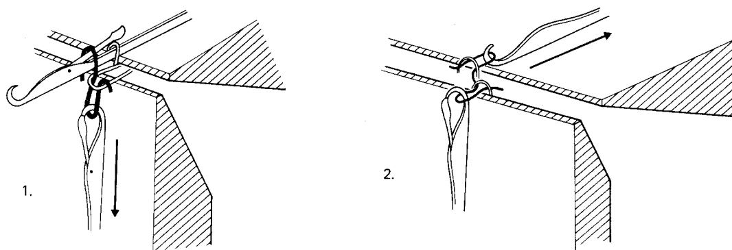
Fig. 7.13 Delayed timing.
