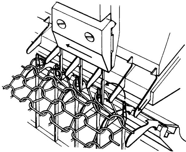
Fig. 17.4 Fashioning points.
