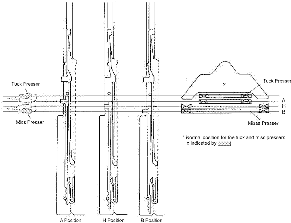
Fig. 19.4 Presser cams.
