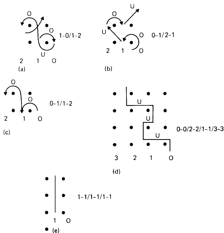
Fig. 23.5 Overlap/underlap variations.
