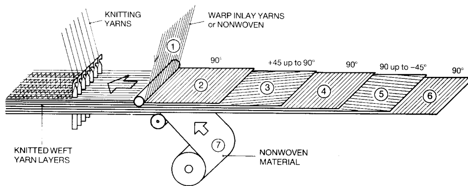
Fig. 30.3 Principle of the LIBA multi-axial magazine weft insertion warp knitting machine. Up to 6 yarn layers and one fleece layer are possible [LIBA].
