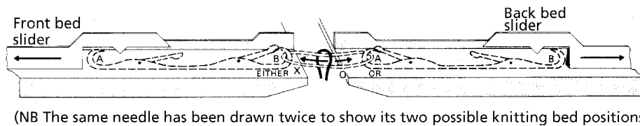
Fig. 7.17 Purl knitting using sliders.
