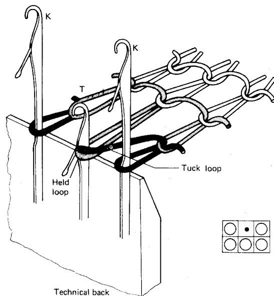
Fig. 9.4 Tuck stitch produced on a latch-needle machine.
