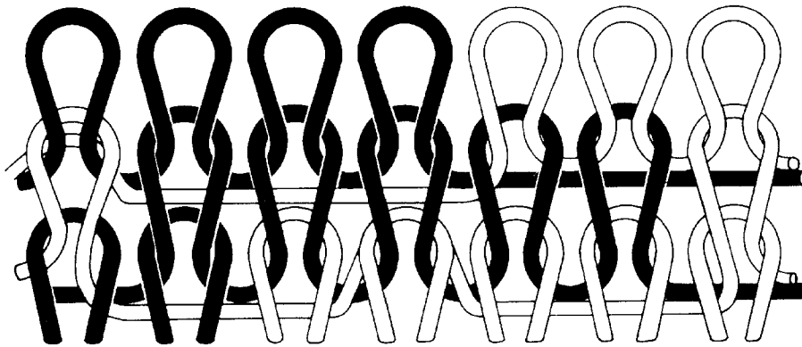
Fig. 10.5 Accordion fabric.
