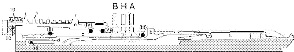
Fig. 19.3 Knitting elements.
