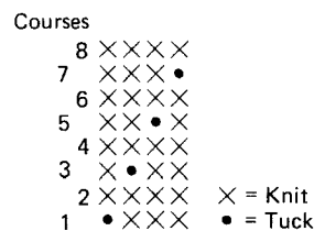
Fig. 21.2 Notation of 3 × 1 micromesh . Petitioner adidas AG - Exhibit 1012 - Page 288
