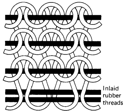
Fig. 16.3 Accordion welt top.
