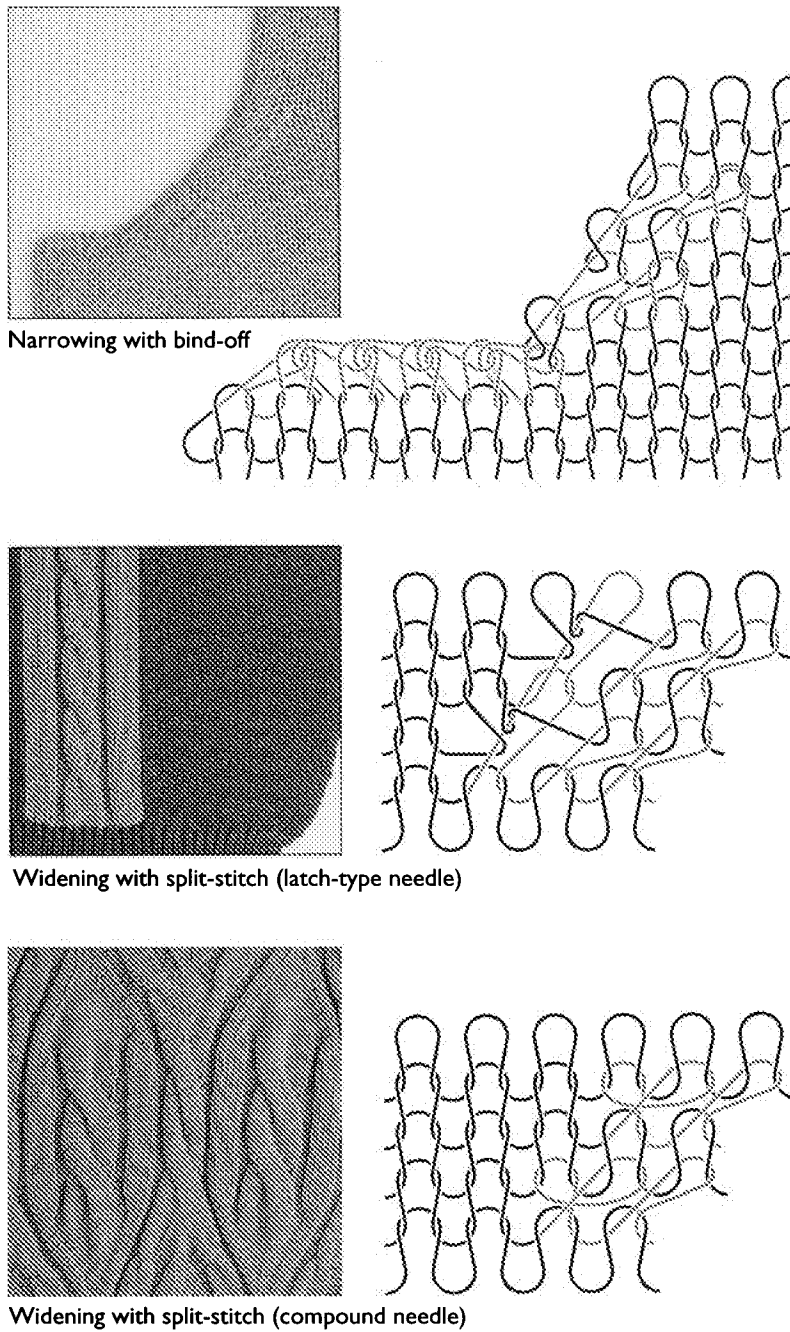
Fig. 16.10 Modern integral garment technology assures precisely-formed loops which are crucial to the production of shaped garments [Shima Seiki].
