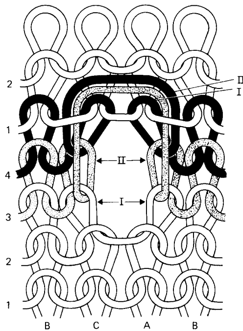
Fig. 15.5 Pelerine stitch.
