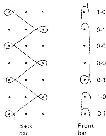
Fig. 26.1 Miss-lapping.
