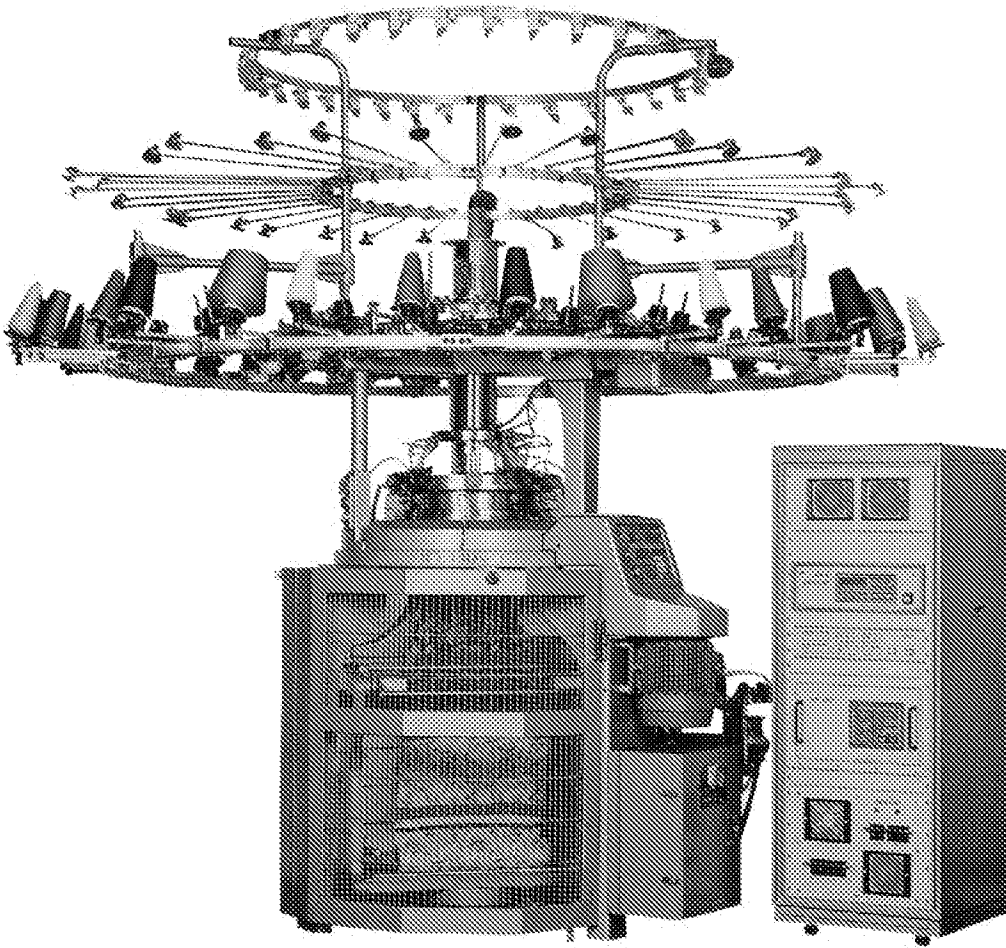
Fig. 12.1 Electronic sampling machine [Monarch].
