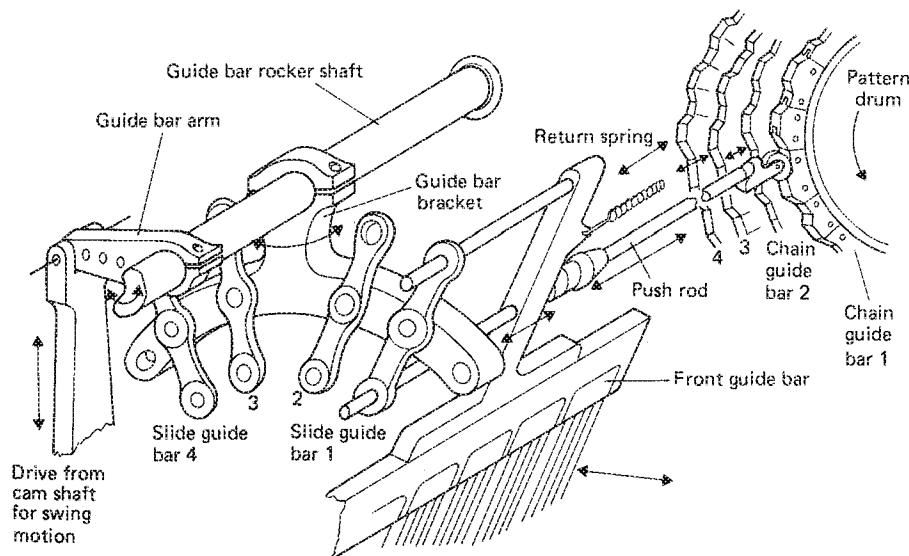
Fig. 23.3 Guide bar swinging and shogging mechanism [Reprinted by permission of Knitting Times , official publication of the NSKA in the USA] Petitioner adidas AG - Exhibit 1012 - Page 315
