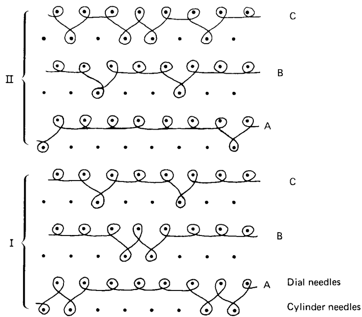
(c)(i) Rib Jacquard with horizontally striped backing
