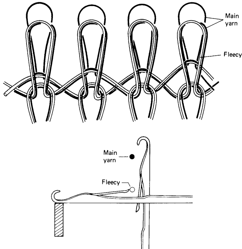
Fig. 14.3 Fleecy interlock.
