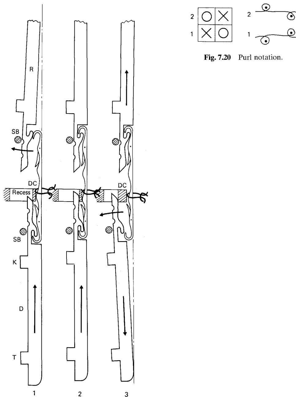
Fig. 7.19 Purl needle transfer action.
