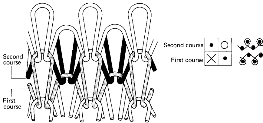
Fig. 18.6 Full cardigan.
