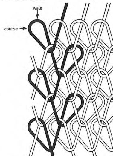
Above Warp knitting
