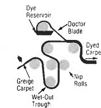
Küster Carpet Dyeing Range
