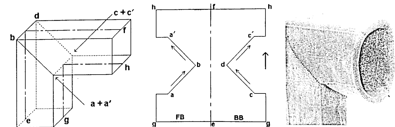
(2) 2D Pattern
