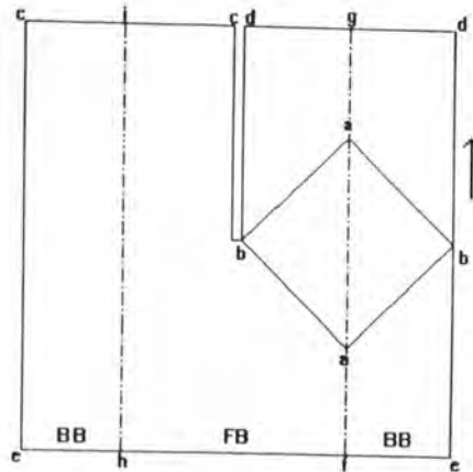
(2) 2D Pattern
