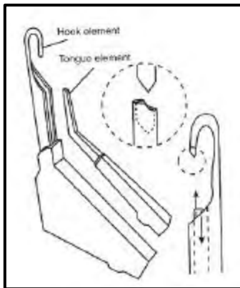
Figure 7.1.3.4a. Compound needle (Kadolph and Langford, 1998)
