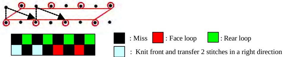
Figure 7.1.2c. Loop transference on front bed for seamless garment knitting
