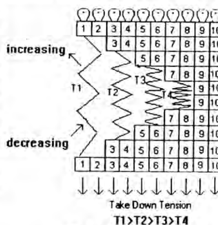
Fig.1 - Fashioning operation: decreasing and increasing the number of knitting needles in one needle bed
