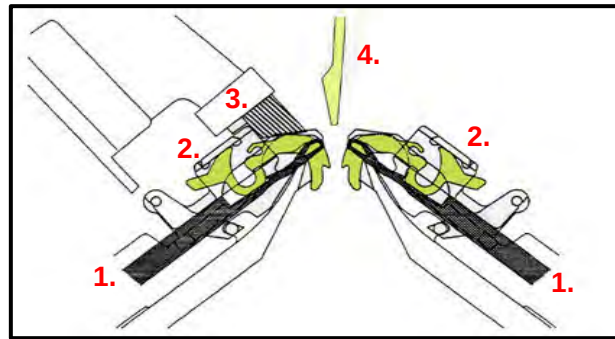
Figure 1.1e. Knitting machine system on flat V-bed machine (Shima Seiki Manual [37])
