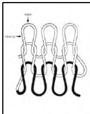
Figure 1.1a. Weft knitting
