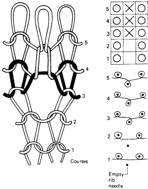
Fig. 9.6 Commencing knitting on an empty rib needle.
