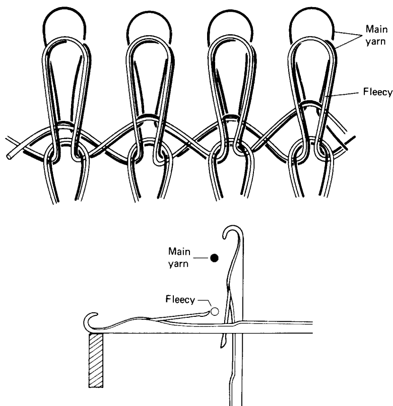
Fig. 14.3 Fleecy interlock.
