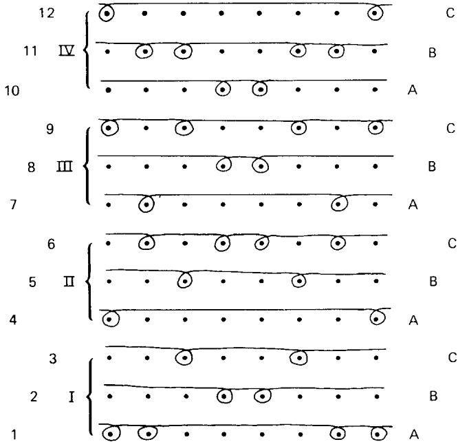
(a) Single jersey knit/miss Jacquard
