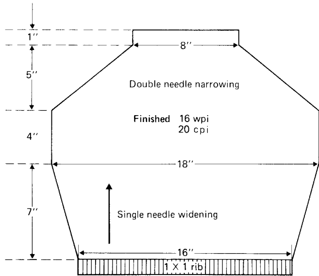
Fig. 16.11 Full-fashioned shaping calculation.
