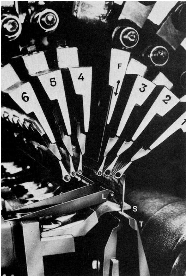
Fig. 27.2 Multi-purpose fall-plate raschel machine [Karl Mayer]. Bars 1, 2, 3 – fall-plate guide bars; bar 4 – knitting guide bar; bars 5, 6 – inlay guide bars. L = latch opening wire; S = holding-down sinker; T = trick plate; F = fall-plate.
