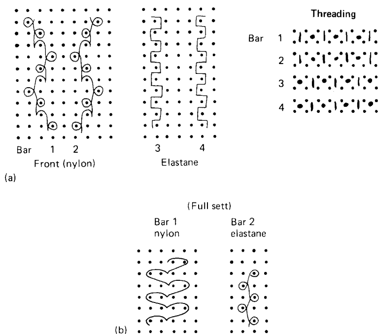
Fig. 28.12 Elastane fabrics.
