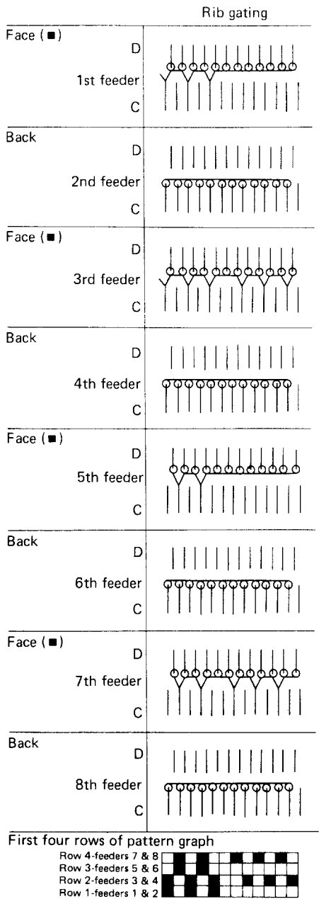
Fig. 13.9 Tuck lace.
