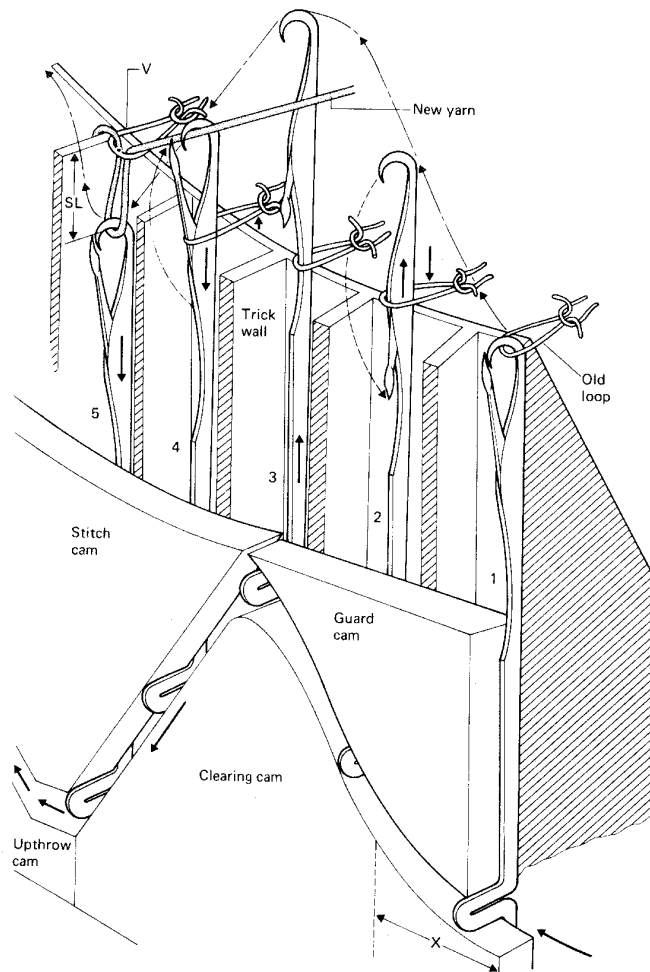
Fig. 3.4 Knitting action of the latch needle.
