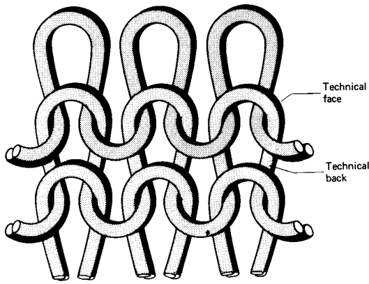
Fig. 6.10 Plating in weft knitting.
