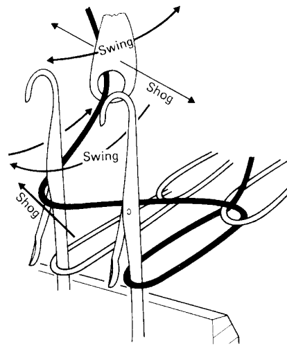
Fig. 4.3 Loop forming by warp guides.
