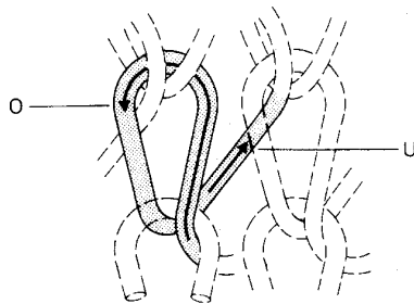
Fig. 5.4 The closed lap.
