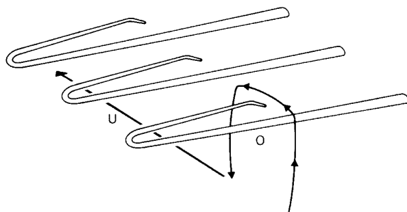
Fig. 5.2 Overlapping and underlapping (warp knitting).
