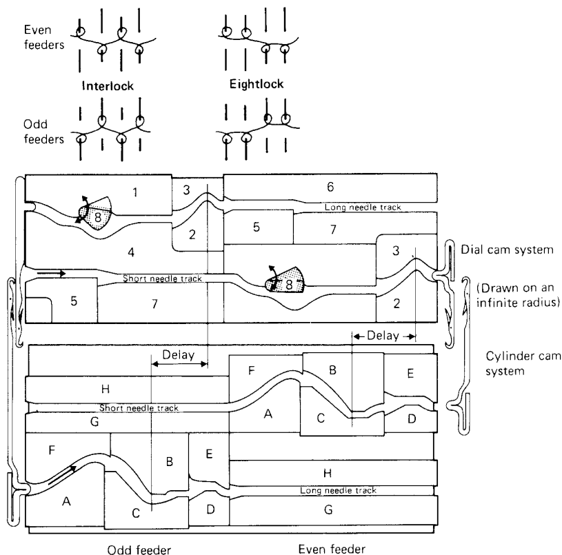
Fig. 7.16 Interlock cam system.
