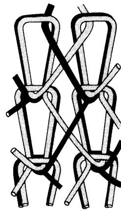
Fig. 6.11 Plating in warp knitting.
