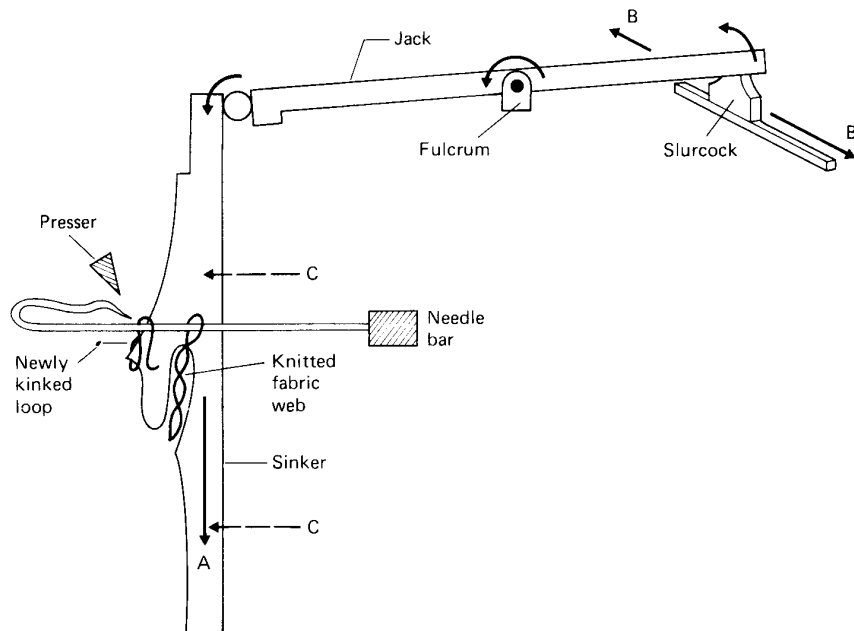
Fig. 2.3 The action of frame knitting.
