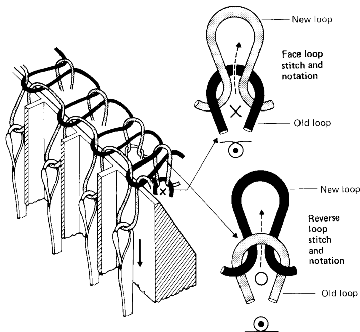
Fig. 5.8 Face- and reverse-meshed loops.
