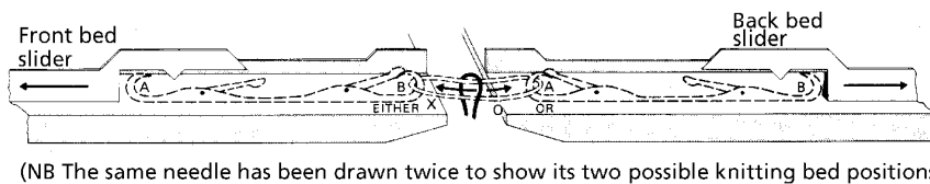
Fig. 7.17 Purl knitting using sliders.
