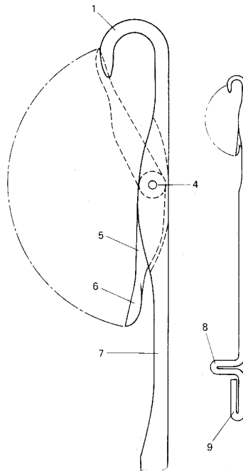
Fig. 3.3 Main features of the latch needle.
