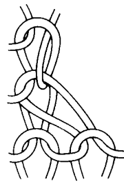
Fig. 6.8 Weft knitted loop transfer.
