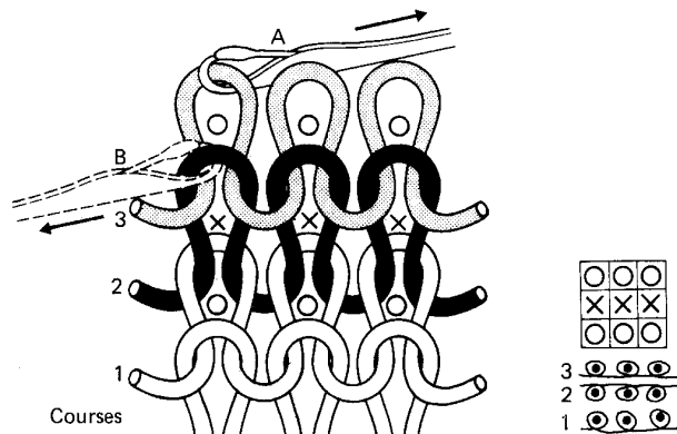
Fig. 7.18 Purl fabric structure.
