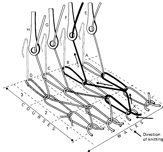
Fig. 6.2 Warp knitting.
