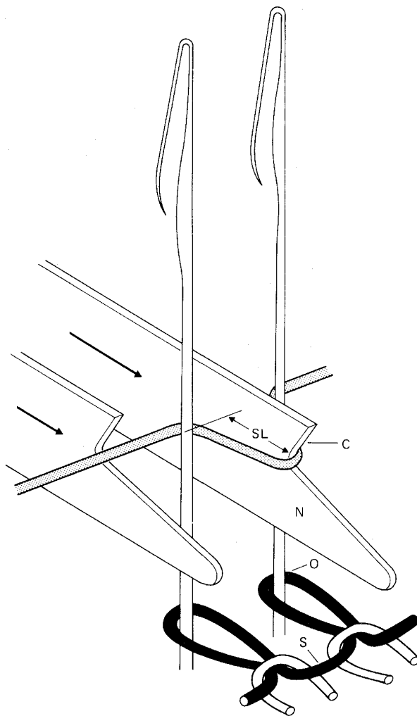
Fig. 4.1 Action of the loop-forming sinker.
