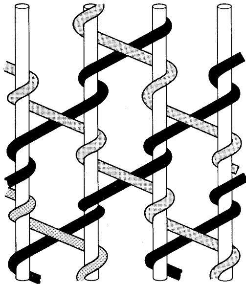
Fig. 1.2 Intertwining and twisting.
