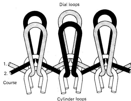
Fig. 7.14 Interlock fabric structure.
