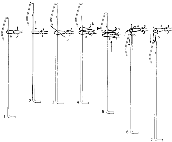
Fig. 3.1 Basic knitting action of a needle.
