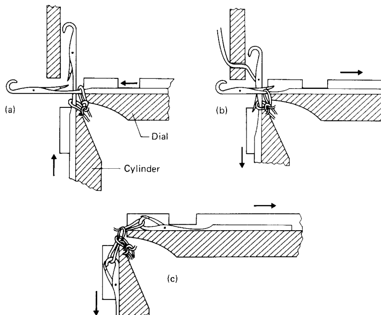
Fig. 7.10 Knitting action of a circular rib machine.
