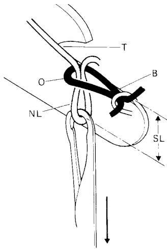
Fig. 4.2 Action of the knock-over sinker.
