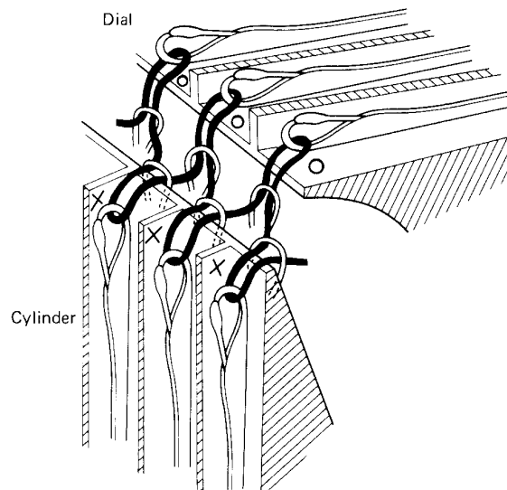
Fig. 7.7 Structure of 1 \times 1 rib.
