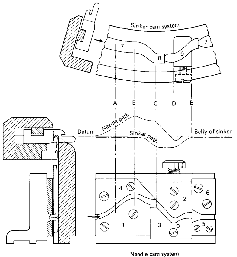
Fig. 7.6 Sinker timing on a single jersey machine.
