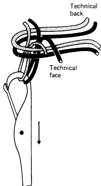
Fig. 6.9 The plating relationship of two yarns.
