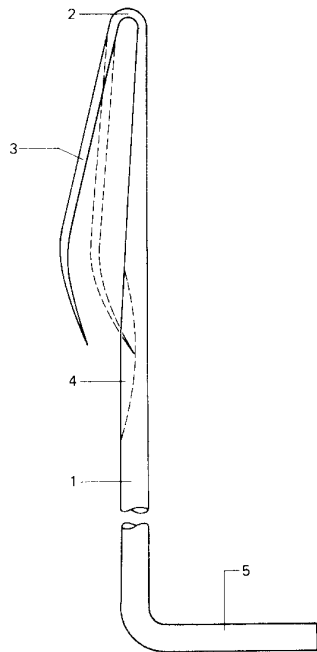
Fig. 3.2 Main parts of the bearded needle.
