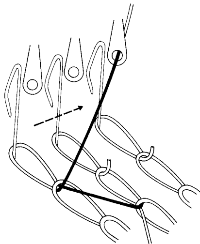
Fig. 5.3 The underlap shog.
