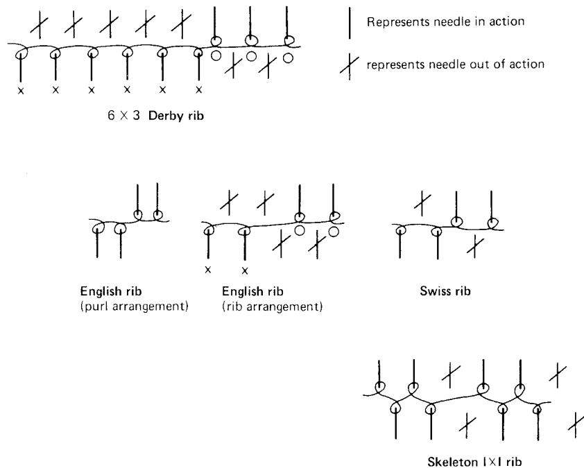
Fig. 7.9 Rib set-outs.
