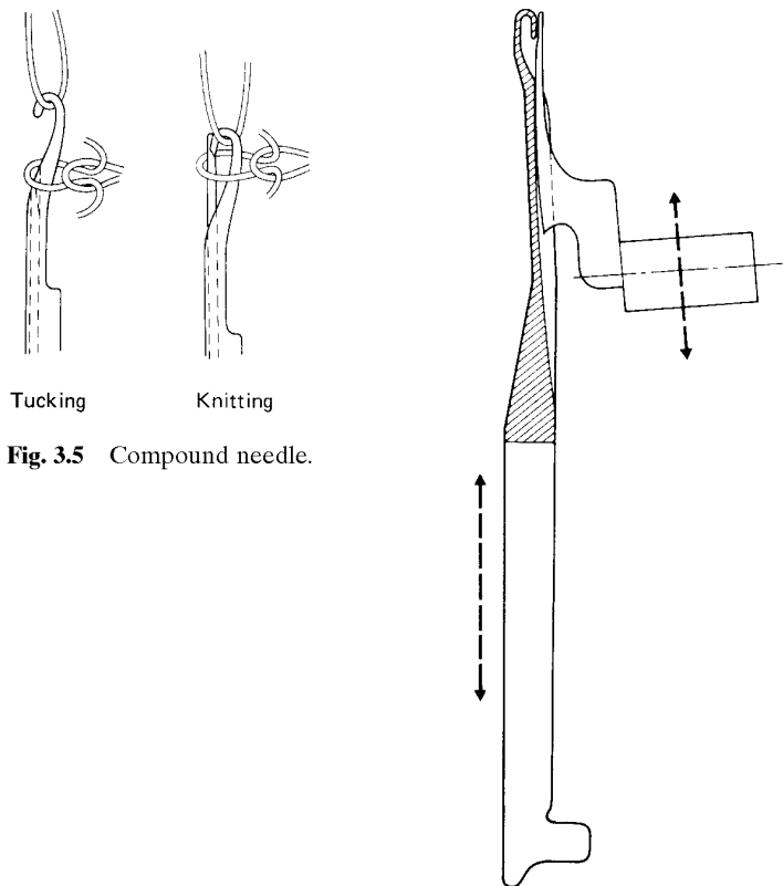
Fig. 3.6 Open-stem slide needle.
