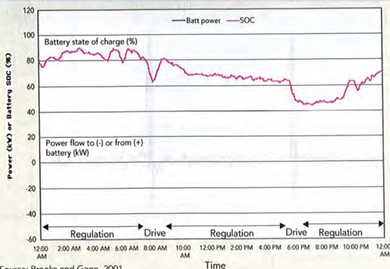
Figure 2: Power Flow and State of Charge How an electric vehicle provides regulation services.
