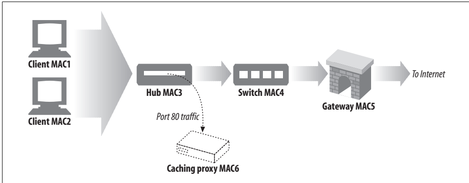
Figure 20-7. MAC forwarding using a layer-4 switch
