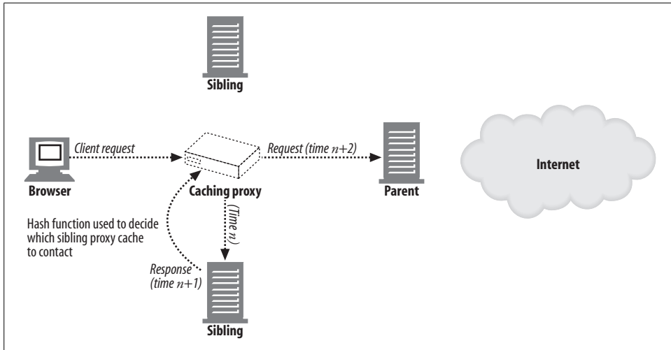
Figure 20-14. CARP redirection
