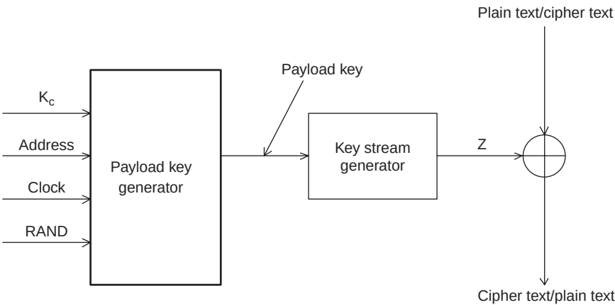
Figure 14.3 Bluetooth encryption.
