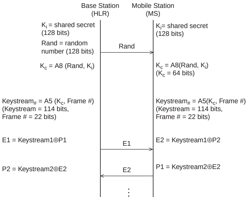
Figure 17.4 GSM encryption.
