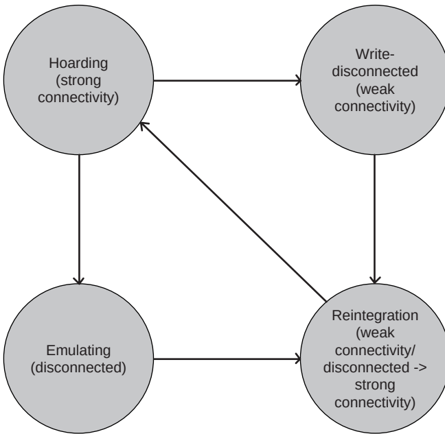
Figure 1.3 State transition used by a coda client (venus) to adapt its functionality to changes in connectivity to a server (venus states hoarding, write disconnected, emulating and reintegration correspond to strong connectivity, weak connectivity, and no connectivity (disconnected), respectively. The reintegration state corresponds to transition to strong connectivity from no/weak connectivity link state.
