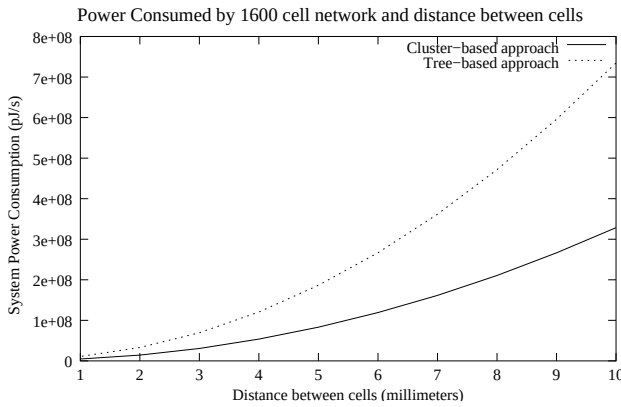
Figure 12: Power consumption vs. distance between nodes for Tree-based and Cluster-based approaches.
