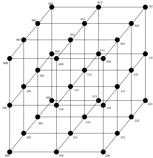
Figure 7: 3D Topology with 6 Neighbors
