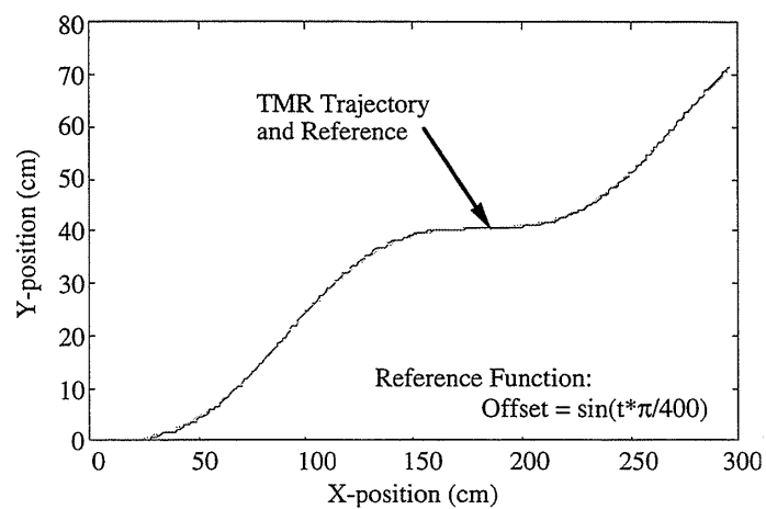
Figure 5-1 Closed-Loop Test Using Table Data as Reference
