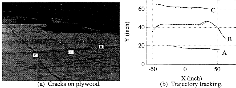
Figure 8-4. Crack Tracking Test Example
