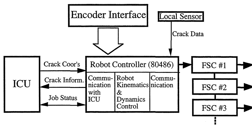
Figure 3-6. General Control System Configuration
