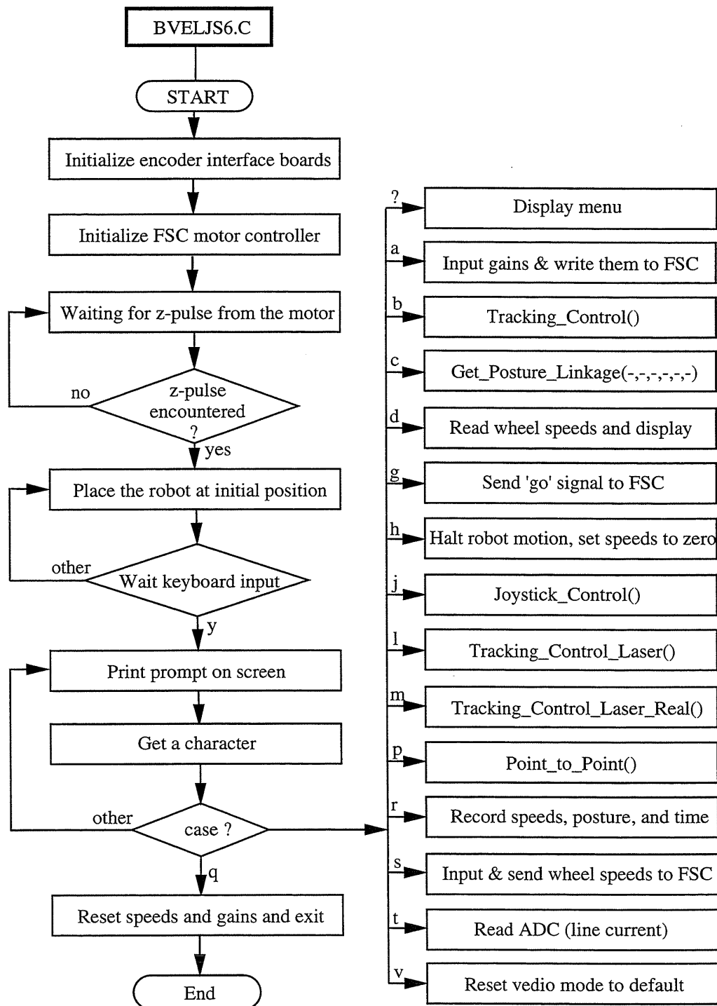
Figure 7-1a. Flow Chart of Control Program, Main Program
