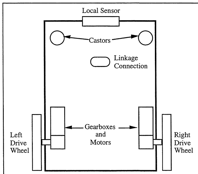
Figure 3-2. Conceptual TMR Layout
