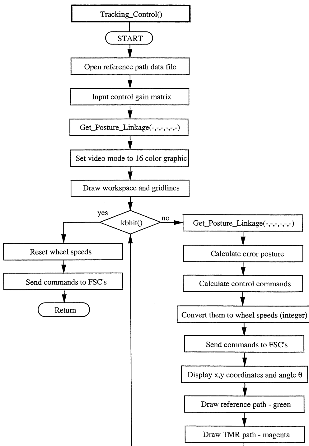
Figure 7-1b. Flow Chart of Control Program, Tracking Control
