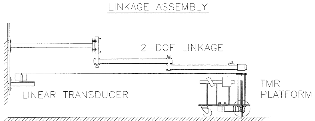
Figure 3-3. TMR Schematic
