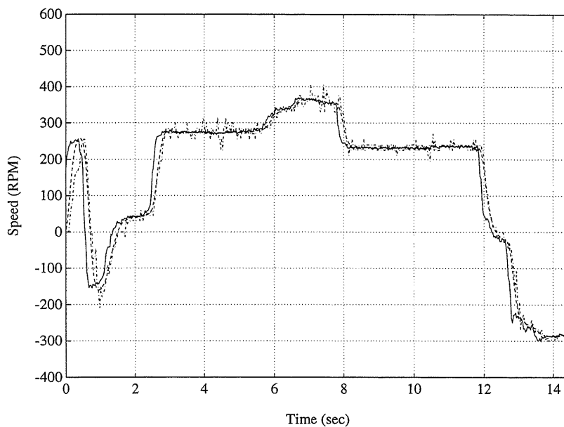
Figure 8-1. Joystick Control Example
