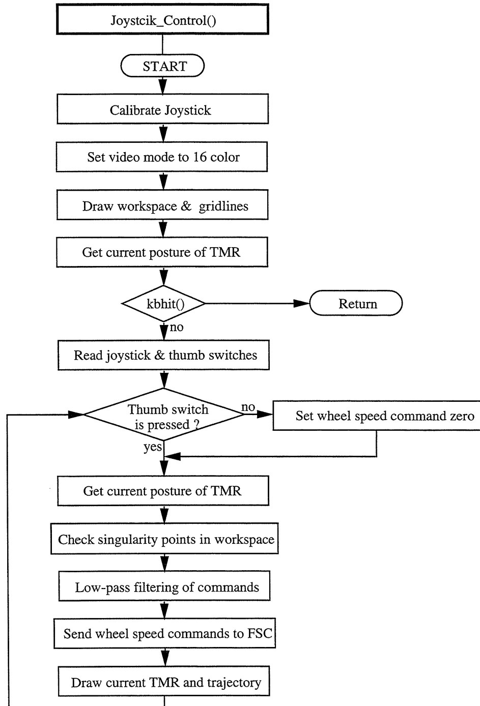
Figure 7-1d. Flow Chart of Control Program, Joystick Control
