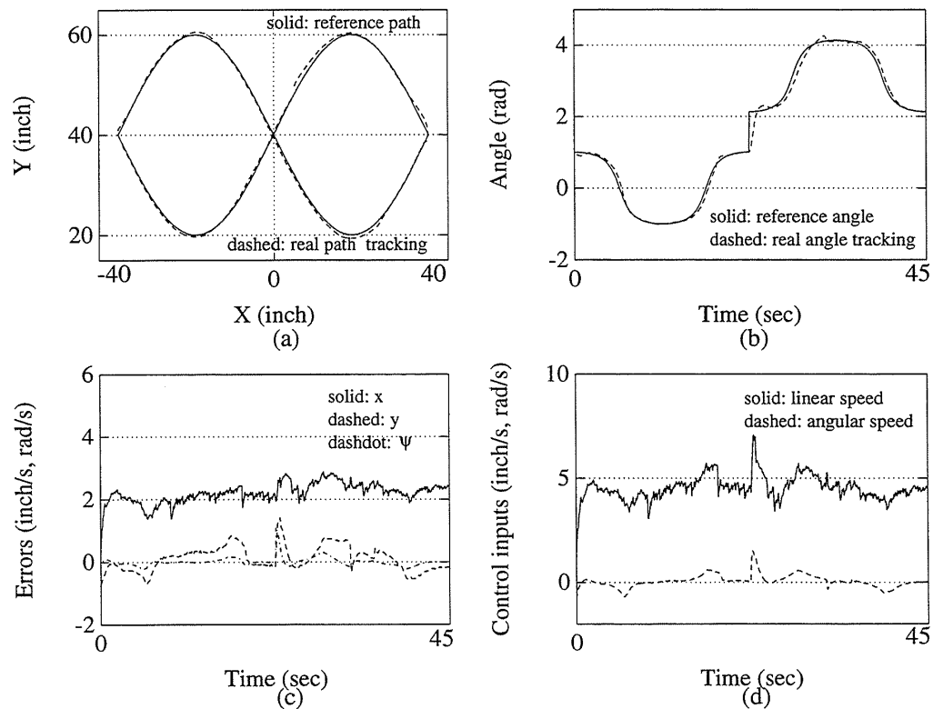
Figure 8-3. Trajectory Tracking Control Example
