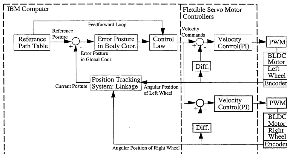
Figure 8-2. TMR Control System Software Structure
