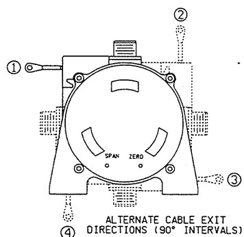
fig 2 Cable Exit
