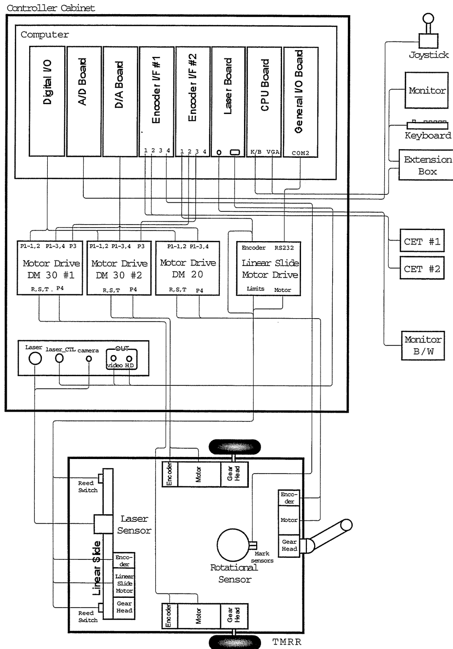
Figure 3-4. Overall wiring diagram of TMRR controller
