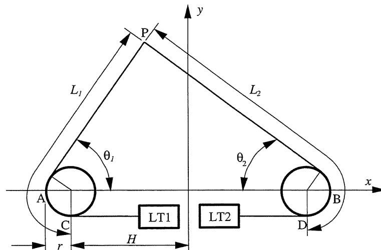
Figure 4-1. Schematic diagram of CET sensor system necessity, yet locate an arbitrary position P in the workspace. The size of the pulleys in the figure are exaggerated for illustrative purposes.
