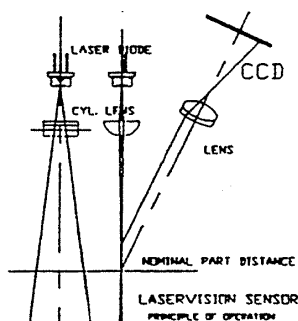
Figure 3.1.1 LaserVision Sensor Optics and Principle of Operation
