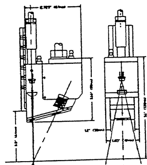
MVS-30 Outline and Optics
