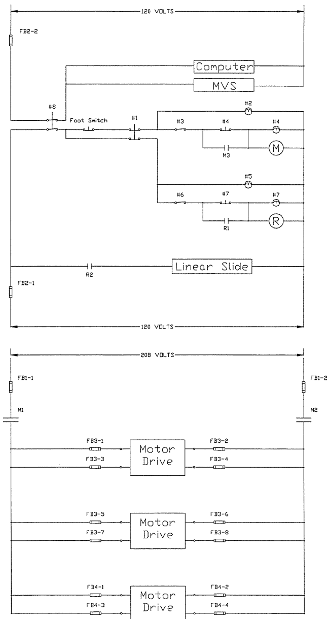
Figure 3-9. Power circuit of TMRR
