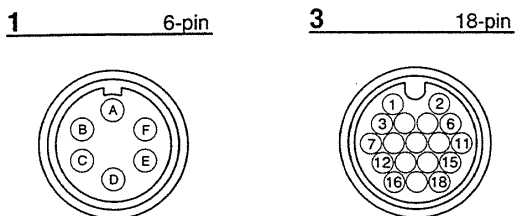
fig. 6 Mating Connectors
