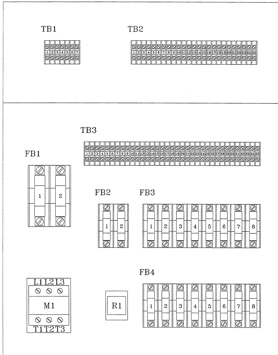
Figure 3-8. Power wiring components on cabinet back panel
