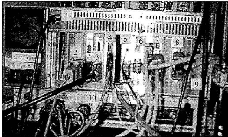
Figure 3-5. Back of computer, 1: keyboard connector, 2: COM1, 3: monitor cable, 4: encoder interface board #2, 5: laser processing board, 6: encoder interface board #1, 7: A/D converter board, 8: D/A converter board, 9: digital I/O board, 10: laser controller
