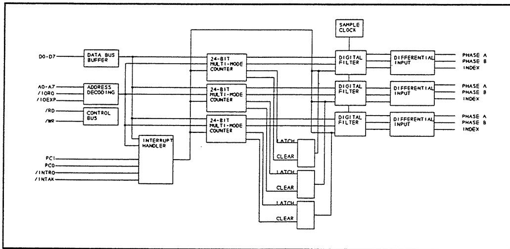
Figure 1.1 Functional block diagram for the 5312
