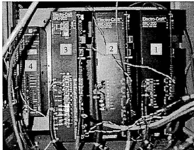
Figure 3-6. Motor drives, 1: DM30 #1, 2: DM30 #2, 3: DM20, 4: linear slide motor drive
