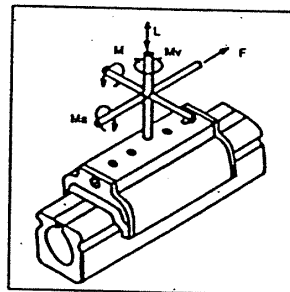
Load, Thrust, and Bending Moments Diagram
