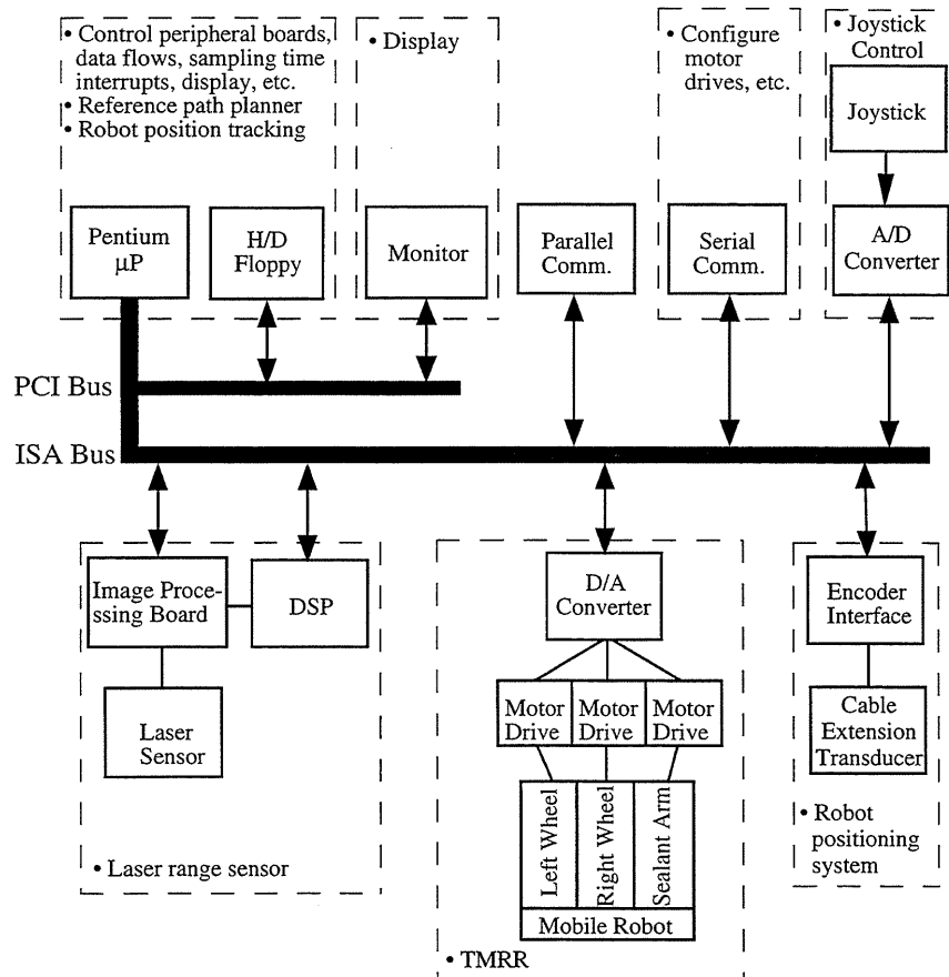
Figure 3-3. Block diagram of control hardware
