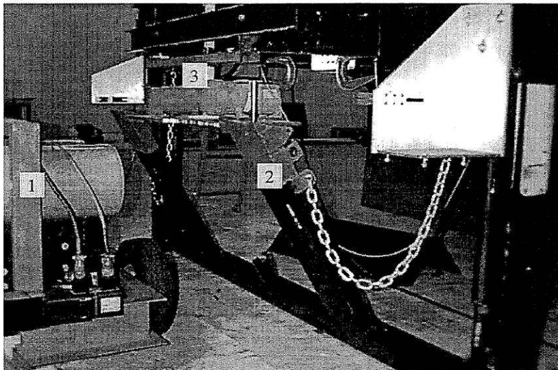
Figure 2-4. TMRR and lifter at the back of truck, 1: TMRR, 2: lifter, 3: CETs
