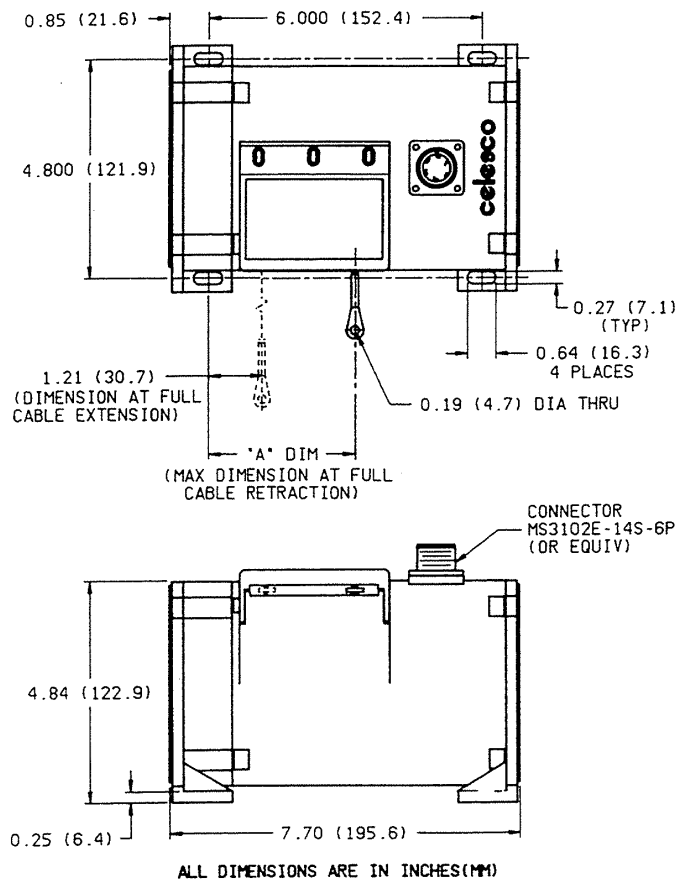
fig. 5 Outline Drawing
