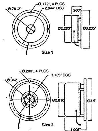
Electromechanical Fail-safe Brake (BR)
