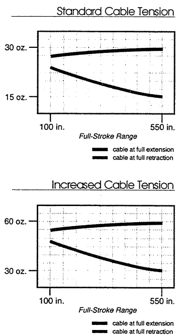
fig 3 Cable Tension
