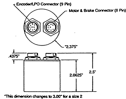
Motor, Brake and Encoder Canister Dimensions (CND)
