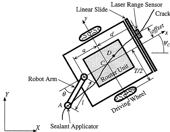
Figure 3-2. Schematic of WMR and Coordinate Systems
