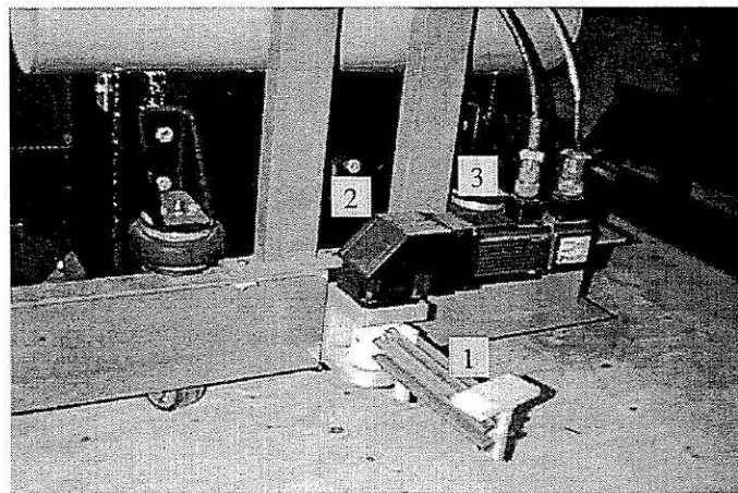
Figure 2-3. Rear arm assembly, 1: arm, 2: gear head, 3: BLDC motor
