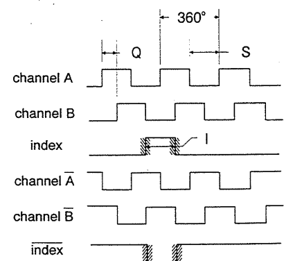
fig. 1 Output Waveforms
