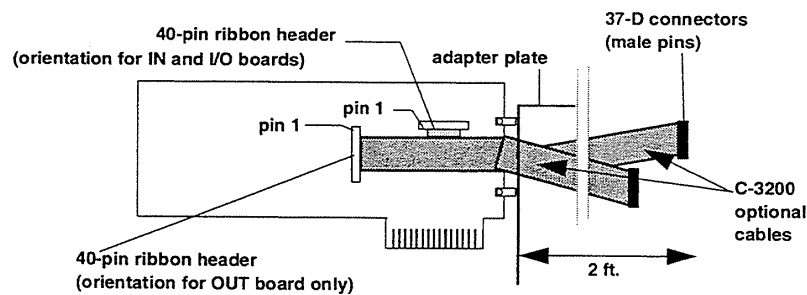
Figure 2-1. General Layout of PIO-32 Series Boards
