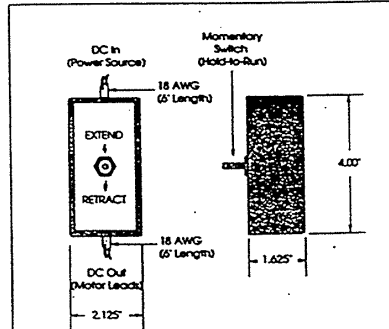
SP01 & *SP01R Switch Pack
