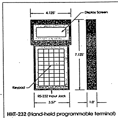
HHT-232 (Hand-held programmable terminal)
