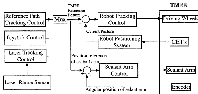
Figure 3-1. Block diagram of control software
