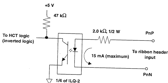
Figure 2-2. Typical Input Circuit
