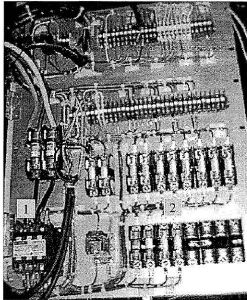
Figure 3-7. Power wiring on cabinet back panel, 1: magnetic contactor, 2: fuse blocks
