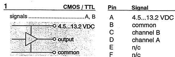
fig 4 Output Stage
