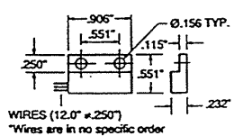
Magnetic Reed Switch (MS)
