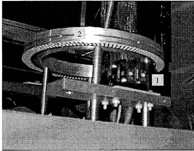
Figure 4-2. Rotational sensor assembly, 1: mark sensor, 2: mark
