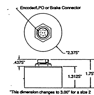
Motor, Brake or Encoder Canister Dimensions (CN)
