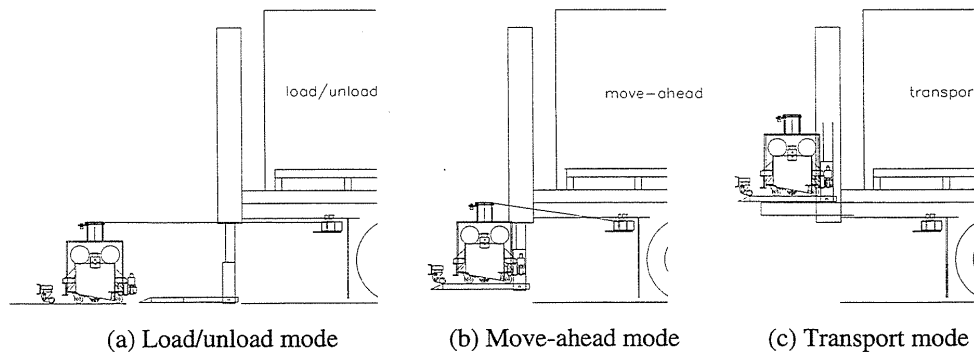
Figure 6-1. Illustration of TMRR liftgate operating modes
