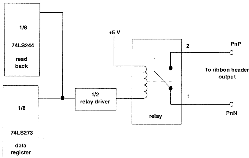
Figure 2-3. Typical Output Circuit
