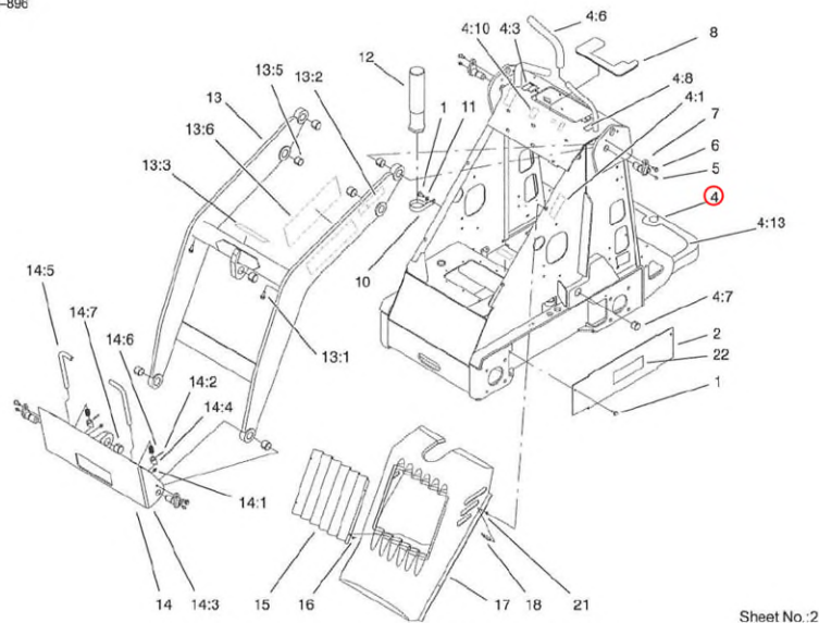
Frame And Loader Arm Assembly
