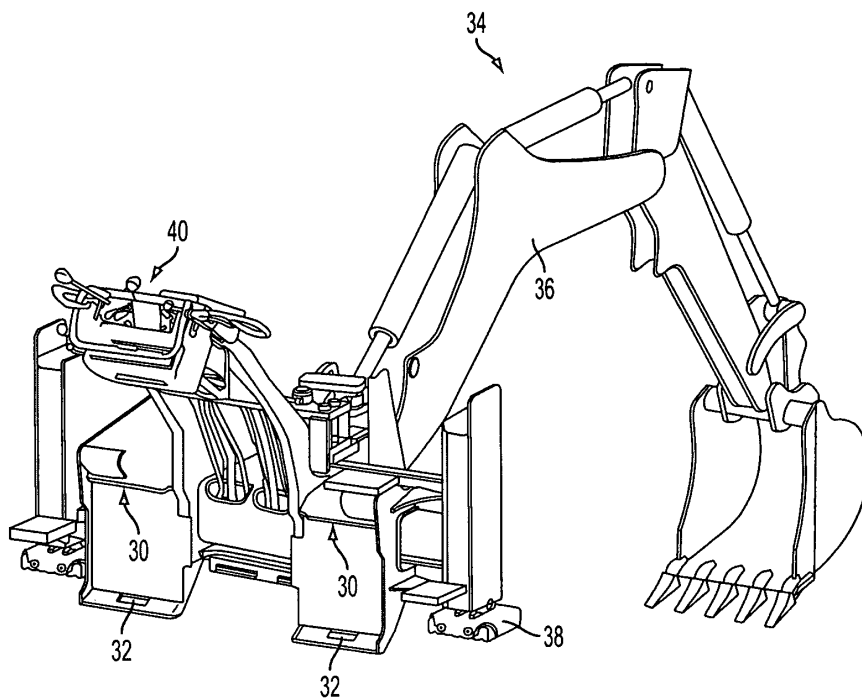
FIG. 3 PRIOR ART
