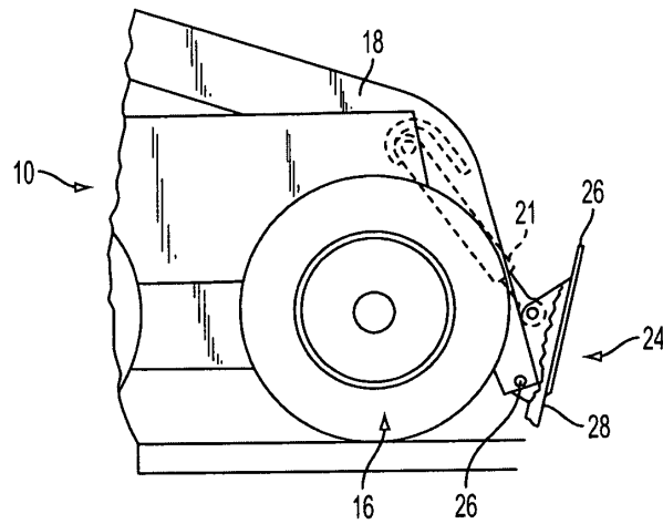
FIG. 2 PRIOR ART
