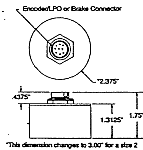
Motor, Brake or Encoder Canister Dimensions (CN)
