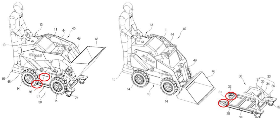
Ex. 1005 at Fig. 7, Fig. 8 (circles identifying position of rear bogie wheels added).
