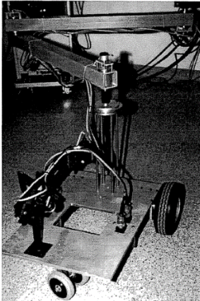
Figure 3-4. TMR Photograph
