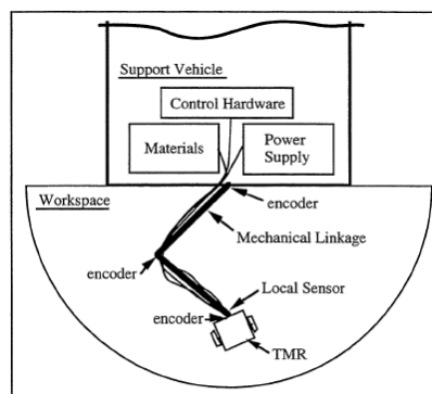
Figure 3-1. Conceptual TMR System Configuration
