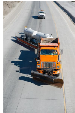
Figure 1. A TowPlow system in its deployed configuration
