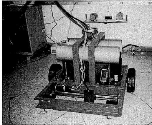
Figure 2-2. Front view of Tethered Mobile Routing Robot
