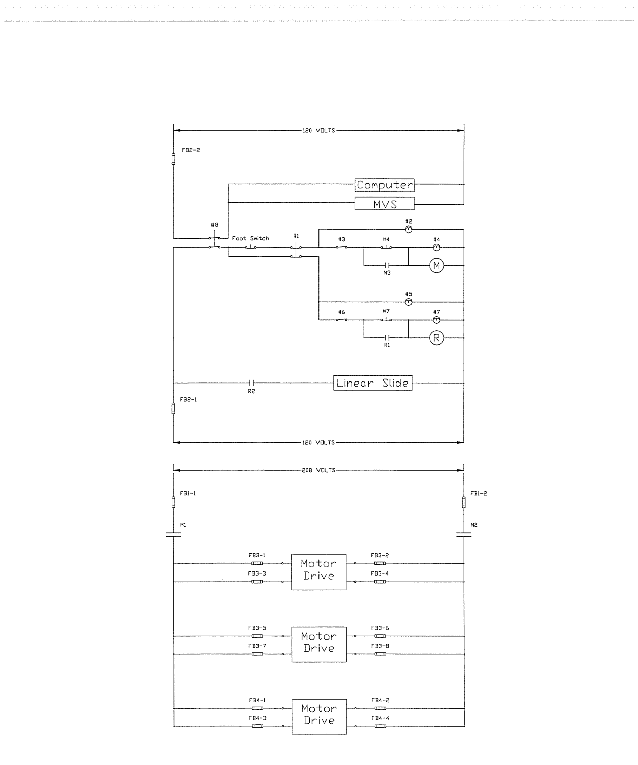
Figure 3-9. Power circuit of TMRR
