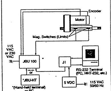
JBU Series
