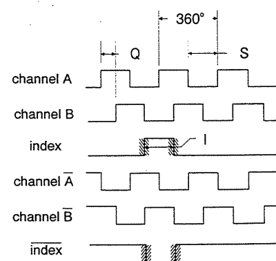
fig. 1 Output Waveforms
