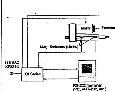
JDI Series
