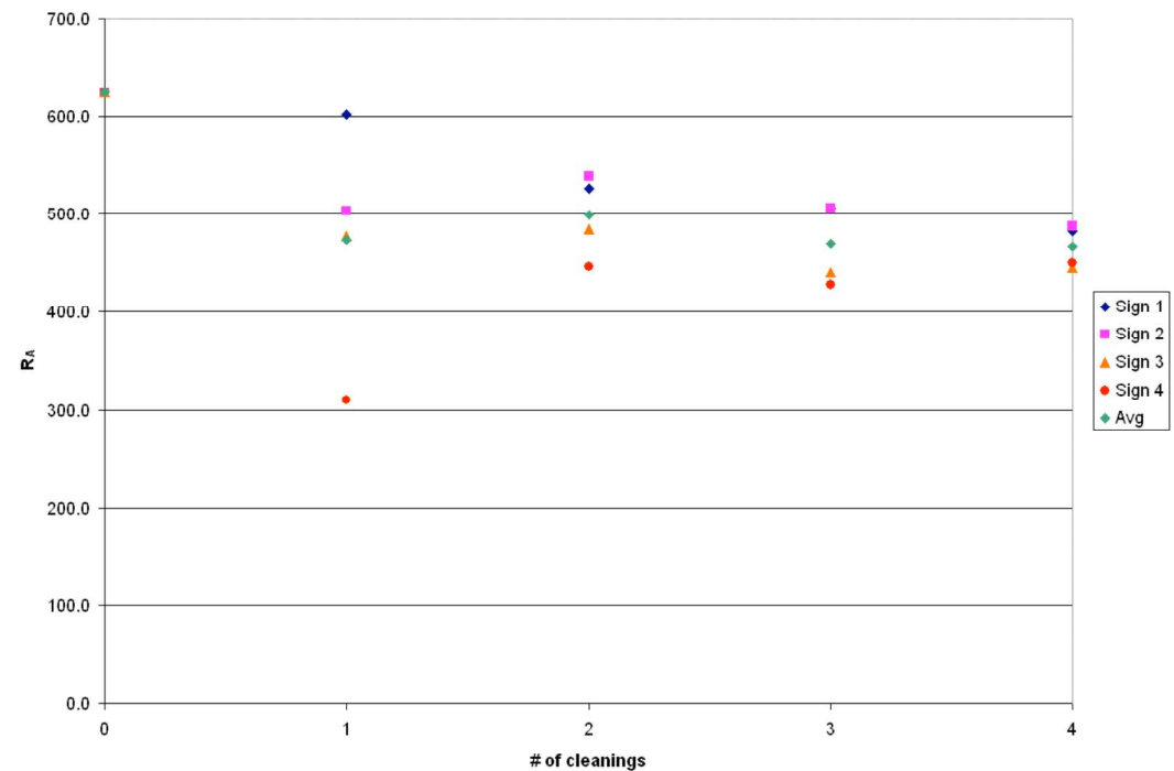
Figure 3-24: Multiple cleanings on painted signs with 1160
