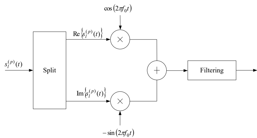
Figure 6.13-1: Downlink modulation
