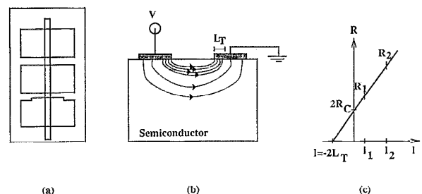
FIG. 1. (a) Sample configuration for I - V and TLM characterization. The thin vertical stripe is a 10 \mu m wide area of exposed GaN. The three wide rectangles are metal contacts separated by 20 and 15 \mu m. (b) Schematic of current flow through planar contacts. Nearly all of the current flows through one transfer length, L_T , of the contacts' front edges. (c) Plot of the measured resistance against the contact separation.
