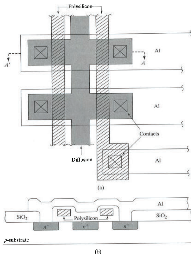
FIGURE 7.1 Portion of a MOS logic circuit showing the use of diffusion, polysilicon, and aluminum interconnections. (a) Top view; (b) cross section through A'-A.
