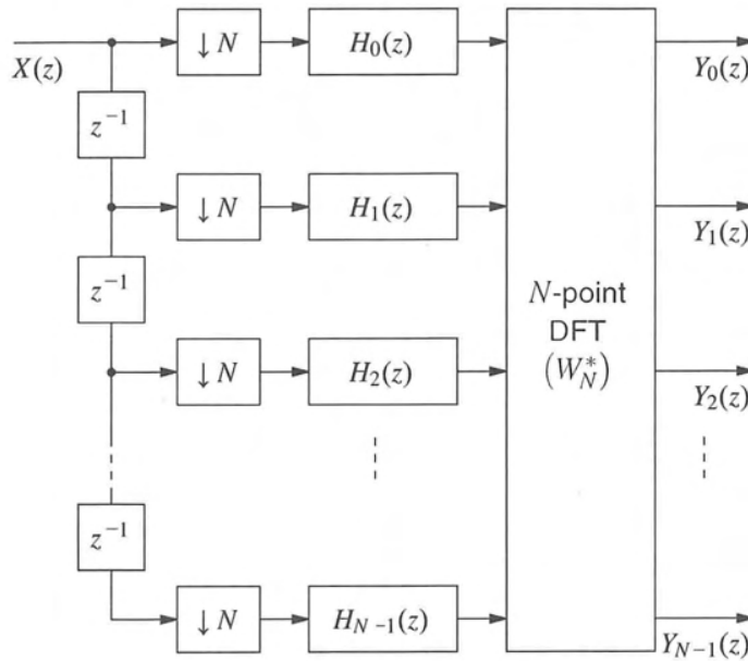
Figure 6.18 A maximally decimated uniform DFT filter bank ( H_k(z) are transfer functions of the polyphase components of H(z) )
