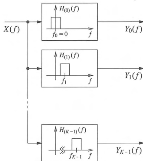
Figure 6.17 The basic principle of a filter bank ( H_k(f) are frequency characteristics of independent individual filters)
