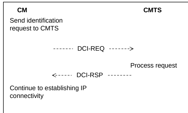
Figure 11-9 Device Class Identification
