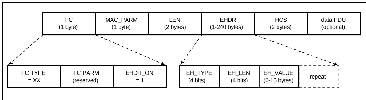
Figure 8-12 Extended MAC Format
