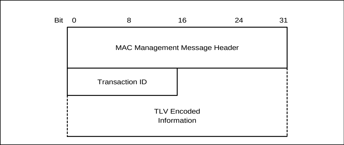
Figure 8-40 Dynamic Channel Change Acknowledge
