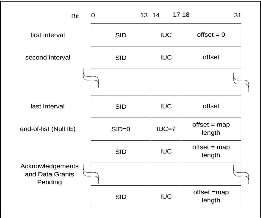
Figure 8-20 MAP Information Element Structure
