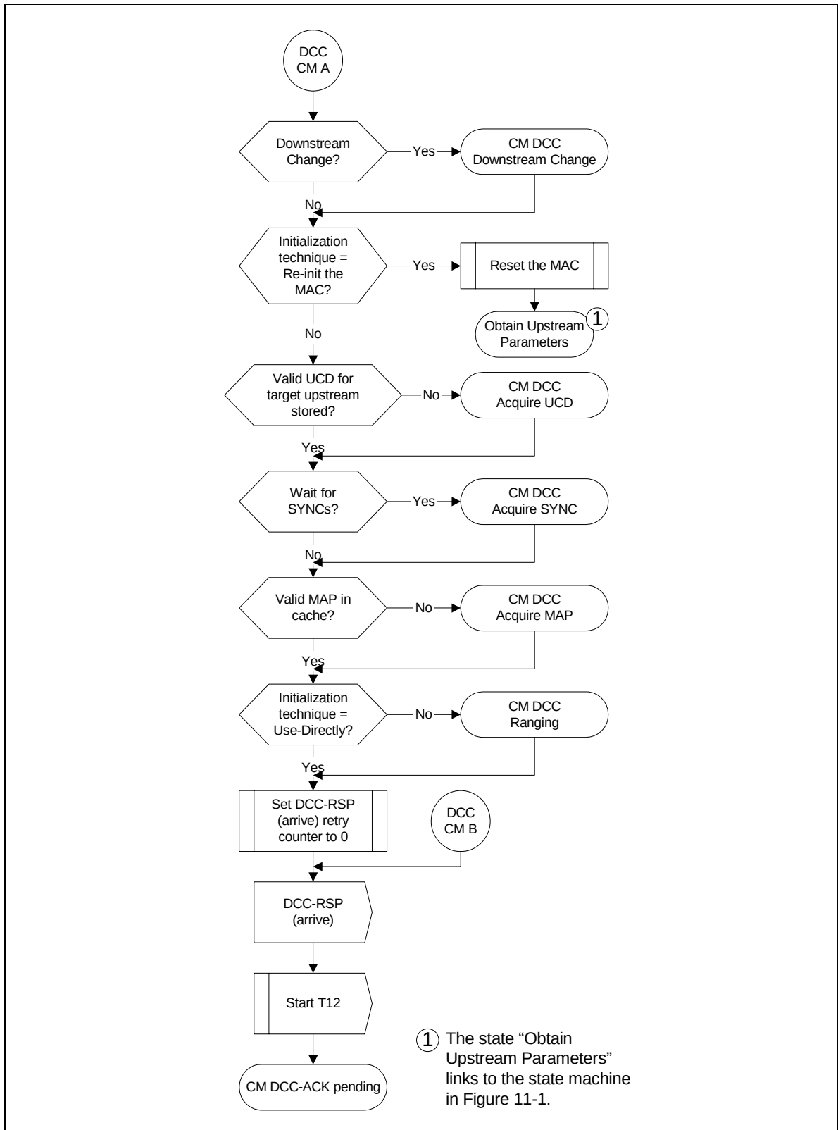
Figure 11-63 Dynamically Changing Channels: CM View Part 2
