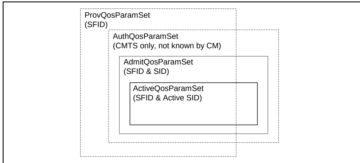
Figure 10-2 Dynamic Authorization Model “Envelopes”
