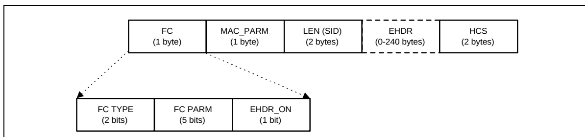
Figure 8-3 MAC Header Format
