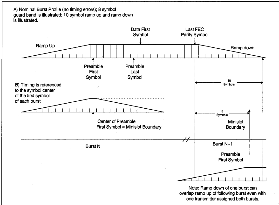
Figure 6-29 Nominal TDMA Burst Timing
