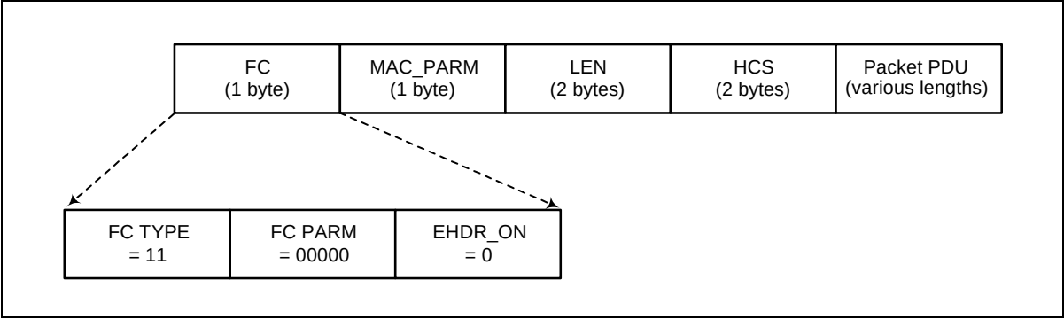
Figure 8-6 Timing MAC Header
