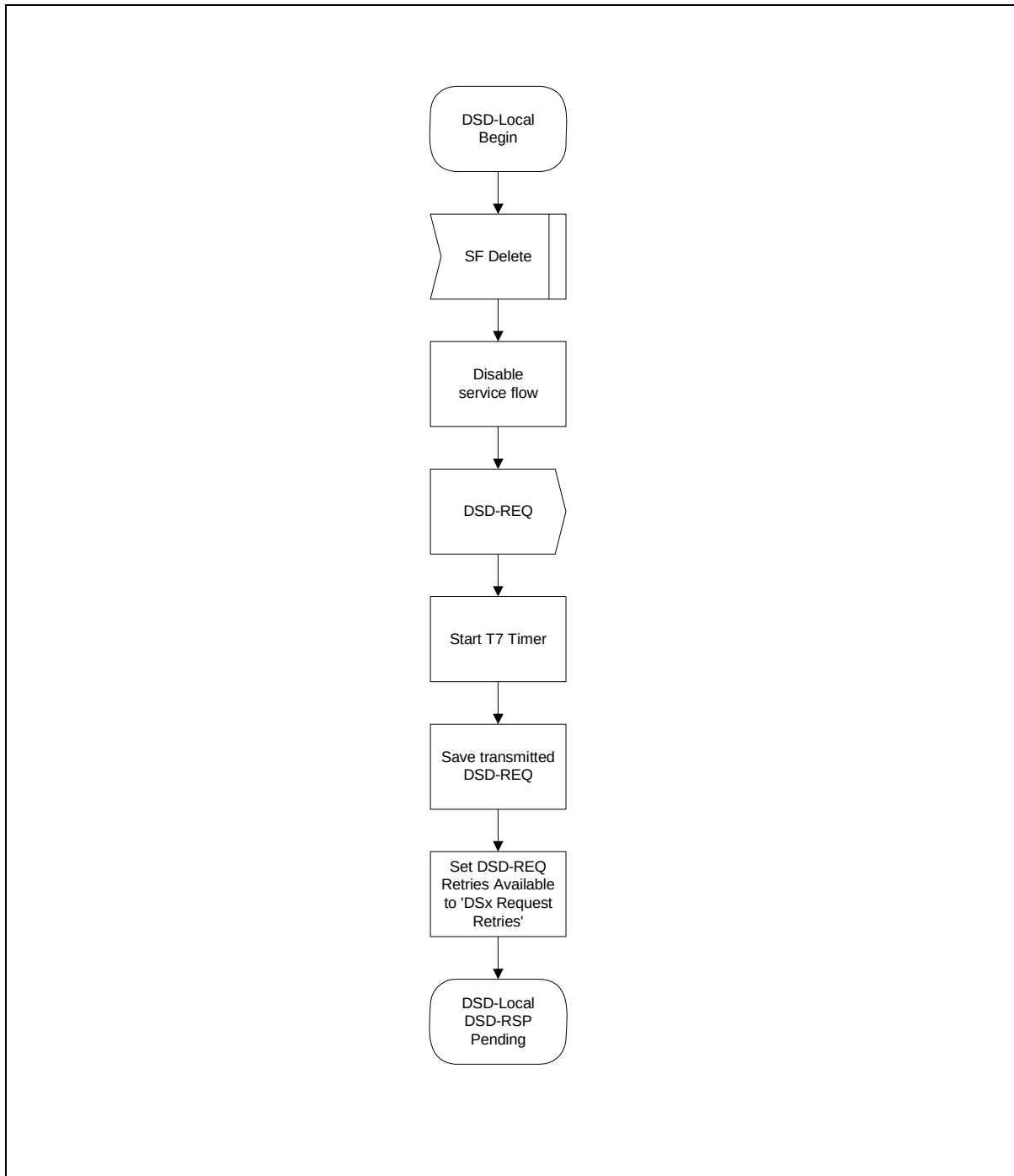
Figure 11-53 DSD—Locally Initiated Transaction Begin State Flow Diagram
