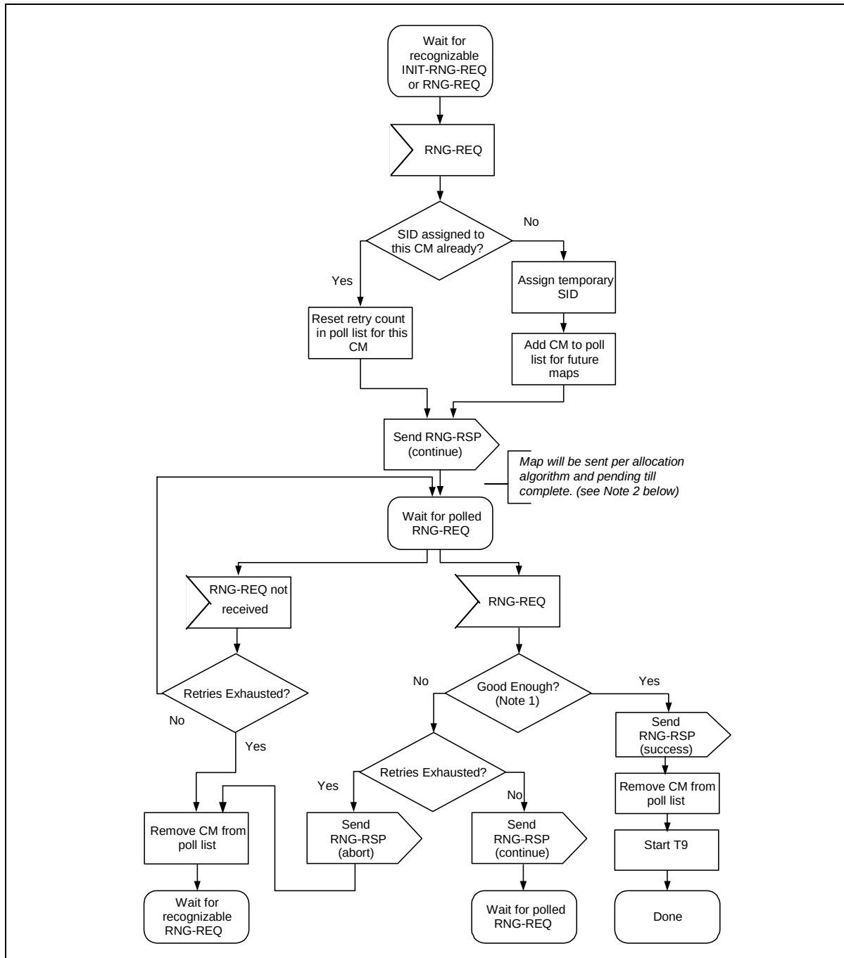
Figure 11-8 Initial Ranging - CMTS 1
