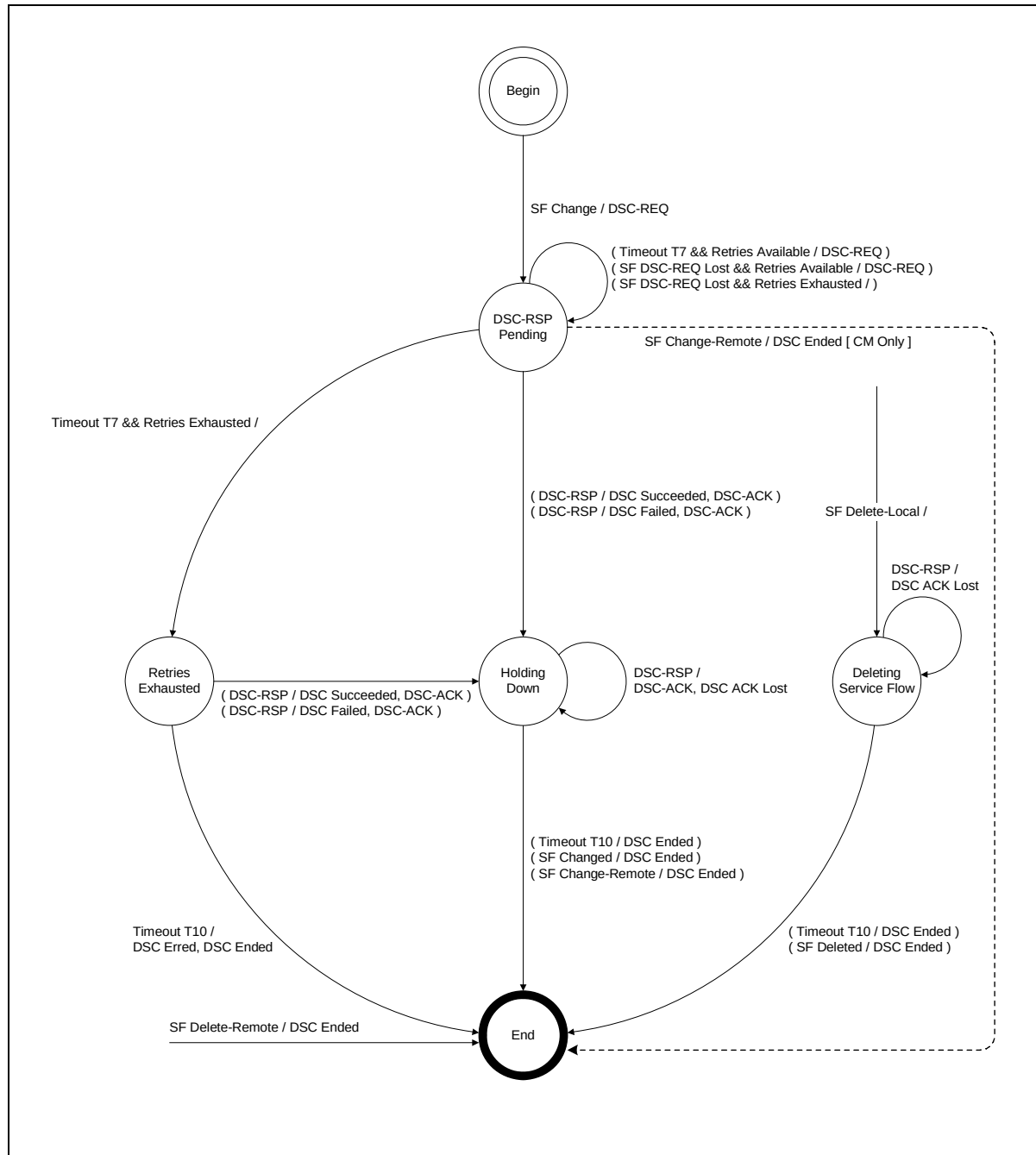
Figure 11-25 DSC—Locally Initiated Transaction State Transition Diagram
