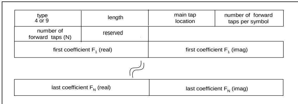
Figure 8-23 Generalized Decision Feedback Equalization Coefficients
