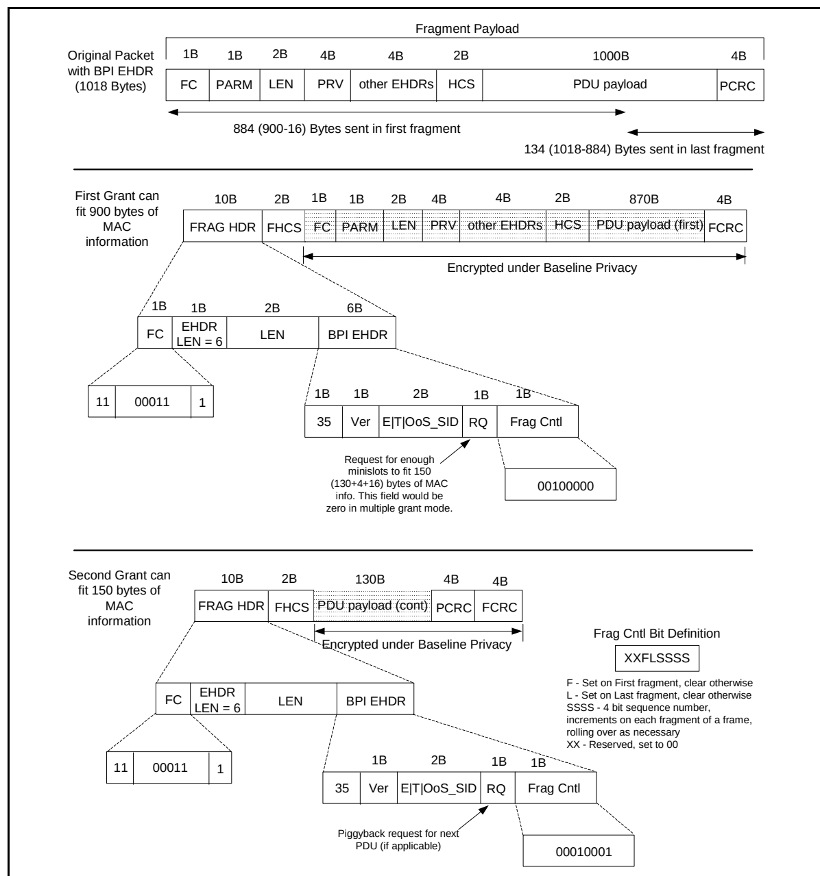
Figure 10-9 Example of Fragmenting a Single Packet
