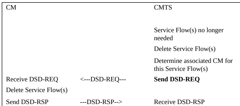
Figure 11-52 Dynamic Service Deletion Initiated from CMTS 2
