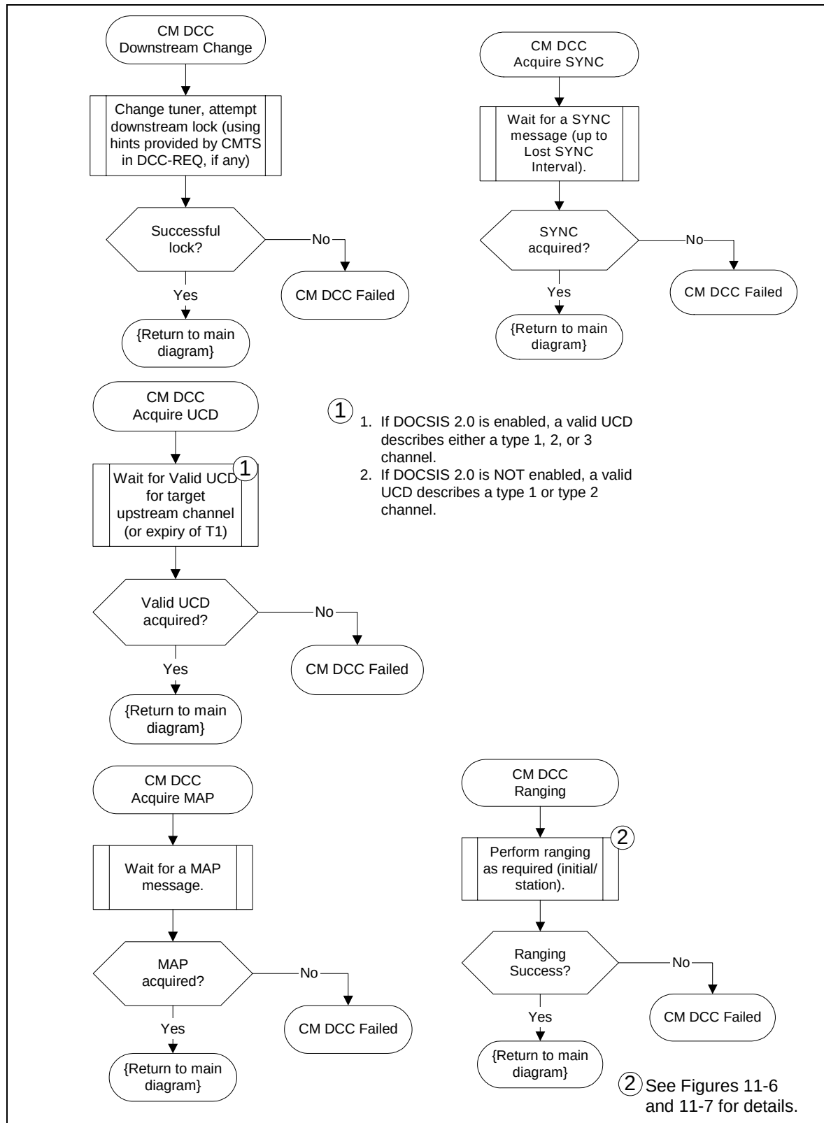
Figure 11-64 Dynamically Changing Channels: CM View Part 3
