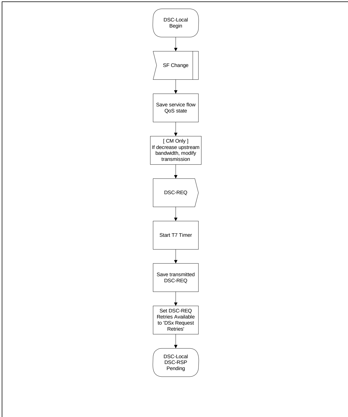
Figure 11-42 DSC—Locally Initiated Transaction Begin State Flow Diagram
