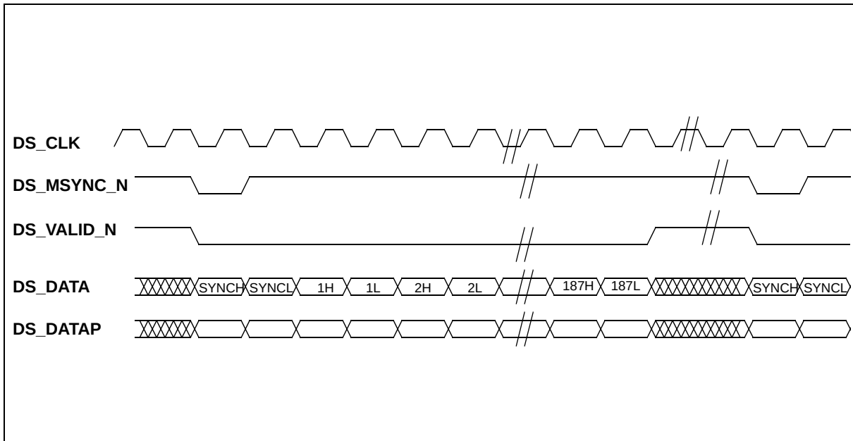
Figure H-2 Downstream Data Signal Protocol for ITU-T Recommendations J.83 Annex A Operation
