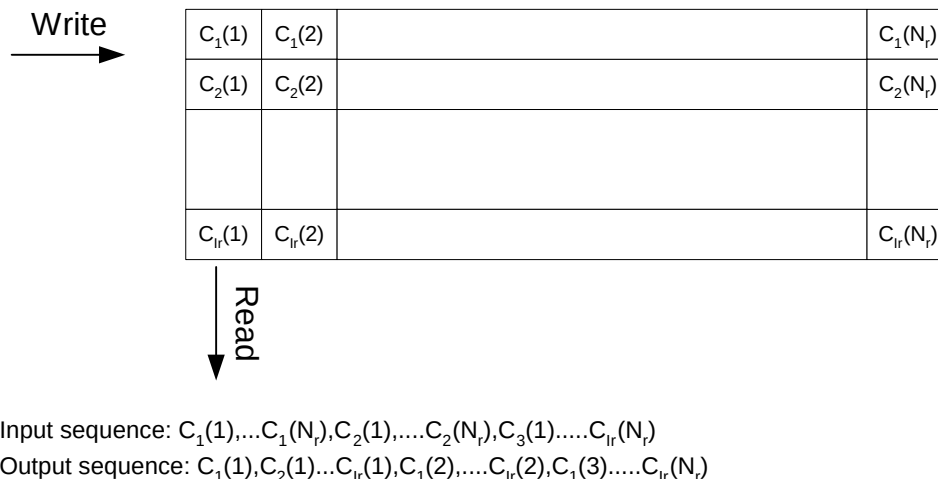
Figure 6-5 Byte Interleaver Operation
