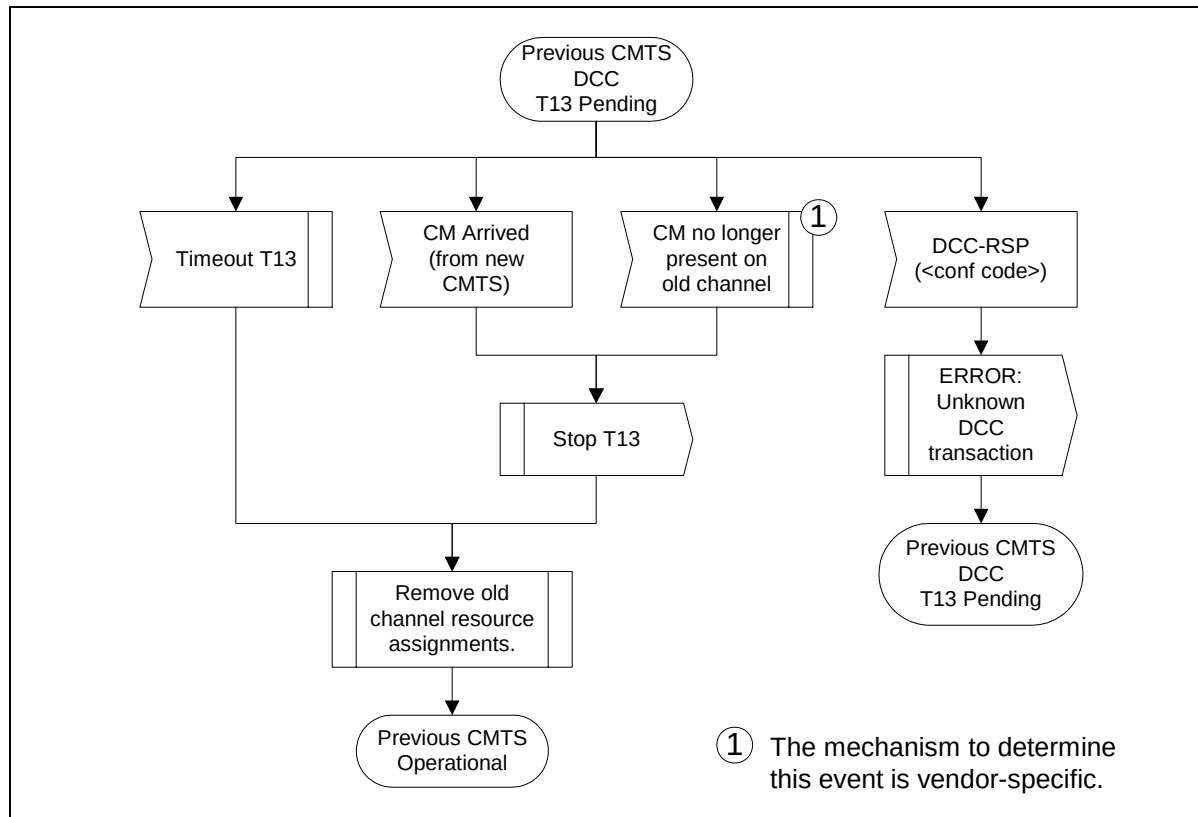
Figure 11-60 Dynamically Changing Channels: CMTS View Part 3
