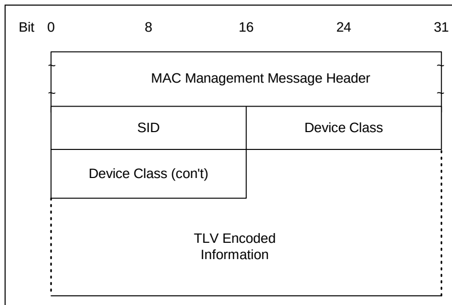
Figure 8-41 Device Class Identification Request
