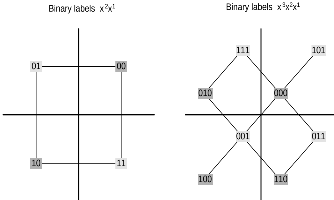
Figure 6-24 QPSK and 8QAM TCM Symbol Mapping
