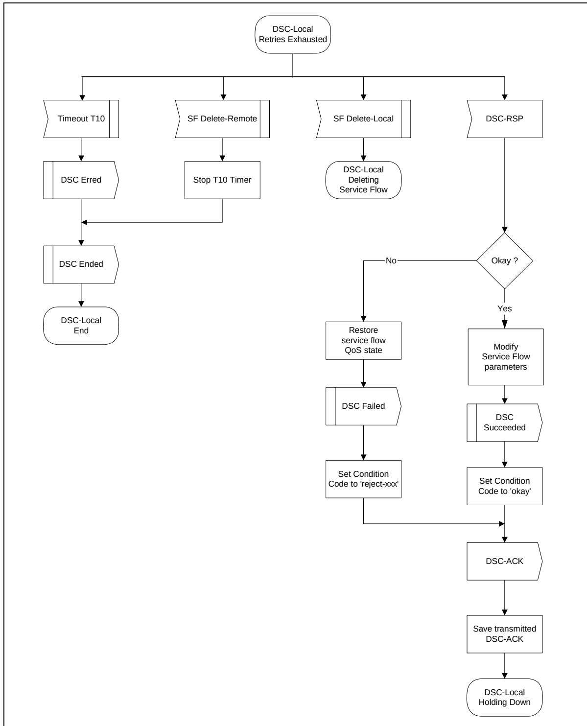
Figure 11-45 DSC—Locally Initiated Transaction Retries Exhausted State Flow Diagram
