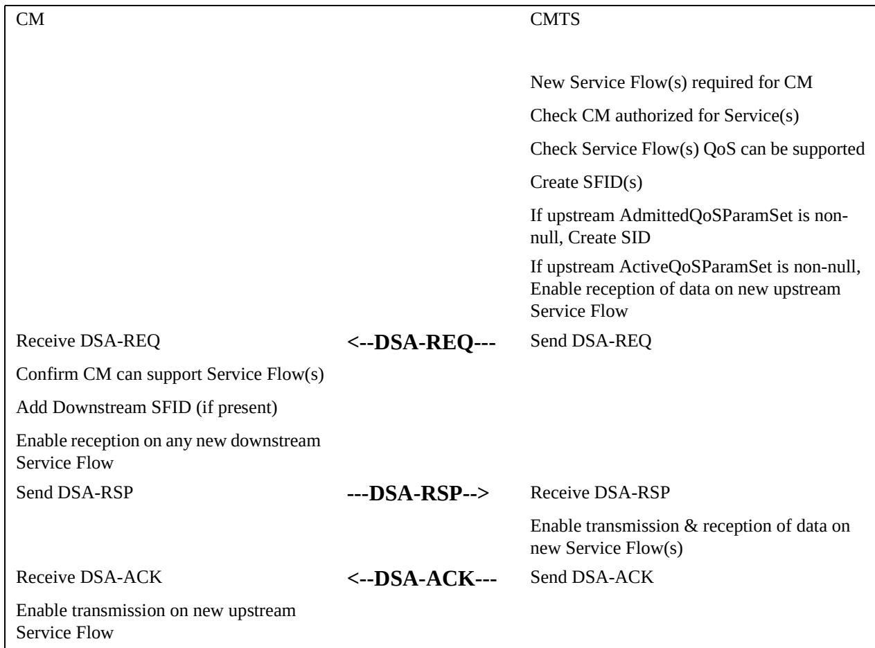
Figure 11-30 Dynamic Service Addition Initiated from CMTS
