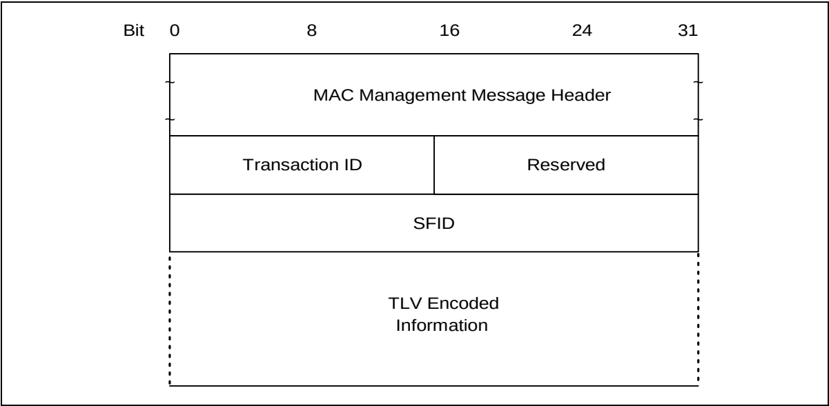
Figure 8-36 Dynamic Service Deletion — Request
