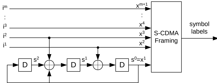
Figure 6-8 Convolutional encoder
