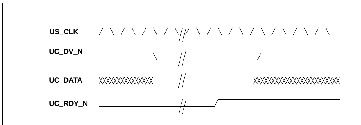
Figure H-6 Upstream Control Message Transfer
