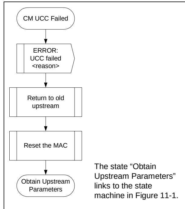
Figure 11-20 Changing Upstream Channels: CM View Part 2
