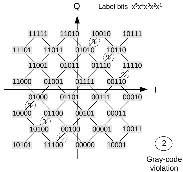
Figure 6-22 32QAM Symbol Mapping
