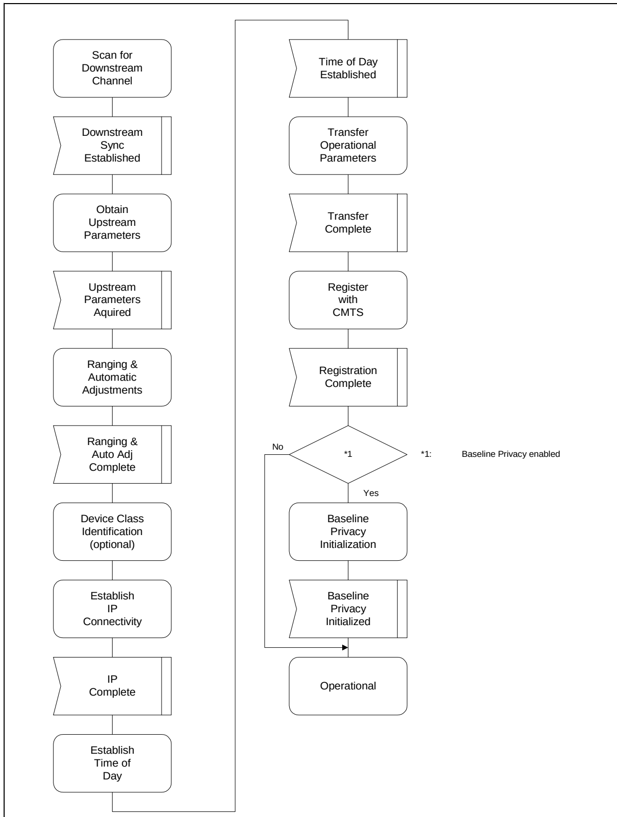
Figure 11-1 CM Initialization Overview
