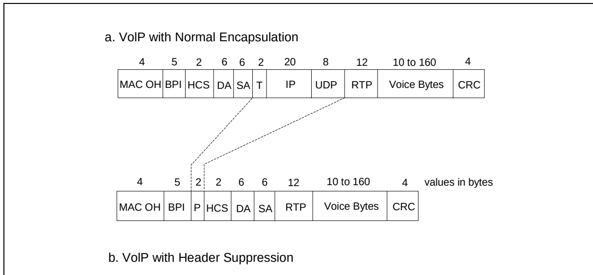
Figure 10-15 Downstream Payload Header Suppression Example
