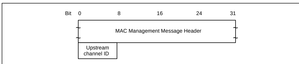
Figure 8-28 Upstream Channel Change Request 1
