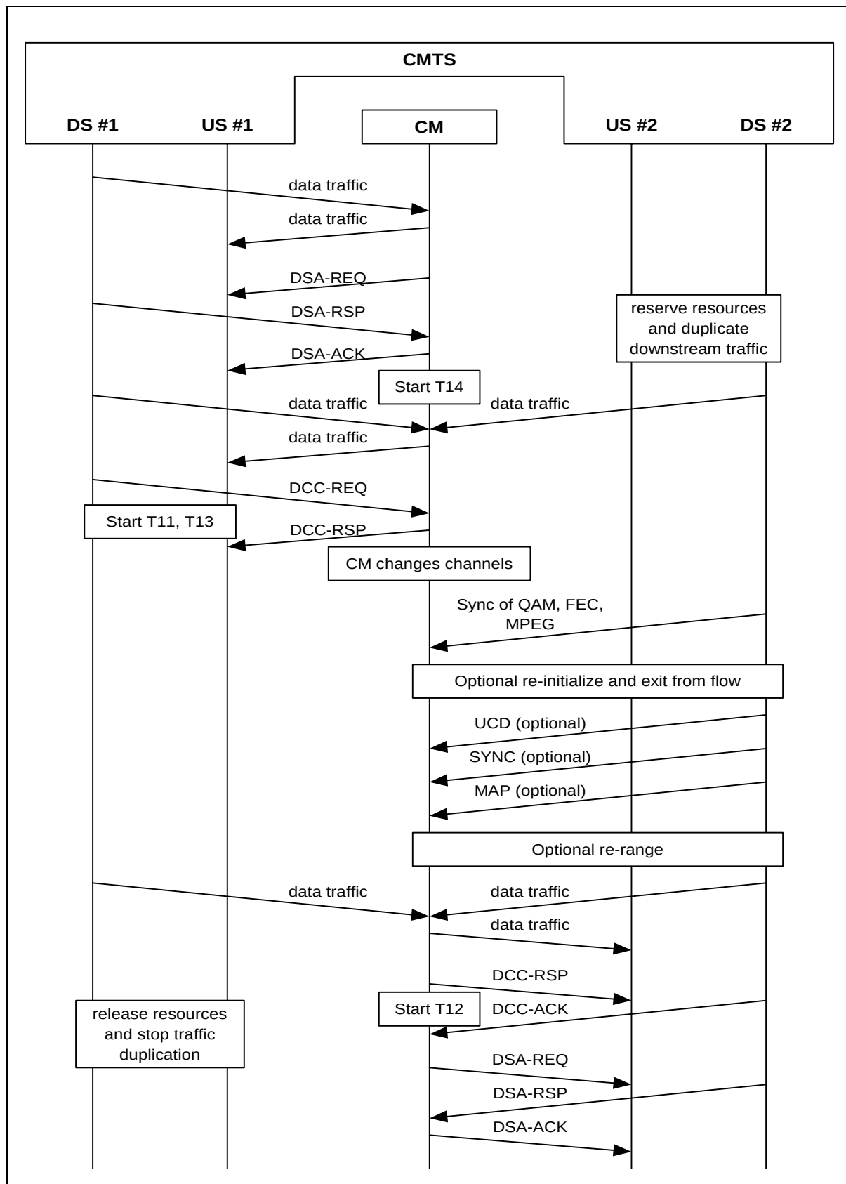
Figure 11-66 DCC Example Operational Flow
