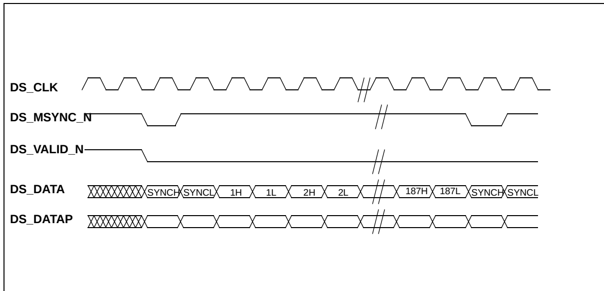
Figure H-3 Downstream Data Signal Protocol for ITU-T Recommendations J.83 Annex B Operation
