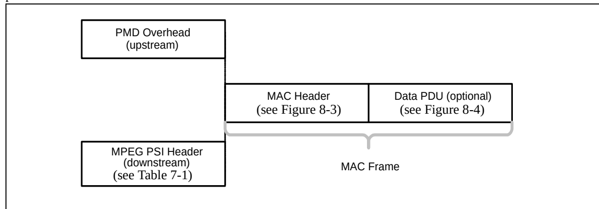
Figure 8-1 Generic MAC Frame Format
