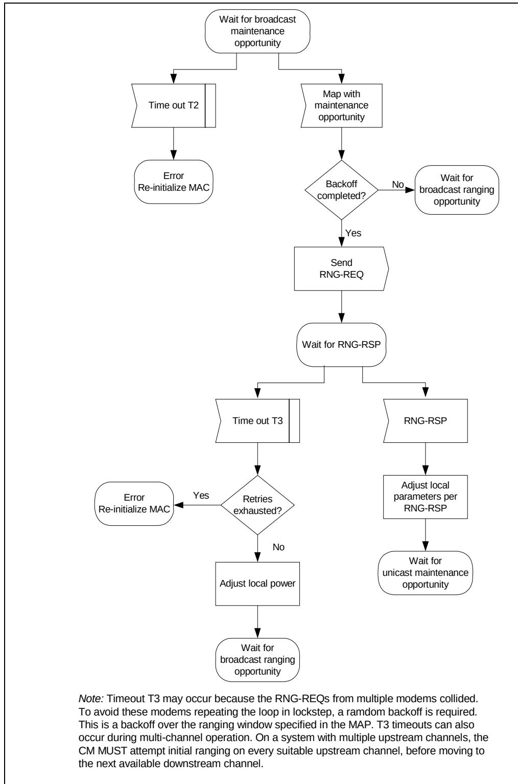
Figure 11-6 Initial Ranging - CM 1
