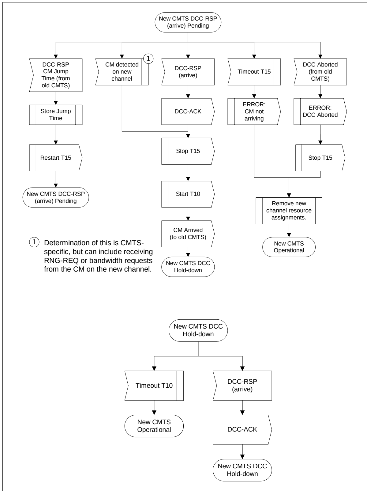
Figure 11-61 Dynamically Changing Channels: CMTS View Part 4
