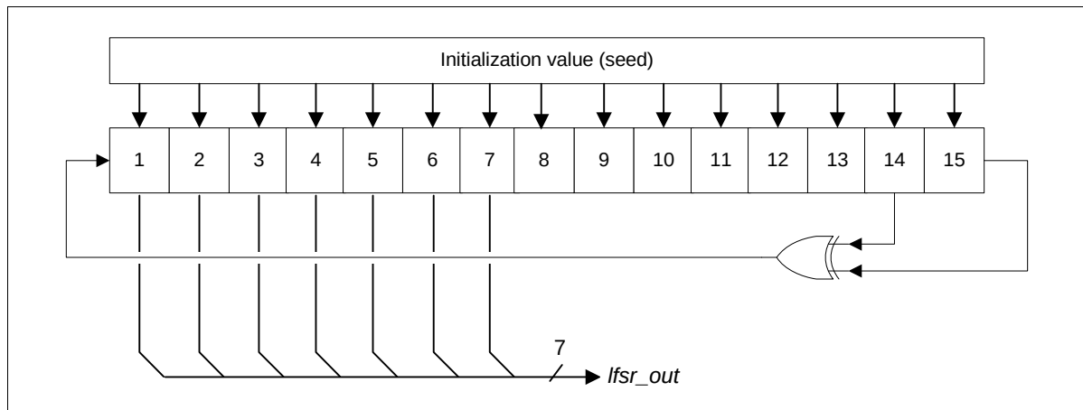
Figure 6-27 Code Hopping Random Number Generator
