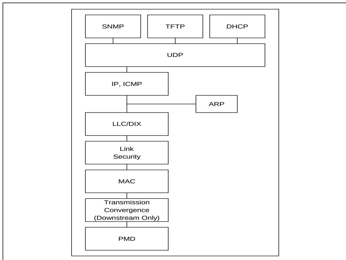
Figure 5-1 Protocol Stack on the RF Interface
