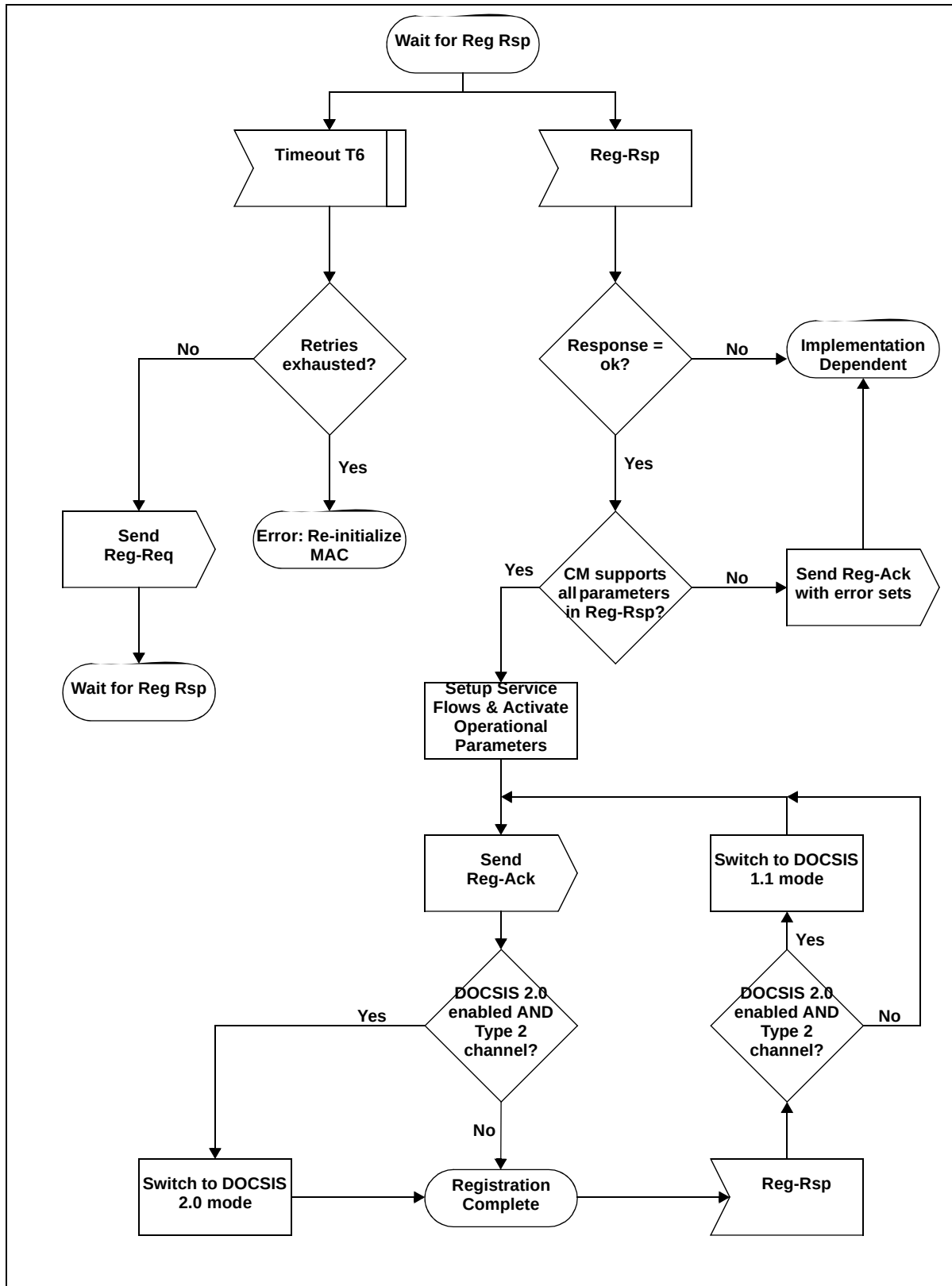
Figure 11-13 Wait for Registration Response — CM 1 2
