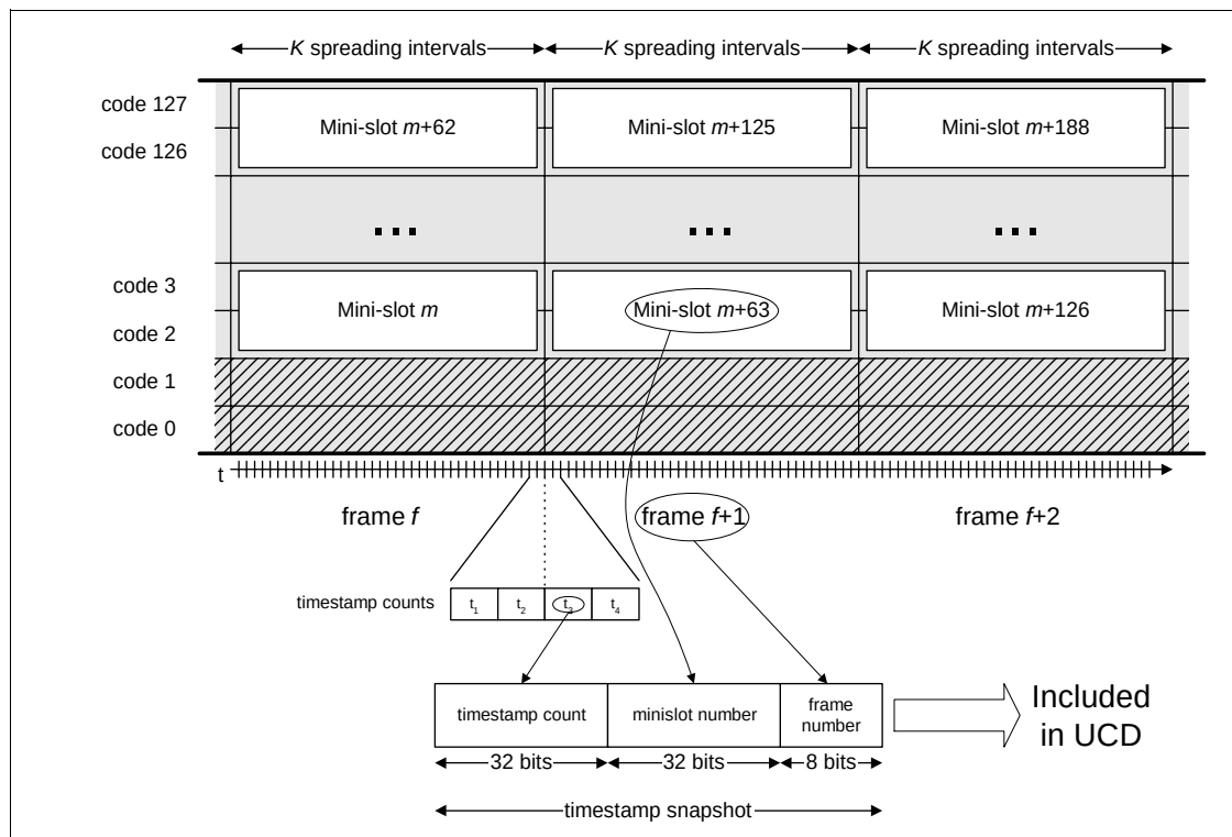
Figure 6-12 Timestamp Snapshot
