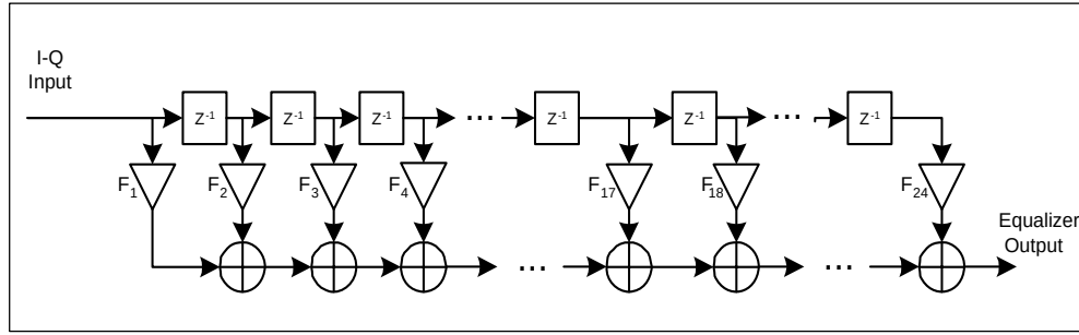
Figure 6-28 Transmit Pre-Equalizer Structure
