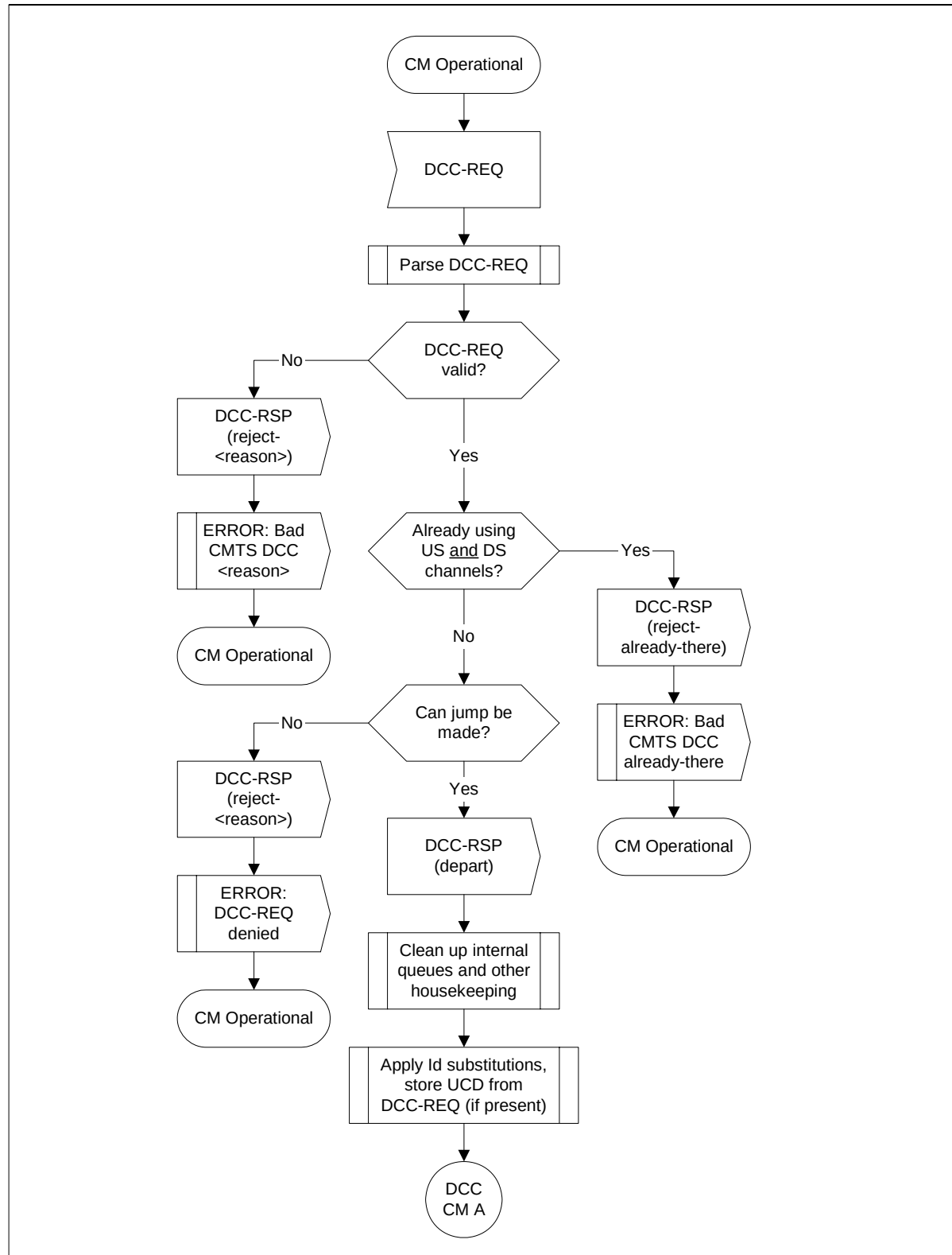
Figure 11-62 Dynamically Changing Channels: CM View Part 1
