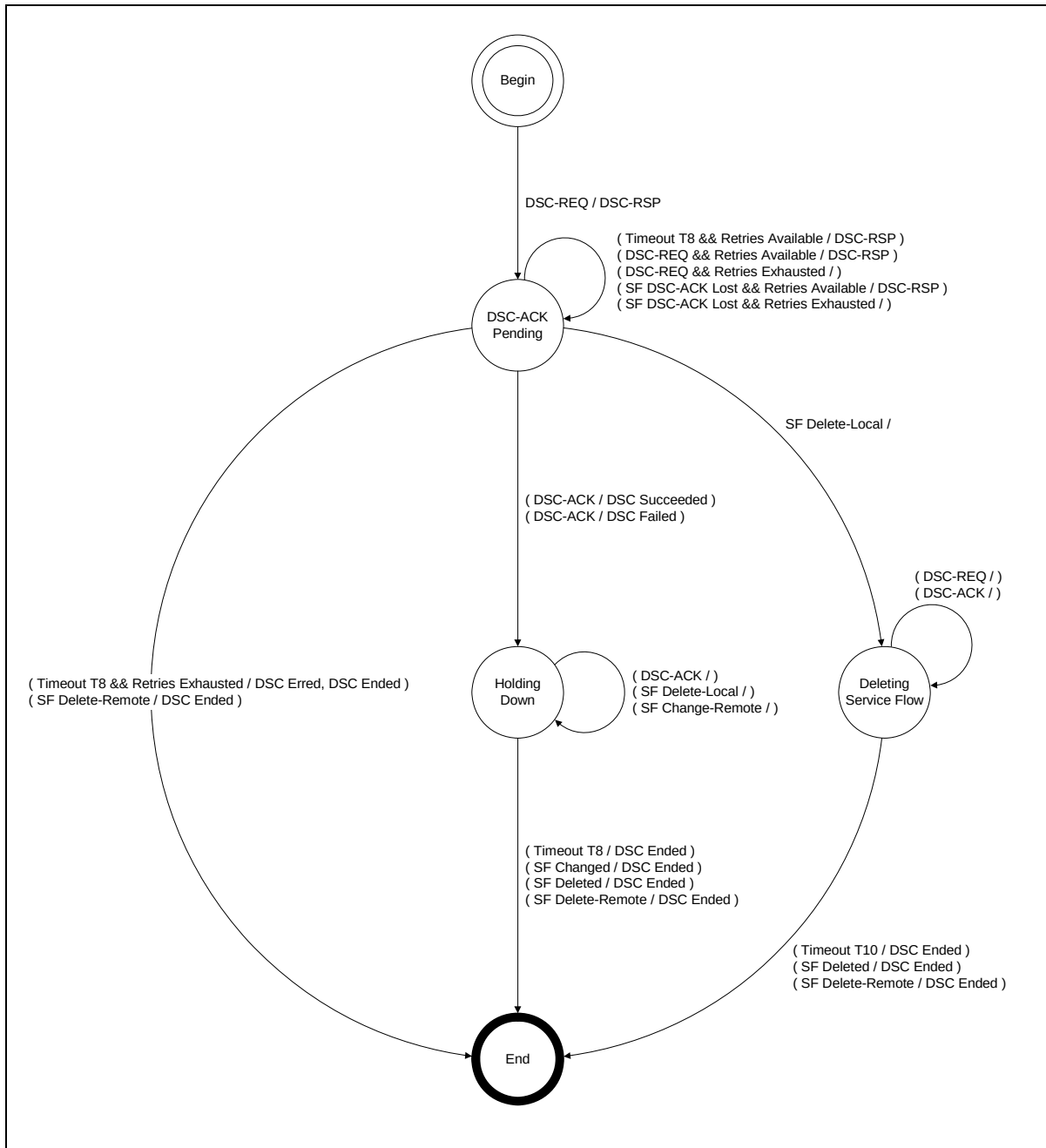
Figure 11-26 DSC—Remotely Initiated Transaction State Transition Diagram
