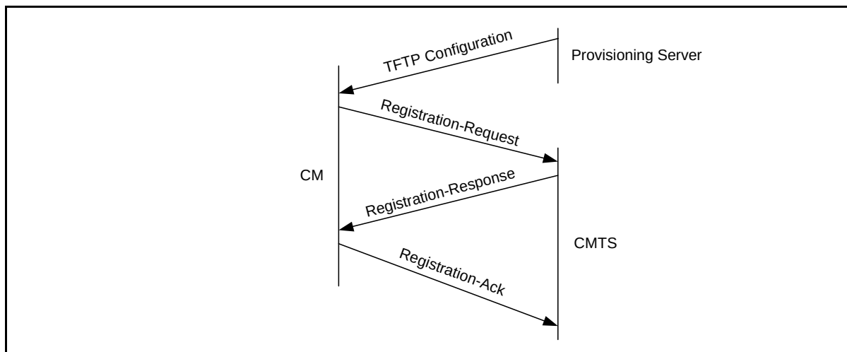
Figure 10-5 Registration Message Flow
