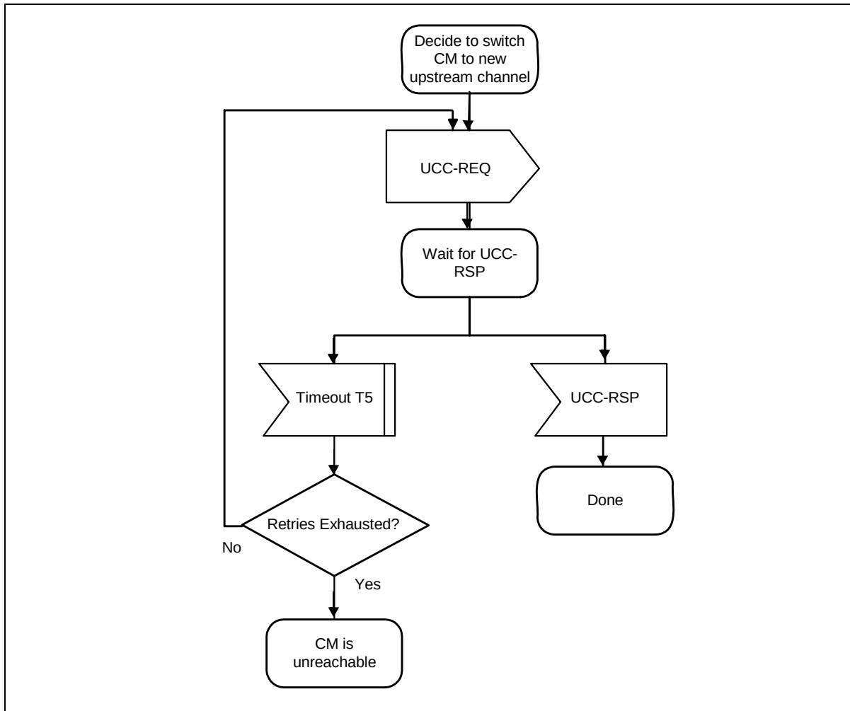
Figure 11-18 Changing Upstream Channels: CMTS View
