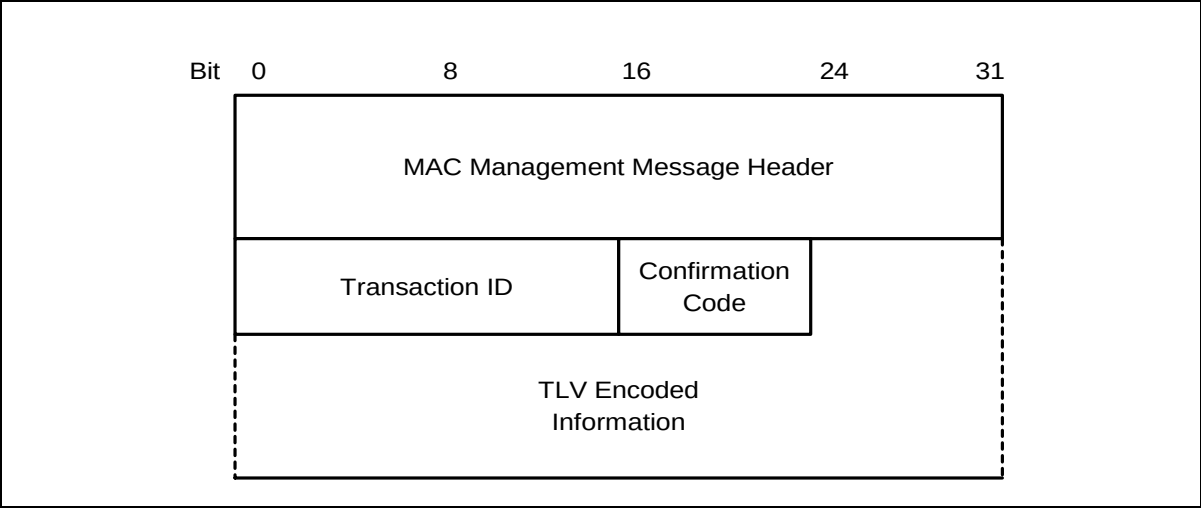
Figure 8-39 Dynamic Channel Change Response
