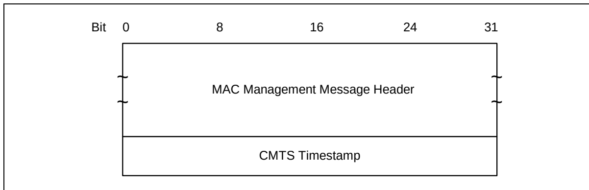
Figure 8-15 Format of Packet PDU Following the Timing Header
