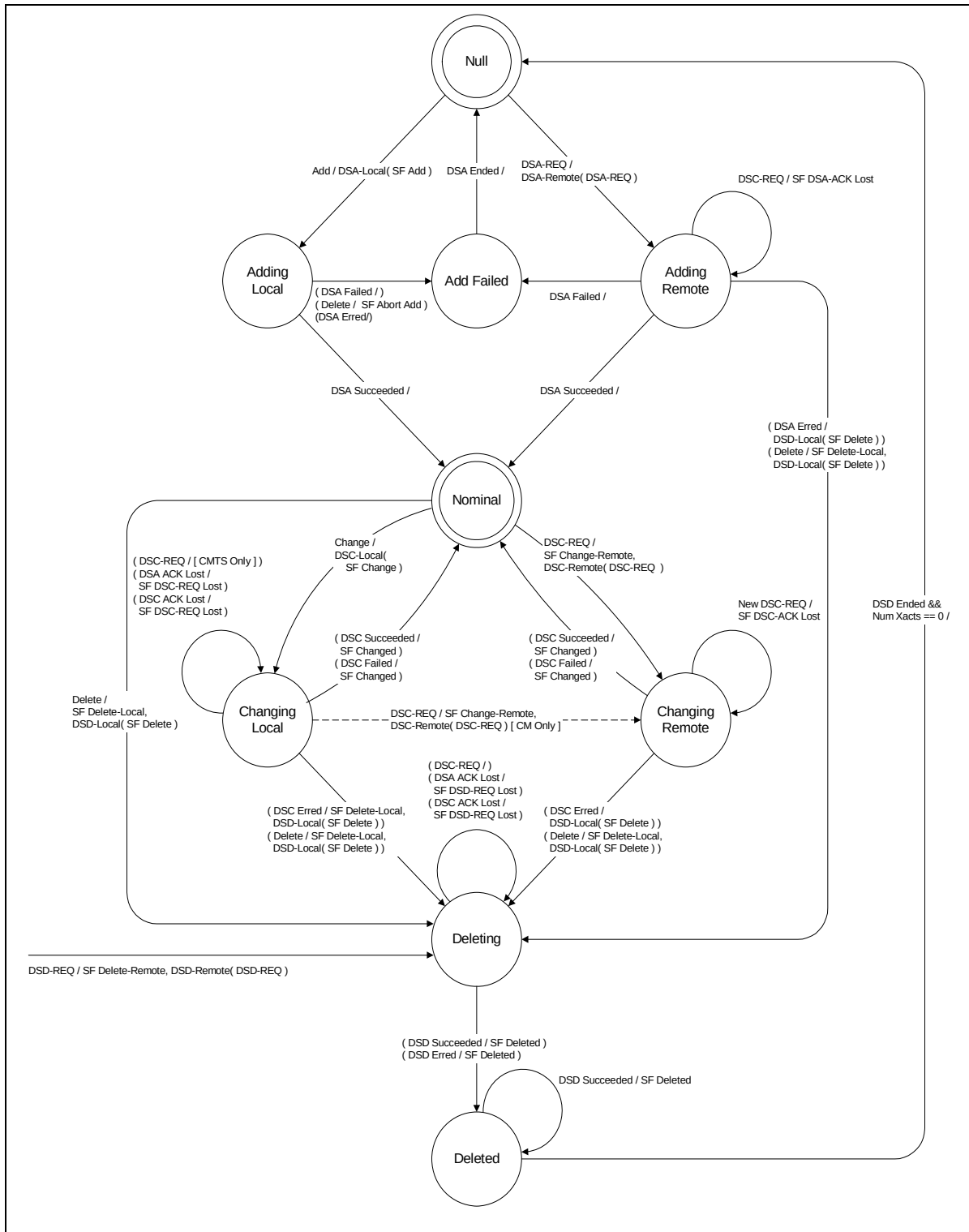
Figure 11-22 Dynamic Service Flow State Transition Diagram
