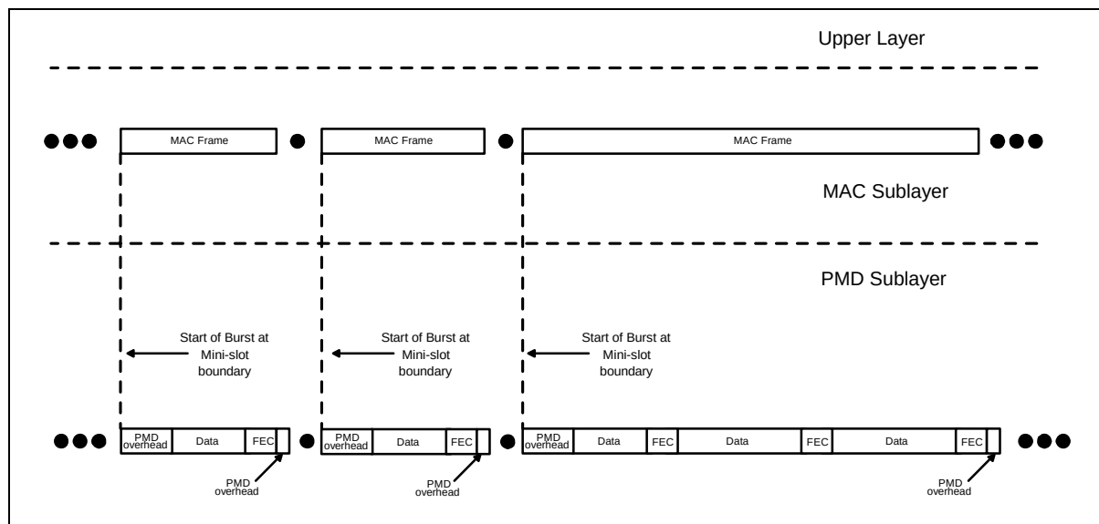
Figure 8-2 Upstream MAC/PMD Convergence
