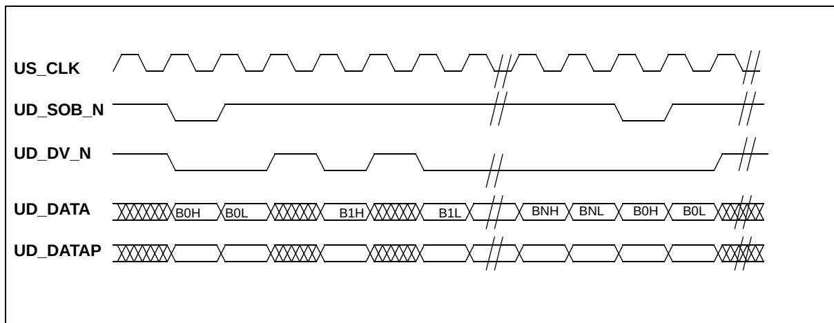
Figure H-4 Upstream Data Protocol
