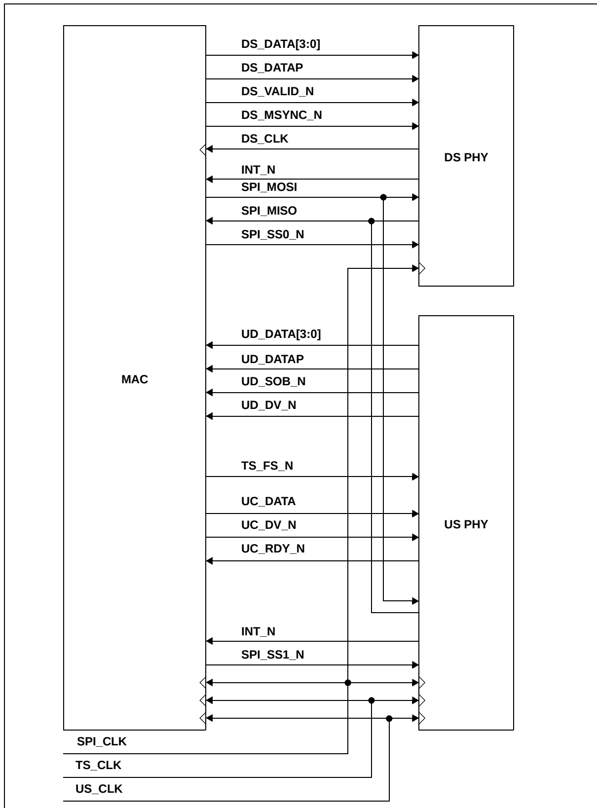
Figure H-1 DMPI Application
