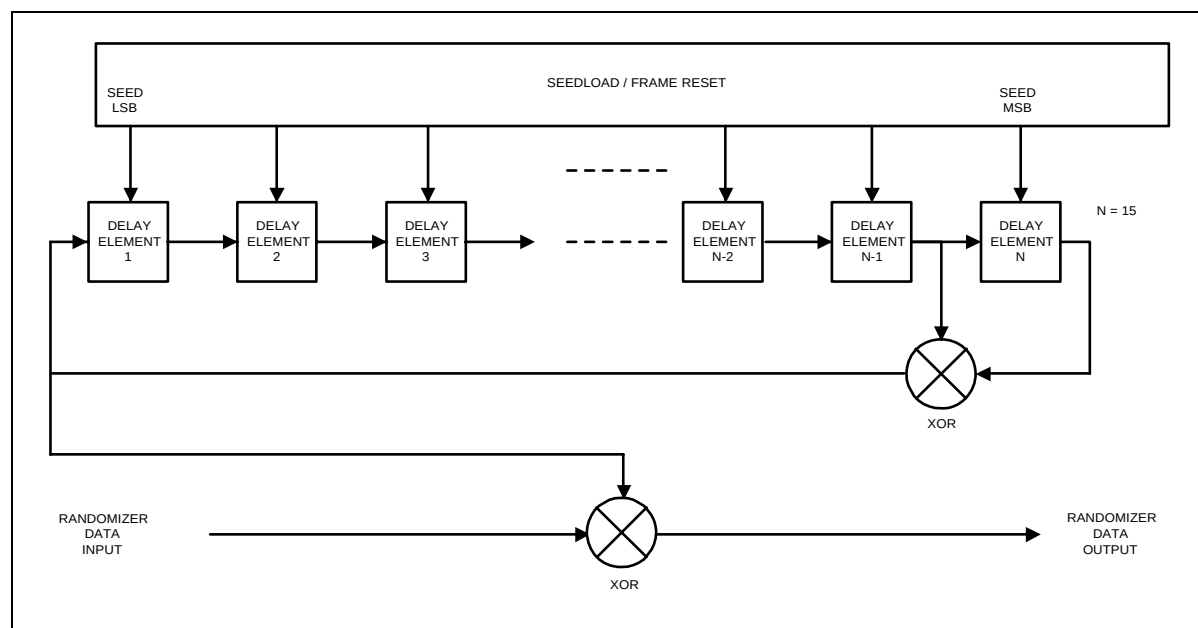
Figure 6-7 Scrambler Structure
