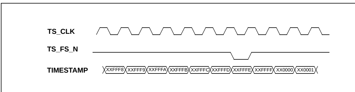
Figure H-5 Counter Synchronization
