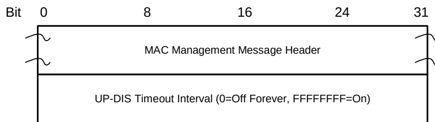
Figure 8-43 UP-DIS message format
