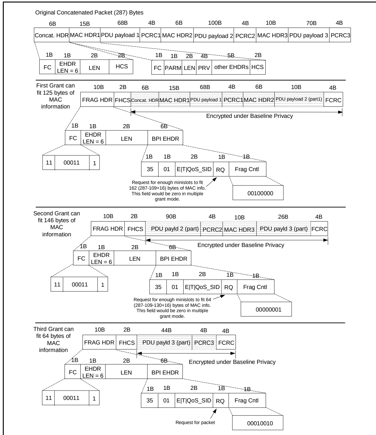
Figure 10-10 Fragmented Concatenated Packet Example
