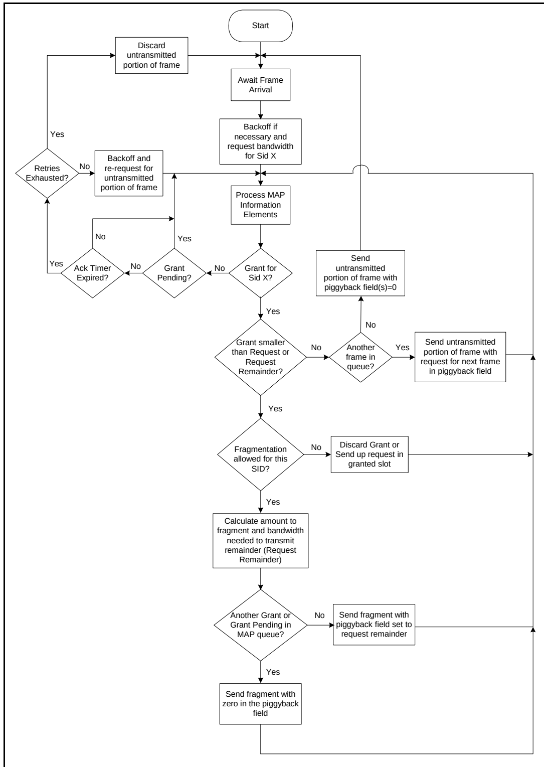
Figure 10-8 CM Fragmentation Flowchart 1
