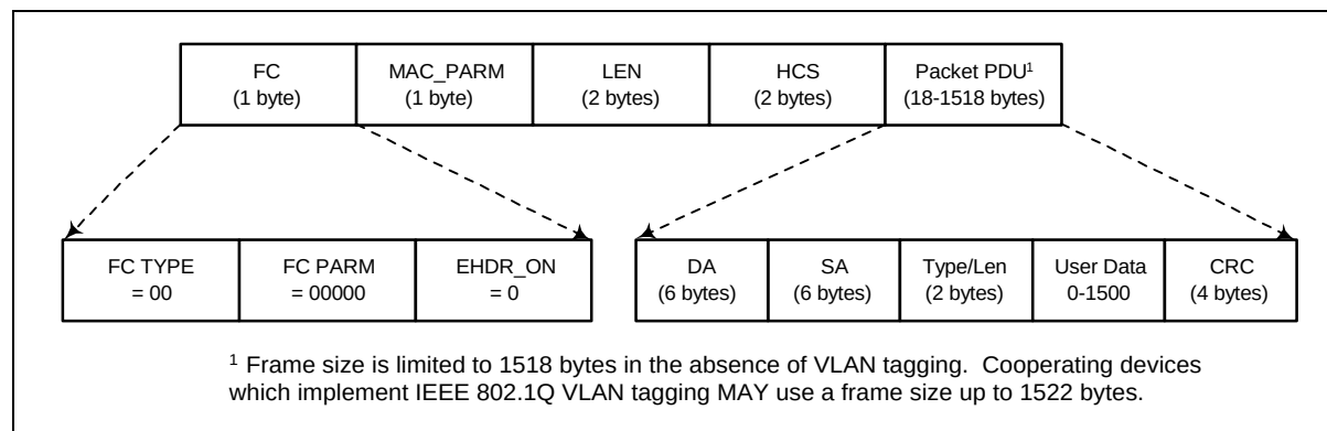
Figure 8-4 Ethernet/802.3 Packet PDU Format
