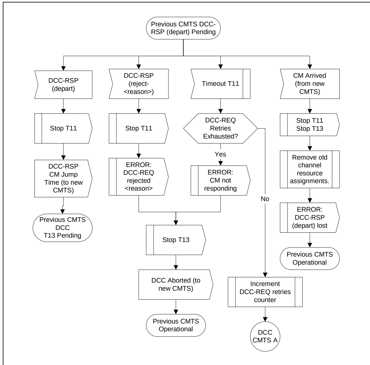
Figure 11-59 Dynamically Changing Channels: CMTS View Part 2
