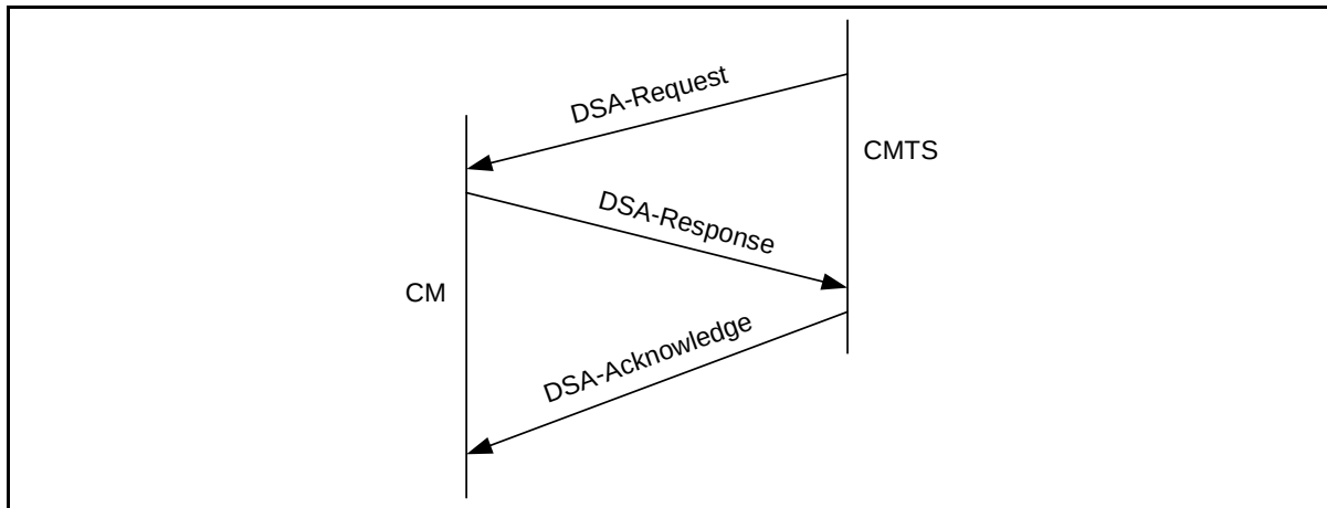
Figure 10-7 Dynamic Service Addition Message Flow — CMTS Initiated
