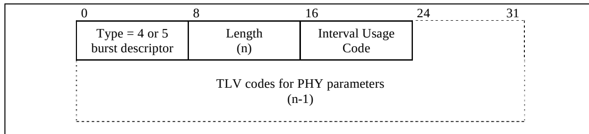
Figure 8-17 Top-Level Encoding for Burst Descriptors
