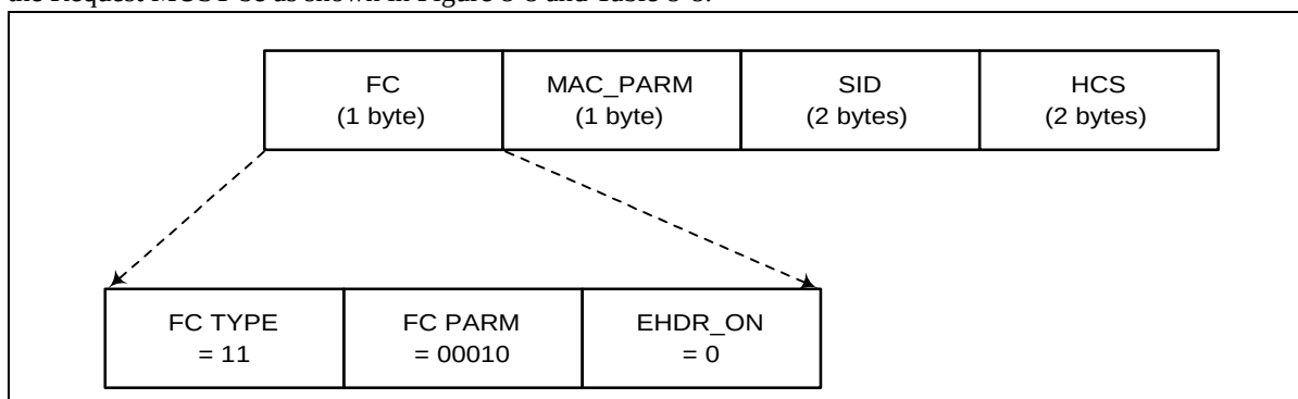
Figure 8-8 Request Frame Format
