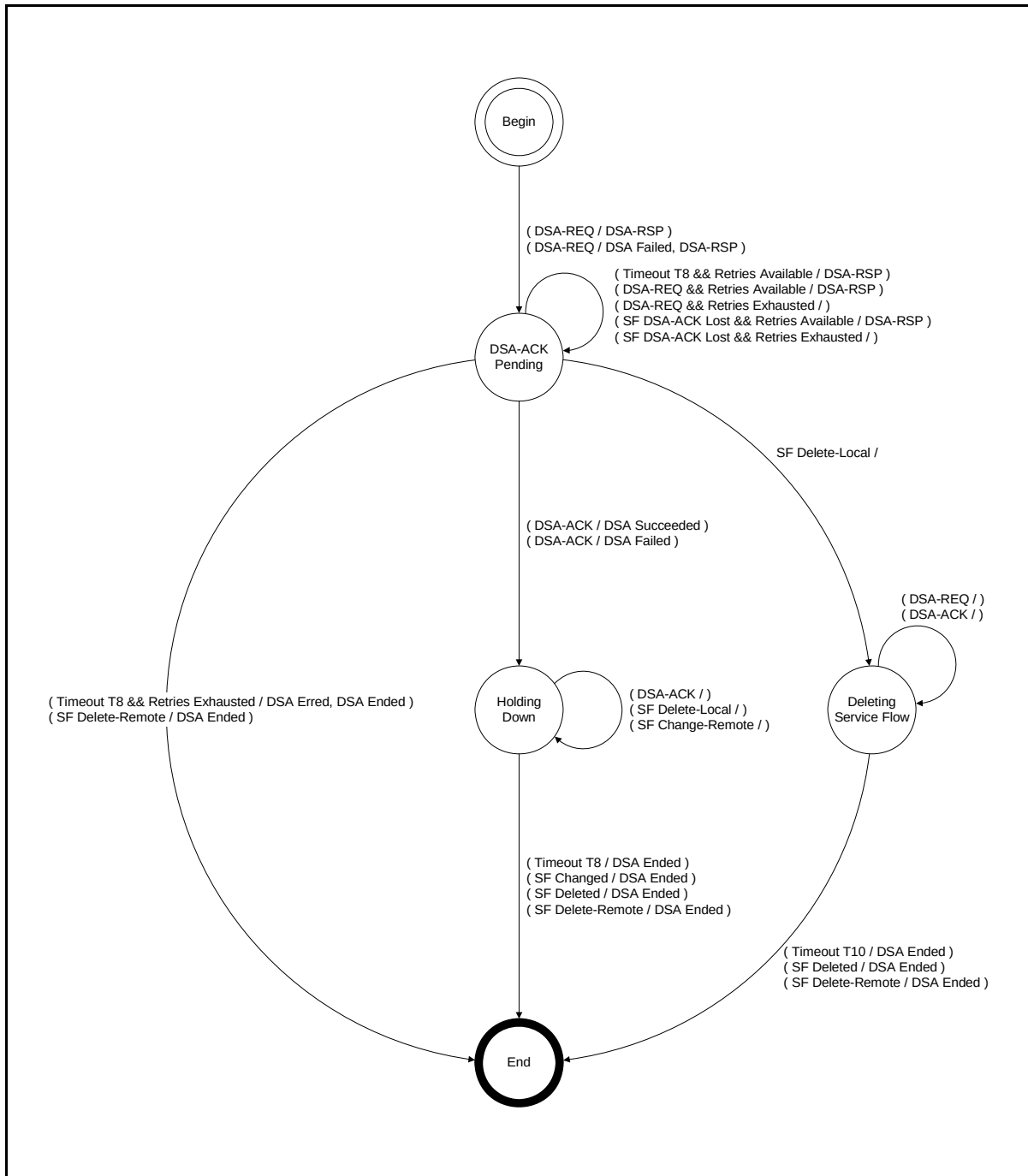
Figure 11-24 DSA—Remotely Initiated Transaction State Transition Diagram
