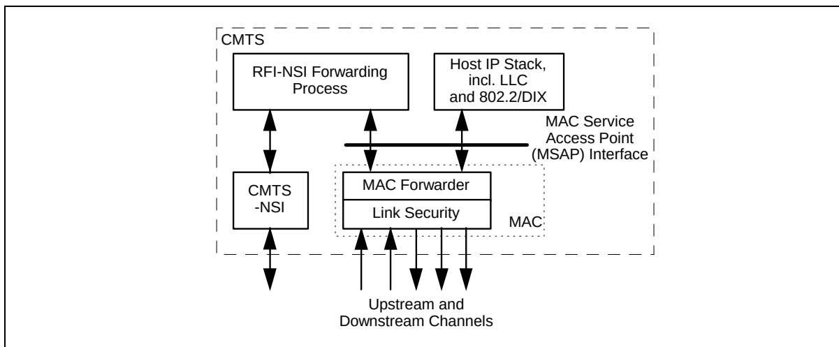
Figure 5-4 MAC Forwarder
