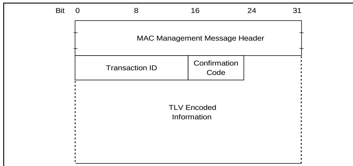
Figure 8-34 Dynamic Service Change — Response
