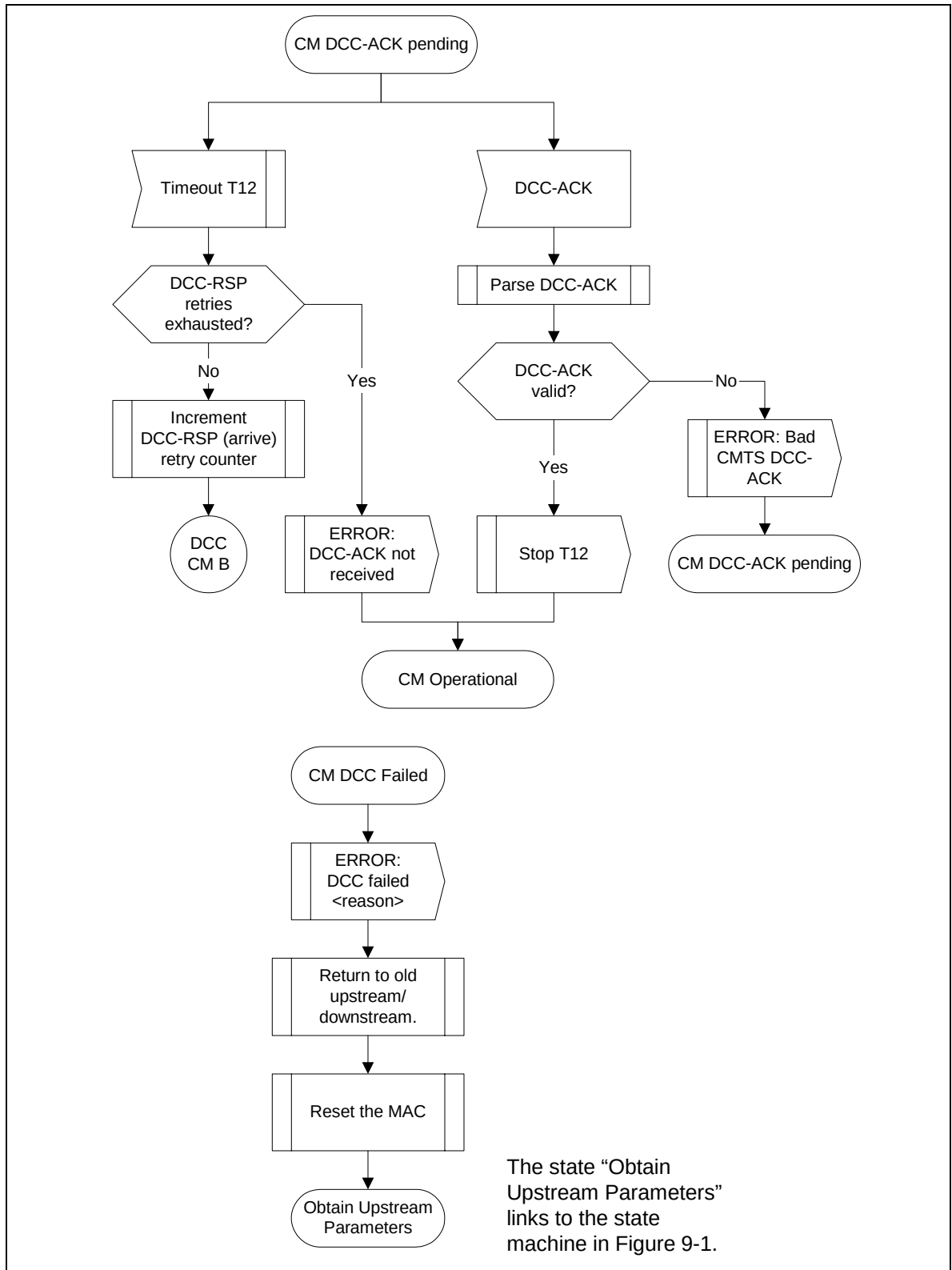
Figure 11-65 Dynamically Changing Channels: CM View Part 4
