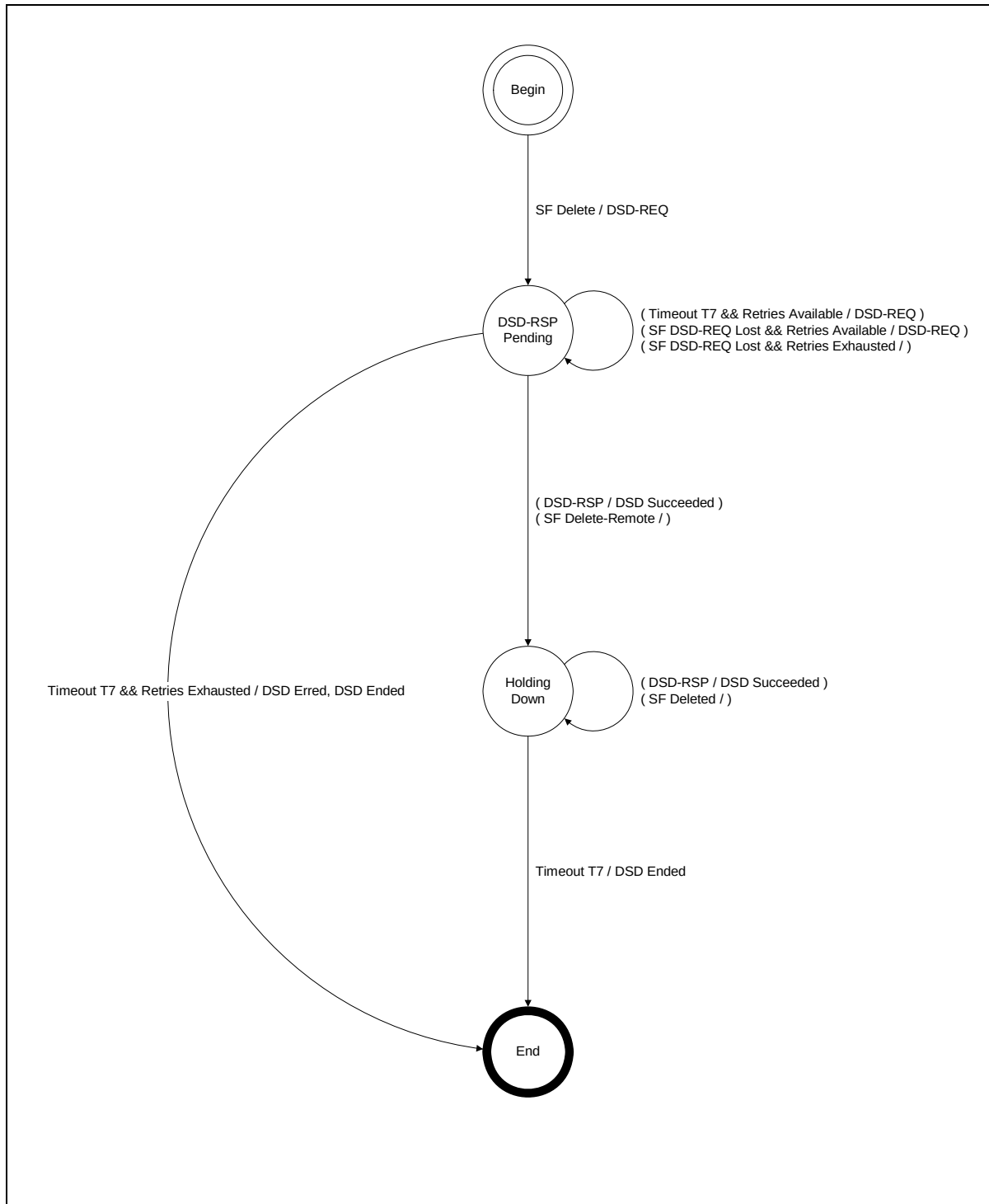
Figure 11-27 DSD—Locally Initiated Transaction State Transition Diagram
