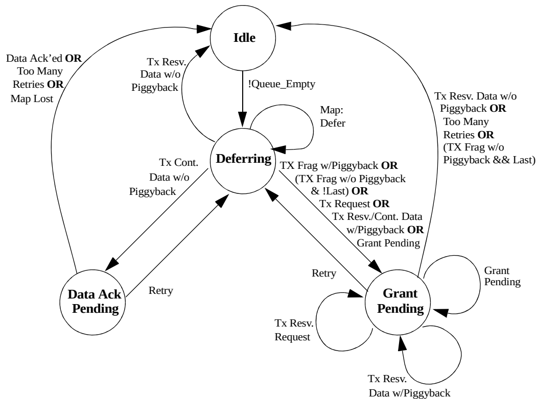
Figure IV-1 Transmission & Deference State Transition Diagram
