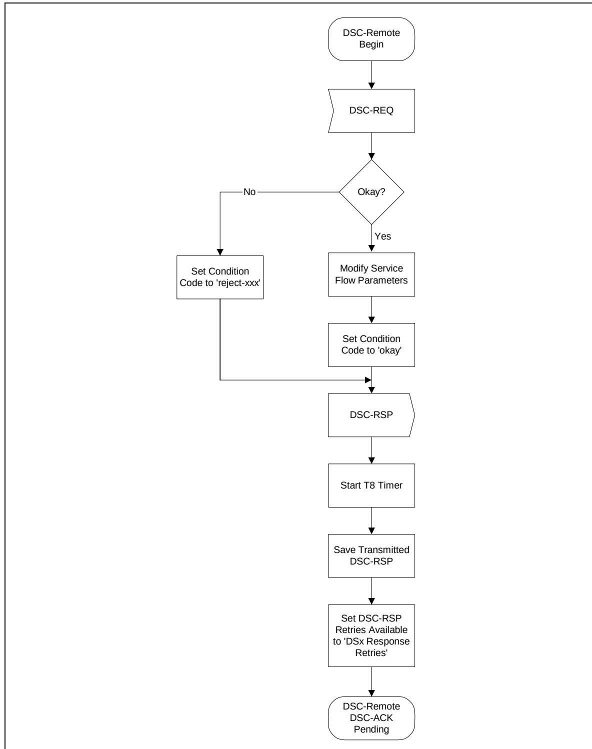
Figure 11-47 DSC—Remotely Initiated Transaction Begin State Flow Diagram 1
