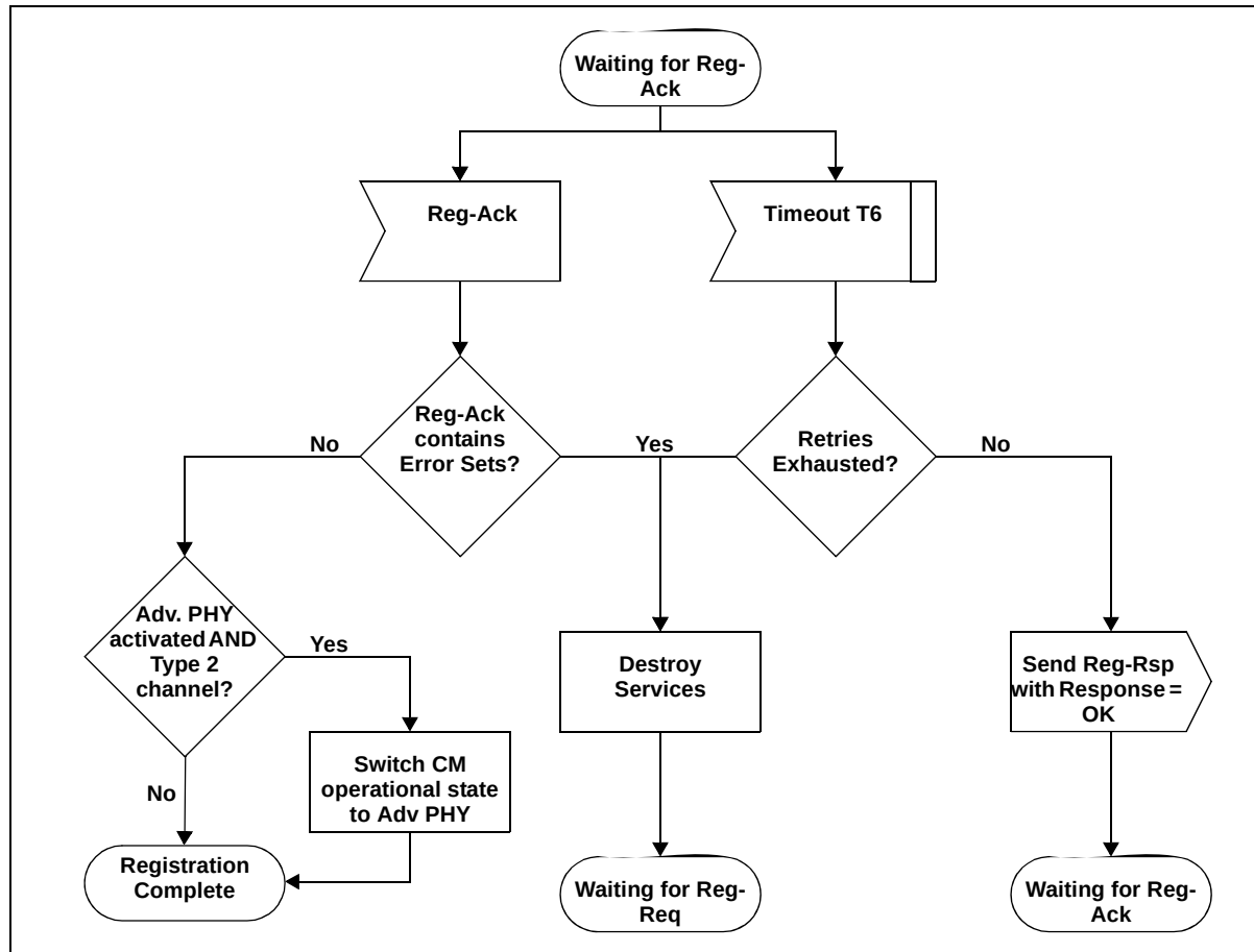
Figure 11-15 Registration Acknowledgment— CMTS 1
