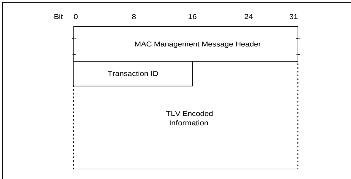
Figure 8-30 Dynamic Service Addition — Request
