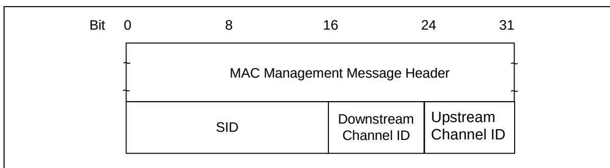
Figure 8-44 Packet PDU Following the Timing Header
