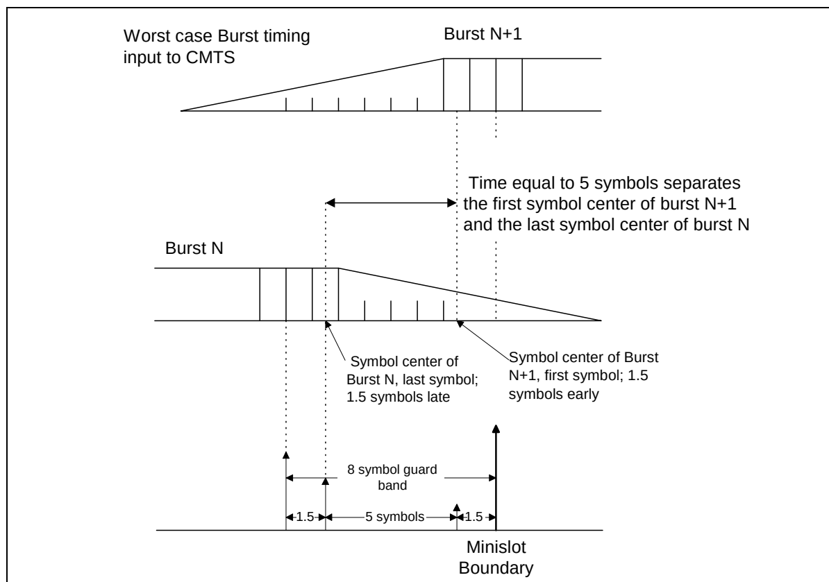
Figure 6-30 Worst-Case TDMA Burst Timing
