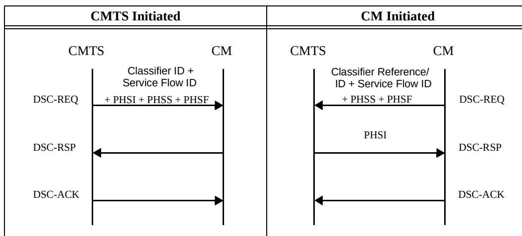
Figure 10-13 Payload Header Suppression Signaling Example
