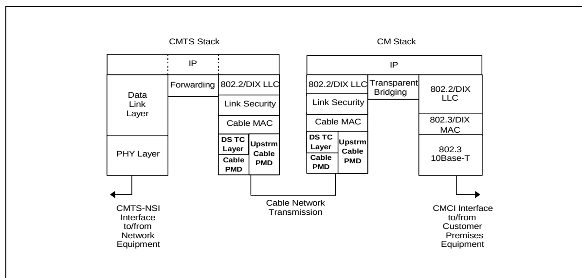
Figure 5-2 Data Forwarding Through the CM and CMTS
