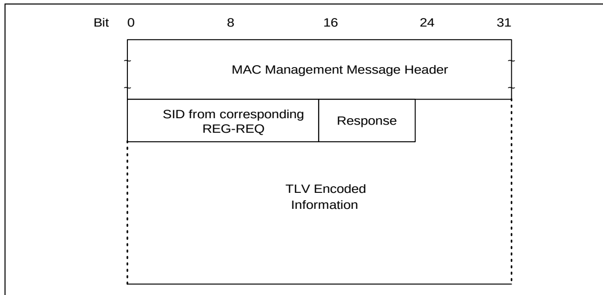
Figure 8-26 Registration Response Format
