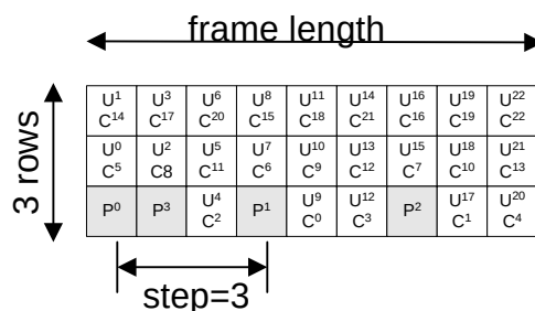
Figure 6-17 Symbol Numbering Without TCM
