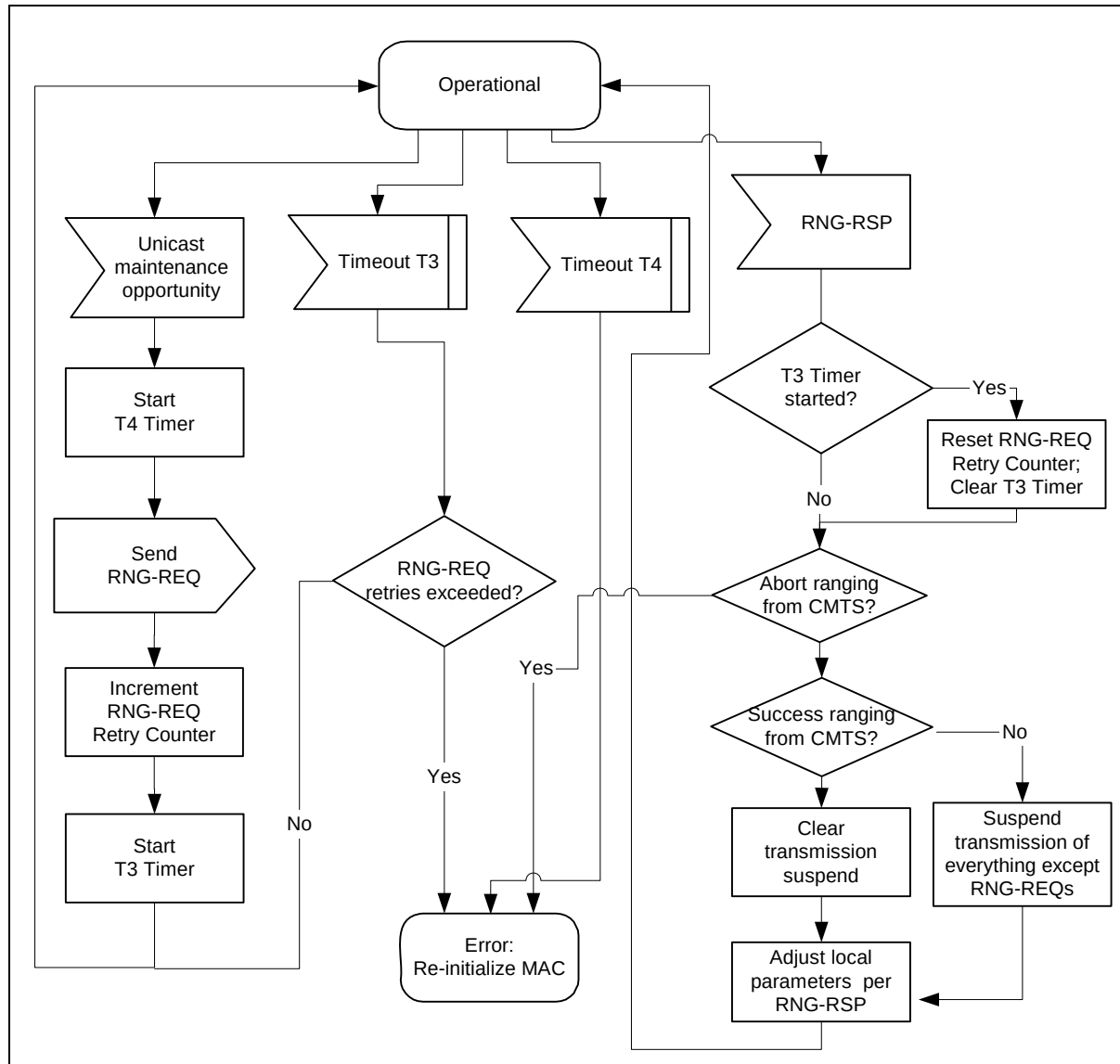
Figure 11-17 Periodic Ranging - CM View
