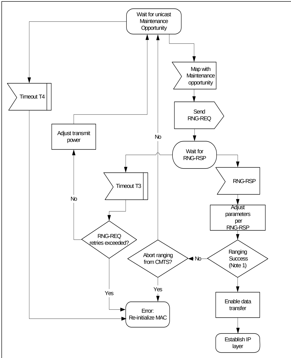
Figure 11-7 Unicast Initial Ranging - CM
