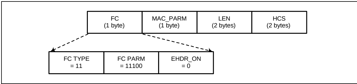
Figure 8-11 Concatenation MAC Header Format
