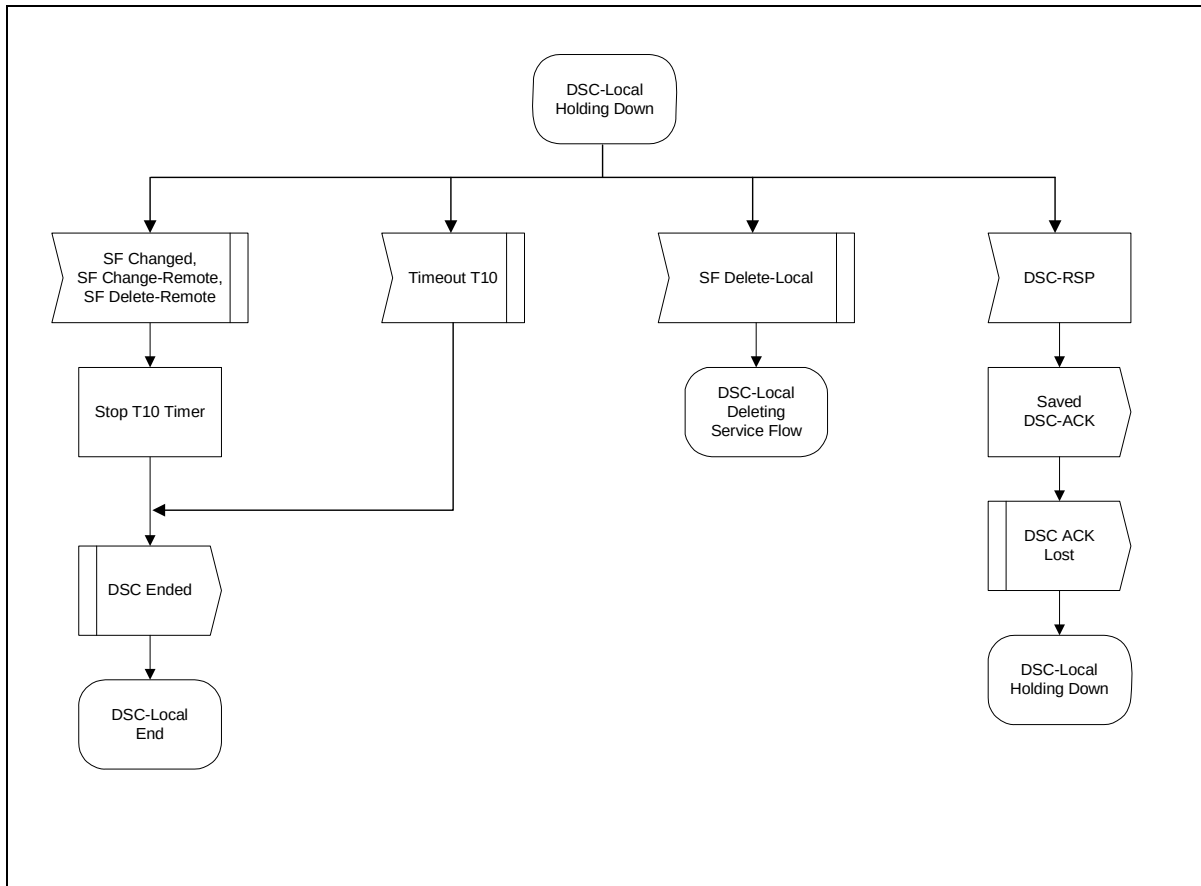
Figure 11-44 DSC—Locally Initiated Transaction Holding Down State Flow Diagram
