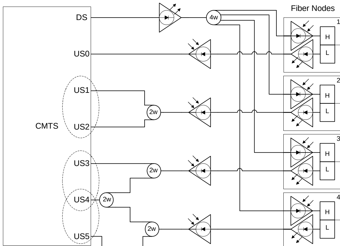
Figure 11-67 Example Combining Network 1
