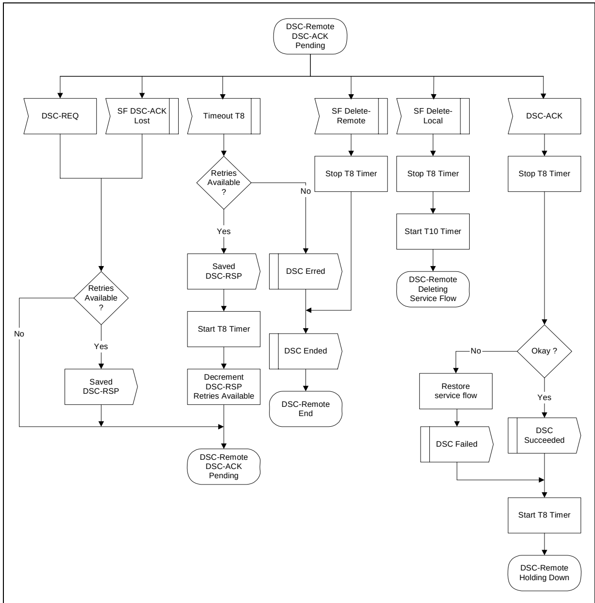
Figure 11-48 DSC—Remotely Initiated Transaction DSC-ACK Pending State Flow Diagram 1
