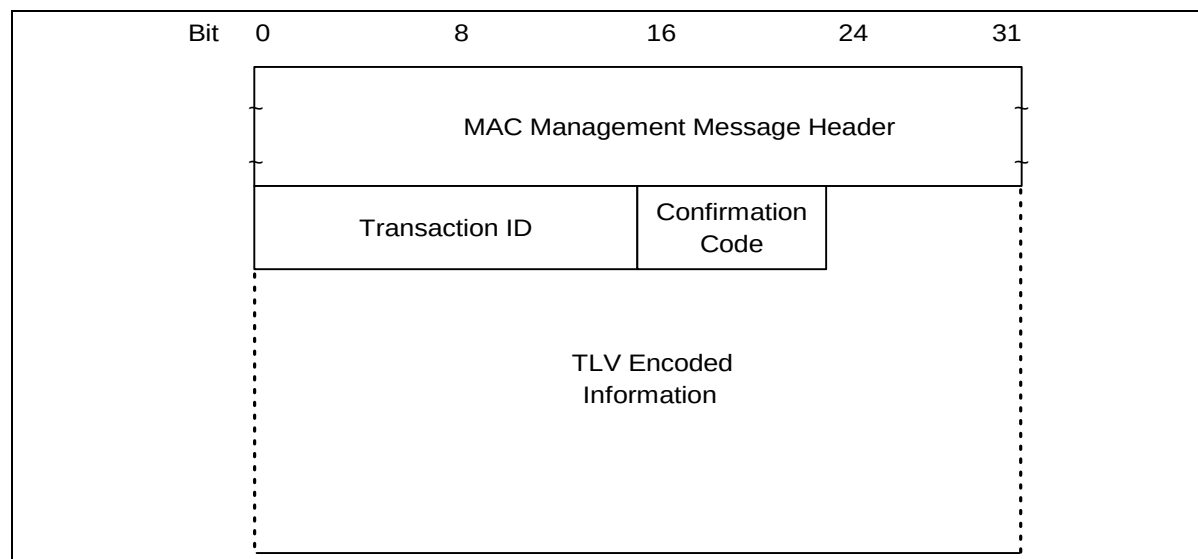
Figure 8-31 Dynamic Service Addition — Response
