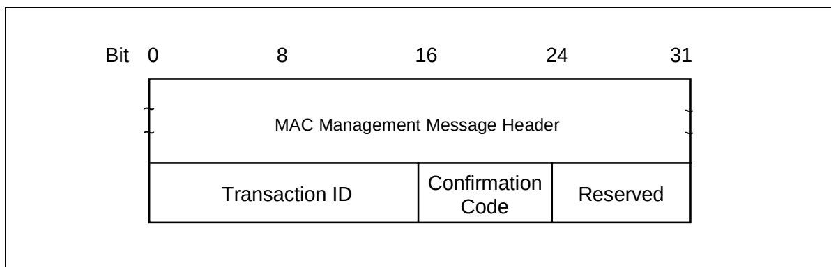
Figure 8-37 Dynamic Service Deletion — Response
