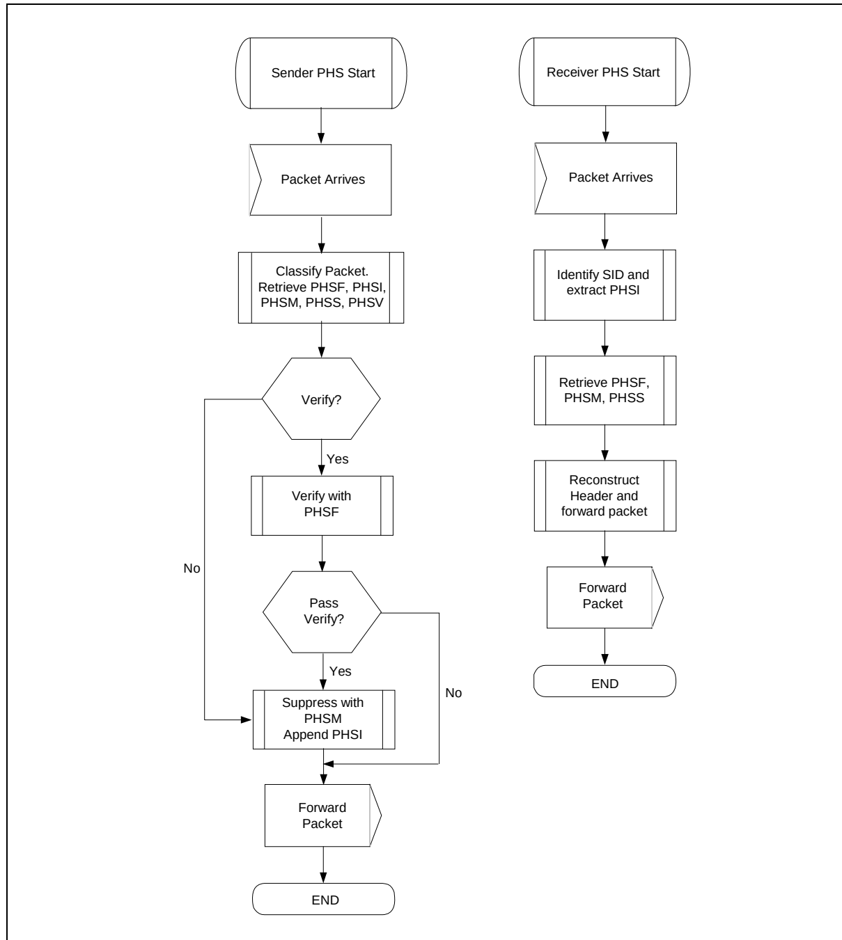
Figure 10-11 Payload Header Suppression Operation
