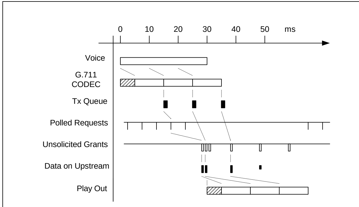
Figure VI-2 VAD Start-Up and Stop
