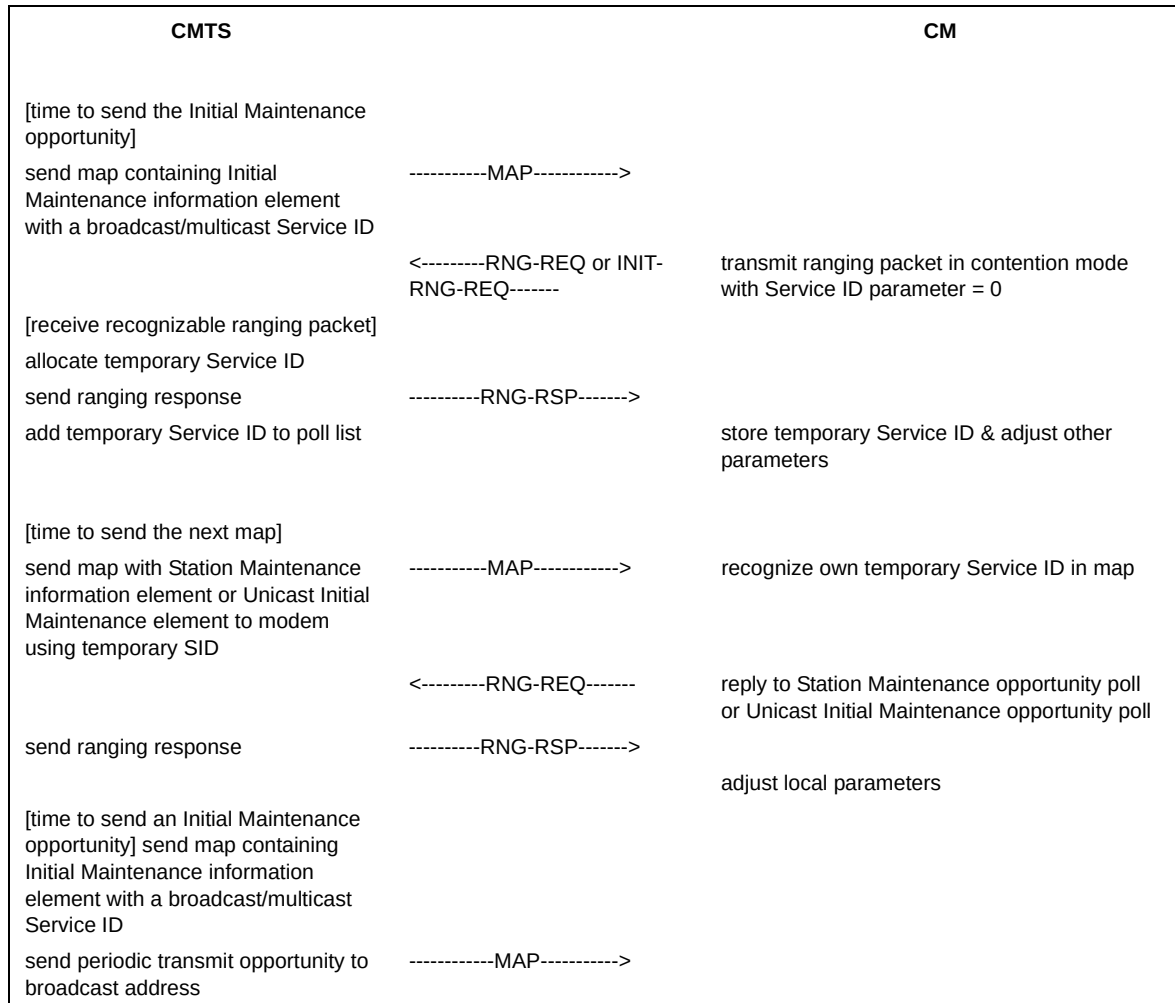
Figure 11-5 Ranging and Automatic Adjustments Procedure
