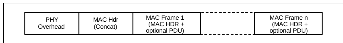
Figure 8-10 Concatenation of Multiple MAC Frames
