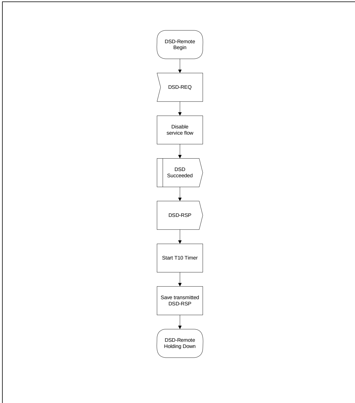
Figure 11-56 DSD—Remotely Initiated Transaction Begin State Flow Diagram
