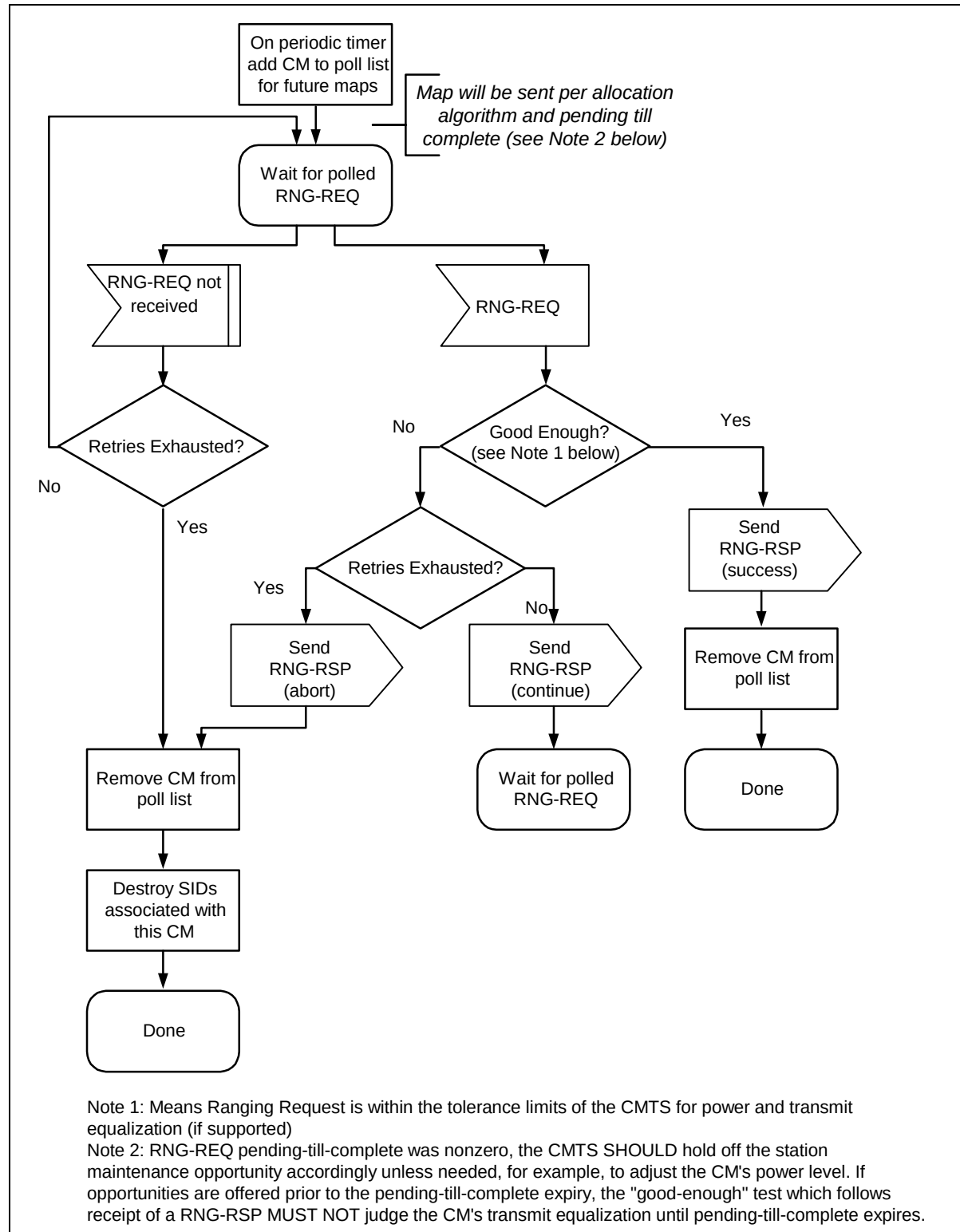
Figure 11-16 Periodic Ranging - CMTS
