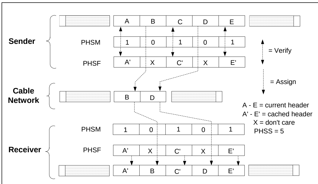
Figure 10-12 Payload Header Suppression with Masking
