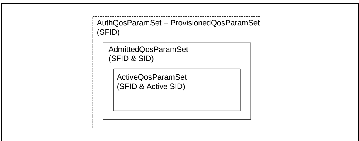
Figure 10-1 Provisioned Authorization Model “Envelopes”
