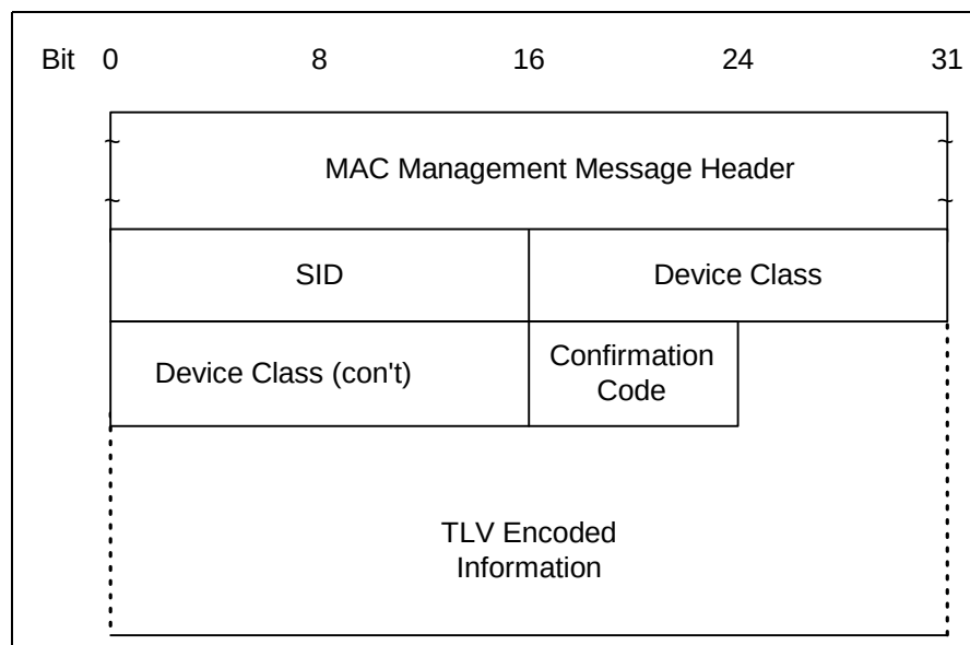
Figure 8-42 Device Class Identification Response
