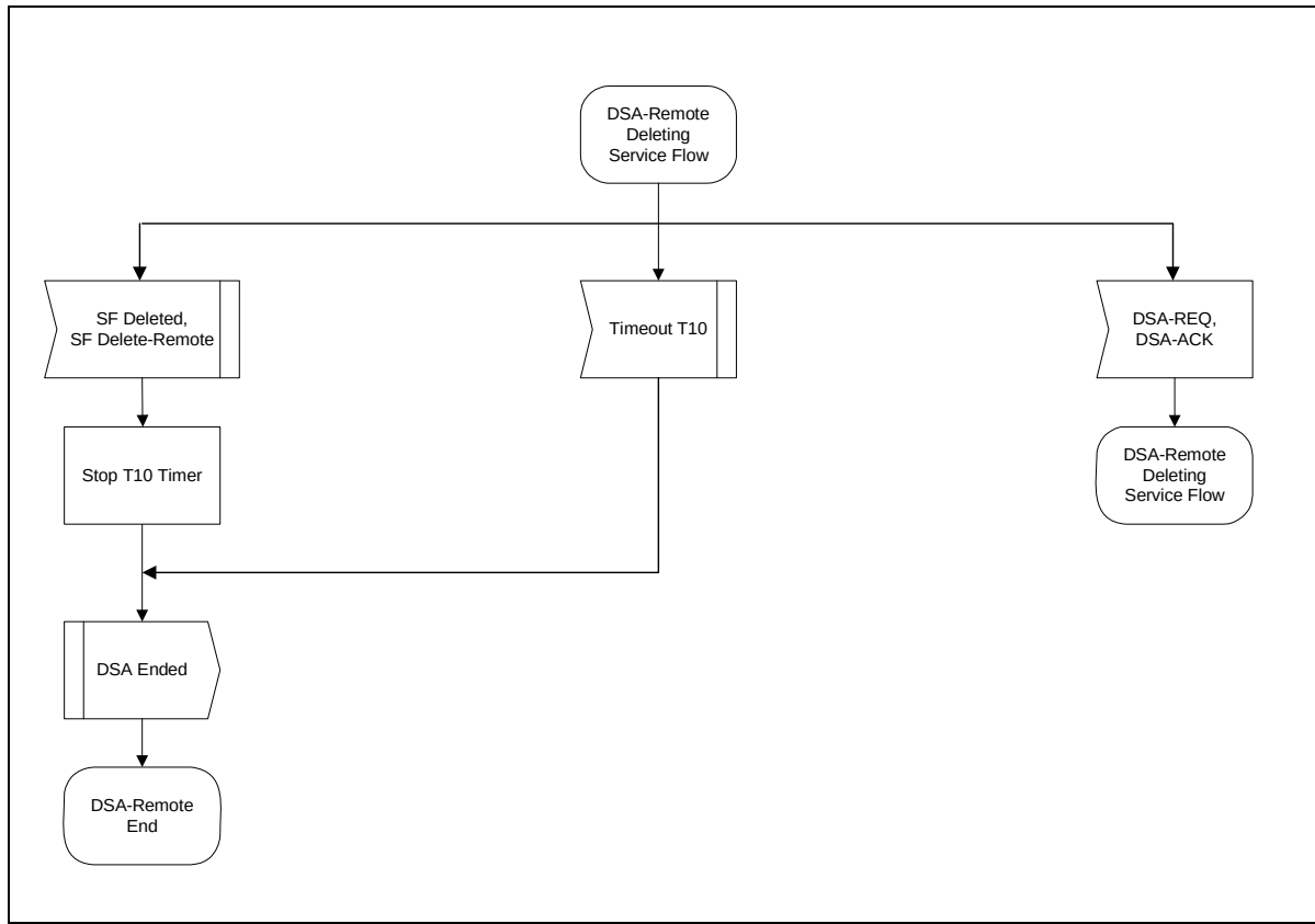
Figure 11-39 DSA—Remotely Initiated Transaction Deleting Service State Flow Diagram
