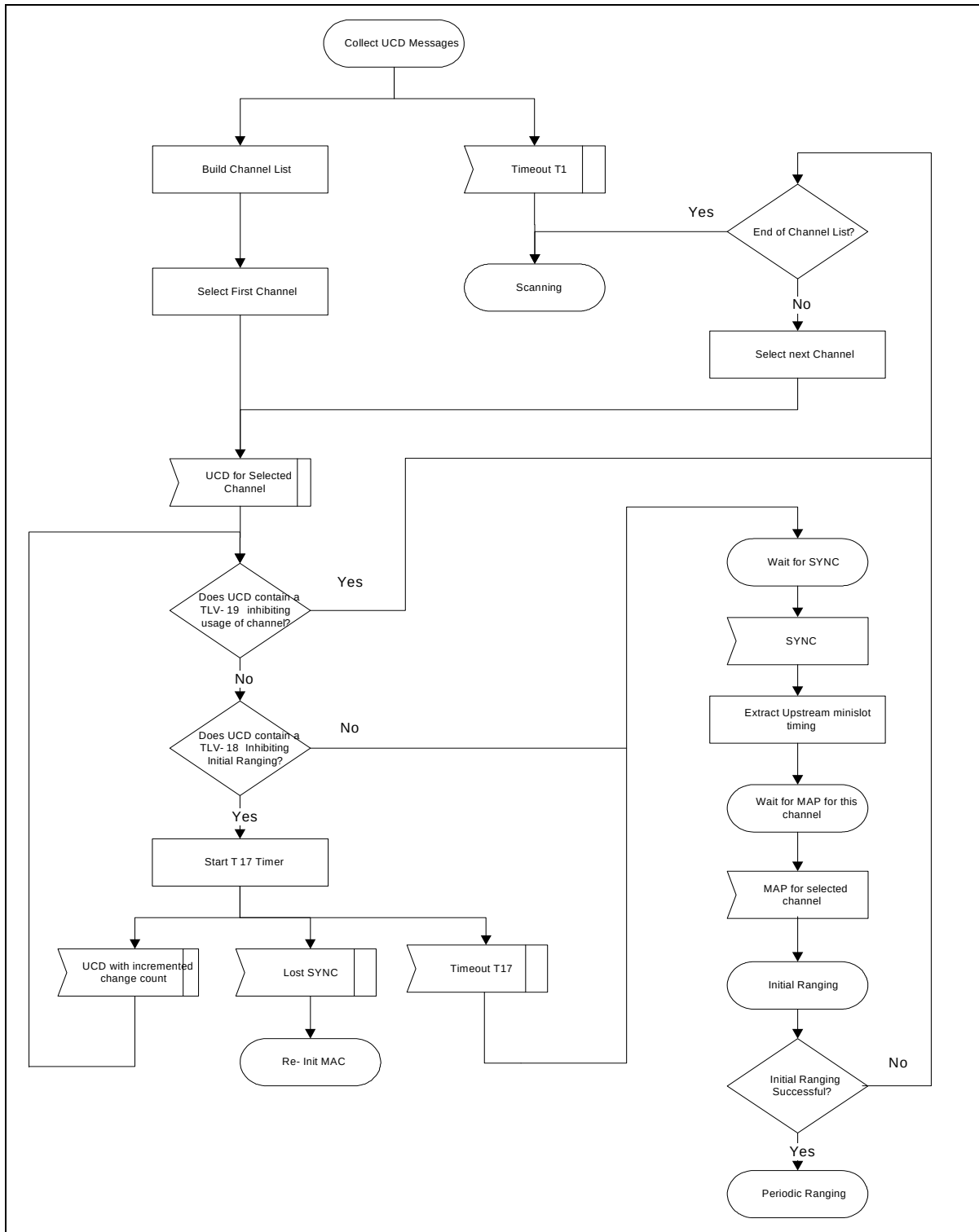
Figure 11-3 Obtaining Upstream Parameters 1
