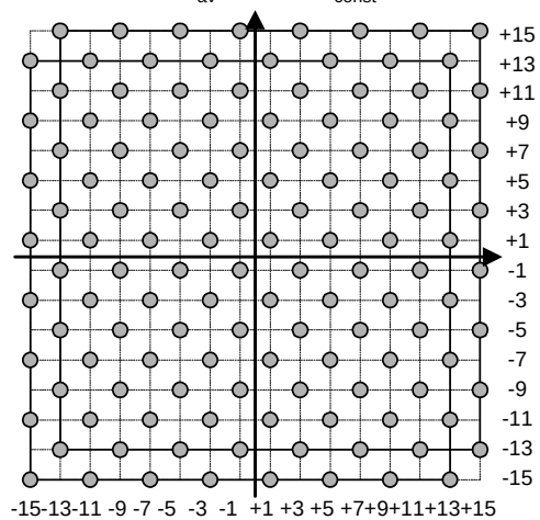
Figure 6-18 Symbol Constellations
