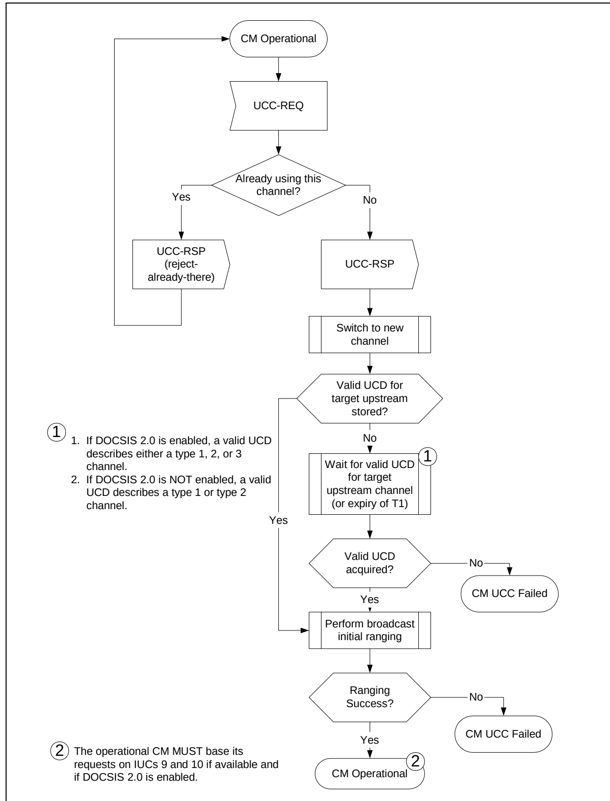
Figure 11-19 Changing Upstream Channels: CM View Part 1
