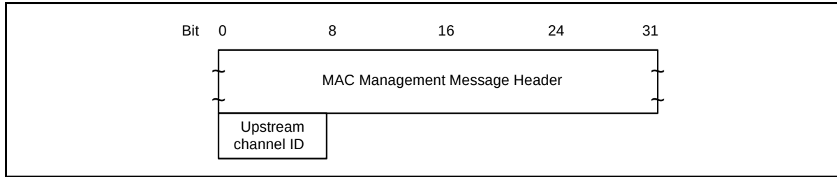
Figure 8-29 Upstream Channel Change Response
