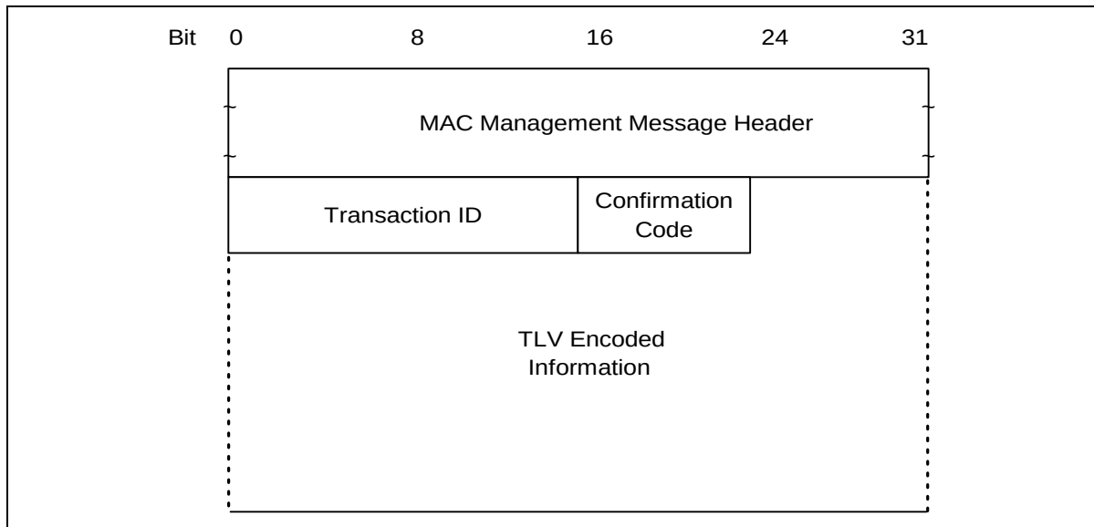
Figure 8-32 Dynamic Service Addition — Acknowledge
