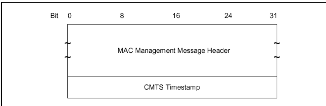
Figure F-1 Format of Packet PDU Following the Timing Header
