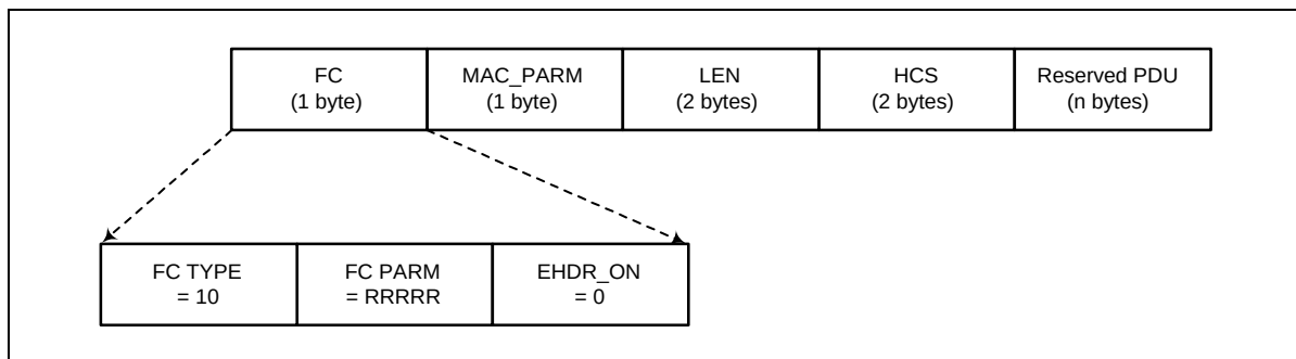
Figure 8-5 Reserved PDU Format
