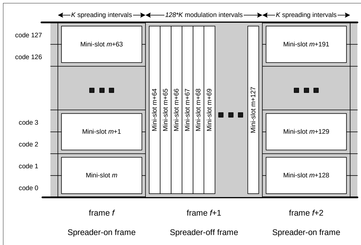
Figure 6-15 S-CDMA and Spreader-off Intervals
