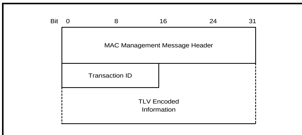
Figure 8-38 Dynamic Channel Change Request
