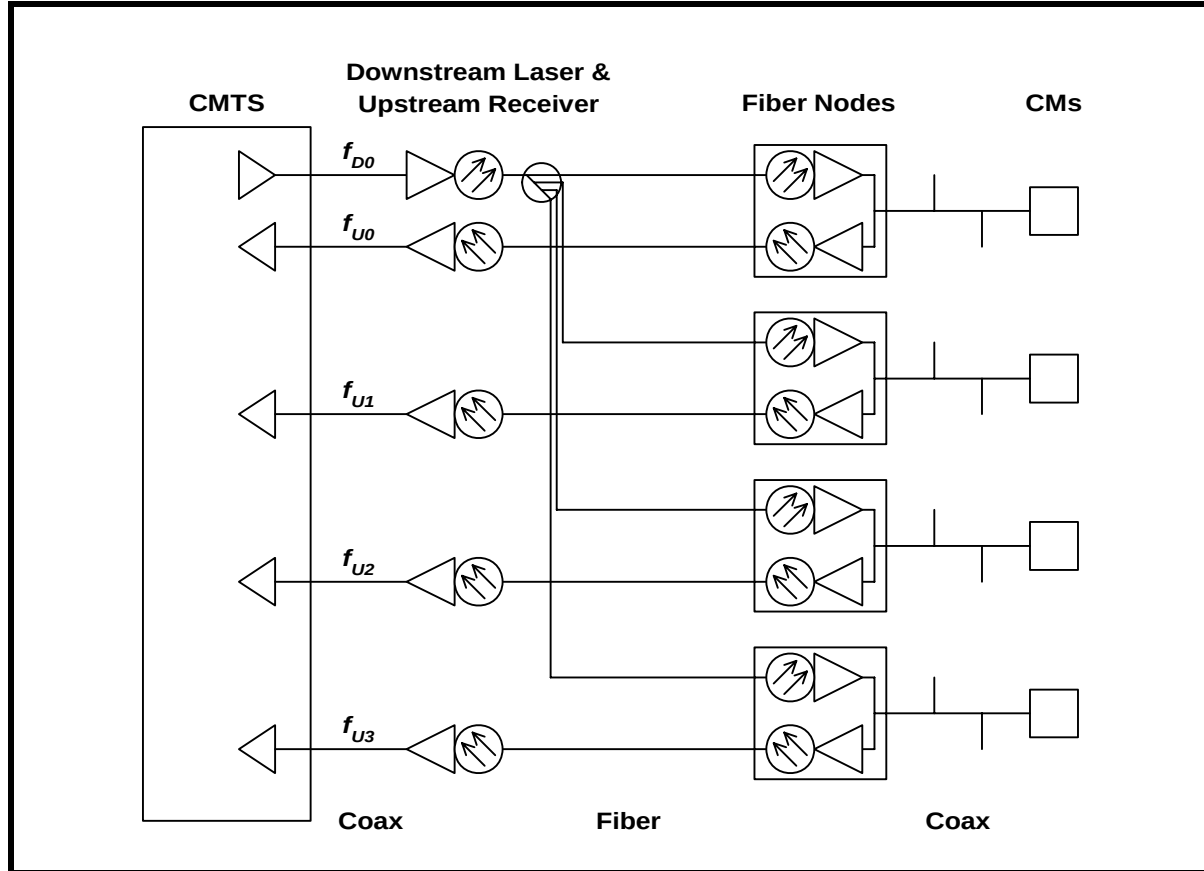
Figure III-1 Single Downstream and Single Upstream Channels per CM
