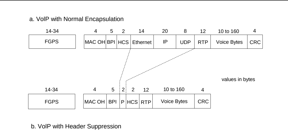
Figure 10-14 Upstream Payload Header Suppression Example
