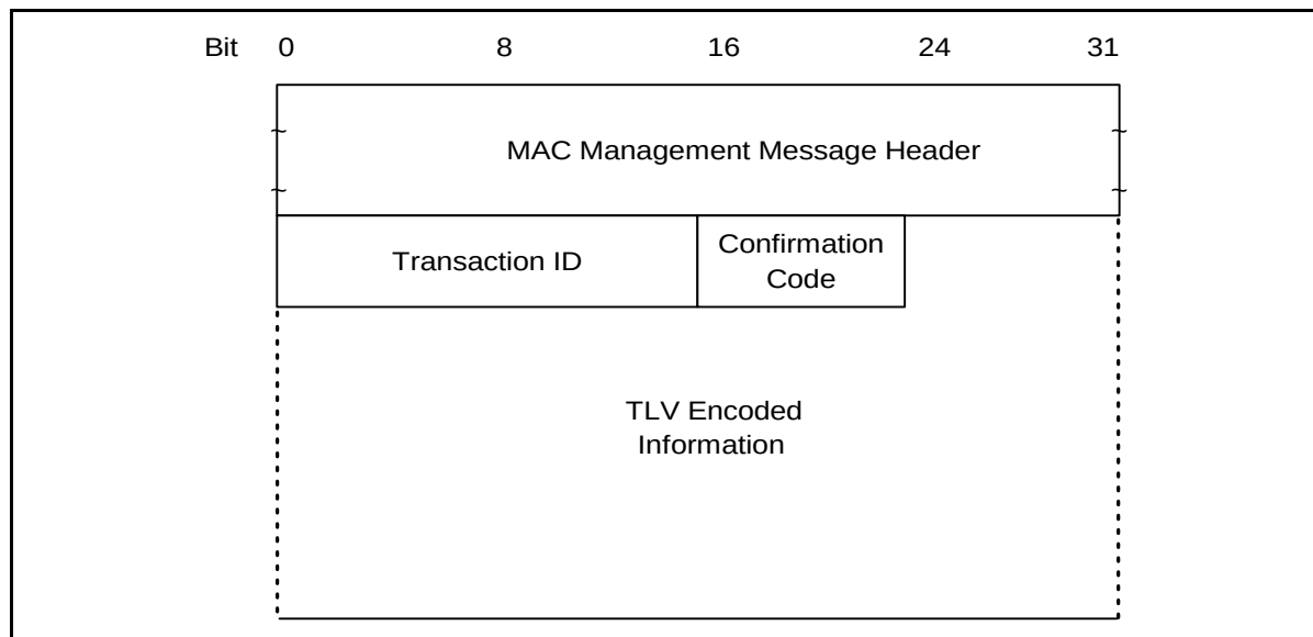
Figure 8-35 Dynamic Service Change — Acknowledge
