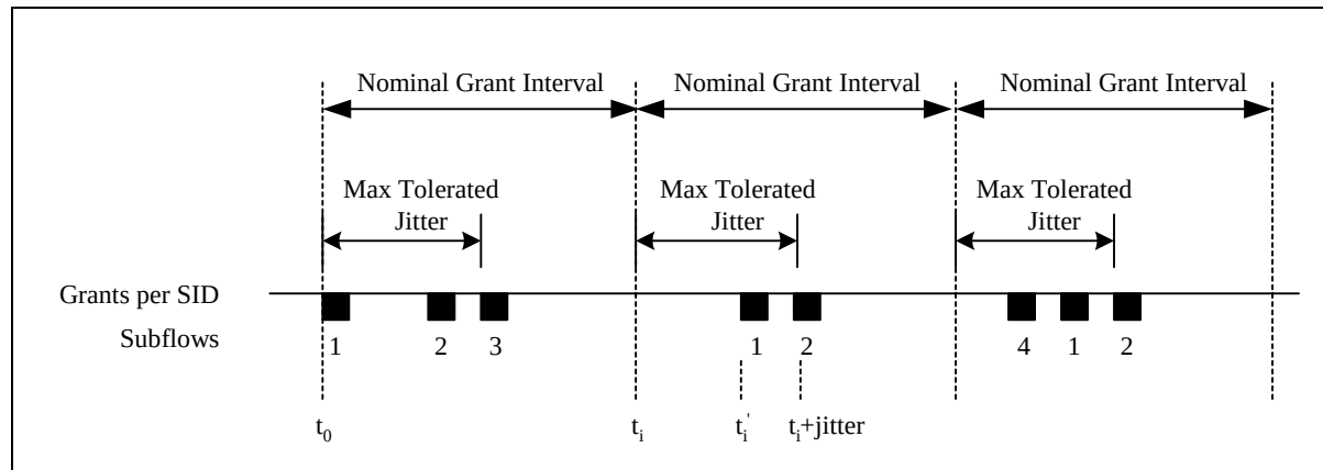
Figure VI-1 Example Jitter with Multiple Grants per SID
