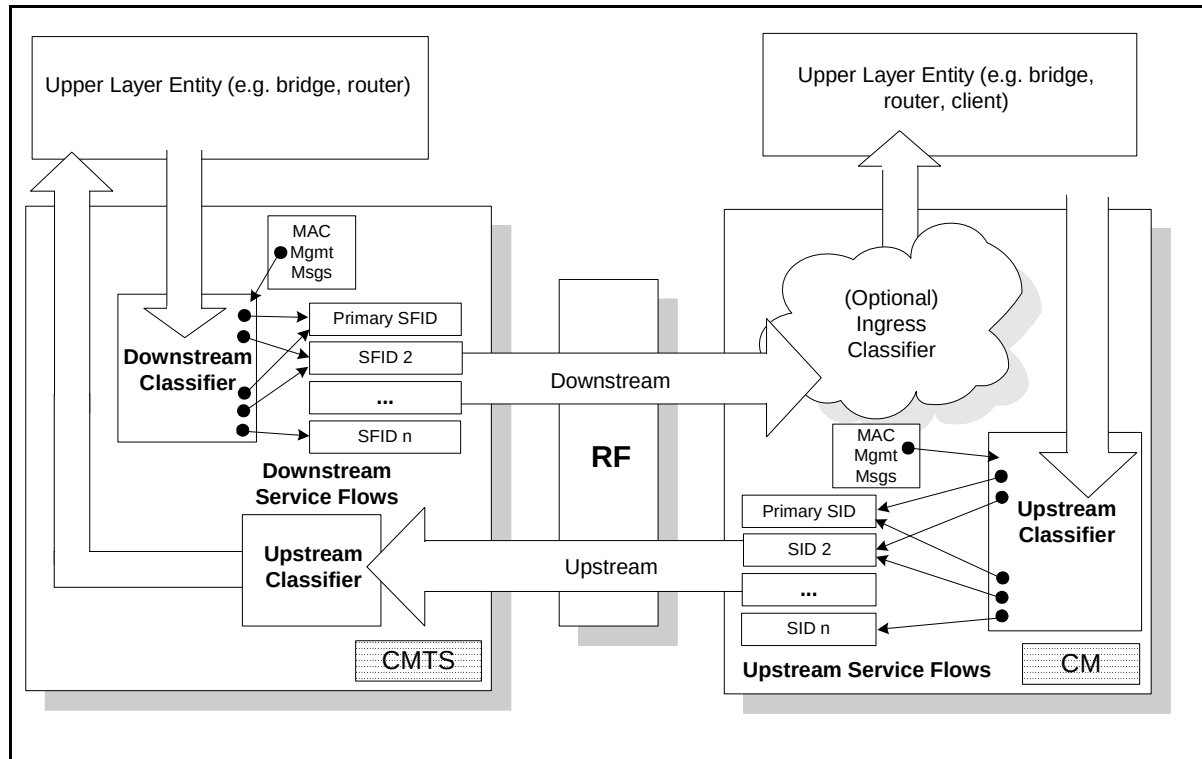
Figure 10-3 Classification within the MAC Layer
