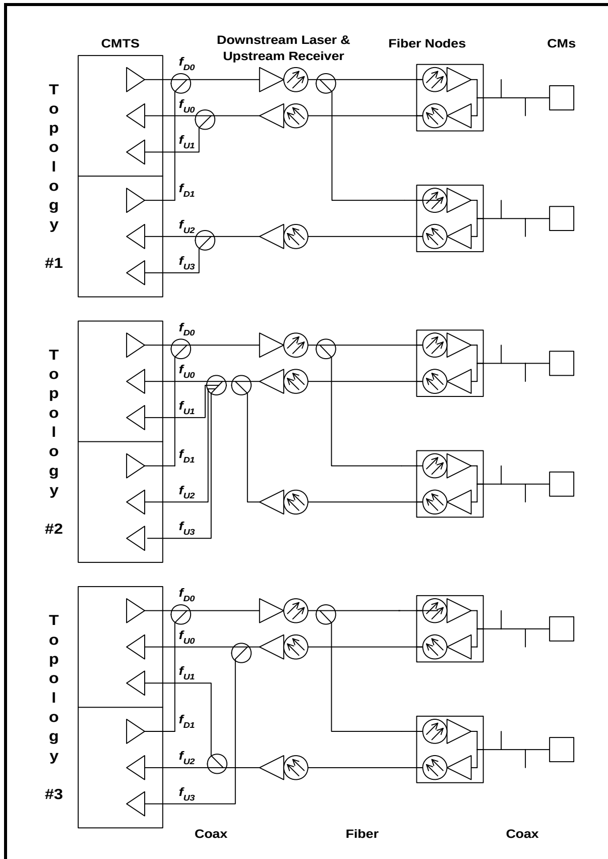
Figure III-2 Multiple Downstream and Multiple Upstream Channels per CM
