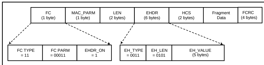
Figure 8-9 Fragmentation MAC Header Format
