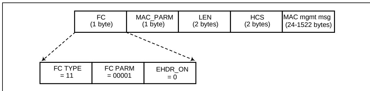
Figure 8-7 Management MAC Header
