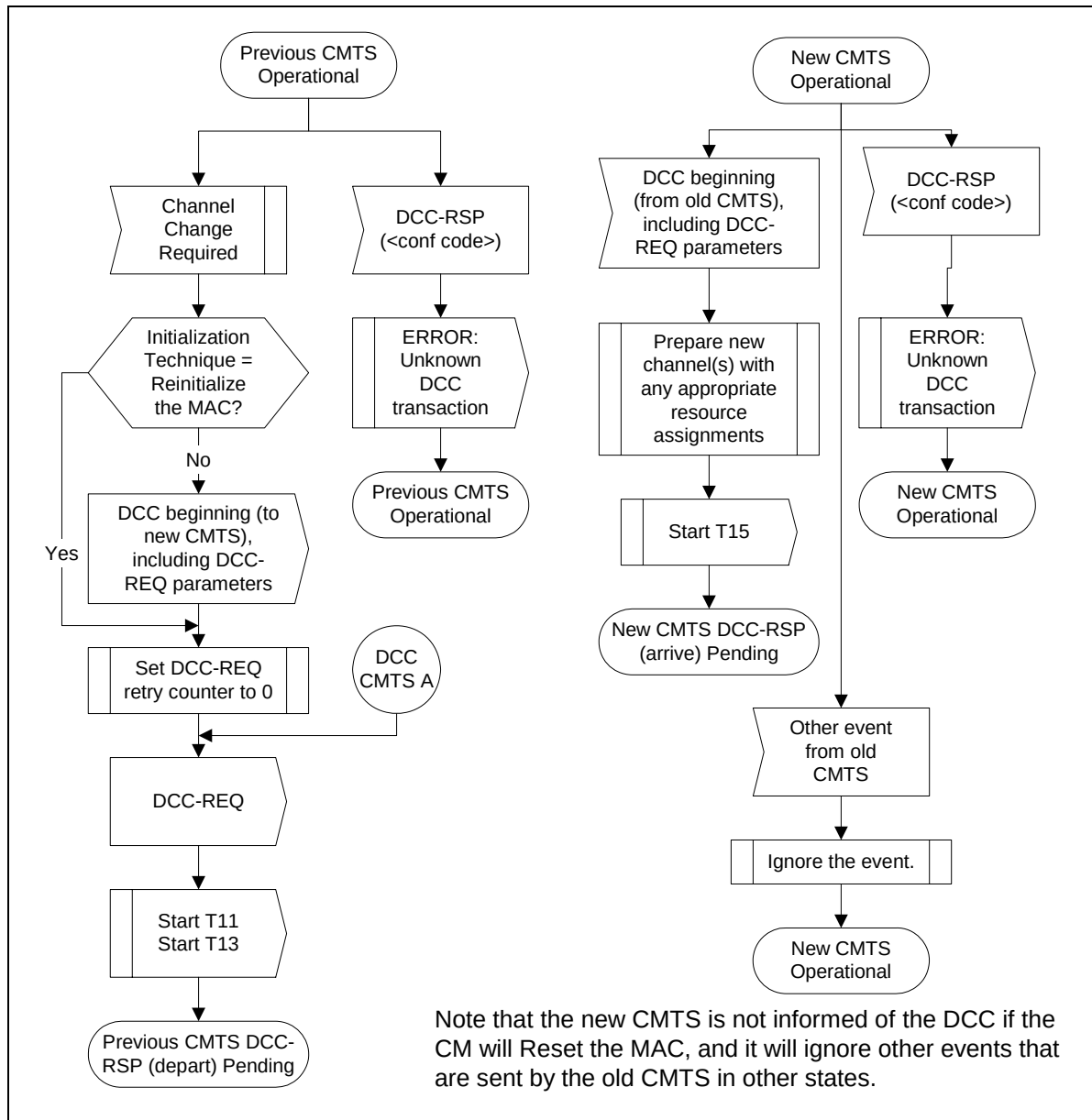
Figure 11-58 Dynamically Changing Channels: CMTS View Part 1
