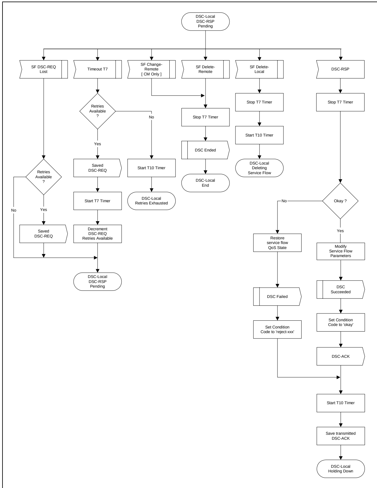
Figure 11-43 DSC—Locally Initiated Transaction DSC-RSP Pending State Flow Diagram
