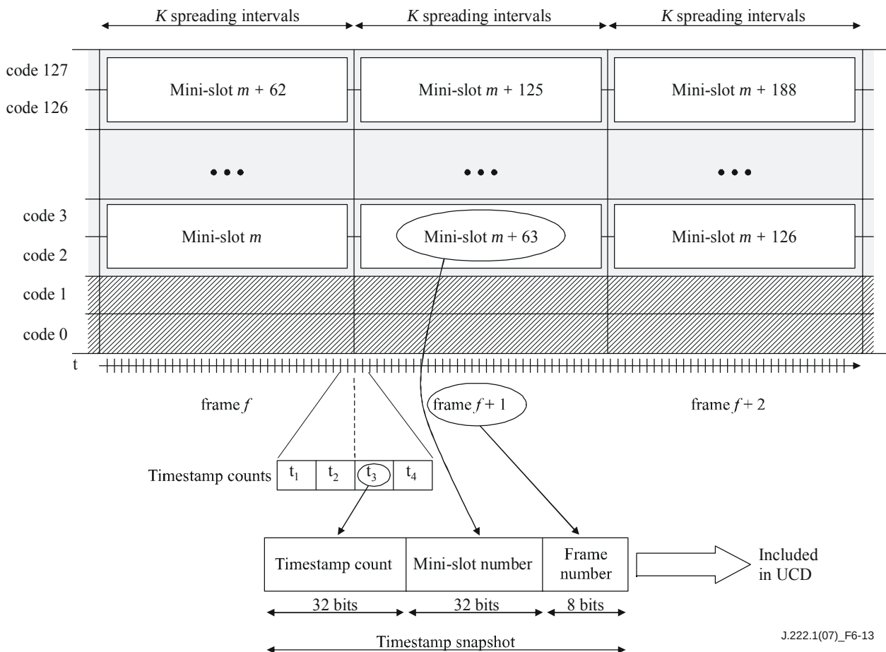
Figure 6-13 – Timestamp snapshot
