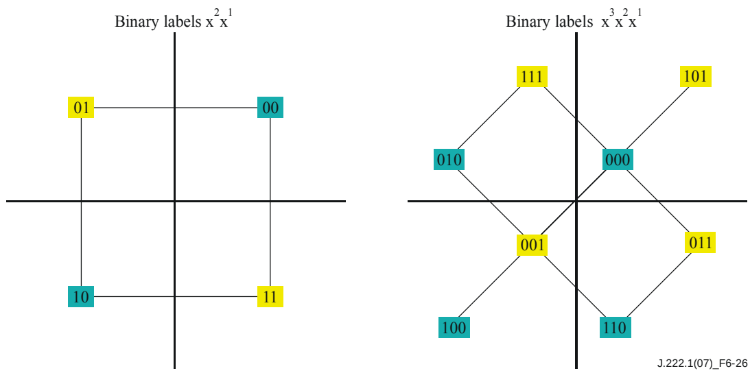
Figure 6-26 – QPSK and 8 QAM TCM symbol mapping
