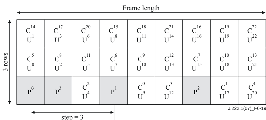
Figure 6-19 – Symbol numbering with and without TCM
