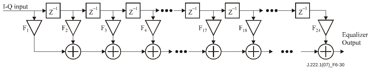
Figure 6-30 – Transmit pre-equalizer structure
