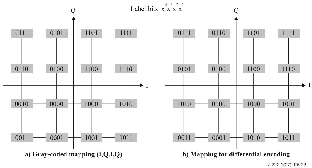
Figure 6-23 – 16 QAM symbol mapping
