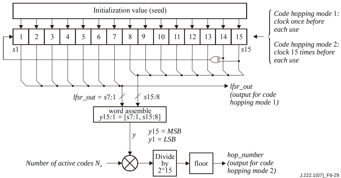
Figure 6-29 – Code hopping random number generator
