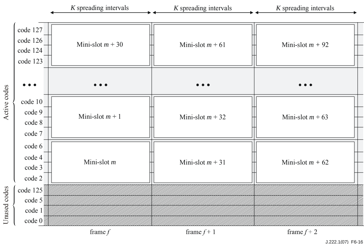
Figure 6-16 – Mini-slot mapping with four codes per mini-slot, 124 active codes, codes 0, 1, 5, and 125 unused; selectable active codes mode 2
