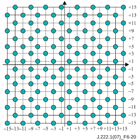
Figure 6-20 – Symbol constellations
