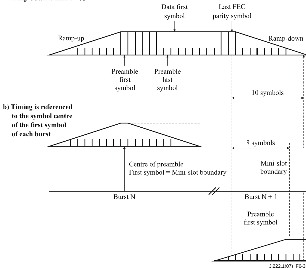
Figure 6-31 – Nominal TDMA burst timing
