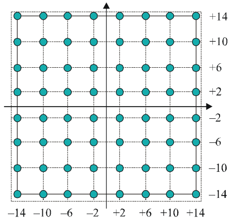
Figure 6-20 – Symbol constellations
