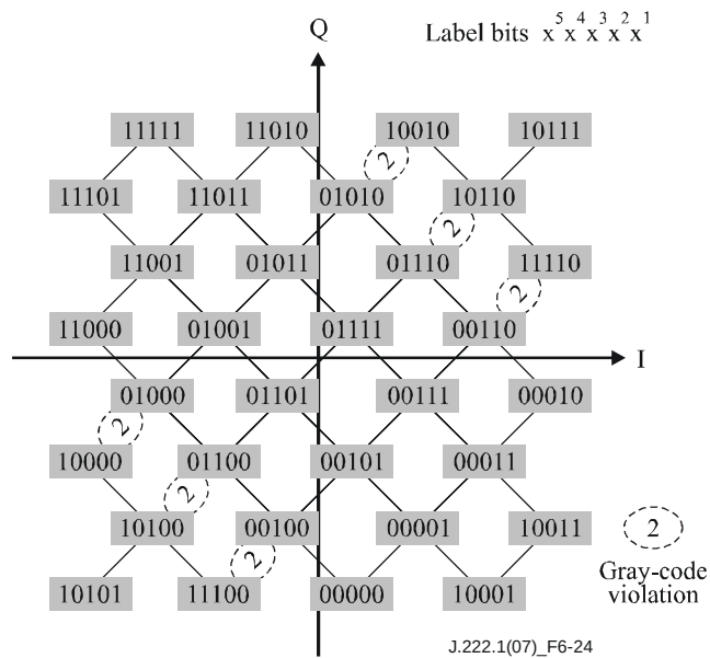
Figure 6-24 – 32 QAM symbol mapping
