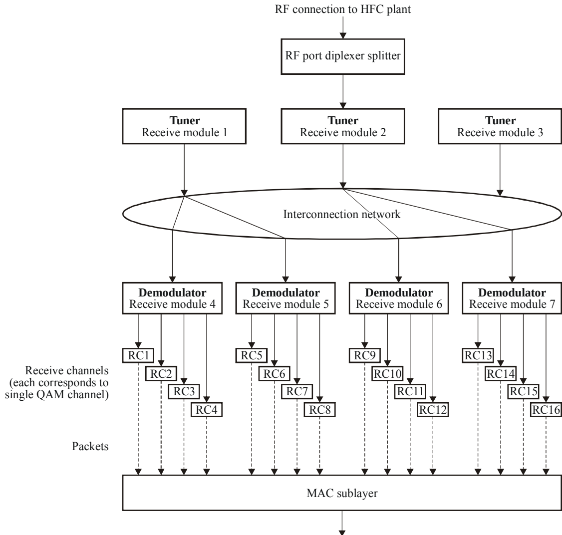
Figure 6-34 – Example manufacturer receive channel profile
