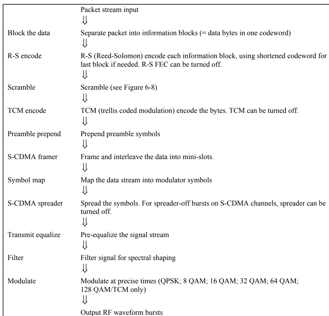
Figure 6-3 – S-CDMA upstream transmission processing
