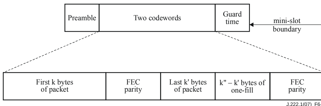
Figure 6-4 – Example frame structures with flexible burst length mode, DOCSIS 3.0 operation
