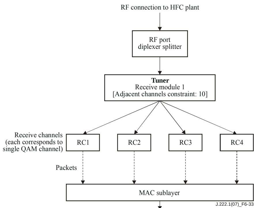
Figure 6-33 – 6 MHz DOCSIS standard receive channel profile 01
