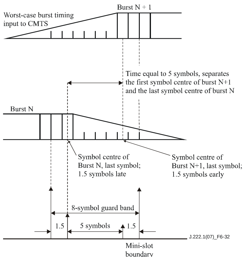
Figure 6-32 – Worst-case TDMA burst timing
