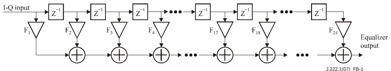
Figure B.1 – Transmit pre-equalizer structure
