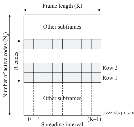
Figure 6-18 – Subframe structure
