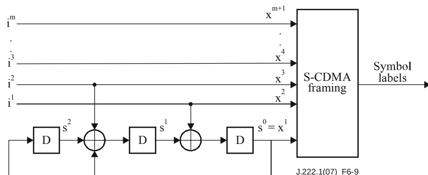
Figure 6-9 – Convolutional encoder
