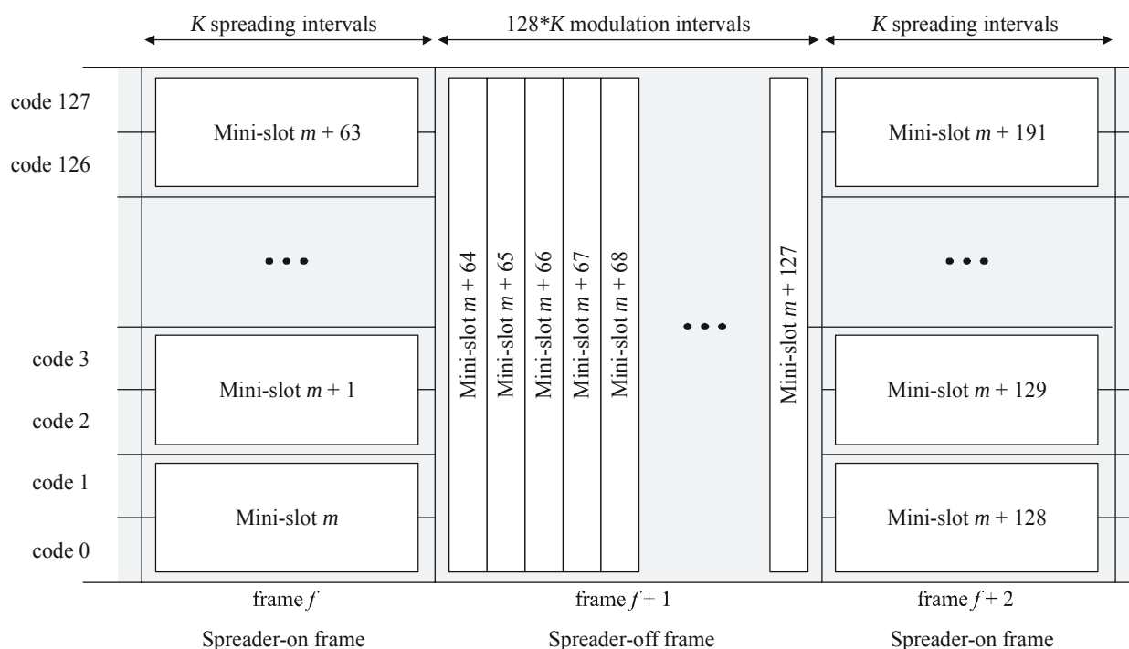
Figure 6-17 – S-CDMA spreader-on and spreader-off intervals
