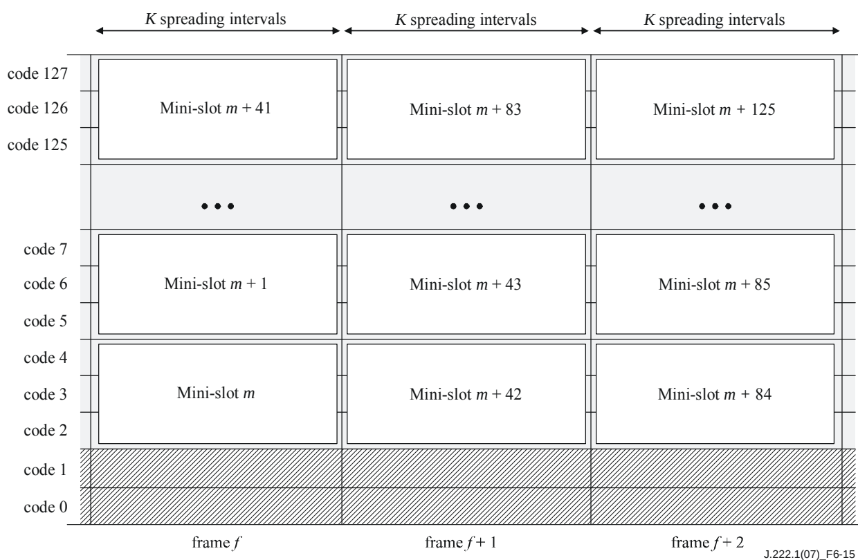
Figure 6-15 – Mini-slot mapping with three codes per mini-slot, 126 active codes
