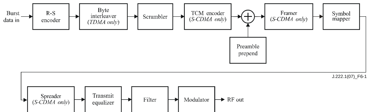
Figure 6-1 – Upstream signal-processing sequence
