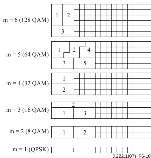
Figure 6-10 – Repetitive patterns of byte mapping to symbol map bits for TCM
