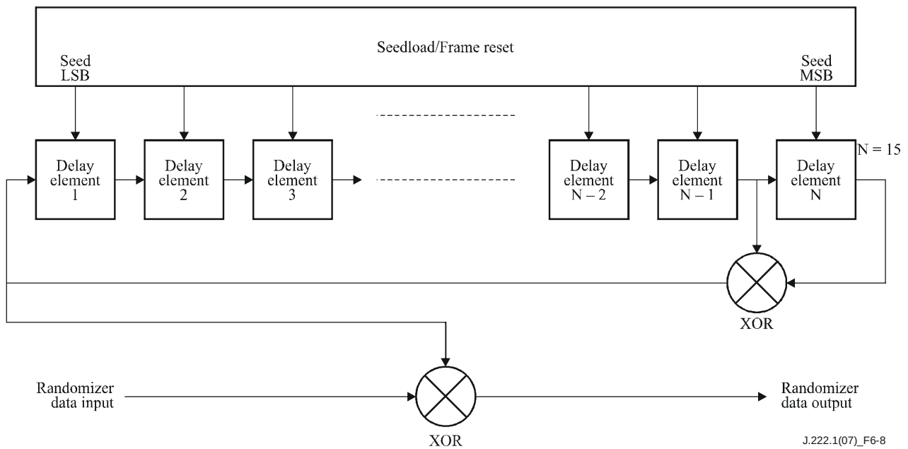
Figure 6-8 – Scrambler structure
