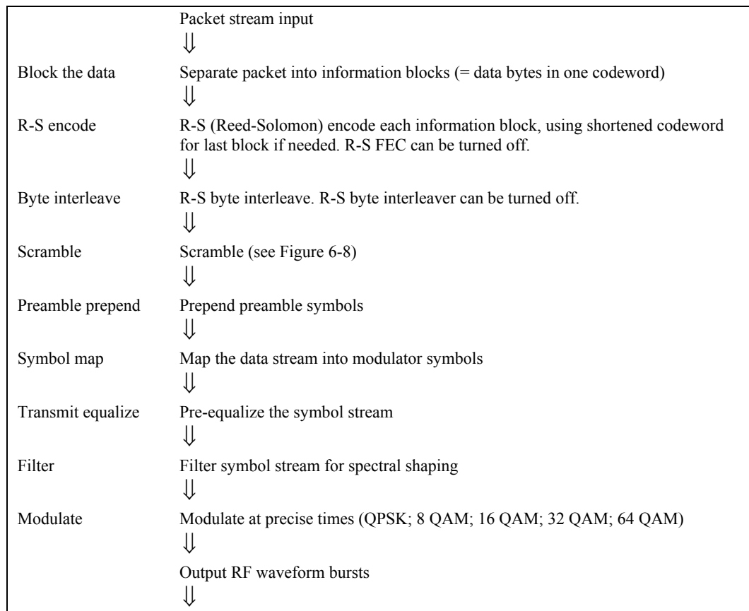
Figure 6-2 – TDMA upstream transmission processing
