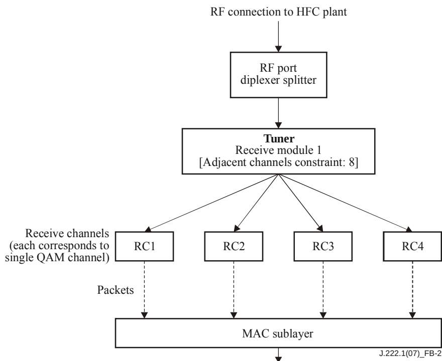
Figure B.2 – 8 MHz DOCSIS standard receive channel profile 01
