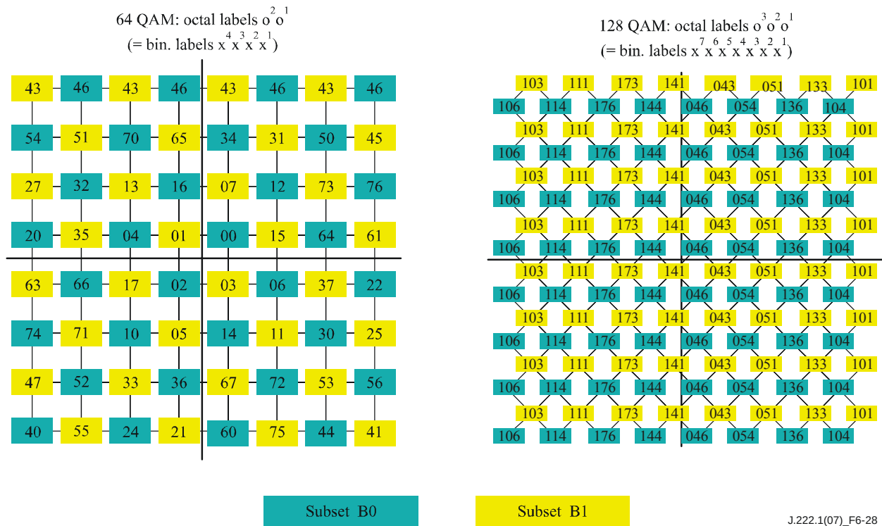
Figure 6-28 – 64 QAM and 128 QAM TCM symbol mapping
