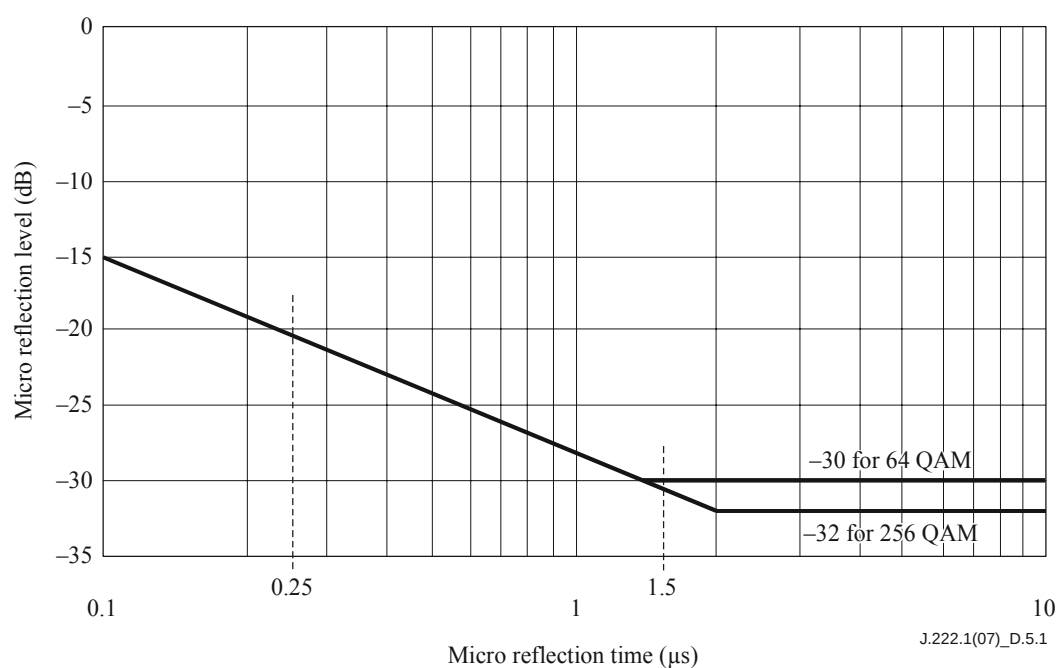
Figure D.1– Micro reflections bound for dominant echo
