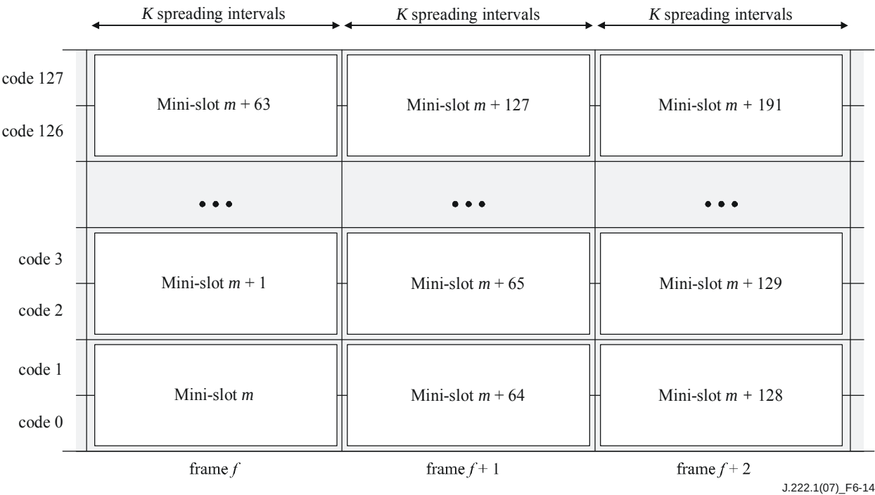
Figure 6-14 – Mini-slot mapping with two codes per mini-slot, 128 active codes
