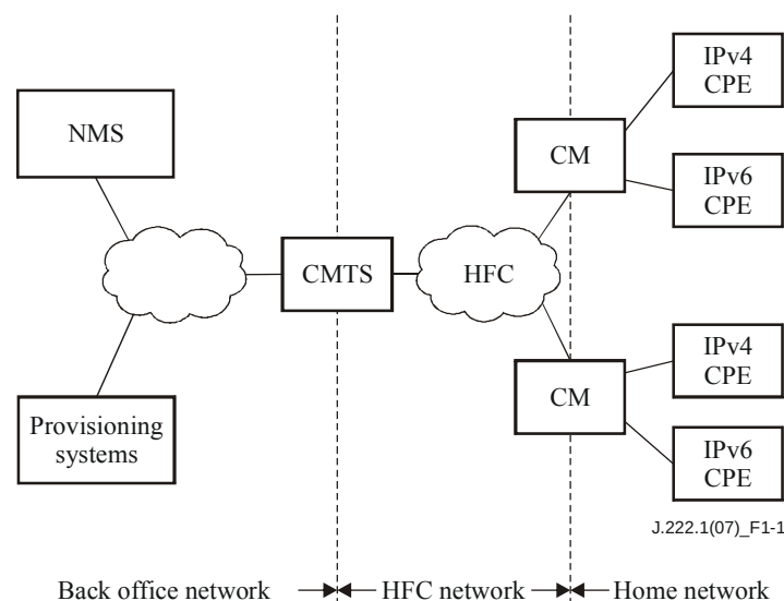
Figure 1-1 – The DOCSIS network
