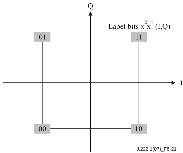
Figure 6-21 – QPSK gray and differential symbol mapping
