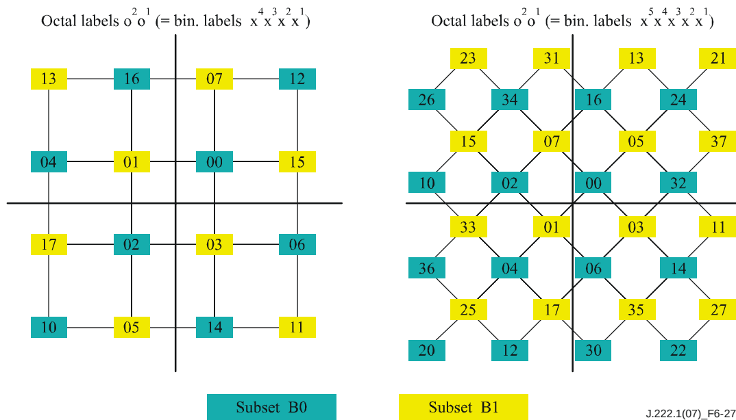
Figure 6-27 – 16 QAM and 32 QAM TCM symbol mapping
