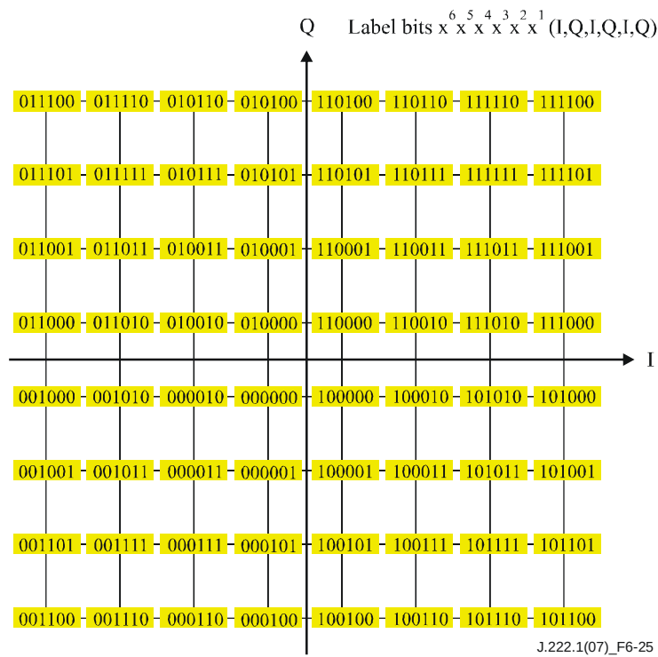
Figure 6-25 – 64 QAM symbol mapping
