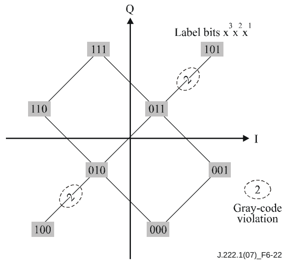
Figure 6-22 – 8 QAM symbol mapping
