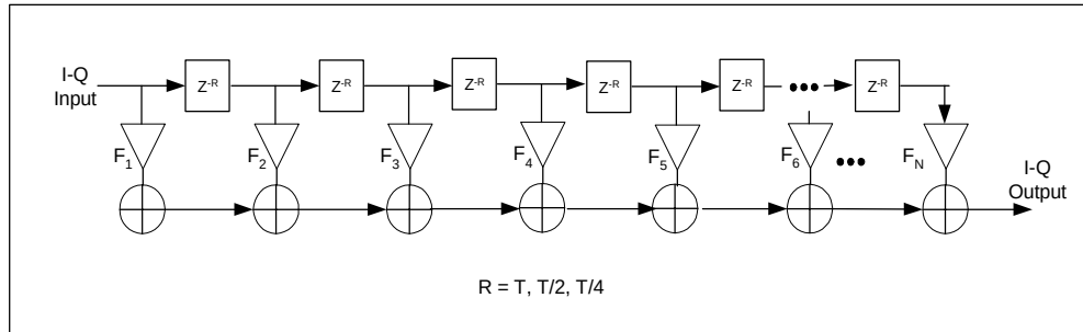
Figure 4-5. Transmit Pre-Equalizer Structure
