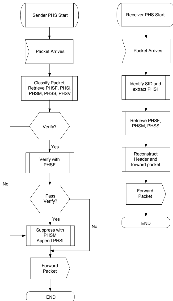
Figure 10–11 Payload Header Suppression Operation
