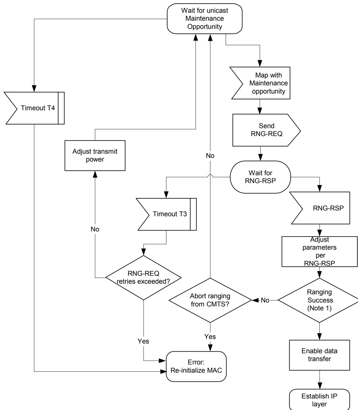
Figure 11-7 Unicast Initial Ranging - CM
