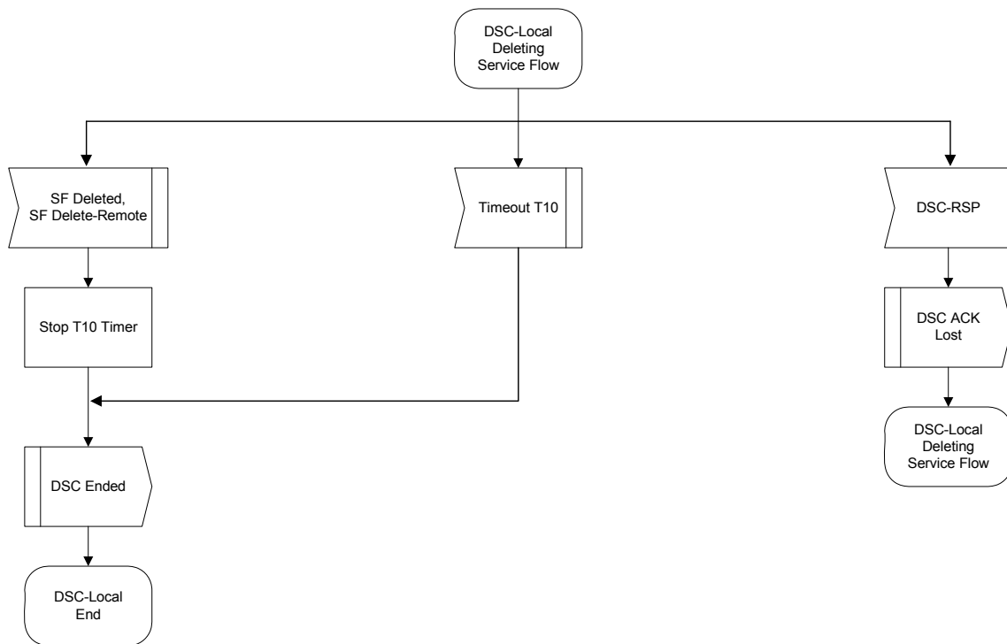
Figure 11–46 DSC—Locally Initiated Transaction Deleting Service Flow State Flow Diagram
