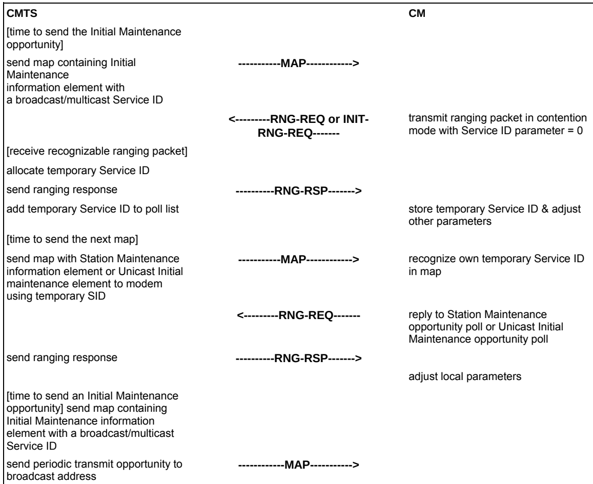
Figure 11–5 Ranging and Automatic Adjustments Procedure
