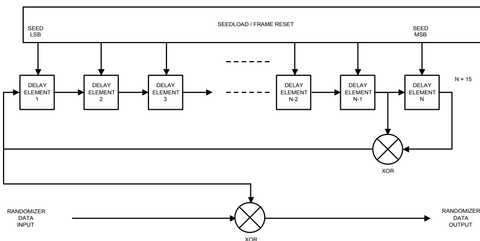
Figure 6–7 Scrambler Structure
