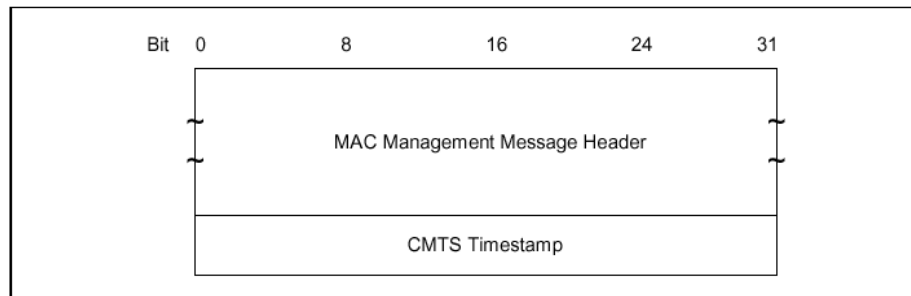
Figure F-3 Format of Packet PDU Following the Timing Header
