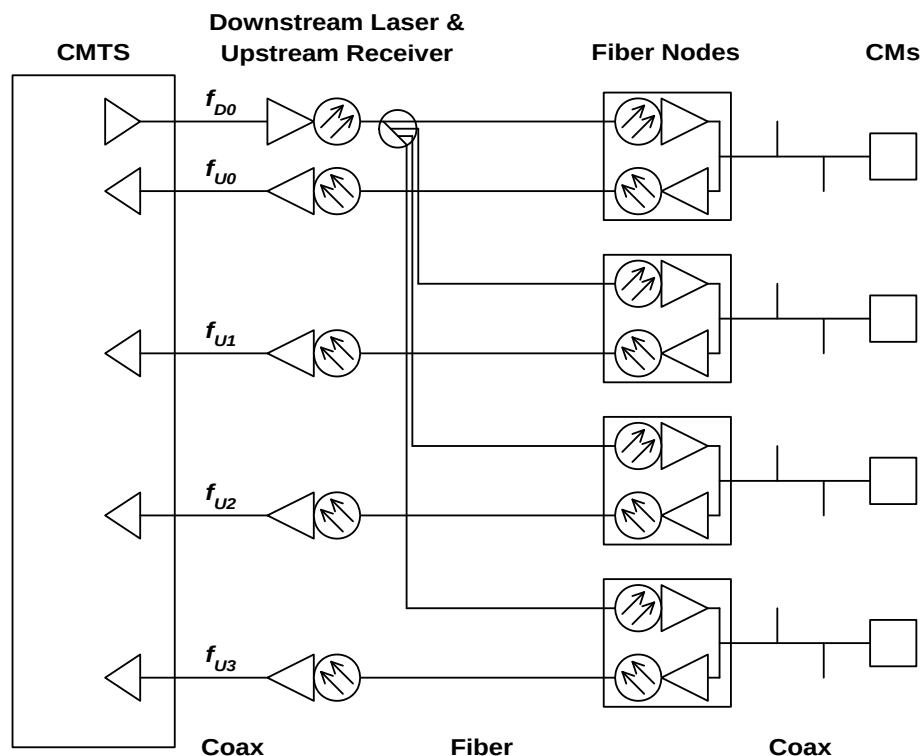
Figure III-1 Single Downstream and Single Upstream Channels per CM
