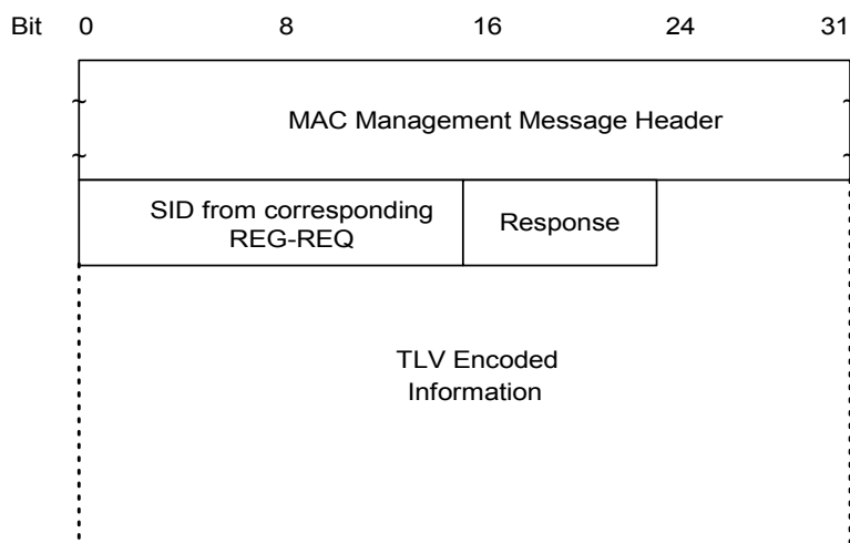
Figure 8-26 Registration Response Format
