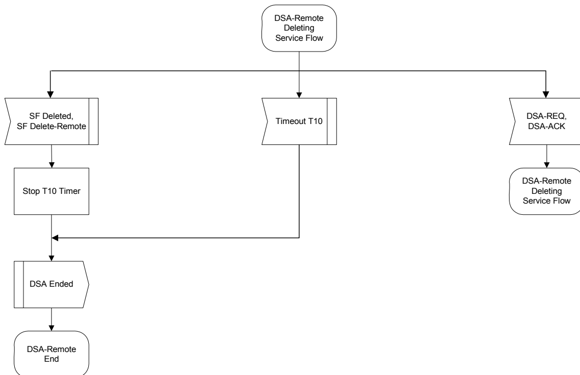
Figure 11–39 DSA—Remotely Initiated Transaction Deleting Service State Flow Diagram
