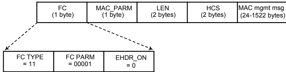
Figure 8–7 Management MAC Header
