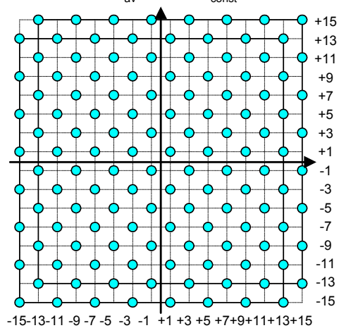
Figure 6–18 Symbol Constellations
