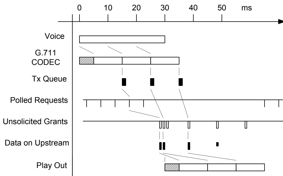
Figure VI-2 VAD Start-Up and Stop
