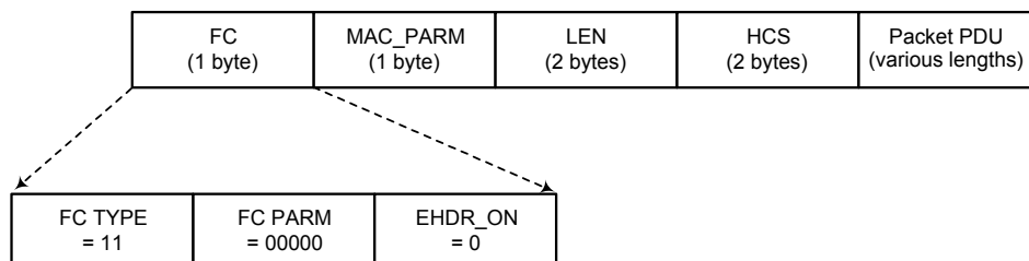
Figure 8–6 Timing MAC Header
