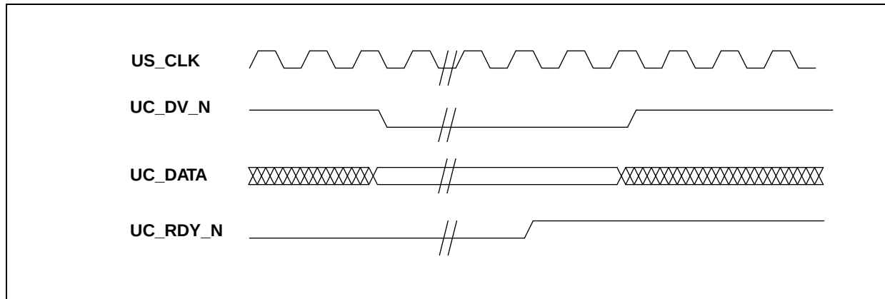
Figure H-6 Upstream Control Message Transfer
