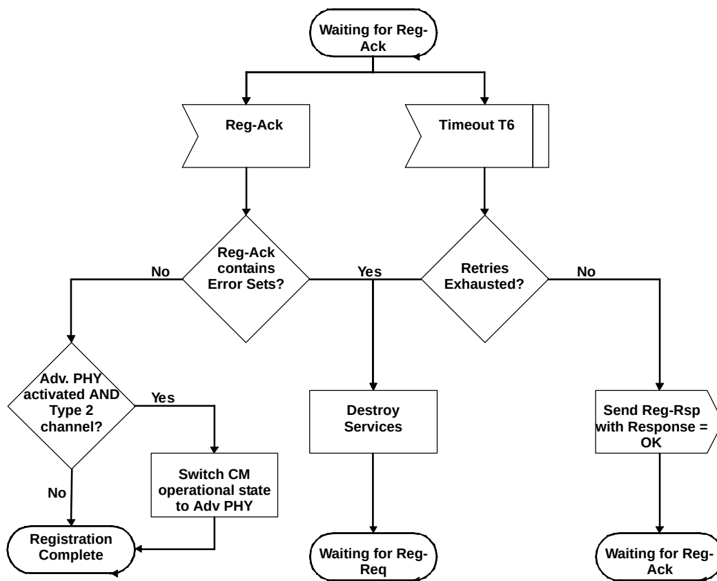
Figure 11–15 Registration Acknowledgment — CMTS 127
