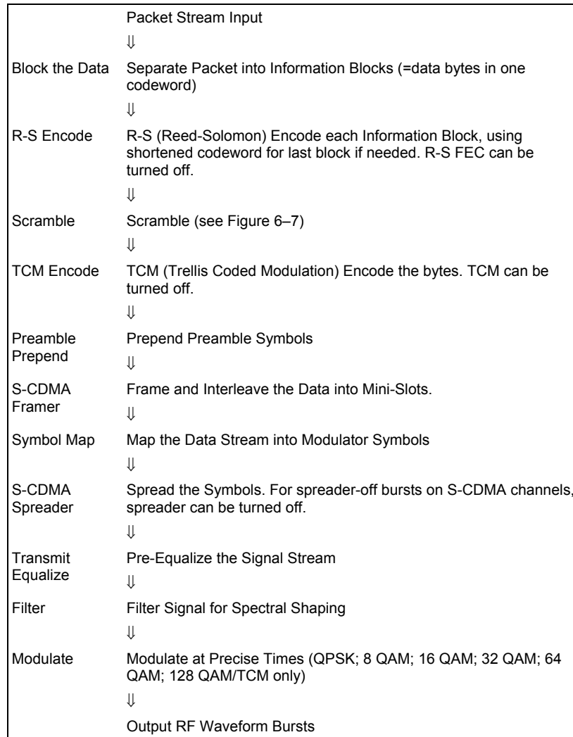
Figure 6–3 S-CDMA Upstream Transmission Processing
