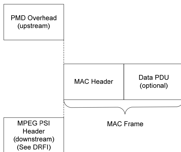
Figure 8–1 Generic MAC Frame Format
