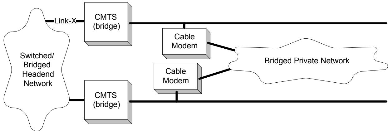
Figure E-2 Spanning Tree Across CMTSes
