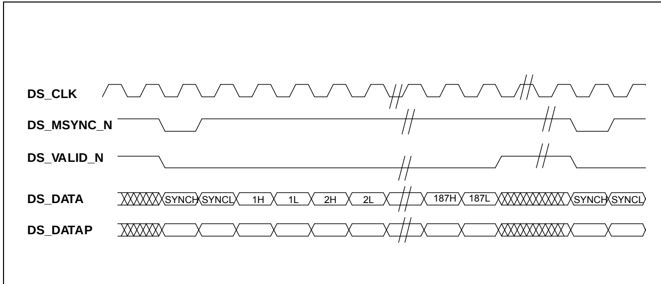
Figure H-2 Downstream Data Signal Protocol for ITU-T Recommendations J.83 Annex A Operation
