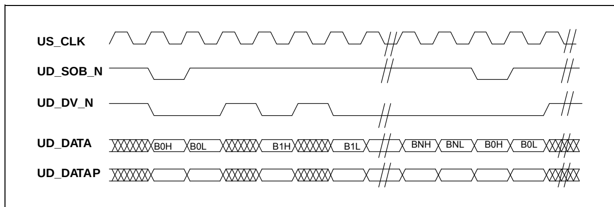
Figure H–4 Upstream Data Protocol
