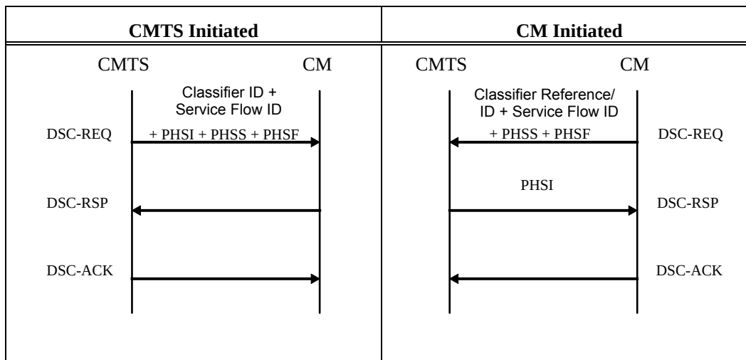
Figure 10–13 Payload Header Suppression Signaling Example
