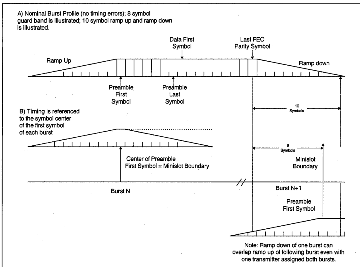
Figure 6–29 Nominal TDMA Burst Timing
