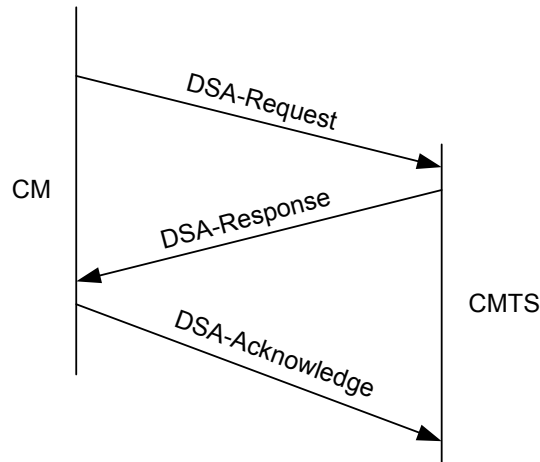
Figure 10–6 Dynamic Service Addition Message Flow — CM Initiated
