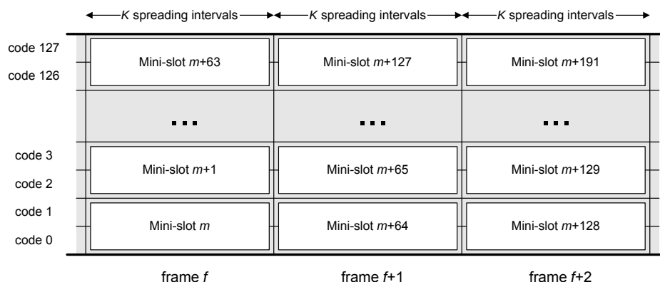
Figure 6–13 Mini-slot Mapping with Two Codes per Mini-slot, 128 Active Codes
