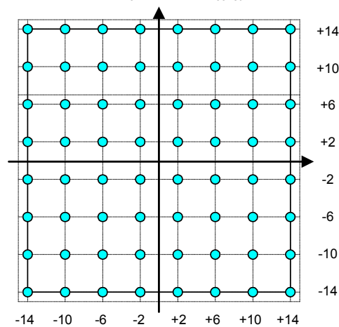
Figure 6–18 Symbol Constellations
