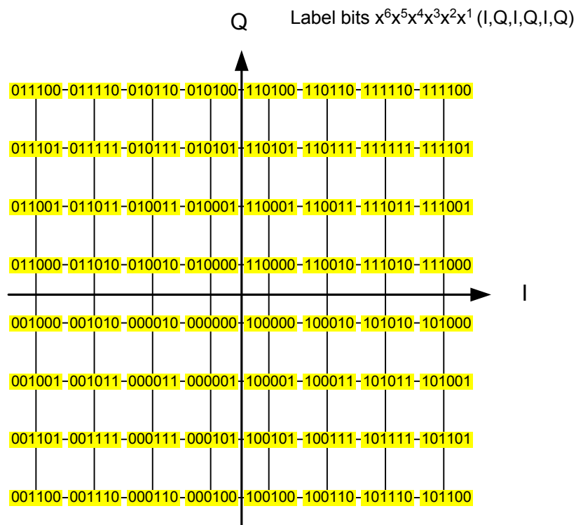
Figure 6-23 64QAM Symbol Mapping
