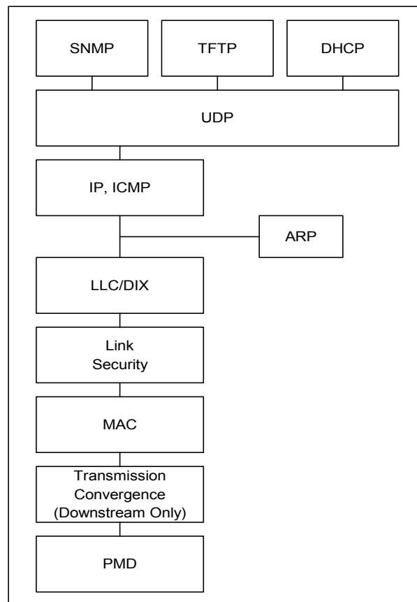
Figure 5–1 Protocol Stack on the RF Interface
