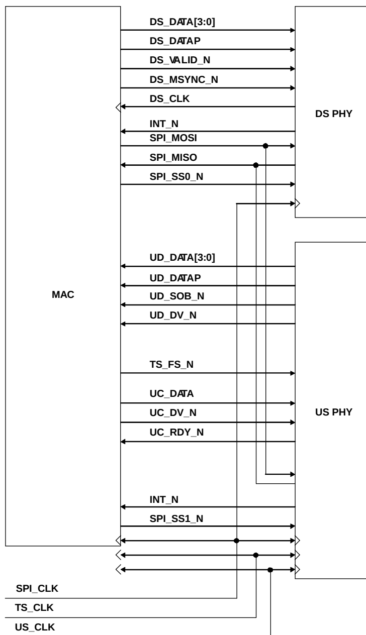
Figure H–1 DMPI Application
