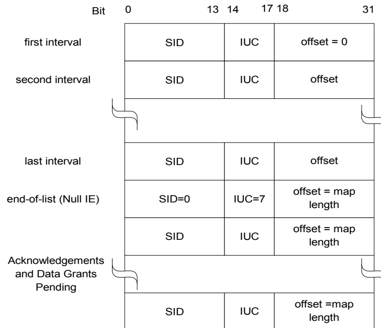
Figure 8–20 MAP Information Element Structure
