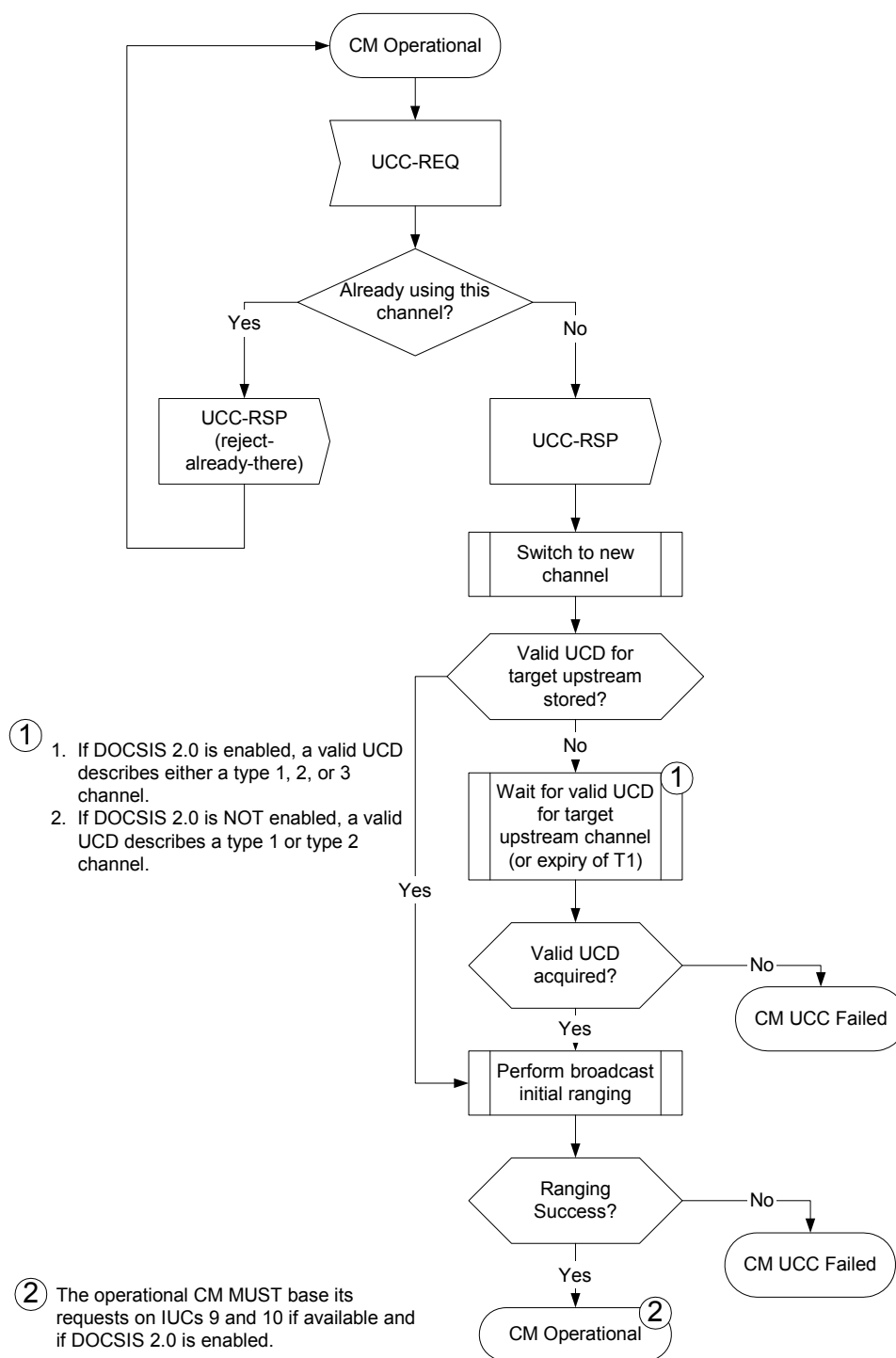
Figure 11–19 Changing Upstream Channels: CM View Part 1
