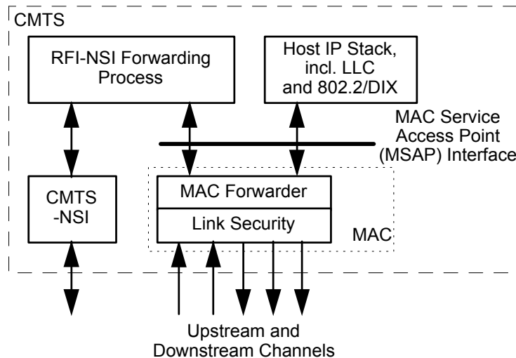
Figure 5–4 MAC Forwarder
