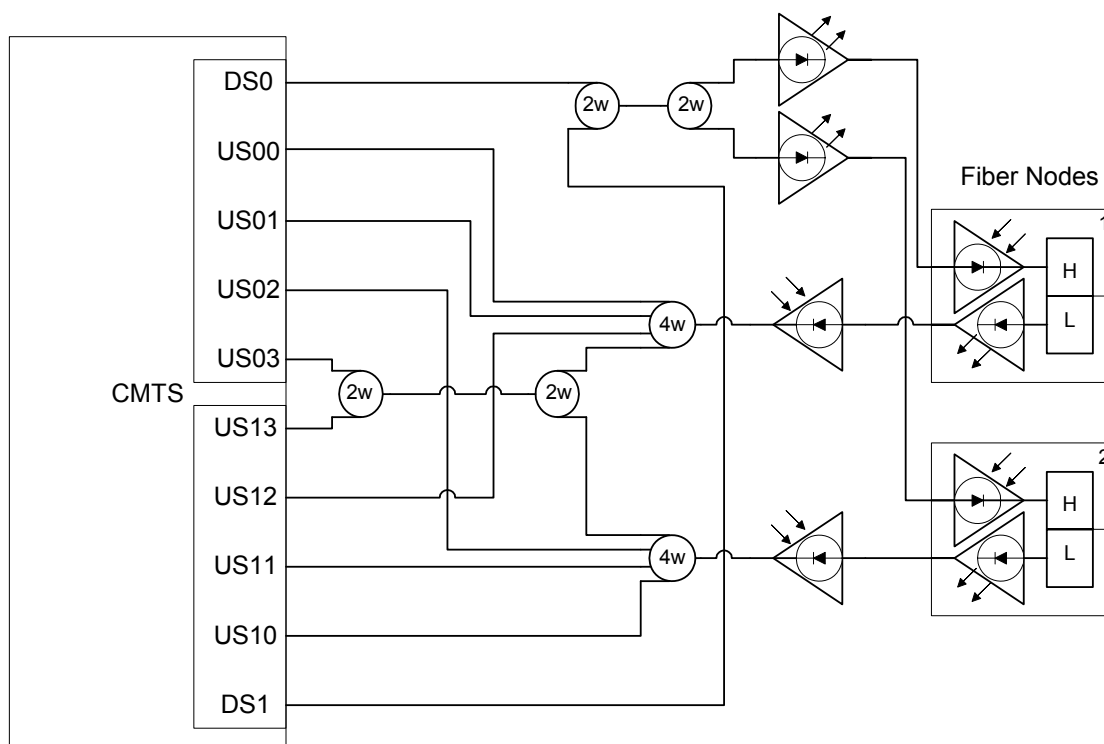
Figure 11-68 Example Combining Network 2
