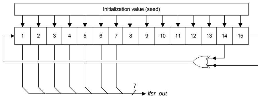
Figure 6-27 Code Hopping Random Number Generator
