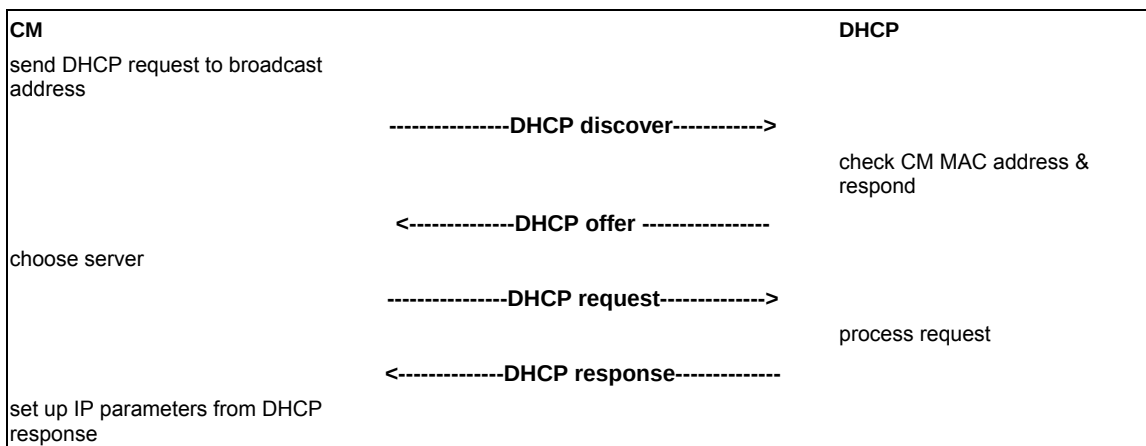
Figure 11–10 Establishing IP Connectivity
