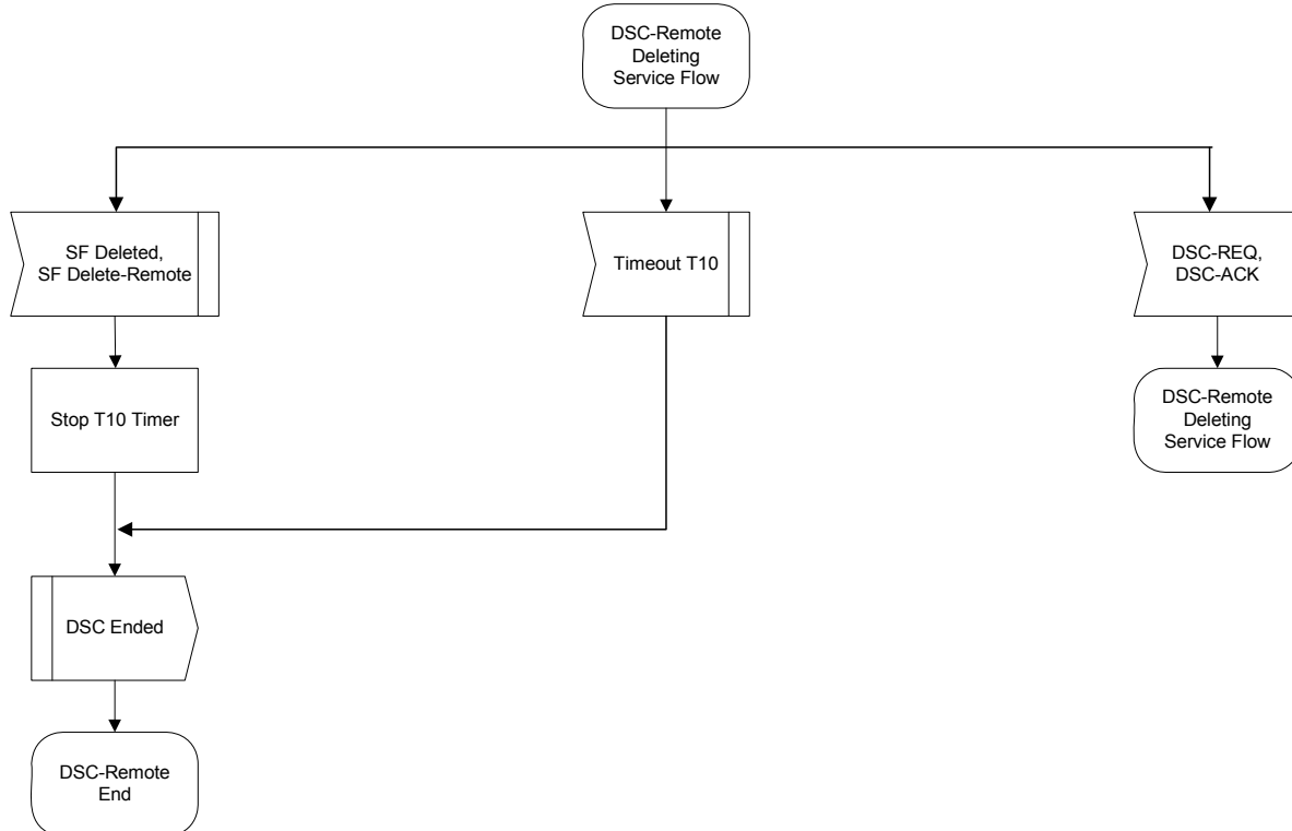
Figure 11-50 DSC—Remotely Initiated Transaction Deleting Service Flow State Flow Diagram
