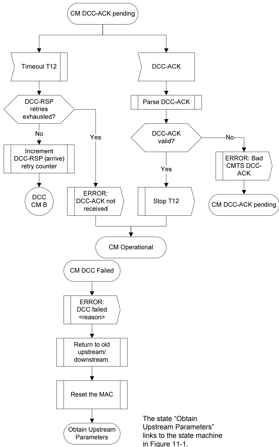
Figure 11–65 Dynamically Changing Channels: CM View Part 4
