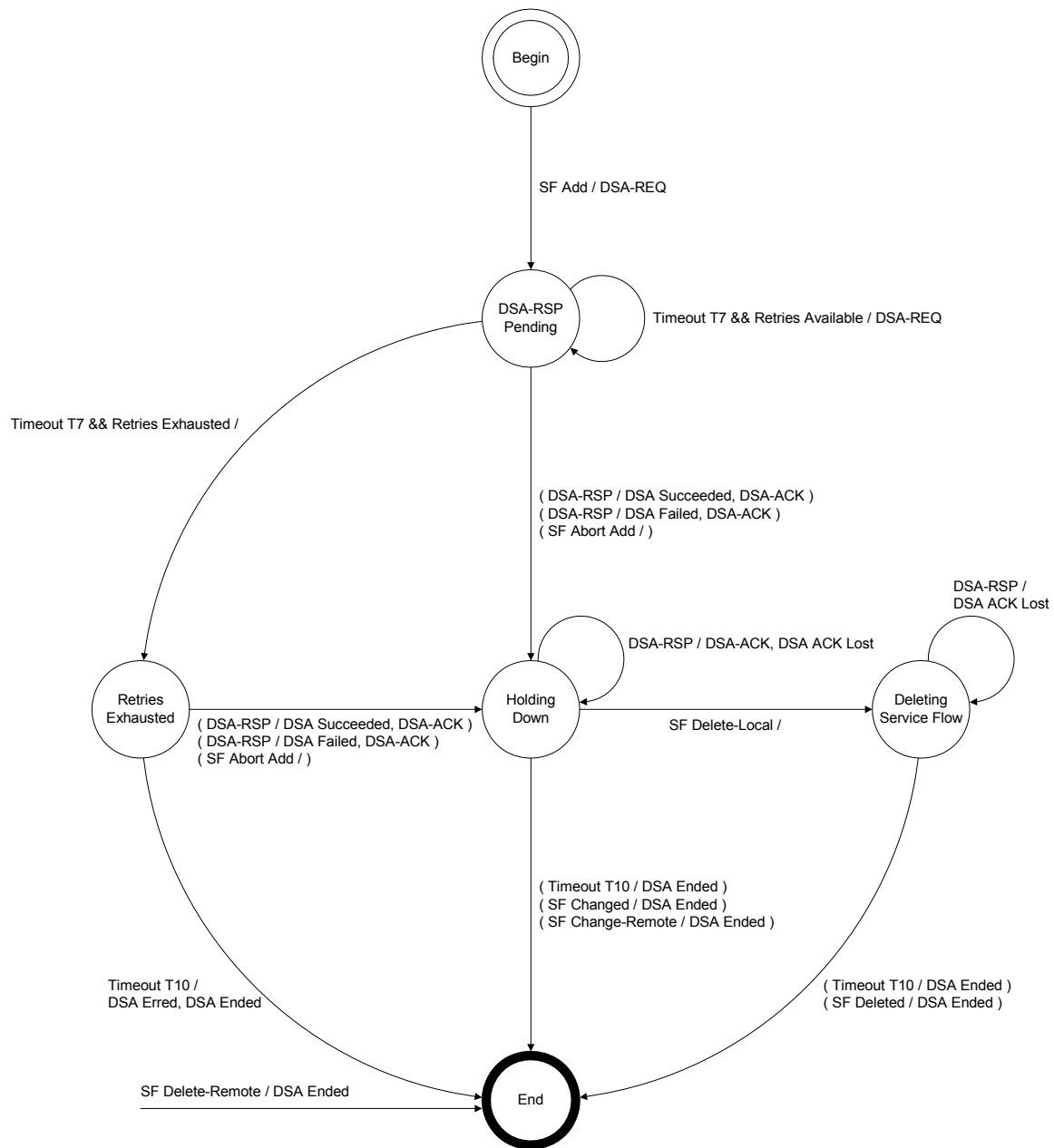
Figure 11–23 DSA—Locally Initiated Transaction State Transition Diagram
