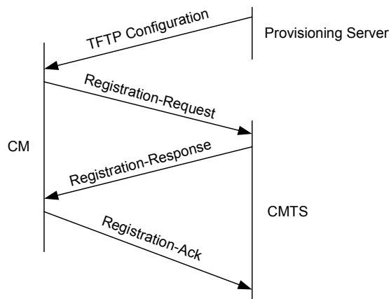
Figure 10–5 Registration Message Flow
