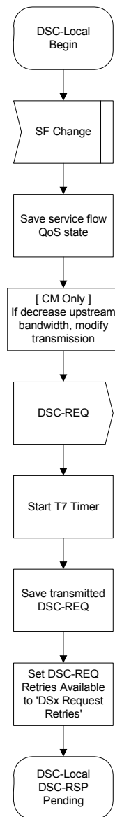
Figure 11-42 DSC—Locally Initiated Transaction Begin State Flow Diagram
