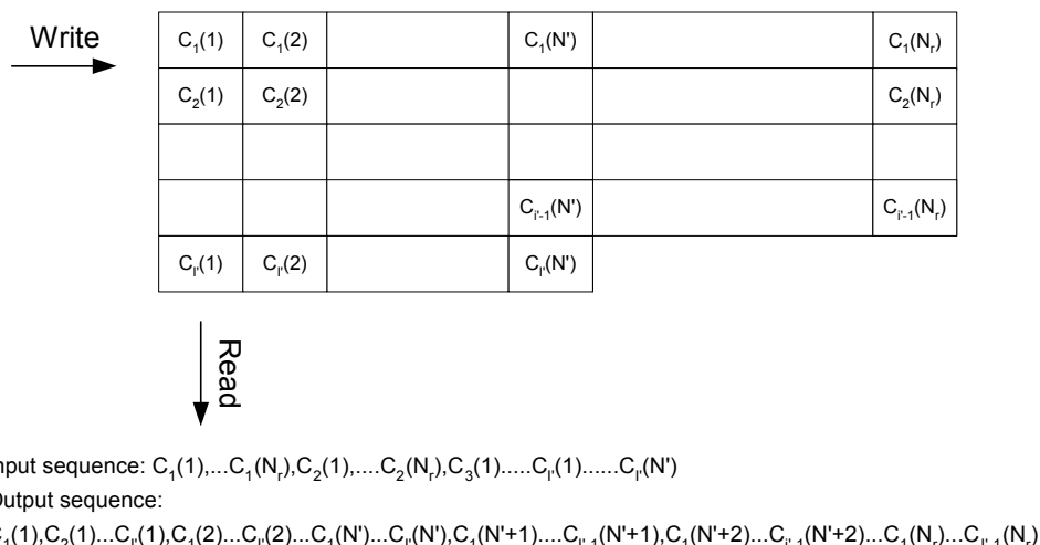
Figure 6–6 Interleaver operation for last interleaver block (with shortened last codeword)
