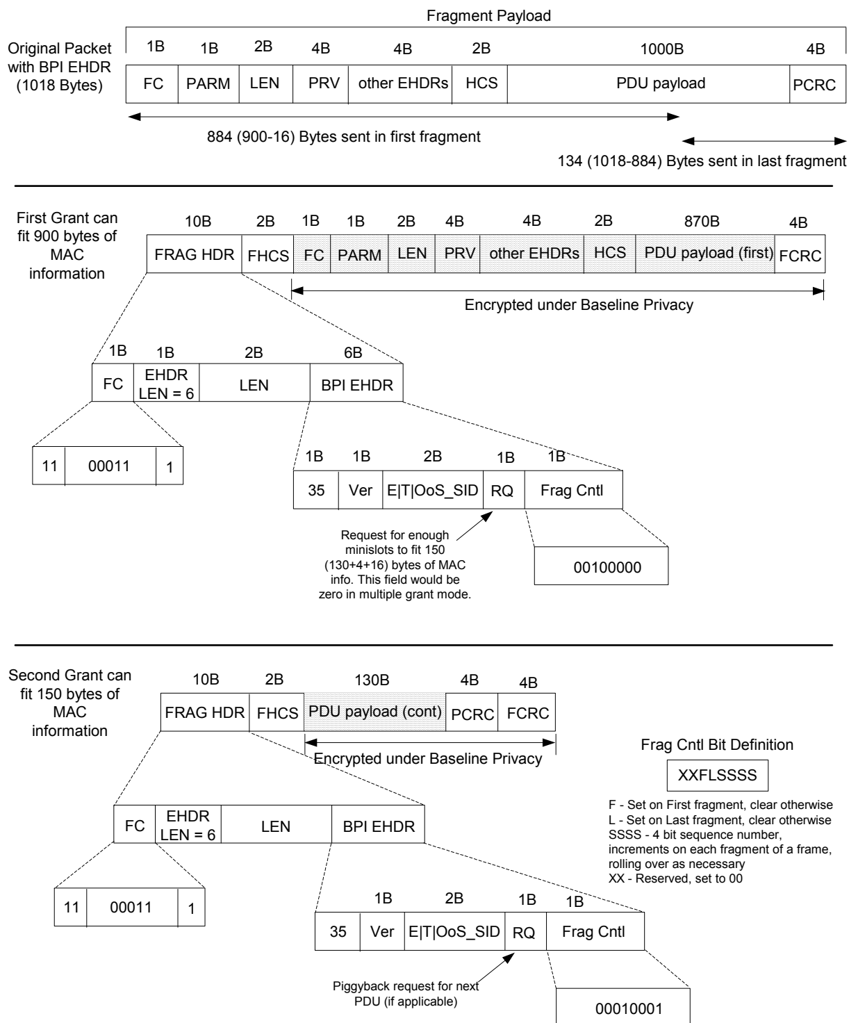
Figure 10-9 Example of Fragmenting a Single Packet
