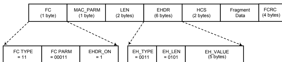
Figure 8–9 Fragmentation MAC Header Format
