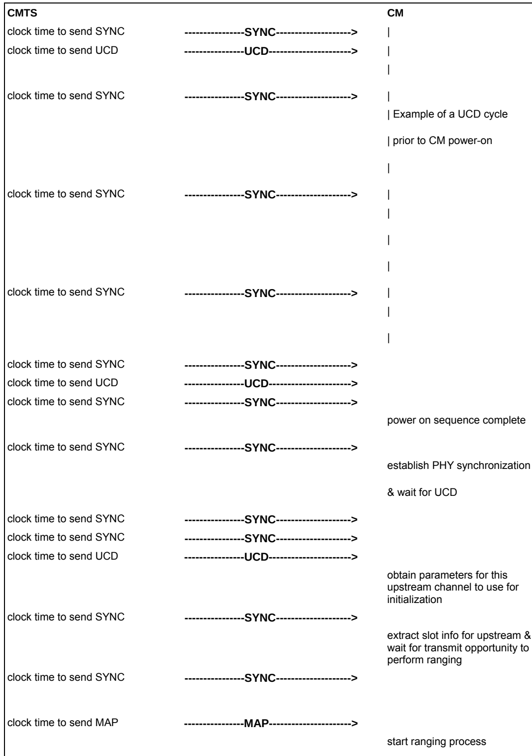
Figure 11–4 Message Flows During Scanning and Upstream Parameter Acquisition
