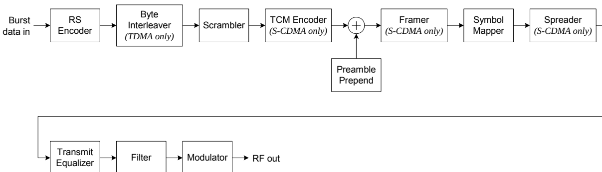
Figure 6-1 Upstream signal-processing sequence
