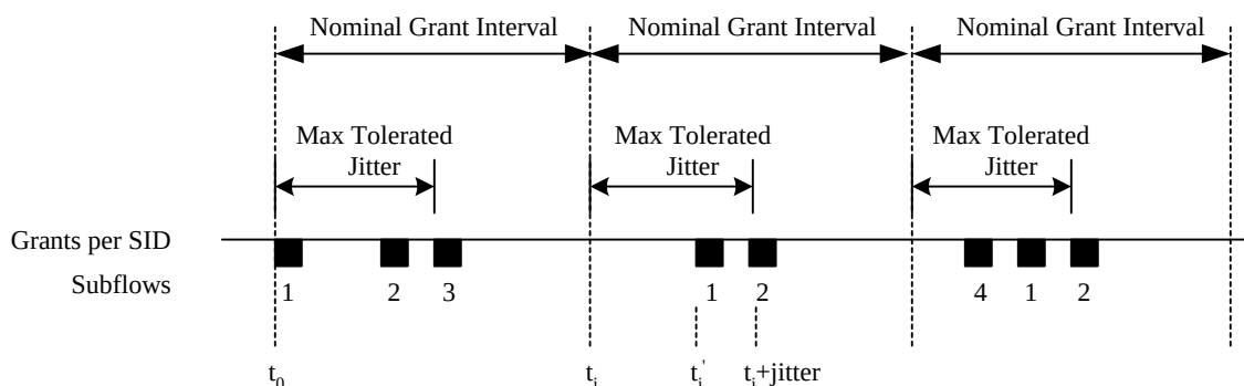
Figure VI–1 Example Jitter with Multiple Grants per SID
