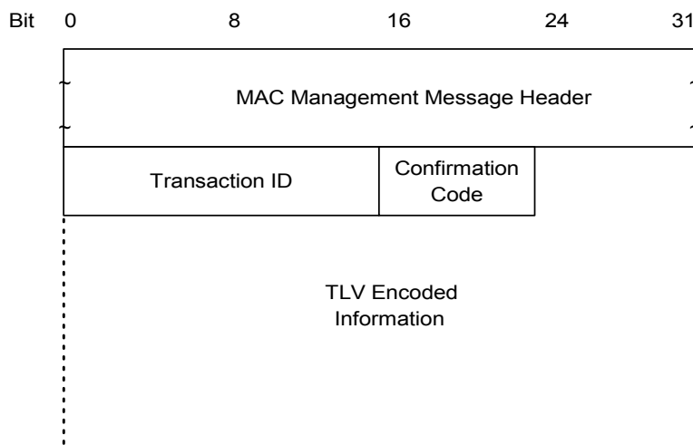
Figure 8–32 Dynamic Service Addition — Acknowledge
