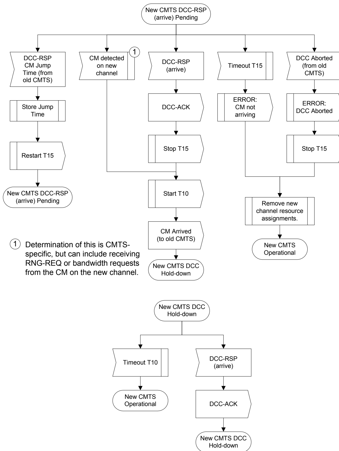
Figure 11–61 Dynamically Changing Channels: CMTS View Part 4
