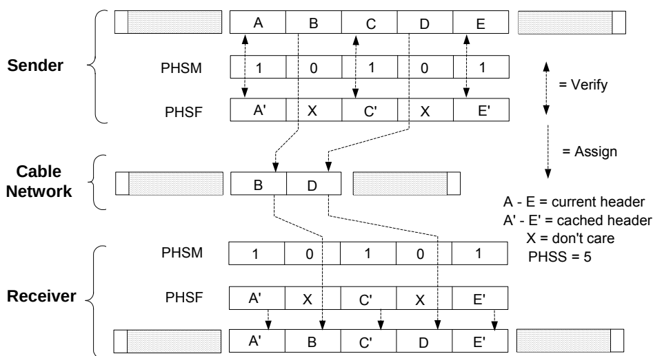
Figure 10–12 Payload Header Suppression with Masking
