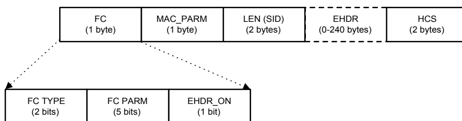
Figure 8–3 MAC Header Format
