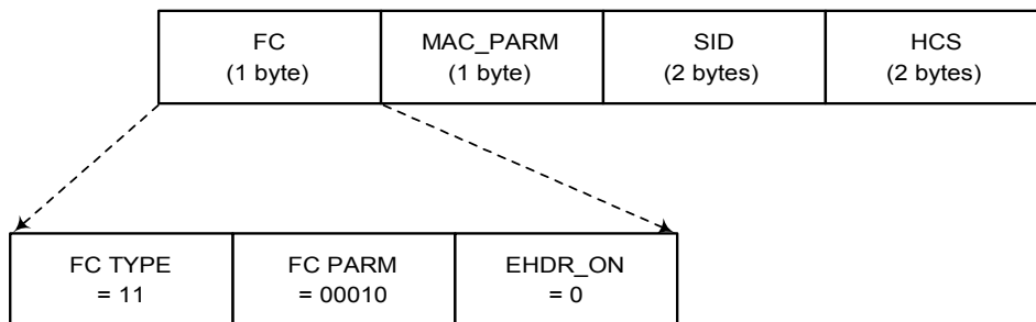
Figure 8–8 Request Frame Format
