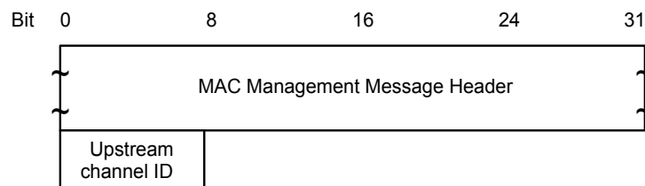
Figure 8-29 Upstream Channel Change Response
