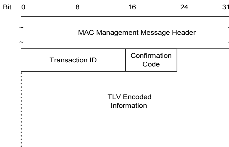
Figure 8–35 Dynamic Service Change — Acknowledge
