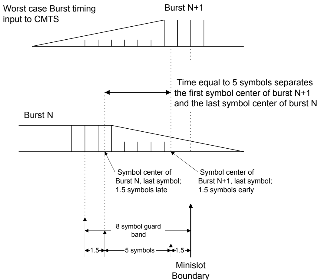
Figure 6–30 Worst-Case TDMA Burst Timing
