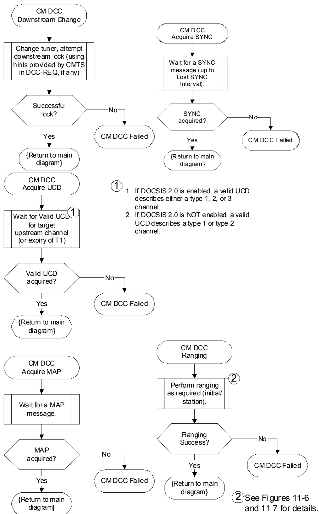
Figure 11-64 Dynamically Changing Channels: CM View Part 3
