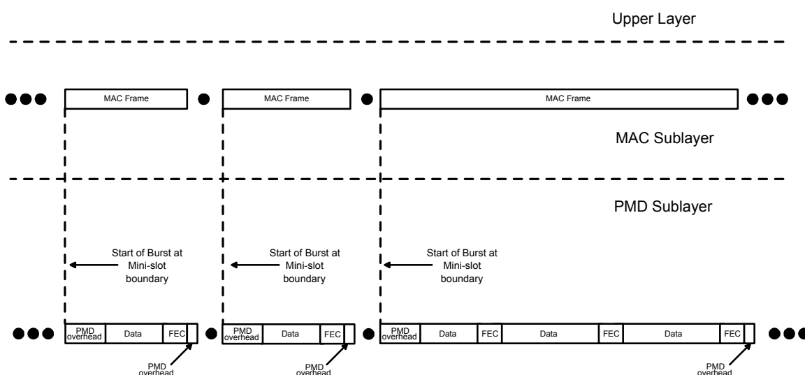
Figure 8–2 Upstream MAC/PMD Convergence
