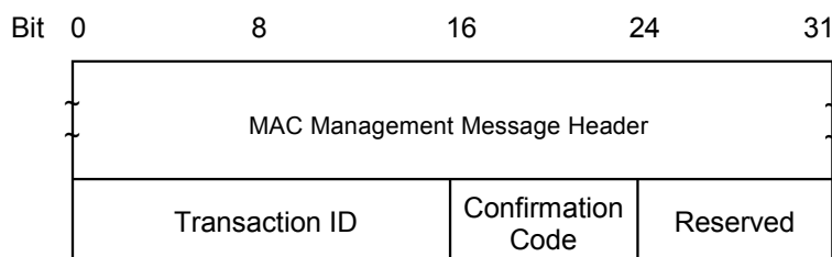
Figure 8–37 Dynamic Service Deletion — Response
