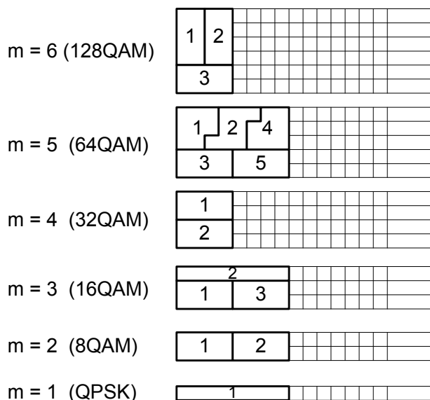
Figure 6–9 Repetitive patterns of byte mapping to symbol map bits for TCM
