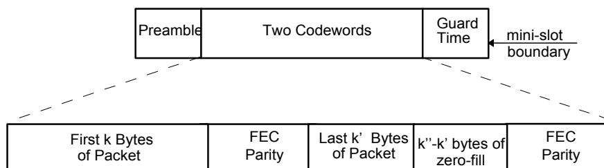
Figure 6-4 Example Frame Structures with Flexible Burst Length Mode
