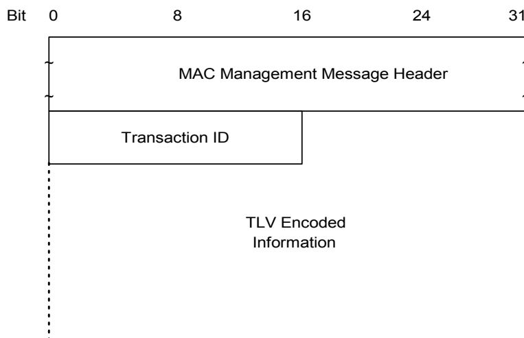
Figure 8–33 Dynamic Service Change — Request
