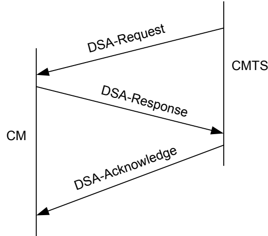
Figure 10–7 Dynamic Service Addition Message Flow — CMTS Initiated
