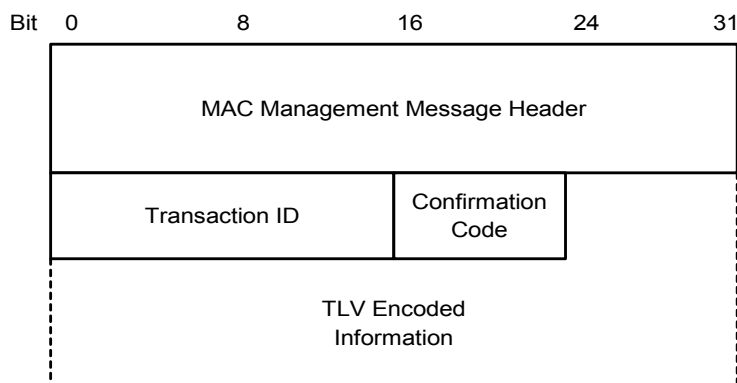
Figure 8–39 Dynamic Channel Change Response
