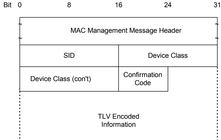
Figure 8–42 Device Class Identification Response
