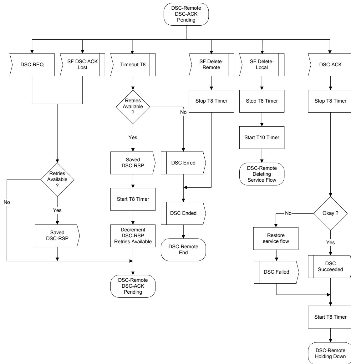
Figure 11-48 DSC—Remotely Initiated Transaction DSC-ACK Pending State Flow Diagram 139
