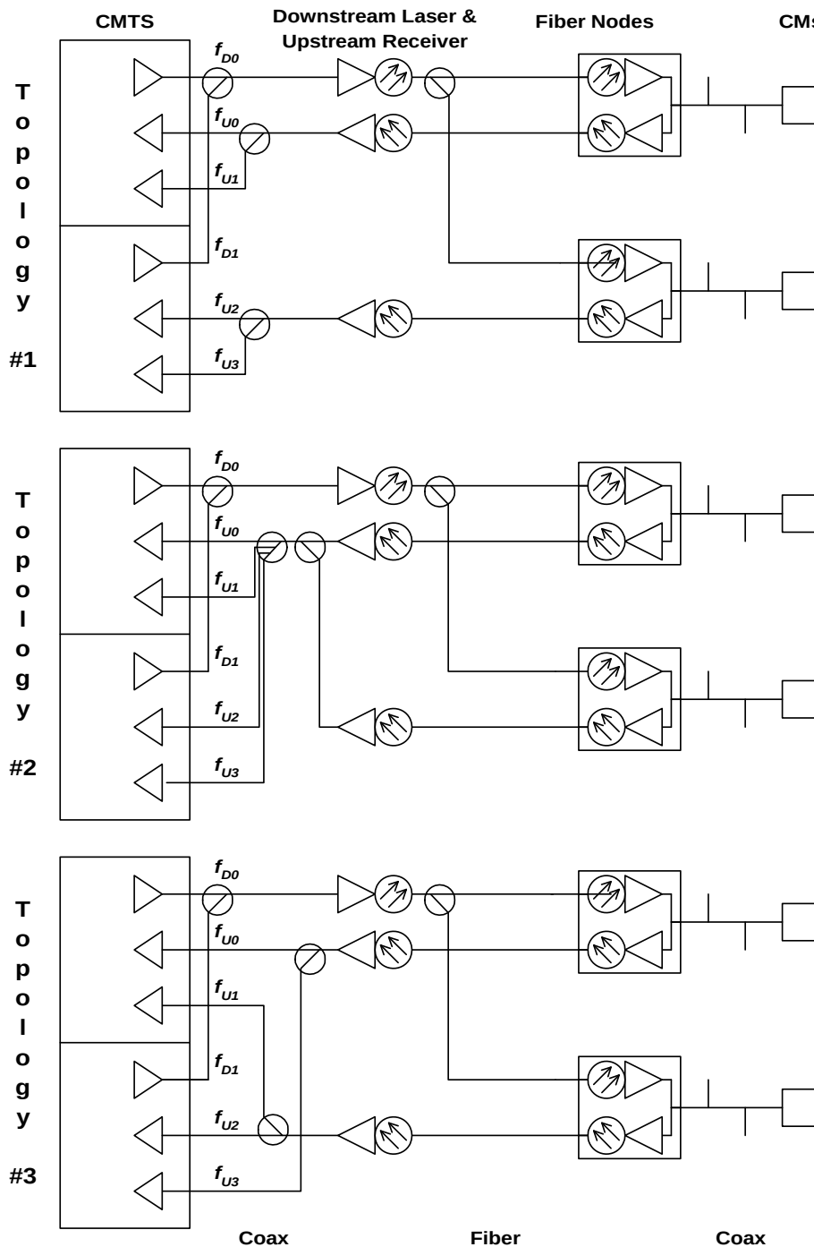
Figure III–2 Multiple Downstream and Multiple Upstream Channels per CM
