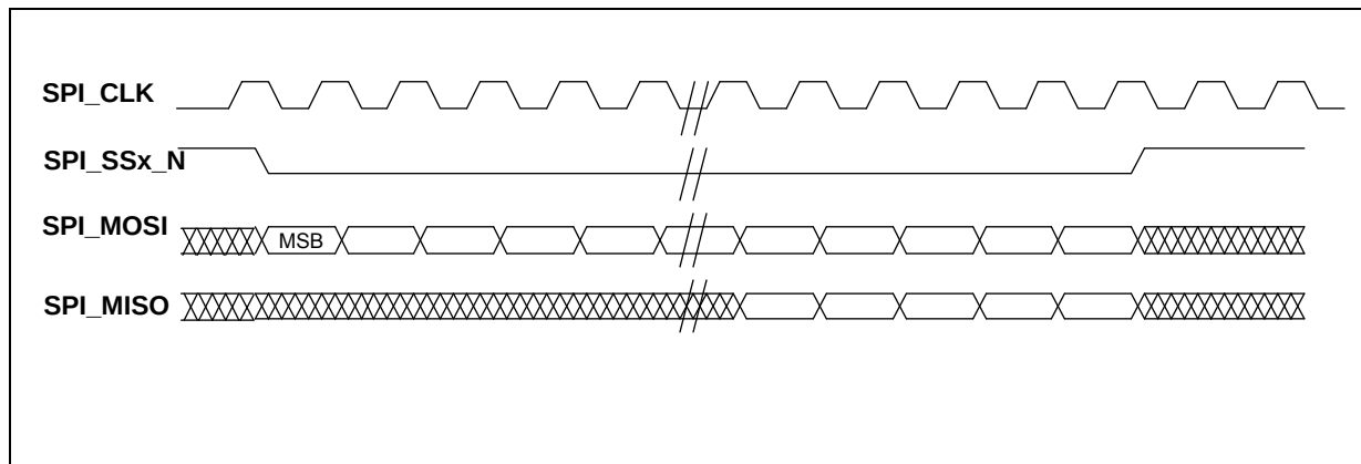
Figure H–7 SPI Bus Transaction
