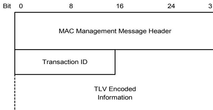
Figure 8–38 Dynamic Channel Change Request
