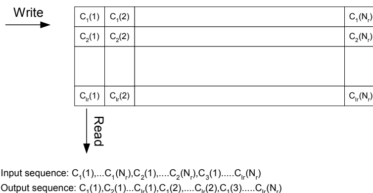
Figure 6–5 Byte Interleaver Operation
