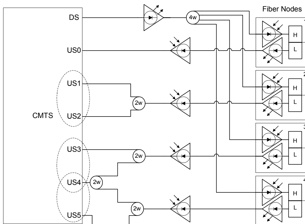
Figure 11–67 Example Combining Network 1
