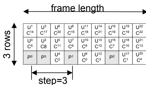
Figure 6-17 Symbol Numbering Without TCM
