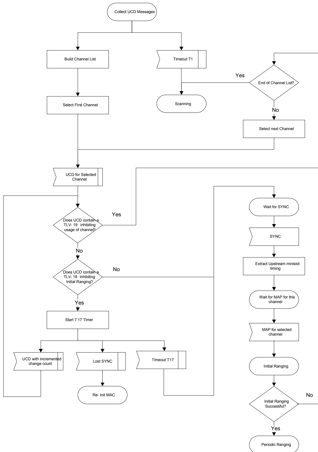
Figure 11–3 Obtaining Upstream Parameters 121
