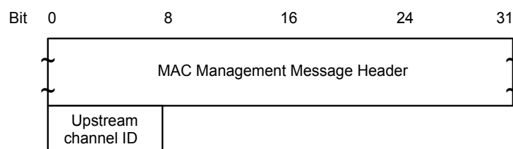
Figure 8–28 Upstream Channel Change Request 82
