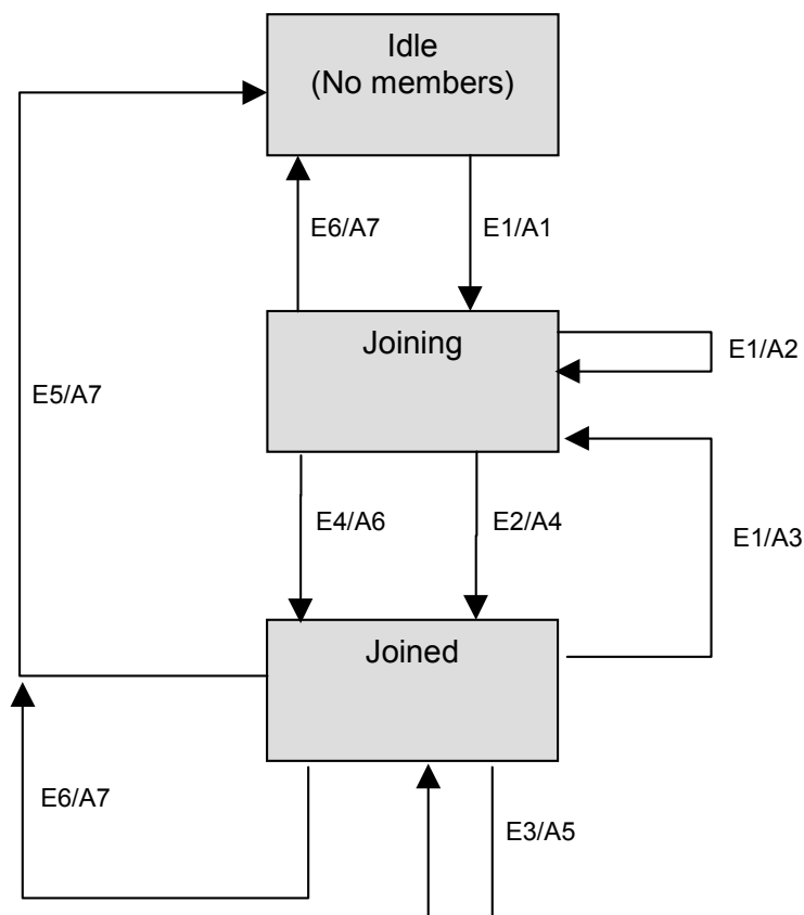
Figure V-1 IGMP Support – CM passive mode
