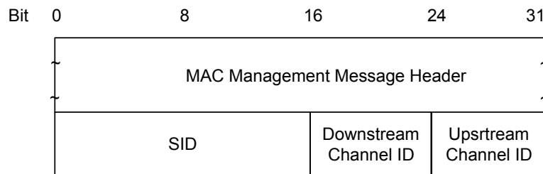
Figure 8–44 Packet PDU Following the Timing Header
