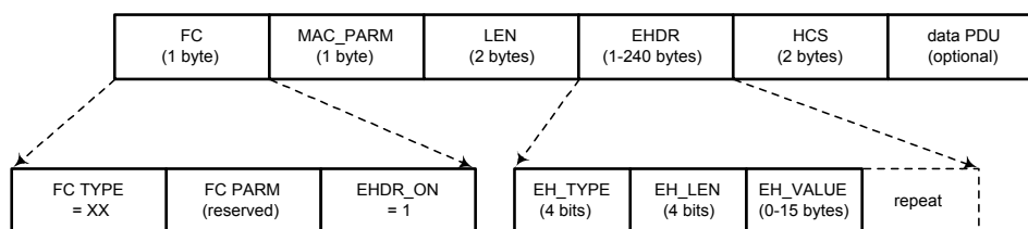
Figure 8–12 Extended MAC Format
