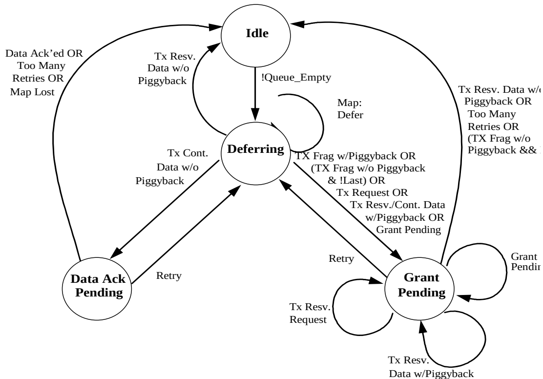
Figure IV-1 Transmission & Deference State Transition Diagram
