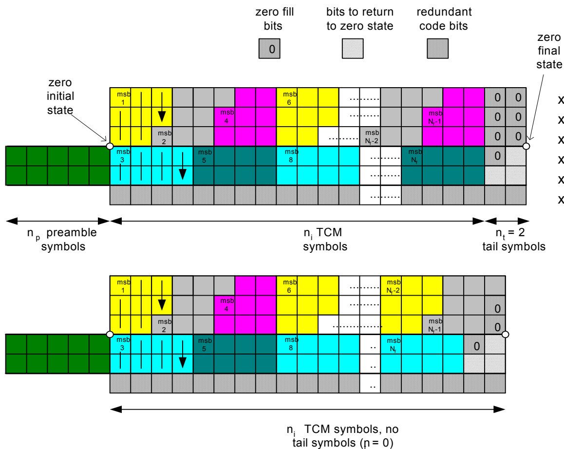
Figure 6-10 Example byte to bit assignment for 64 QAM
