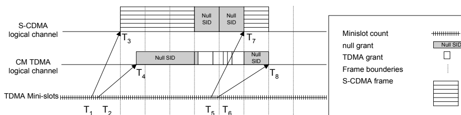
Figure 9-3 Logical S-CDMA TDMA channels
