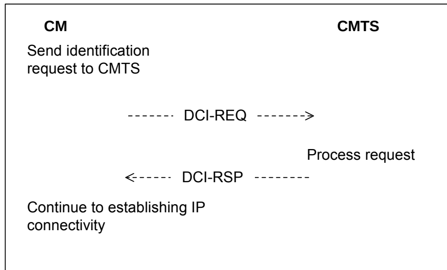
Figure 11–9 Device Class Identification
