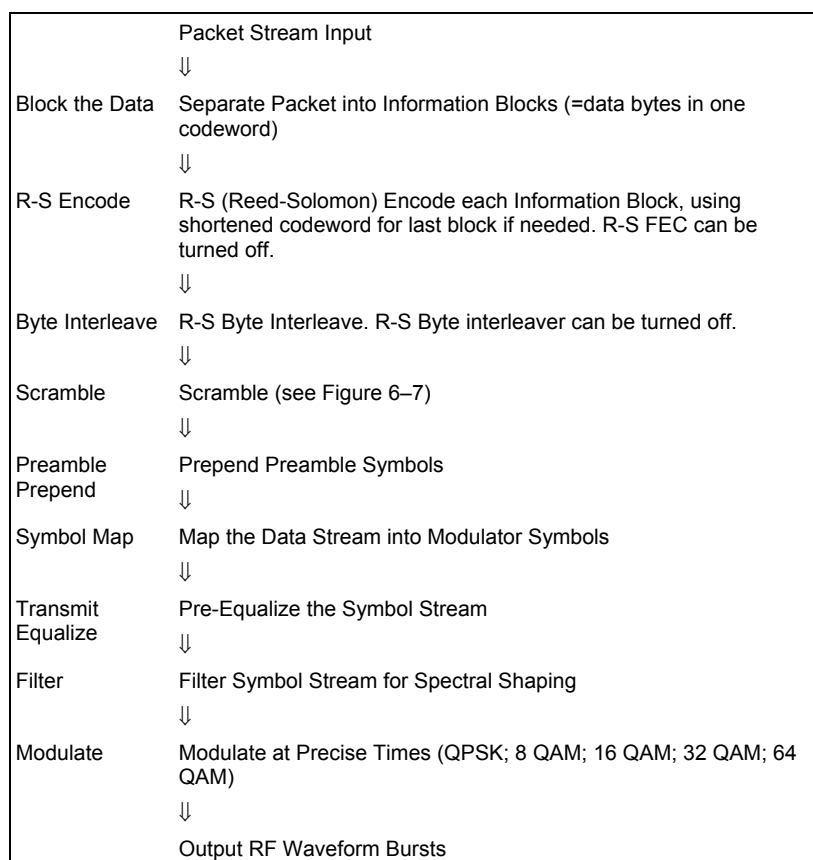
Figure 6-2 TDMA Upstream Transmission Processing
