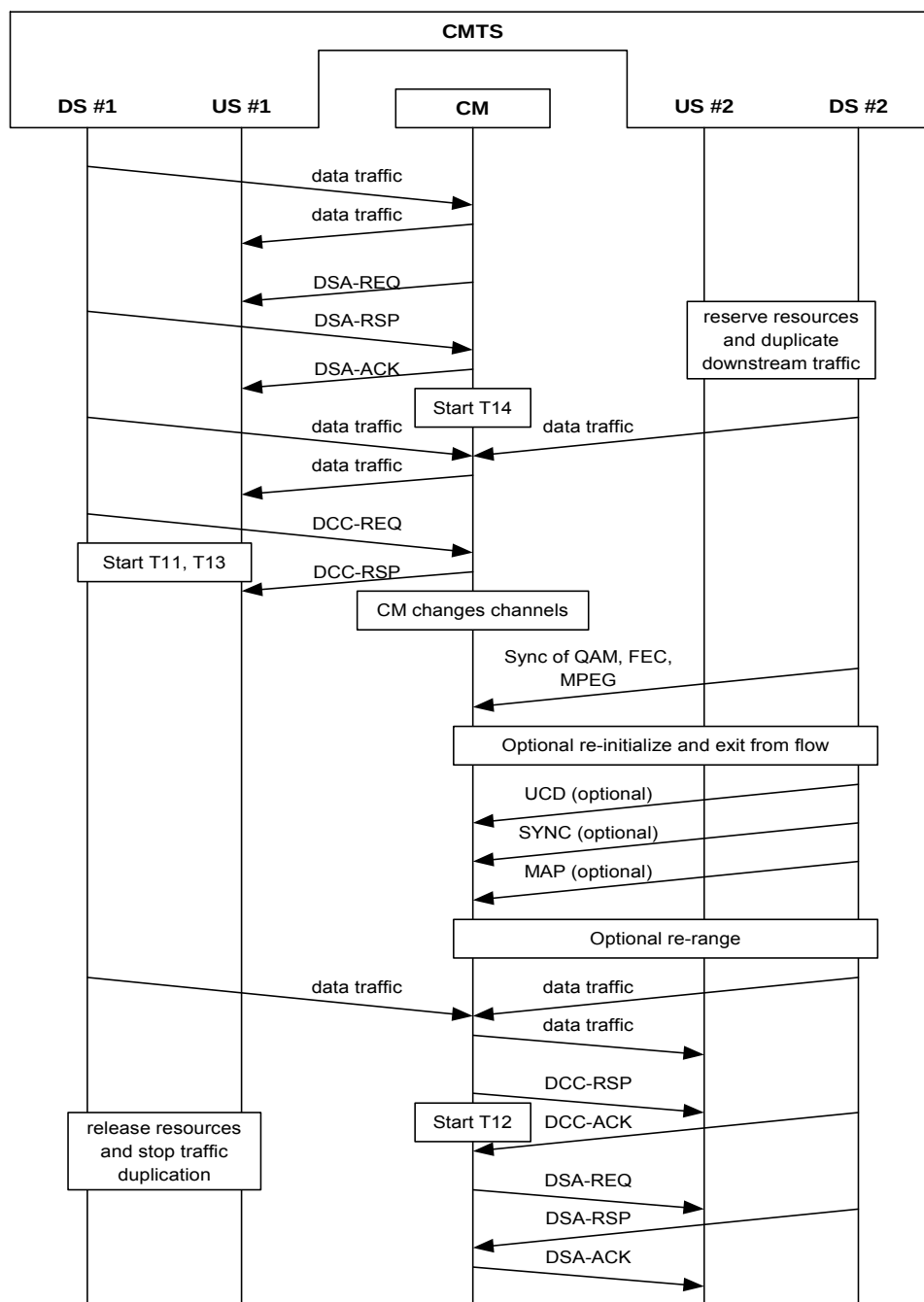
Figure 11–66 DCC Example Operational Flow
