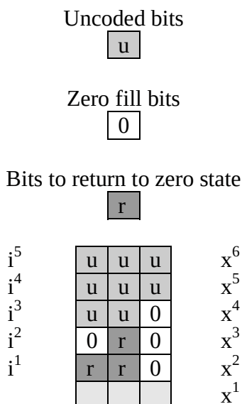
Figure 6–11 Example of return to zero bits followed by “0”
