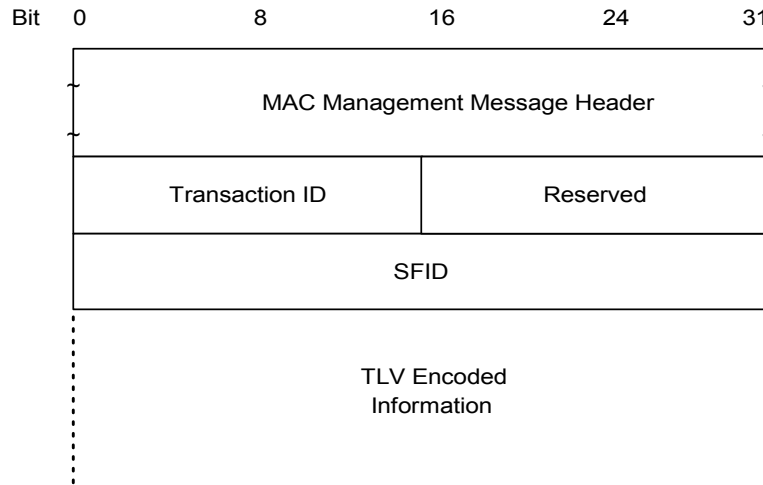
Figure 8–36 Dynamic Service Deletion — Request
