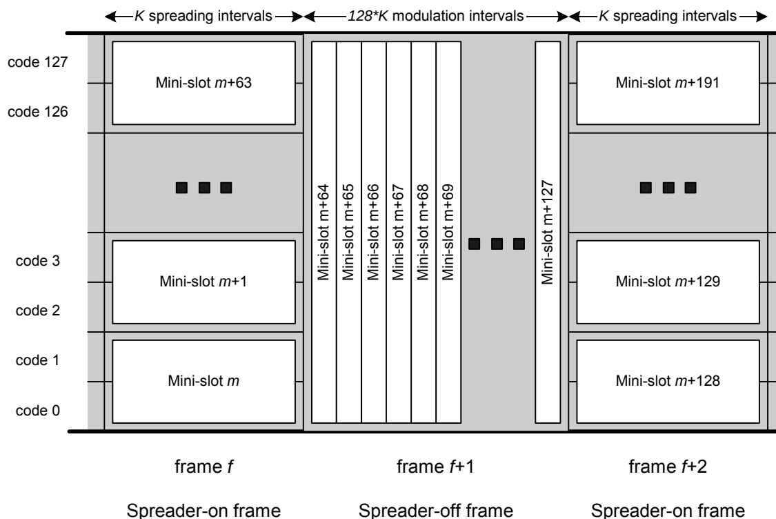
Figure 6-15 S-CDMA and Spreader-off Intervals
