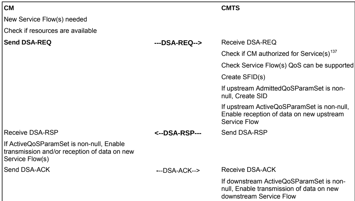
Figure 11–29 Dynamic Service Addition Initiated from CM
