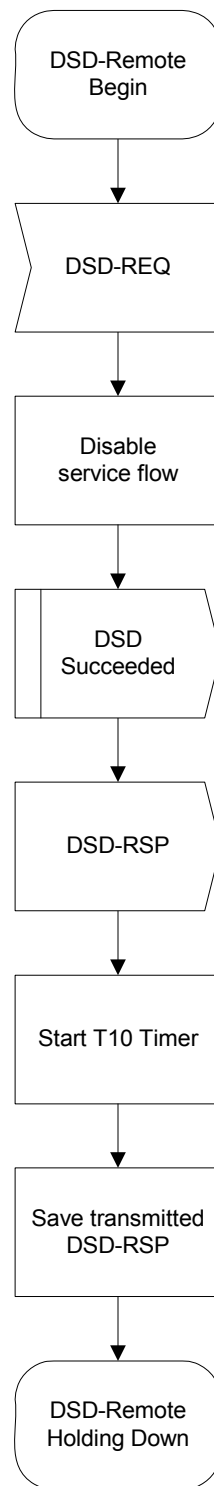
Figure 11–56 DSD—Remotely Initiated Transaction Begin State Flow Diagram
