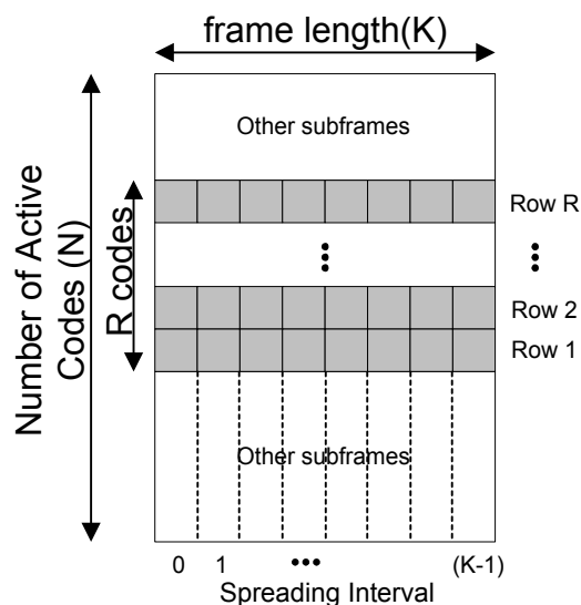
Figure 6–16 Subframe structure
