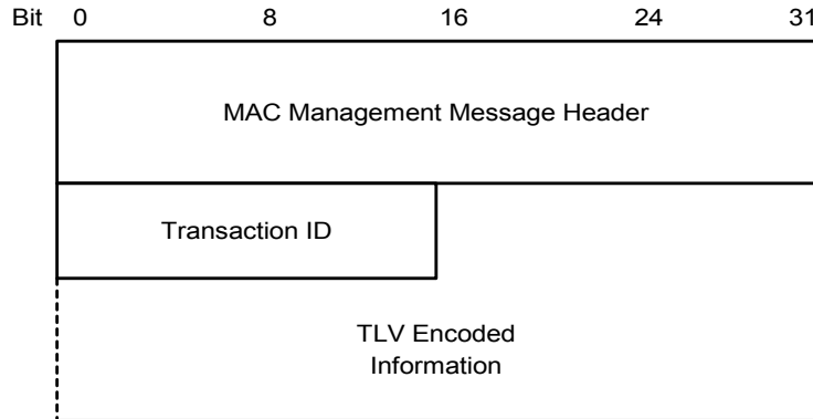
Figure 8–40 Dynamic Channel Change Acknowledge
