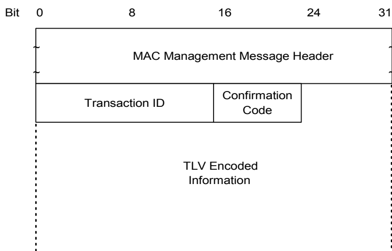
Figure 8–34 Dynamic Service Change — Response
