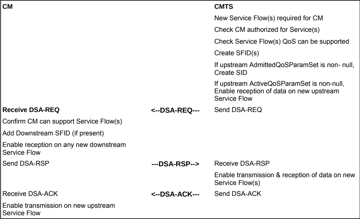
Figure 11–30 Dynamic Service Addition Initiated from CMTS
