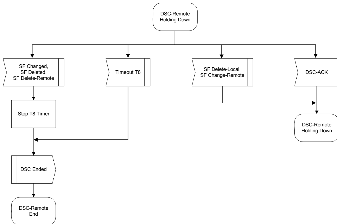
Figure 11-49 DSC—Remotely Initiated Transaction Holding Down State Flow Diagram
