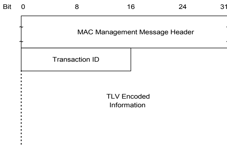
Figure 8-30 Dynamic Service Addition — Request
