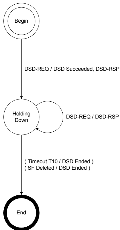
Figure 11–28 Dynamic Deletion (DSD) - Remotely Initiated Transaction State Transition Diagram
