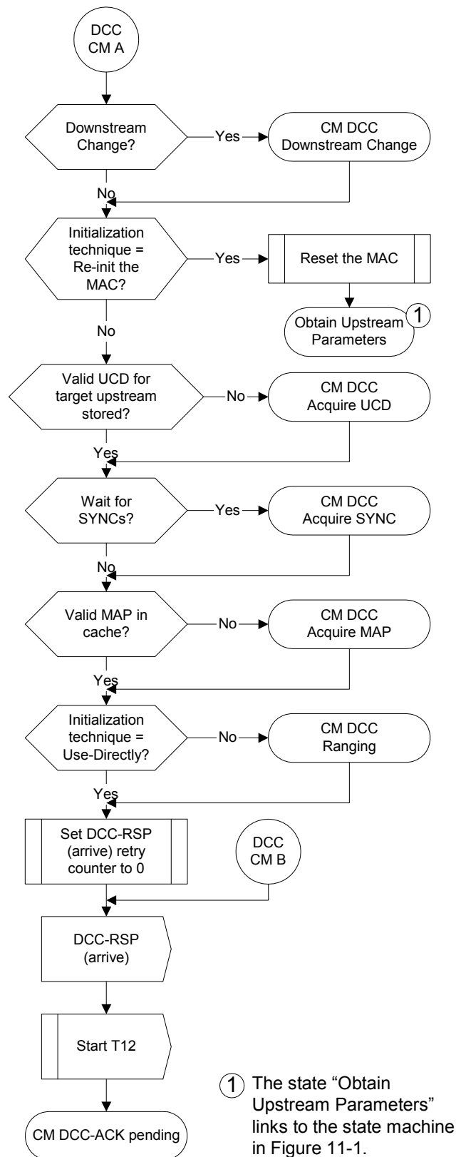
Figure 11–63 Dynamically Channels: CM View Part 2
