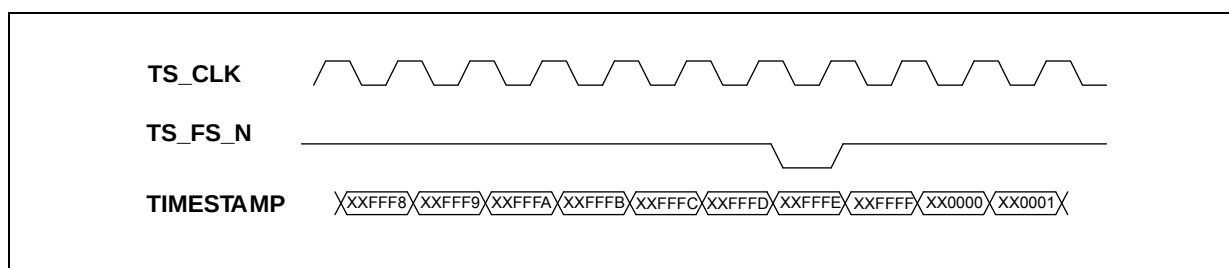
Figure H-5 Counter Synchronization
