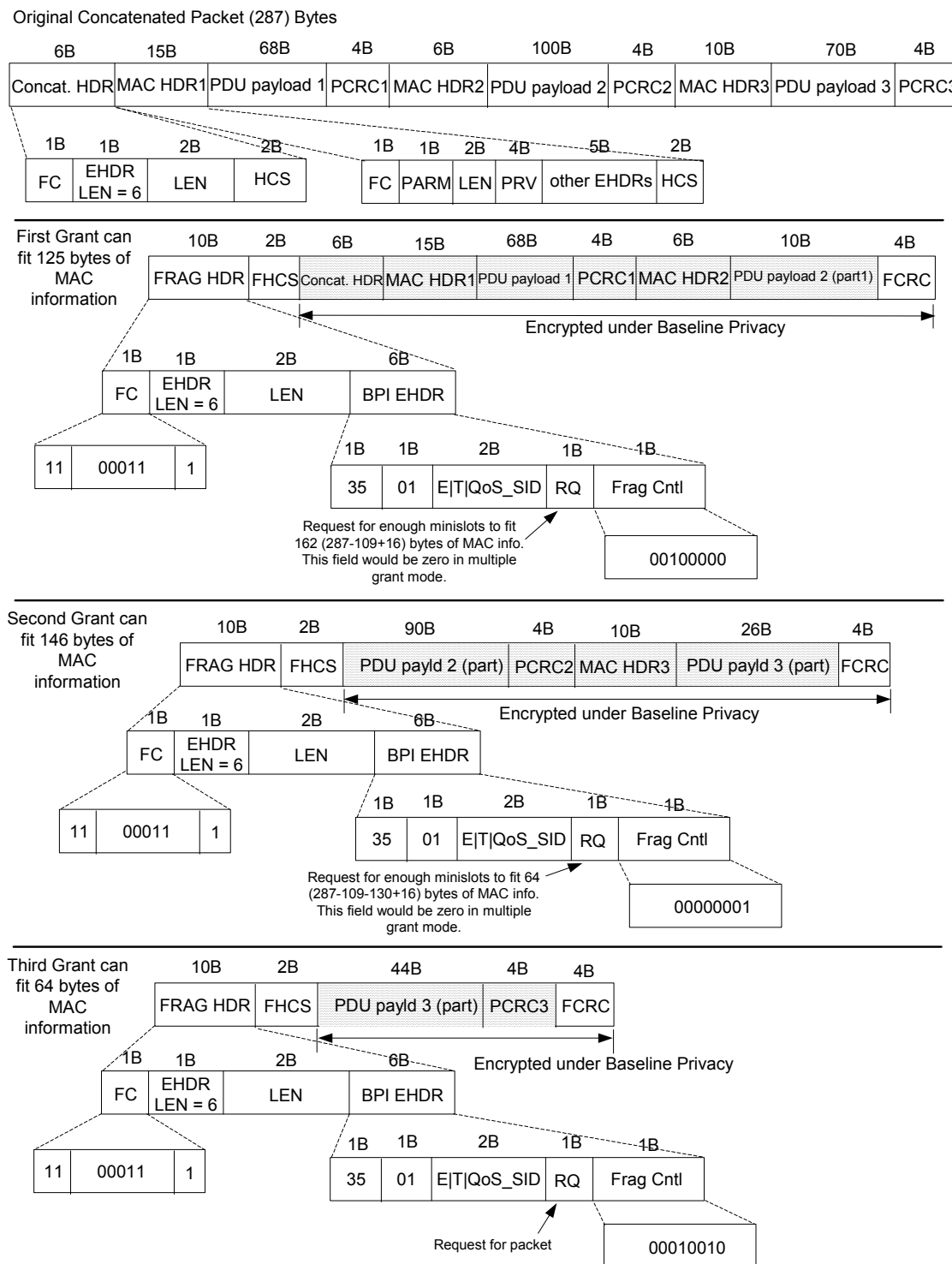
Figure 10–10 Fragmented Concatenated Packet Example
