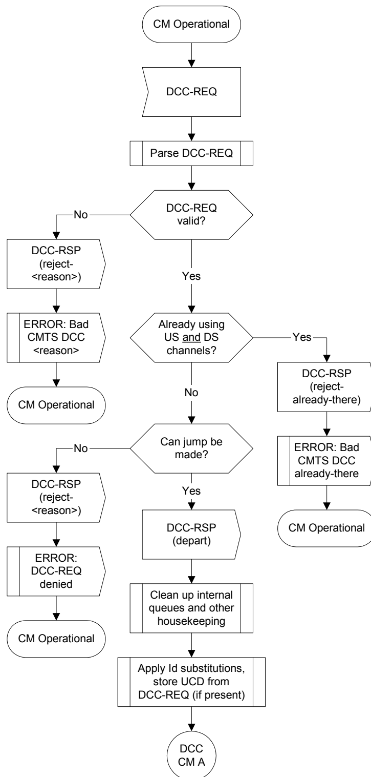
Figure 11–62 Dynamically Changing Channels: CM View Part 1
