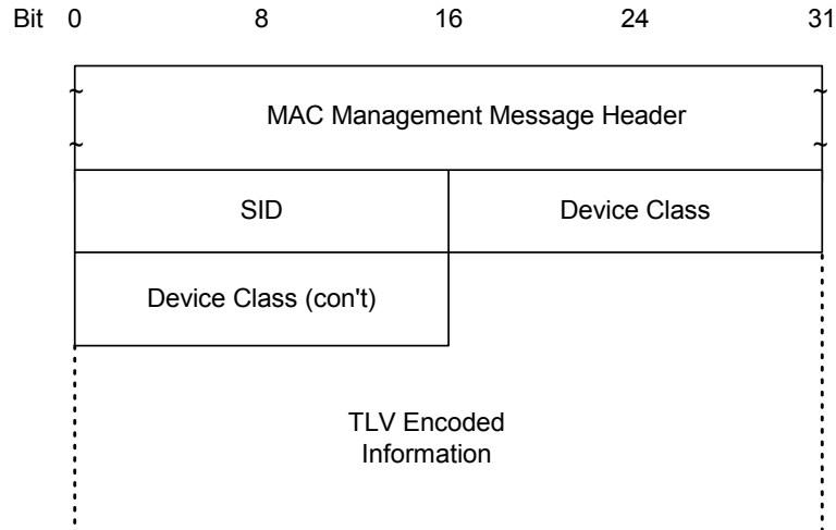
Figure 8–41 Device Class Identification Request
