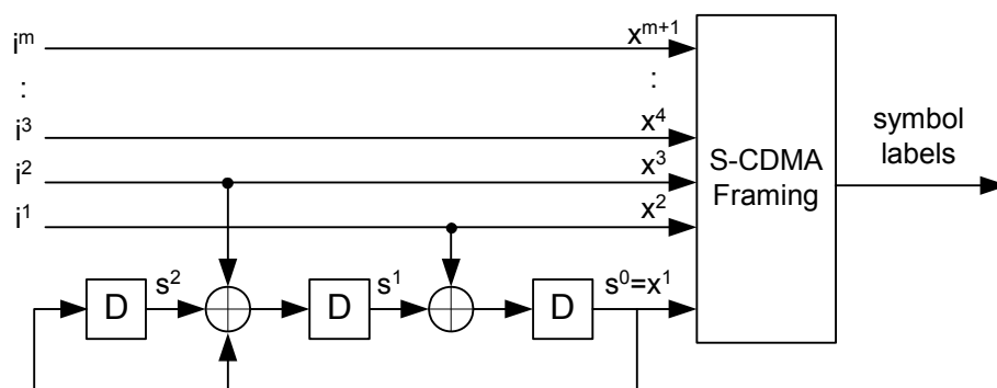
Figure 6–8 Convolutional encoder
