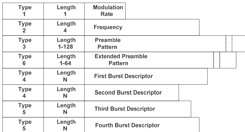
Figure 8–18 Example of UCD Encoded TLV Data
