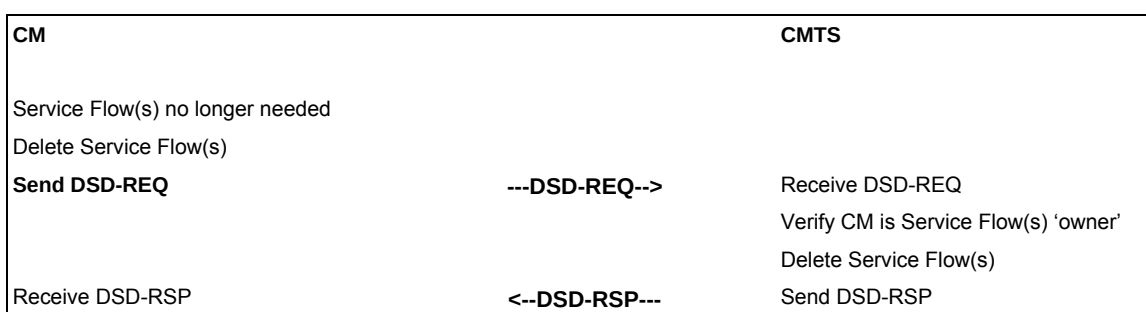
Figure 11–51 Dynamic Service Deletion Initiated from CM
