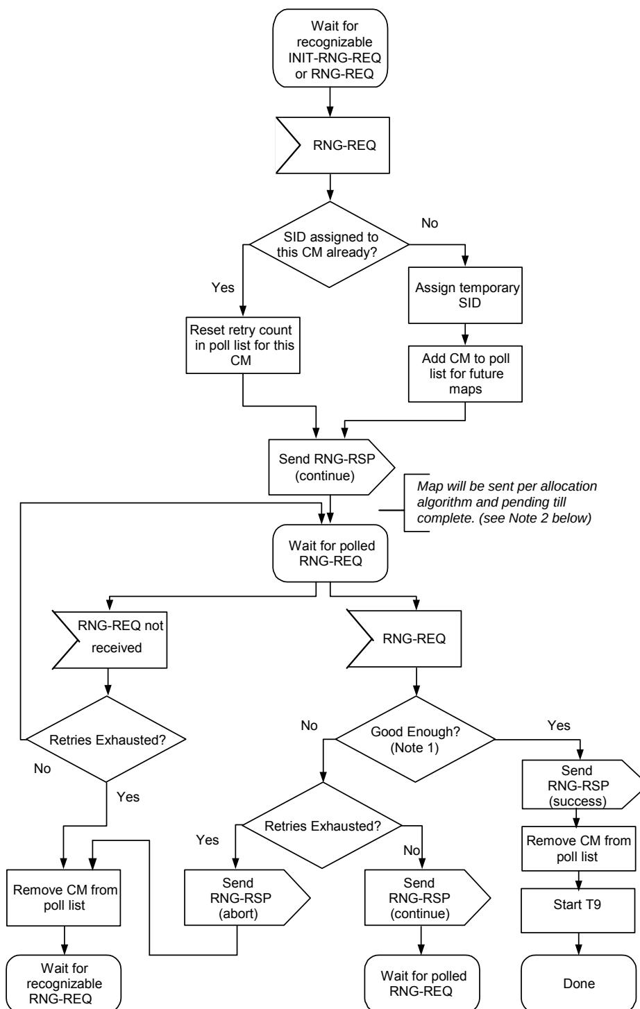
Figure 11-8 Initial Ranging - CMTS 123
