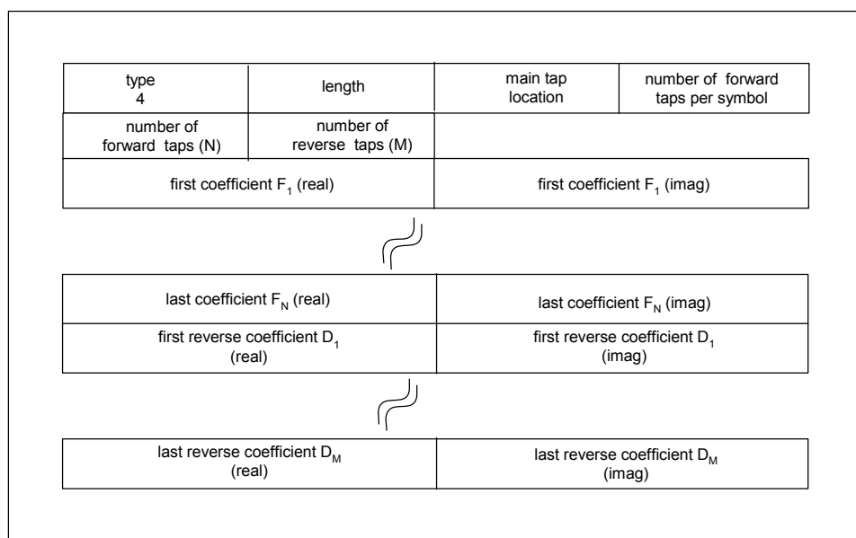
Figure 8–23 Generalized Decision Feedback Equalization Coefficients
