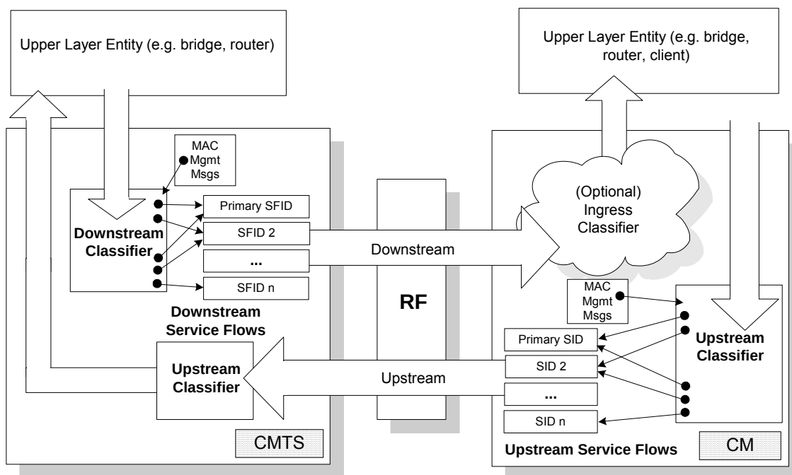
Figure 10-3 Classification within the MAC Layer
