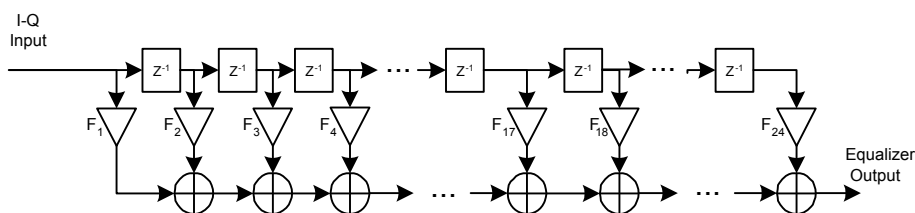
Figure 6-28 Transmit Pre-Equalizer Structure
