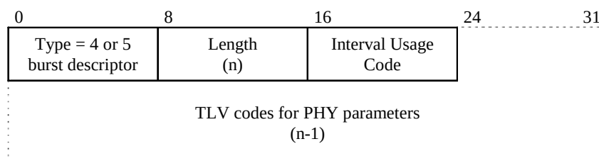
Figure 8-17 Top-Level Encoding for Burst Descriptors
