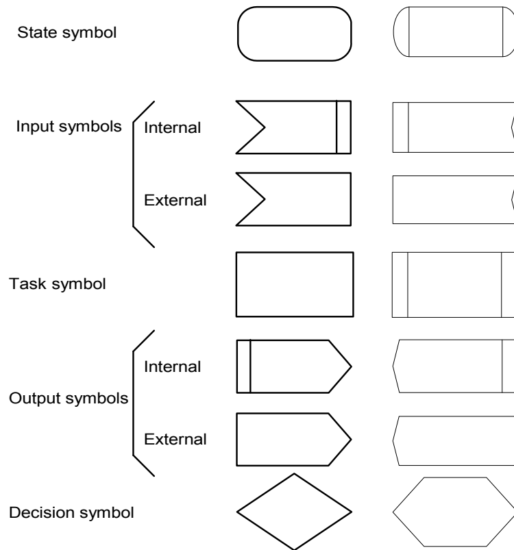
Figure 11-2 SDL Notation
