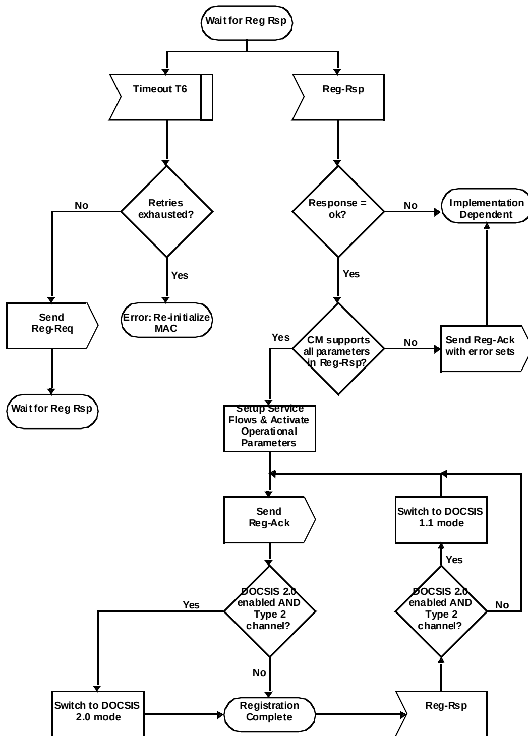
Figure 11–13 Wait for Registration Response — CM 126
