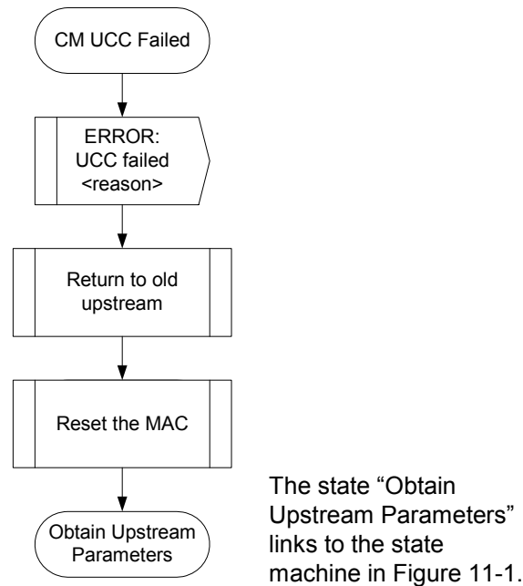
Figure 11–20 Changing Upstream Channels: CM View Part 2
