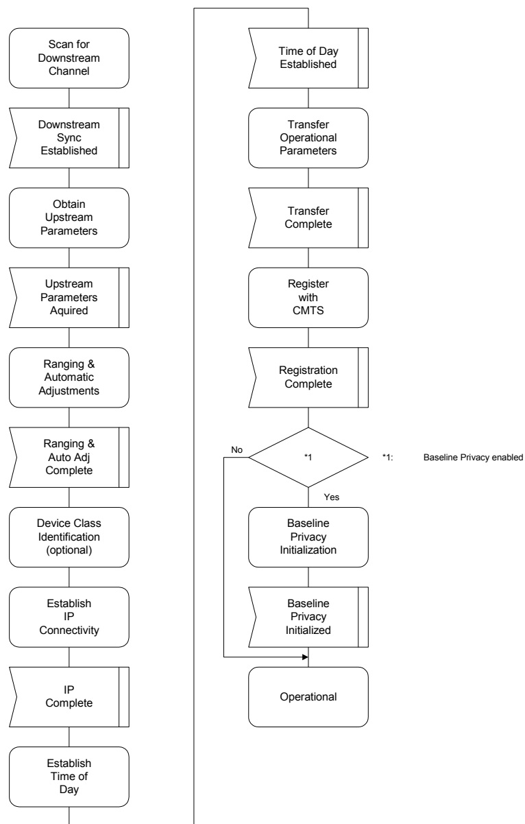
Figure 11–1 CM Initialization Overview
