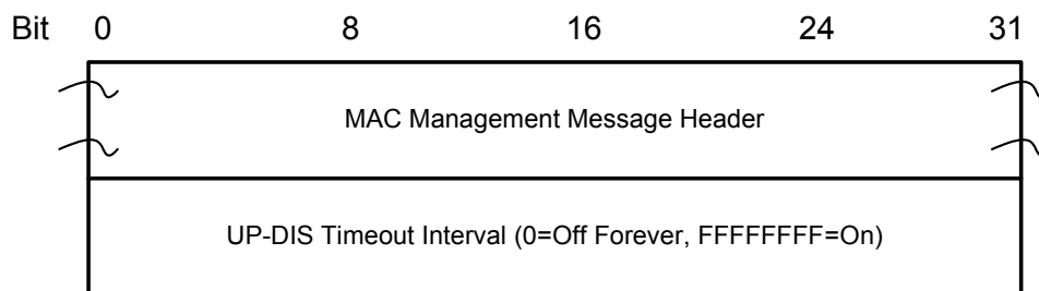
Figure 8–43 UP-DIS message format
