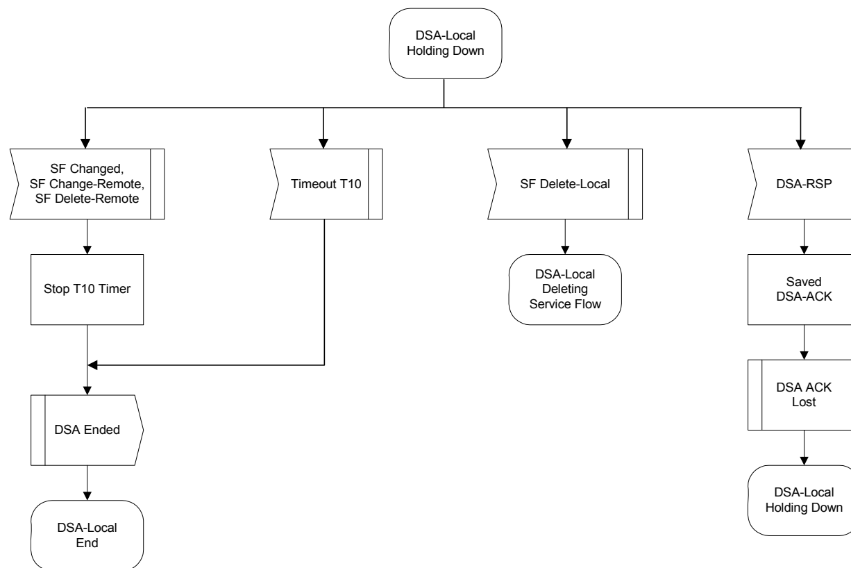
Figure 11–55 DSD—Locally Initiated Transaction Holding Down State Flow Diagram
