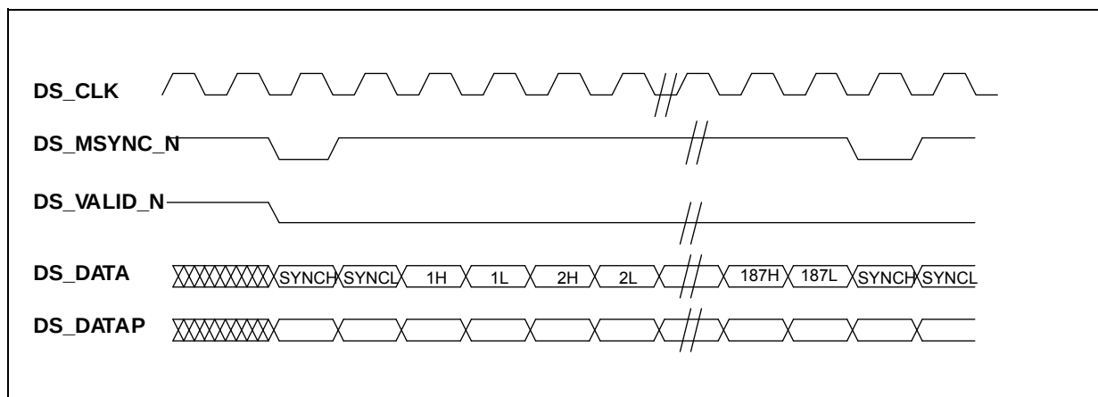
Figure H–3 Downstream Data Signal Protocol for ITU-T Recommendations J.83 Annex B Operation
