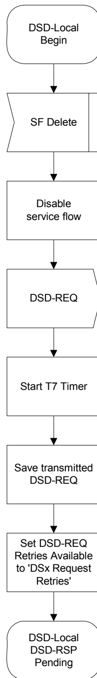
Figure 11–53 DSD—Locally Initiated Transaction Begin State Flow Diagram
