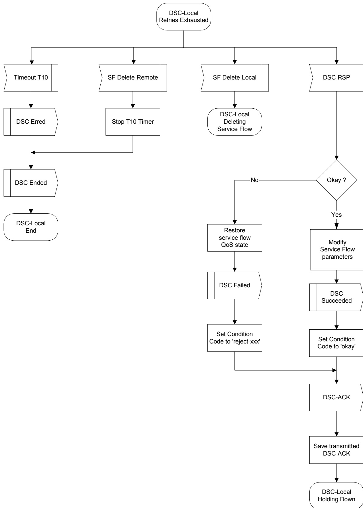
Figure 11–45 DSC—Locally Initiated Transaction Retries Exhausted State Flow Diagram
