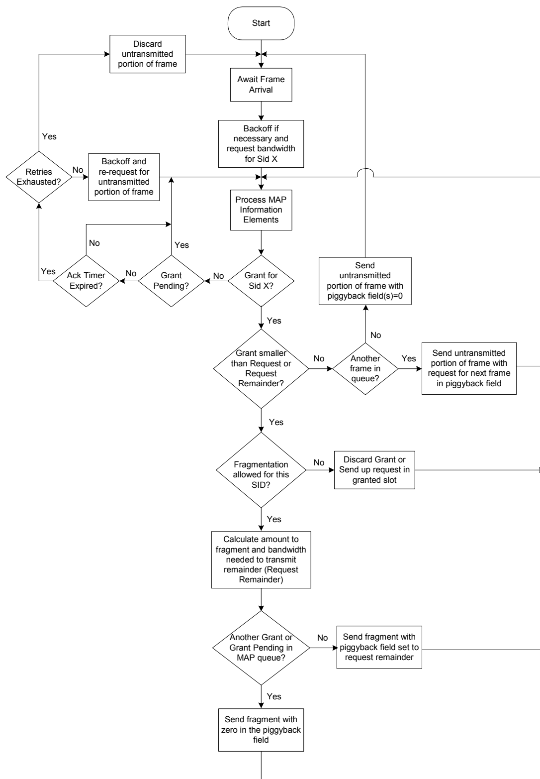
Figure 10–8 CM Fragmentation Flowchart 114
