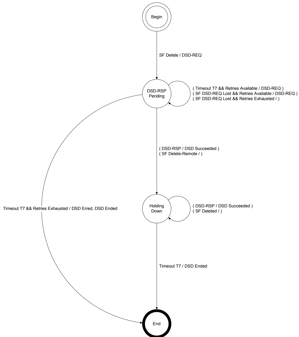
Figure 11–27 DSD—Locally Initiated Transaction State Transition Diagram
