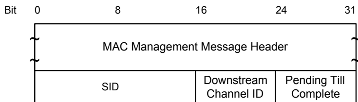
Figure 8–21 Packet PDU Following the Timing Header
