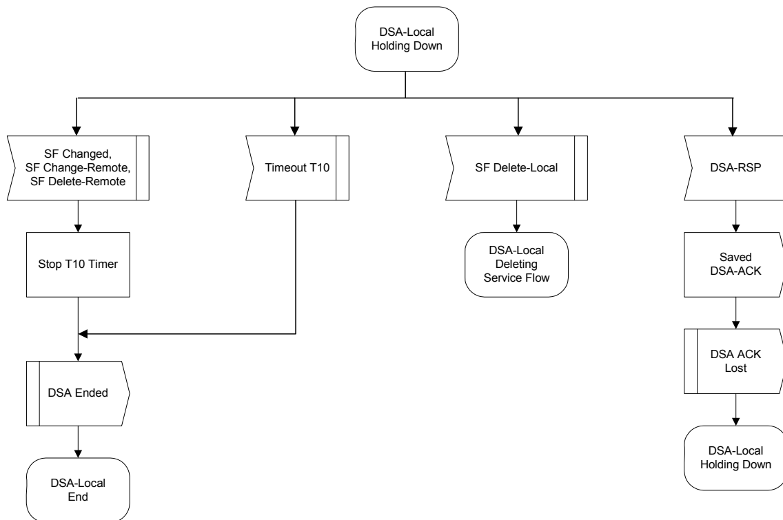
Figure 11–33 DSA—Locally Initiated Transaction Holding State Flow Diagram
