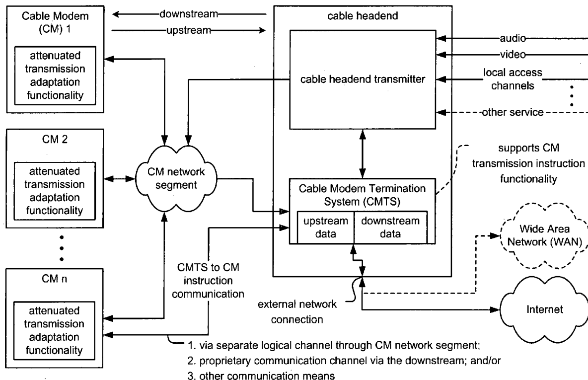
cable modem communication system 100
