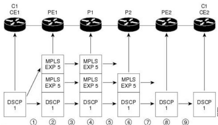
Figure 4: Short Pipe Mode Operation
