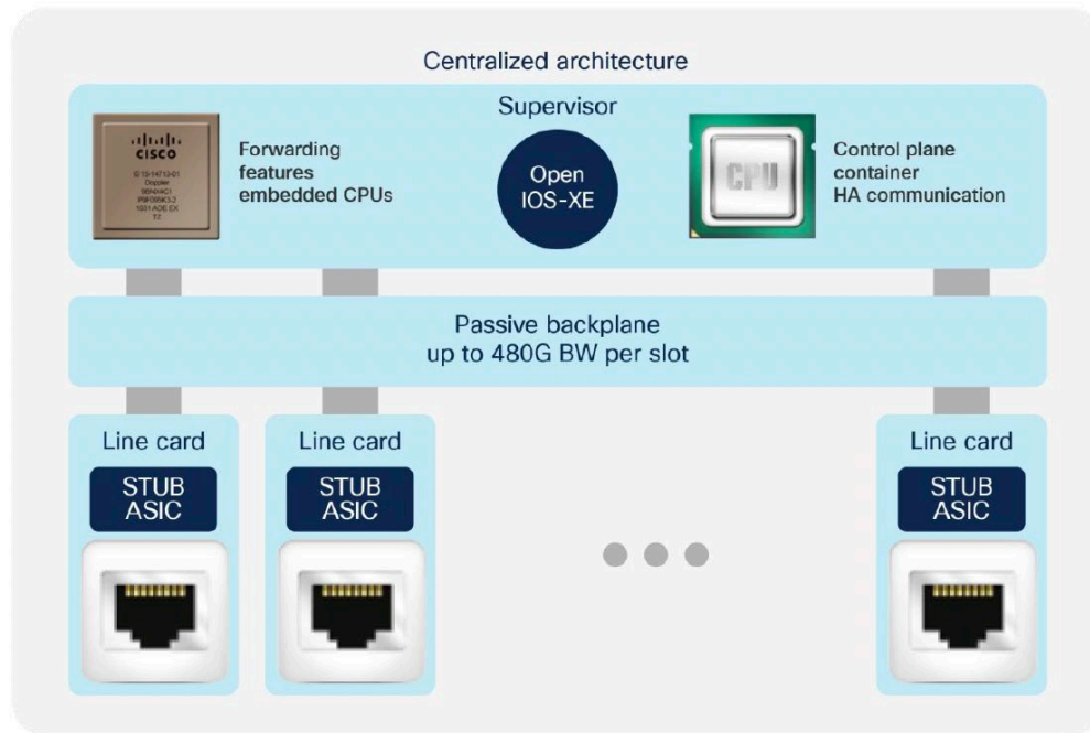
Figure 5. Cisco Catalyst 9400 Series architecture
