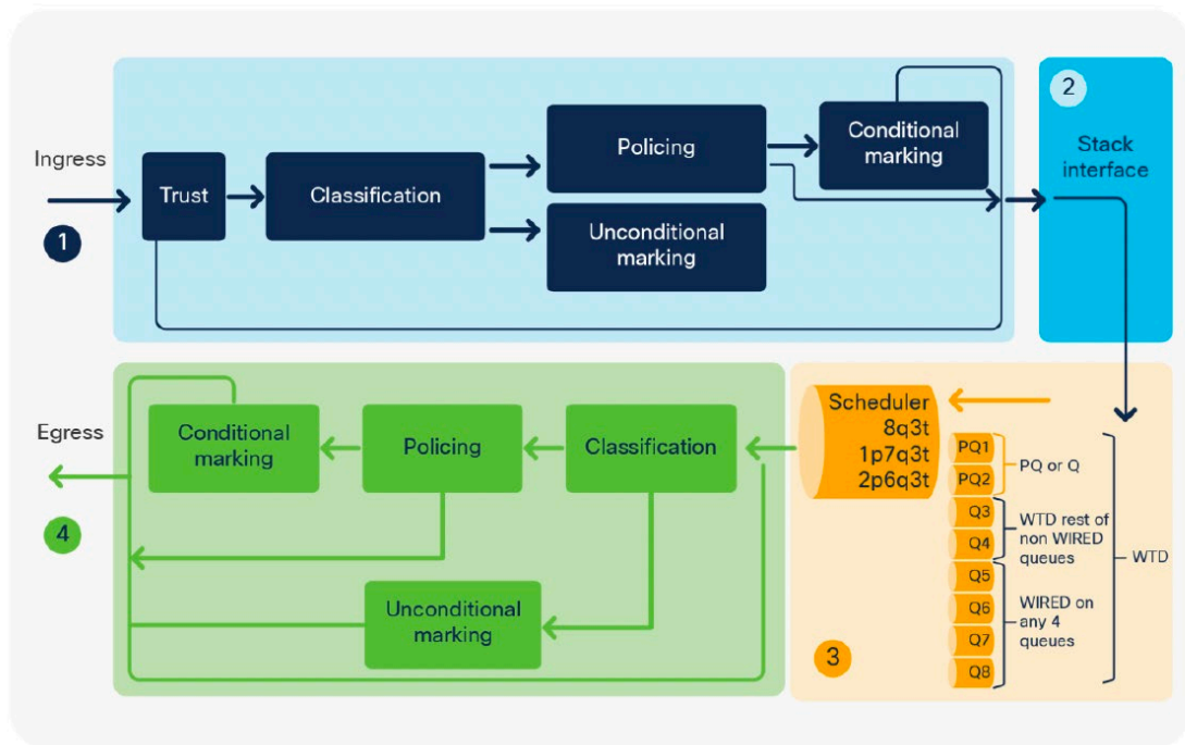
Figure 12. QoS tools per ASIC block
