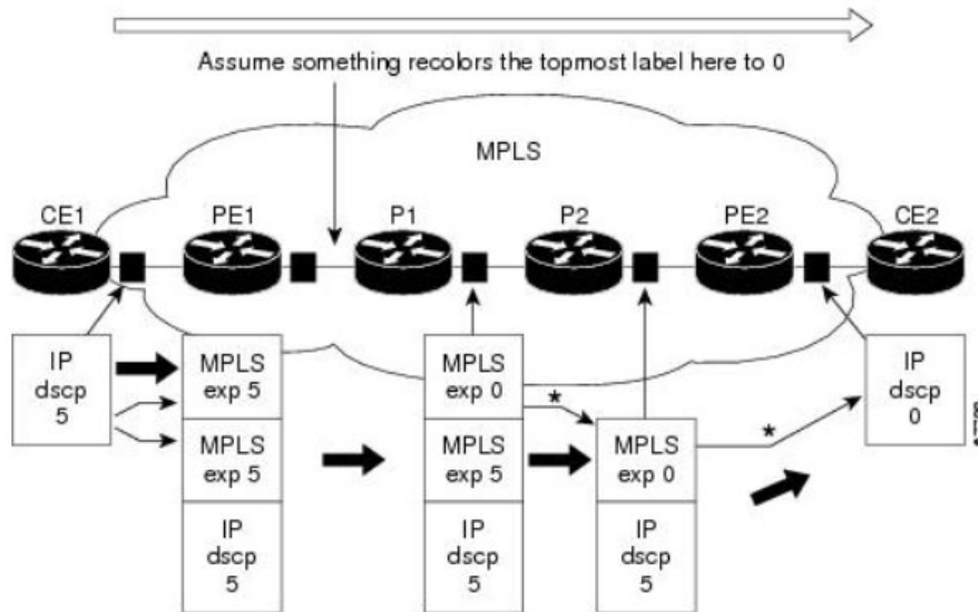
Figure 5: Uniform Mode Operation
