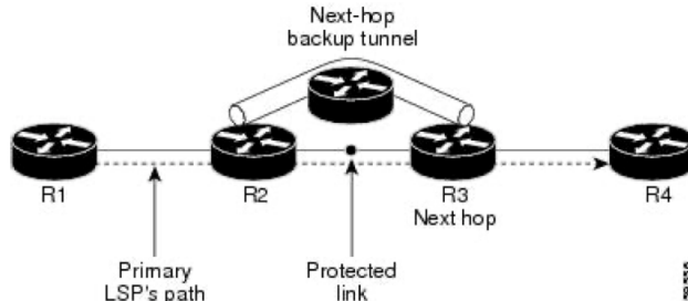
Figure 1 NHOP Backup Tunnel
