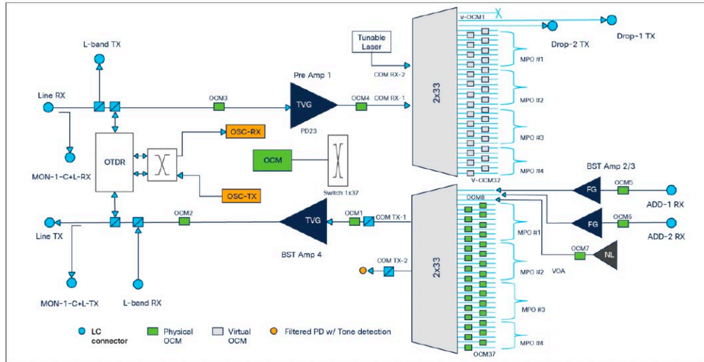
Figure 3. NCS 1010 OLT-C functional layout
