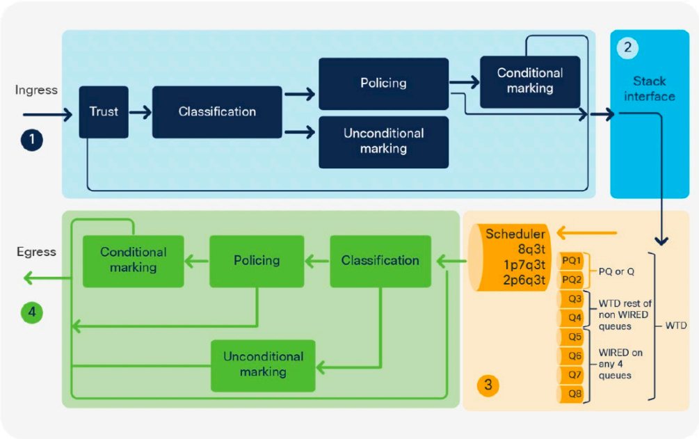
Figure 12. QoS tools per ASIC block
