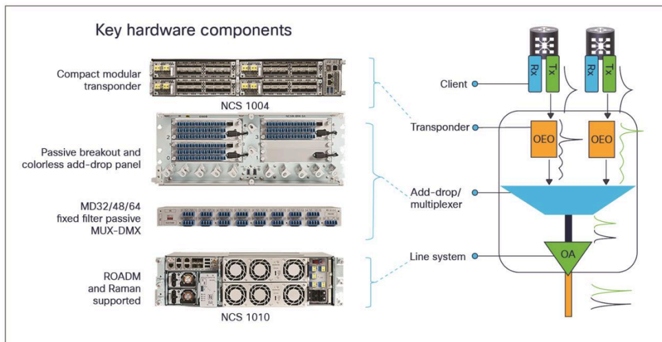
Figure 1. NCS 1010 solution components
