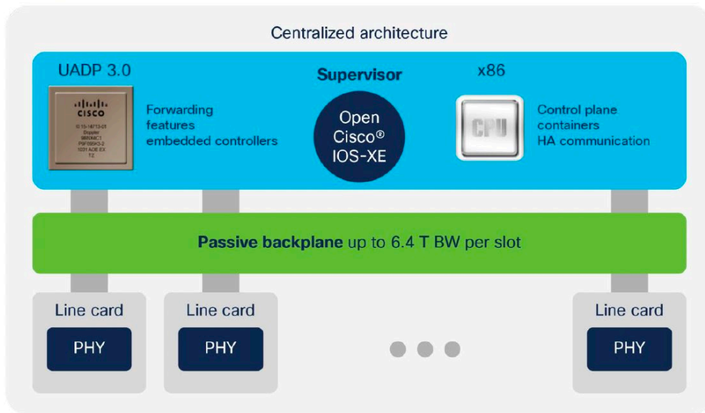
Figure 9. Cisco Catalyst 9600 Series architecture
