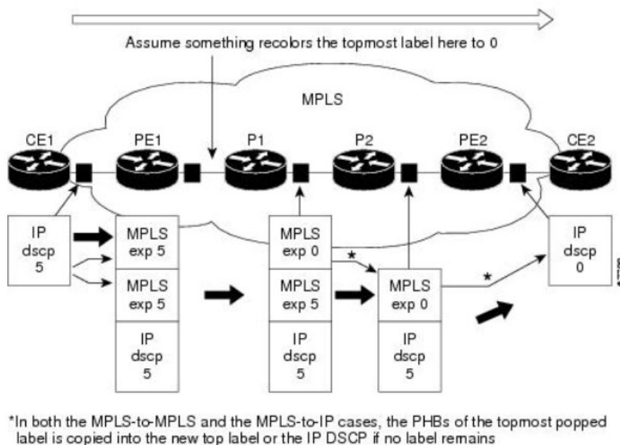
Figure 5: Uniform Mode Operation
