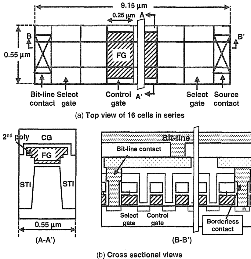
FIGURE 3.14 Schematic view of the SA-STI cell with floating-gate (FG) wing. (a) Top view of 16 cells in series. (b) Cross-sectional views of A-A' and B-B' in (a). Three key technologies to achieve 5 \cdot F^2 (F: feature size) cell size has been introduced. (1) A stacked floating-gate structure has been applied in order to reduce the gate space aspect. A first poly-Si gate is self-aligned with the active area. A second poly-Si gate is formed over the exposed first gate to achieve a high coupling ratio ( >0.6 ) with floating-gate wing. (2) The second poly-Si gate has been patterned with spacing of 0.15 \mu\text{m} by a novel SiN spacer process. This process has made it possible to realize 0.55\text{-}\mu\text{m} -pitch isolation. (3) The borderless bit-line and source-line contacts which are self-aligned with the select gate can eliminate a space between the contacts and the gate.
