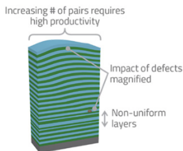
Fig. 6: Film stack deposition challenges. Source: Lam Research.
