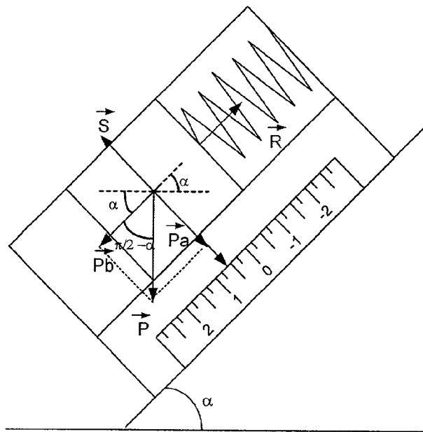
Figure 6: Accelerometer laying at an angle
