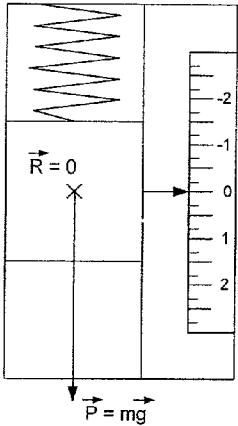
Figure 5: System in free fall
