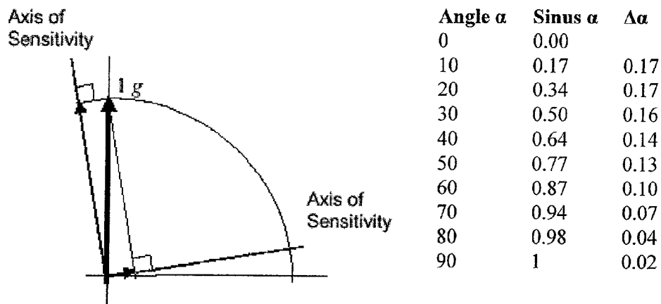
Figure 7 Axes of sensitivity
