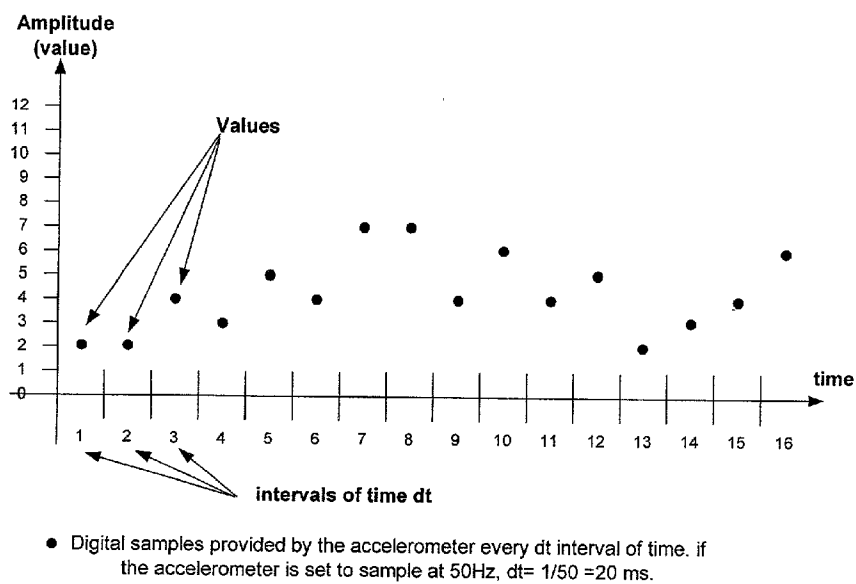
Figure 19: Example of digital samples captured by the accelerometer at 50Hz
