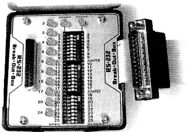
Breakout box.
