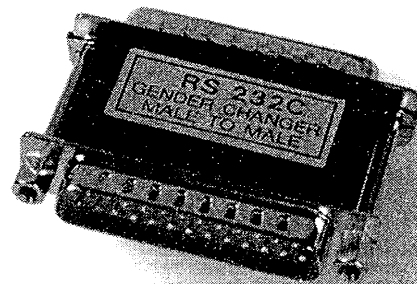
Gender changer.
