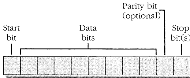
Asynchronous transmission. The coding of a typical character sent in asynchronous transmission.
