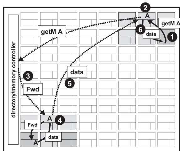
FIGURE 6-9. VH_{Dir-Dir} Example. VH_{Dir-Dir} 's second-level coherence (dashed lines) facilitates VM reassignment and content-based page sharing.
