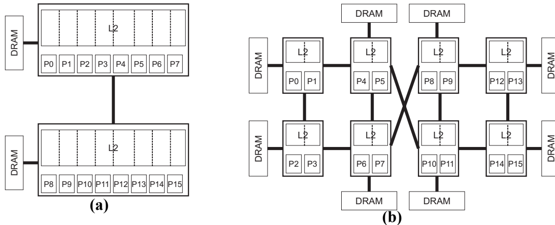
FIGURE 5-7. Alternative 16-core M-CMP Configurations.
