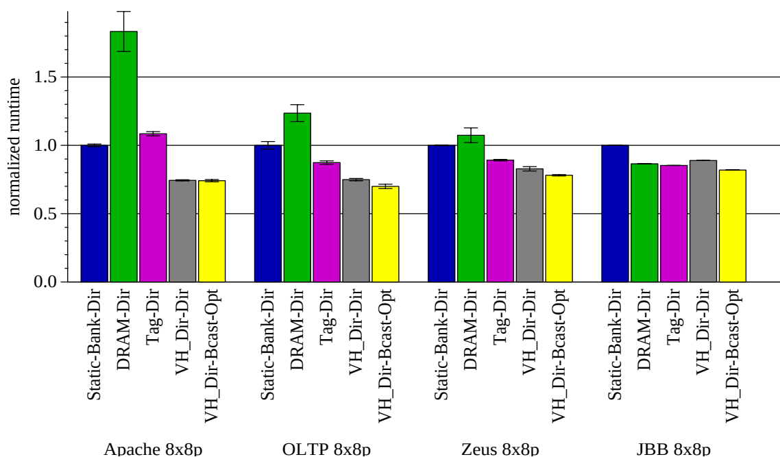
FIGURE 6-12. Normalized Runtime for 8x8p Homogeneous Consolidation.
