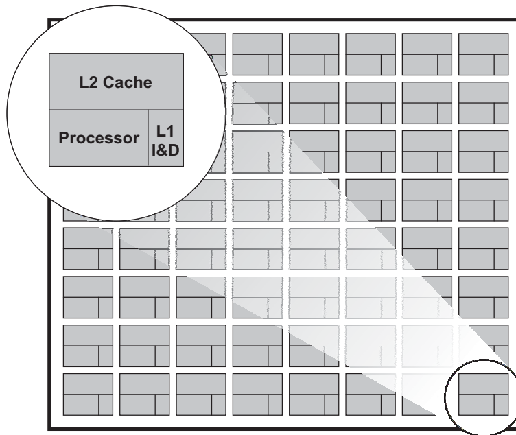
FIGURE 1-3. CMP Design for the Virtual Hierarchies work of Chapter 6
