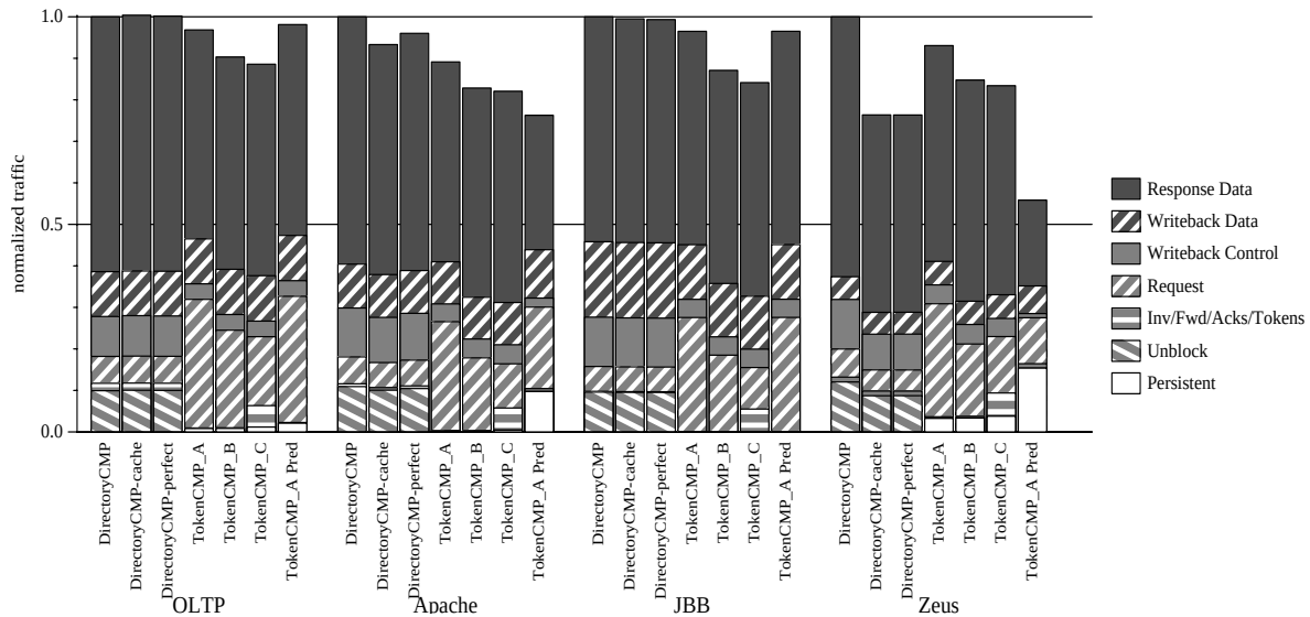
FIGURE 5-5. Normalized Intra-CMP Traffic.
