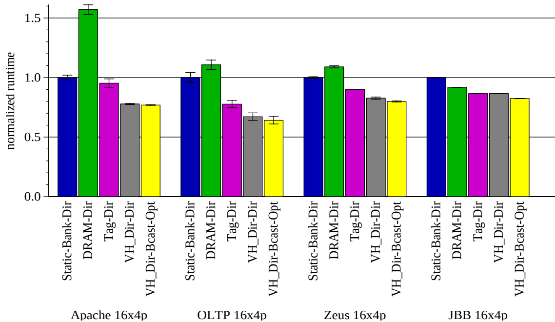
FIGURE 6-15. Normalized Runtime for 16x4p Homogeneous Consolidation.
