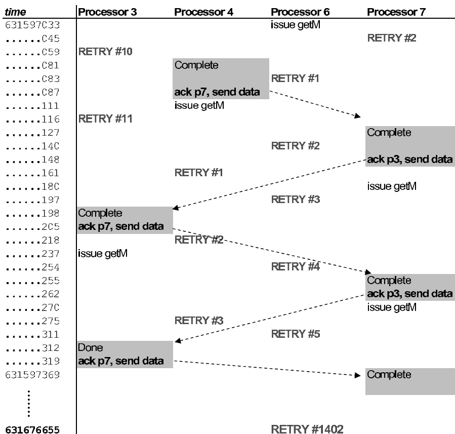
FIGURE 4-11. Excerpt of a GREEDY-ORDER trace running OMPmgrid for a single cache block. . Processor 6's request is pathologically starved for over 75,000 cycles.
