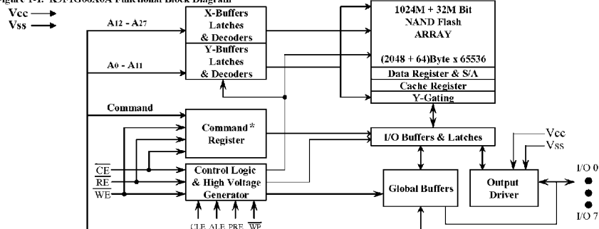
Figure 2-1. K9F1G08X0A (X8) Organization
