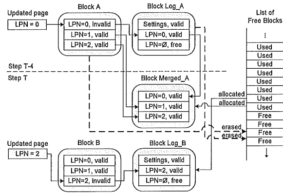
Figure 9: Memorex device page update. Using hybrid mapping and a full merge operation during garbage collection. LPN = Logical Page Number. LPN 2 is written to the log block of block B and the original LPN 2 marked invalid. If this requires a new log block, an old log block (Log_A) must be freed by doing a merge with its corresponding data block.
