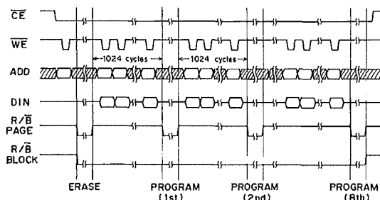
Fig. 8. Switching waveforms of block-page mode.
