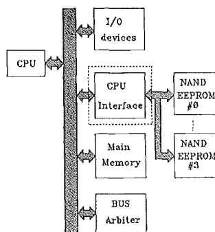
Fig. 14. Block diagram of computer system with NAND EEPROM's.
