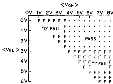
Fig. 10. Schmo plot of test READ mode.
