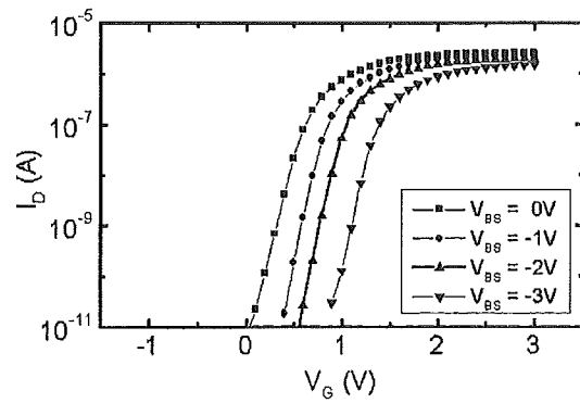
Fig. 5. SSL transistor I_d - V_g characteristic with various body bias.
