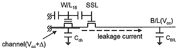
Fig. 4. Schematic of W/L_{15} to SSL coupling.
