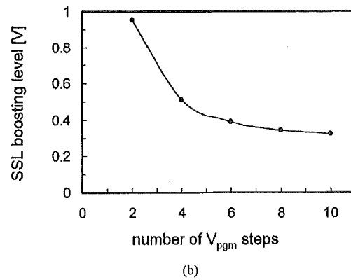
Fig. 6. Peak coupling between W/L_{15} and string-select-line transistor with (a) V_{pgm} rising time and (b) the number of V_{pgm} steps within 5 \mu s at a ISPP step.
