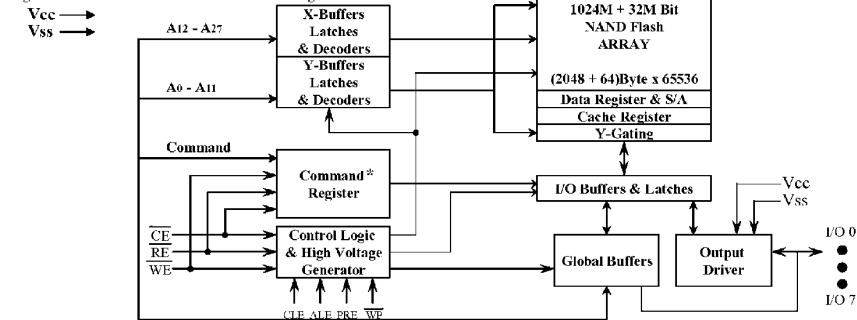
Figure 2-1. K9F1G08X0A (X8) Organization
