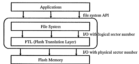
Fig. 1. Overall architecture of flash memory system.
