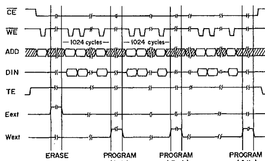
Fig. 12. Switching waveforms of test erase/program mode.
