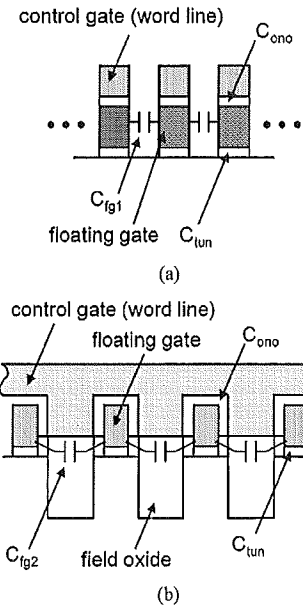
Fig. 10. Schematic cross-sectional view of the NAND flash memory cell array and the parasitic capacitance between adjacent two floating gates. (a) C_{fg1} in the bitline direction. (b) C_{fg2} in the wordline direction.
