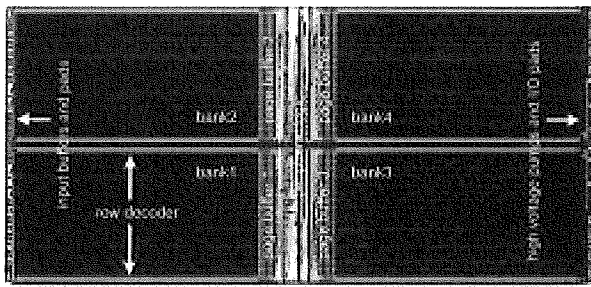
Fig. 1. Chip micrograph.
