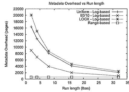
Figure 11: Metadata overhead versus run length.
